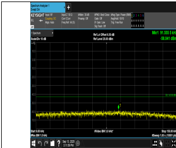
EGPRS1900-512-2-0.009~0.15MHz-PASS
