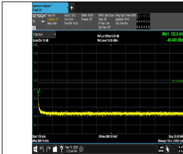
EGPRS1900-661-2-0.15~30MHz-PASS
