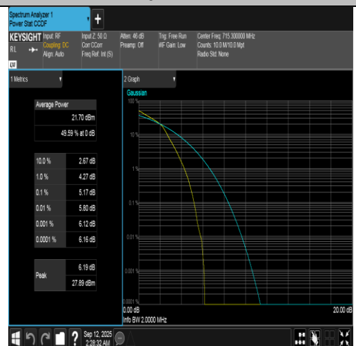
Band12-1.4MHz-16QAM-23173-6RB#0-PASS
