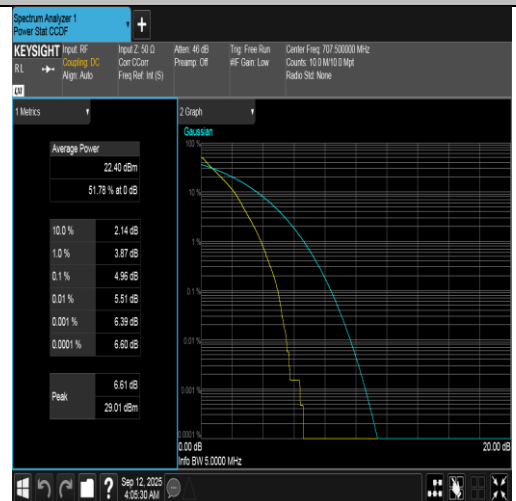
Band12-5MHz-QPSK-23095-25RB#0-PASS
