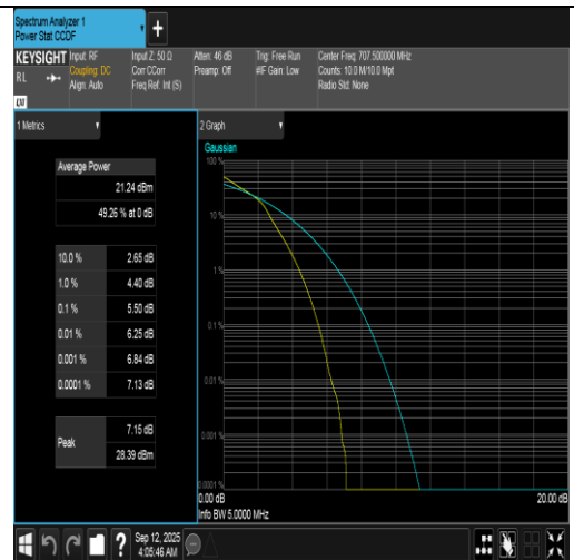
Band12-5MHz-16QAM-23095-25RB#0-PASS
