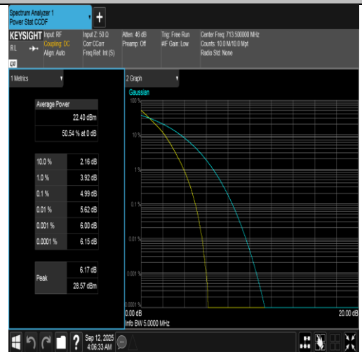
Band12-5MHz-QPSK-23155-25RB#0-PASS
