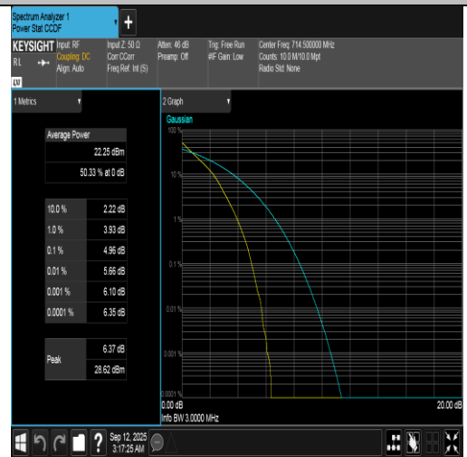
Band12-3MHz-QPSK-23165-15RB#0-PASS
