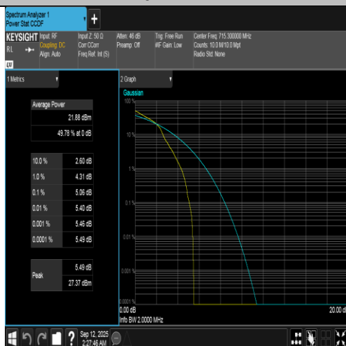
Band12-1.4MHz-16QAM-23173-1RB#0-PASS
