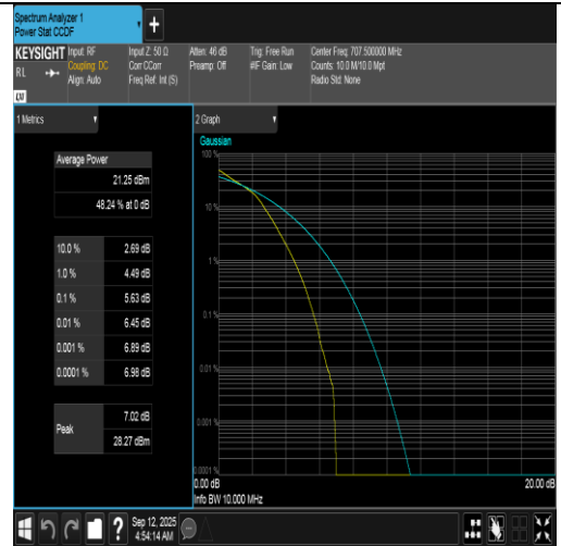
Band12-10MHz-16QAM-23095-50RB#0-PASS
