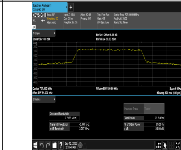
Band12-3MHz-16QAM-23095-15RB#0-PASS
