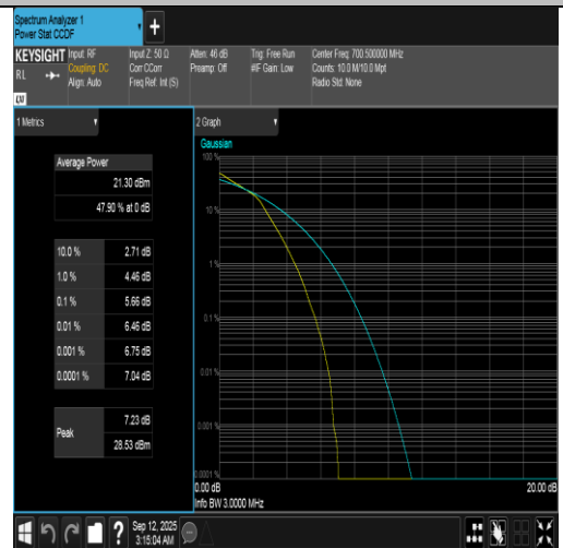
Band12-3MHz-16QAM-23025-15RB#0-PASS
