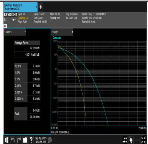
Band12-10MHz-QPSK-23130-50RB#0-PASS
