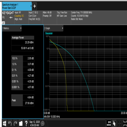
Band12-10MHz-QPSK-23130-1RB#0-PASS
