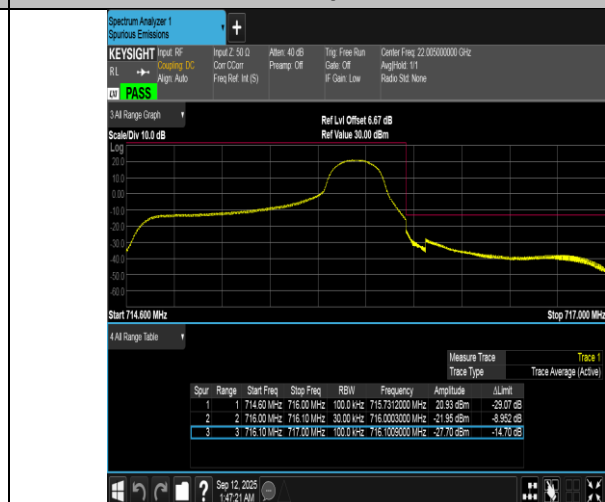
Band12-1.4MHz-QPSK-23173-1RB#5-PASS
