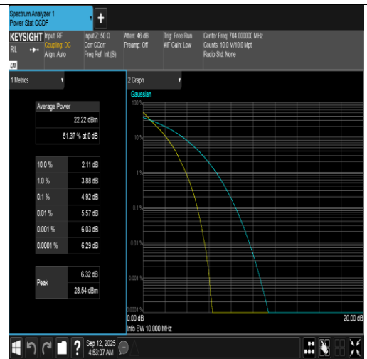
Band12-10MHz-QPSK-23060-50RB#0-PASS
