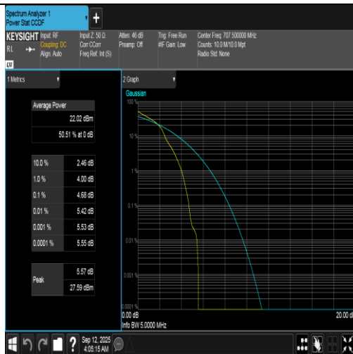
Band12-5MHz-16QAM-23095-1RB#0-PASS
