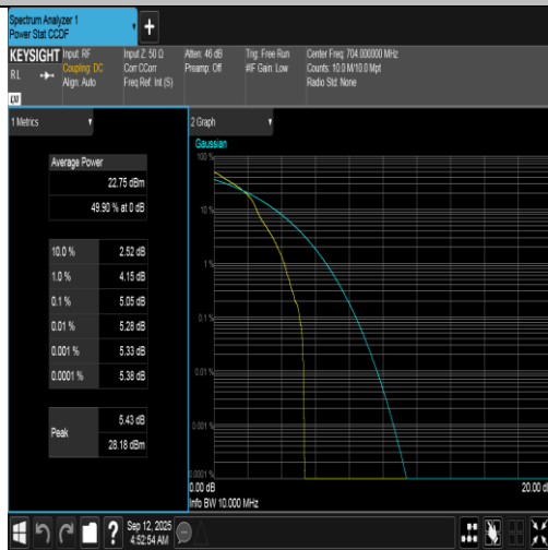
Band12-10MHz-16QAM-23060-1RB#0-PASS
