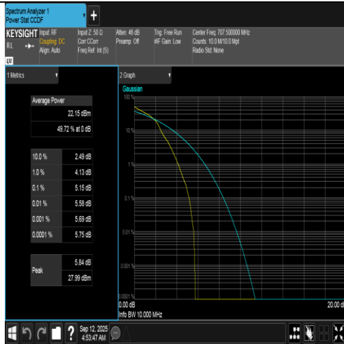
Band12-10MHz-16QAM-23095-1RB#0-PASS
