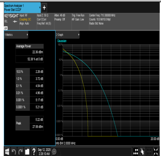
Band12-1.4MHz-QPSK-23173-6RB#0-PASS
