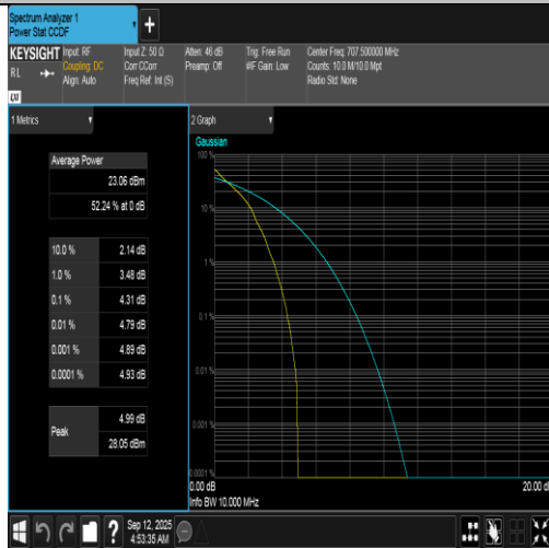
Band12-10MHz-QPSK-23095-1RB#0-PASS
