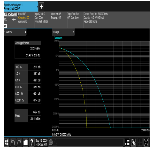
Band12-5MHz-QPSK-23035-25RB#0-PASS
