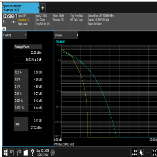
Band12-1.4MHz-16QAM-23095-1RB#0-PASS
