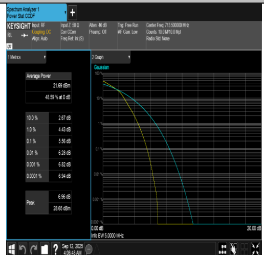
Band12-5MHz-16QAM-23155-25RB#0-PASS
