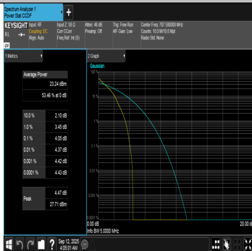
Band12-5MHz-QPSK-23095-1RB#0-PASS
