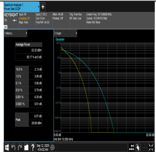
Band12-10MHz-QPSK-23095-50RB#0-PASS
