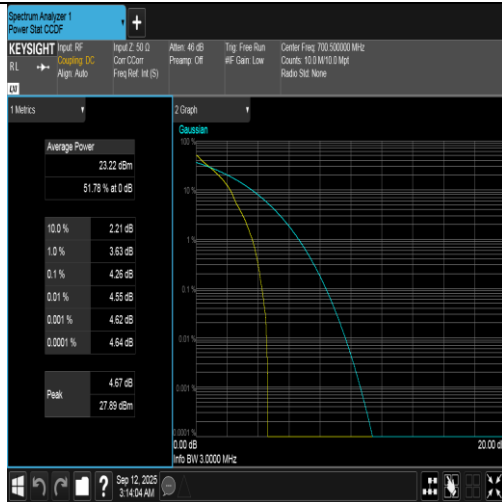
Band12-3MHz-QPSK-23025-1RB#0-PASS
