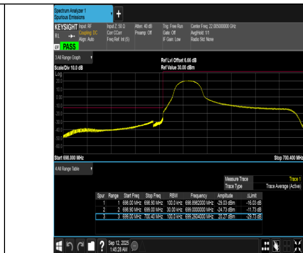
Band12-1.4MHz-16QAM-23017-1RB#0-PASS
