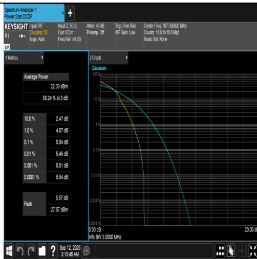
Band12-3MHz-16QAM-23095-1RB#0-PASS
