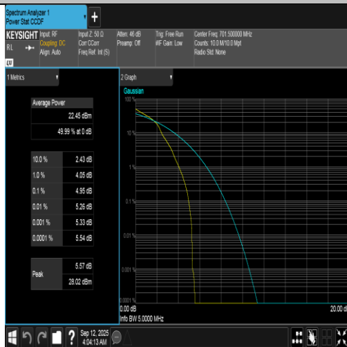
Band12-5MHz-16QAM-23035-1RB#0-PASS
