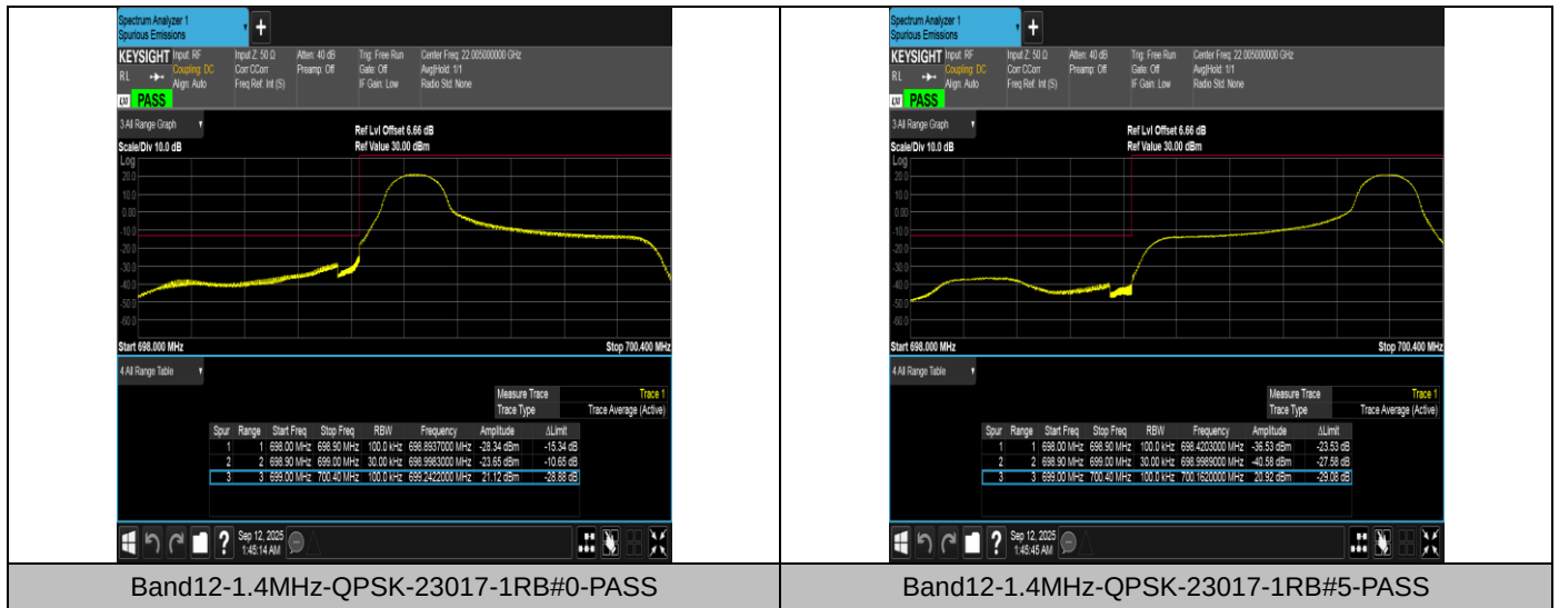
Band12-1.4MHz-QPSK-23017-1RB#0-PASS
