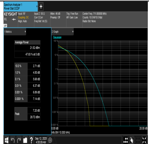
Band12-10MHz-16QAM-23130-50RB#0-PASS
