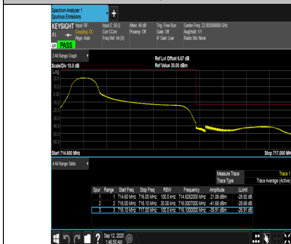
Band12-1.4MHz-QPSK-23173-1RB#0-PASS
