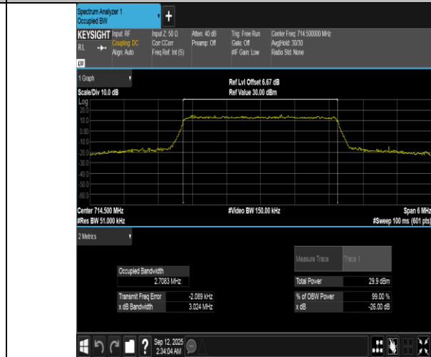
Band12-3MHz-16QAM-23165-15RB#0-PASS
