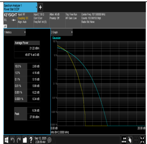
Band12-1.4MHz-16QAM-23095-6RB#0-PASS
