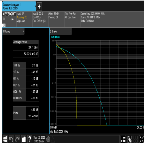
Band12-3MHz-QPSK-23095-1RB#0-PASS
