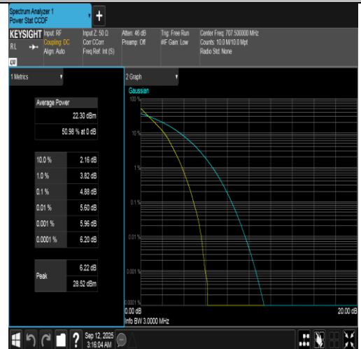
Band12-3MHz-QPSK-23095-15RB#0-PASS
