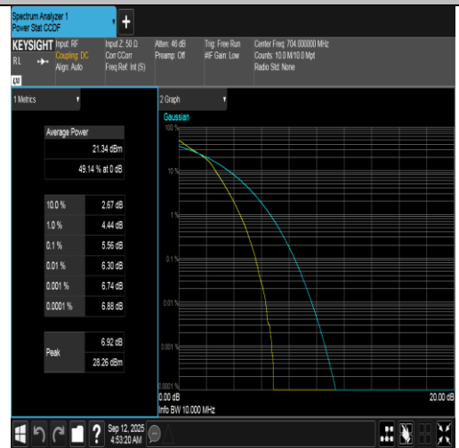
Band12-10MHz-16QAM-23060-50RB#0-PASS
