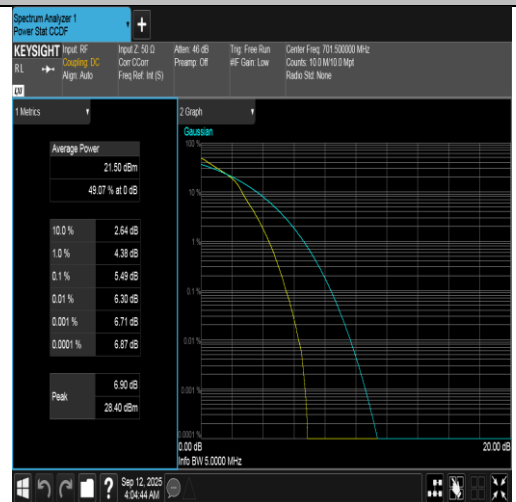
Band12-5MHz-16QAM-23035-25RB#0-PASS
