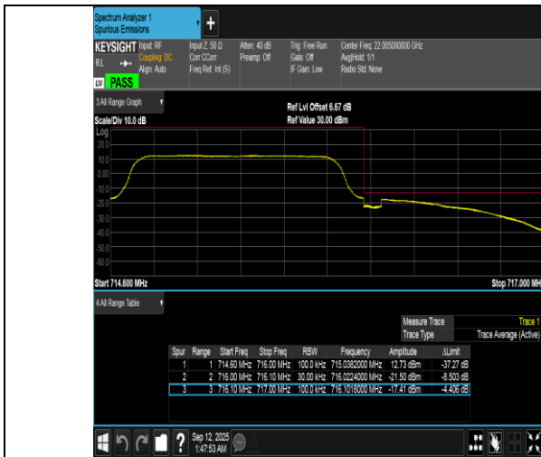
Band12-1.4MHz-QPSK-23173-6RB#0-PASS
