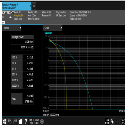
Band12-1.4MHz-QPSK-23173-1RB#0-PASS
