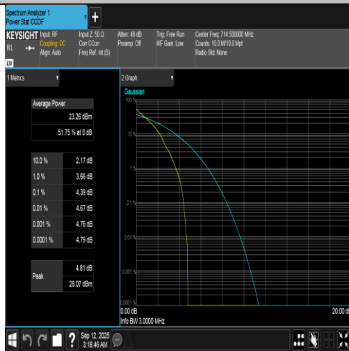
Band12-3MHz-QPSK-23165-1RB#0-PASS
