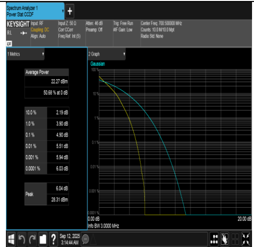
Band12-3MHz-QPSK-23025-15RB#0-PASS
