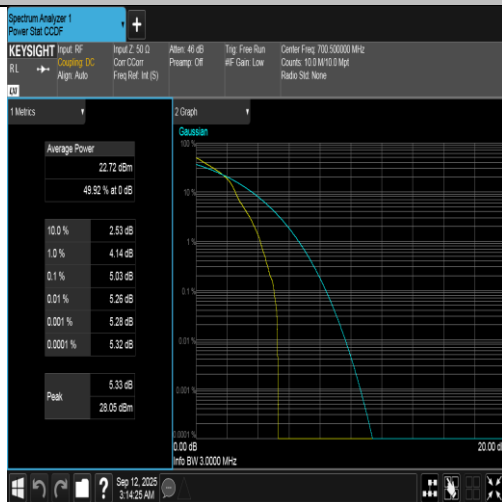
Band12-3MHz-16QAM-23025-1RB#0-PASS
