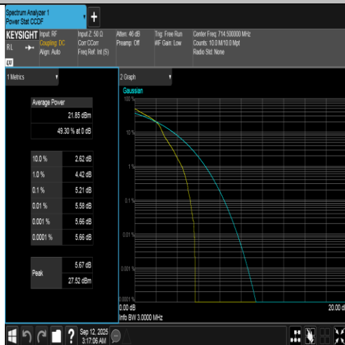
Band12-3MHz-16QAM-23165-1RB#0-PASS
