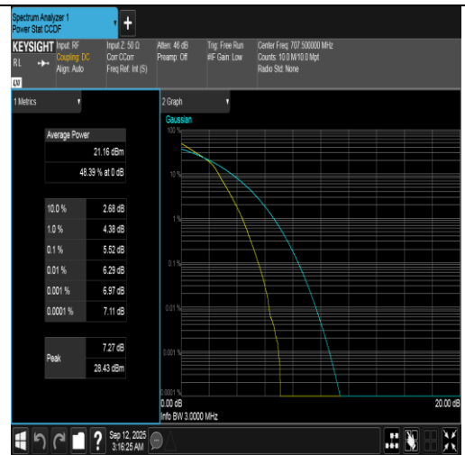
Band12-3MHz-16QAM-23095-15RB#0-PASS
