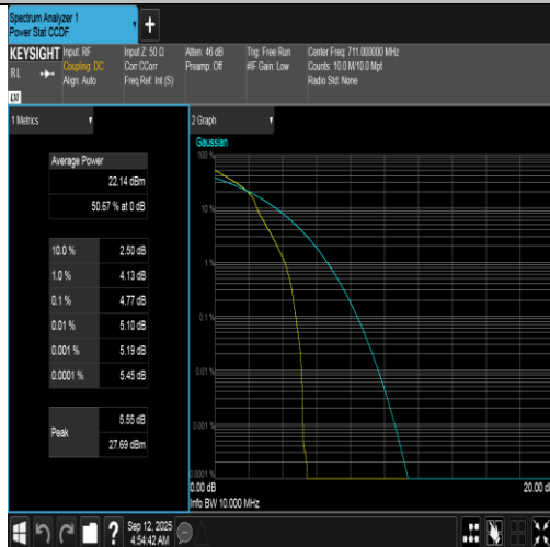
Band12-10MHz-16QAM-23130-1RB#0-PASS
