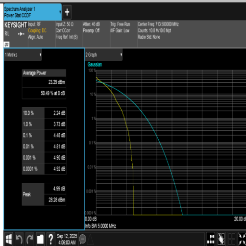
Band12-5MHz-QPSK-23155-1RB#0-PASS
