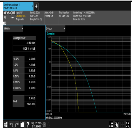
Band12-3MHz-16QAM-23165-15RB#0-PASS
