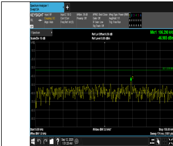
Band12-1.4MHz-16QAM-23017-1RB#5-0.009~0.15-PASS
