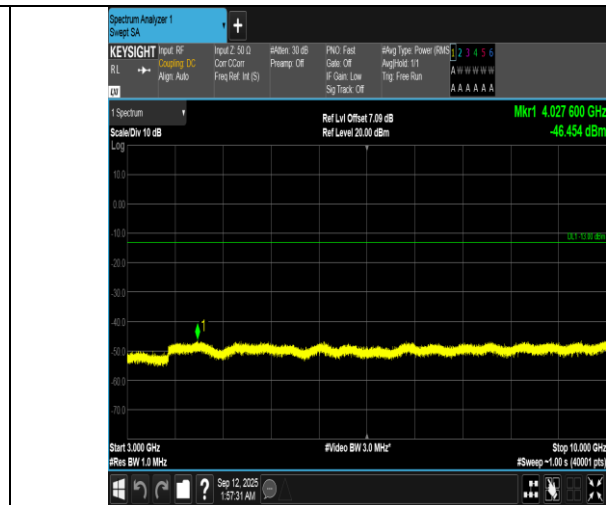
Band12-1.4MHz-QPSK-23095-1RB#5-3000-10000-PASS
