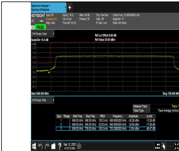
Band12-10MHz-QPSK-23060-50RB#0-PASS
