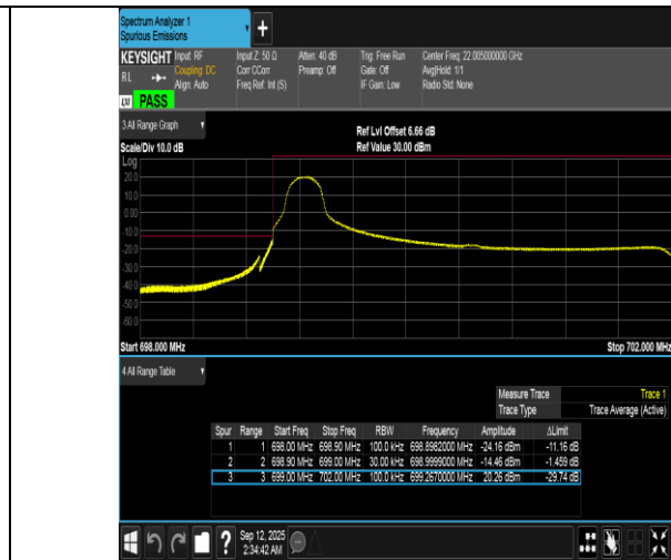
Band12-3MHz-16QAM-23025-1RB#0-PASS
