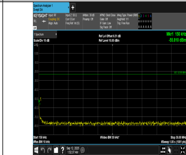
Band12-1.4MHz-QPSK-23017-6RB#0-0.15-30-PASS
