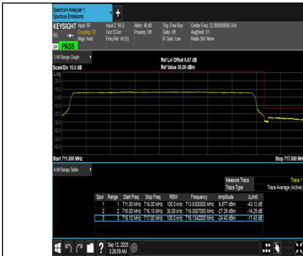
Band12-5MHz-QPSK-23155-25RB#0-PASS
