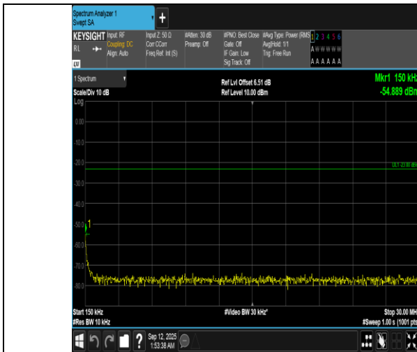
Band12-1.4MHz-16QAM-23017-6RB#0-0.15~30-PASS
