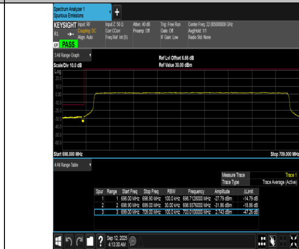
Band12-10MHz-16QAM-23060-50RB#0-PASS
