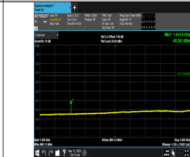
Band12-1.4MHz-QPSK-23095-6RB#0-1000-3000-PASS
