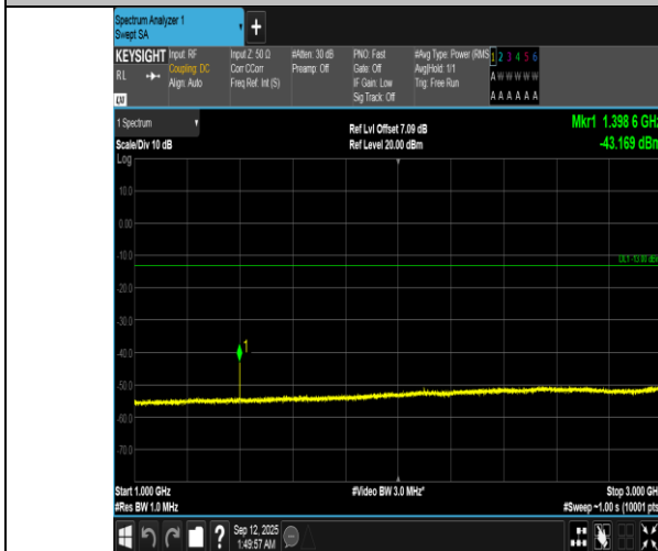
Band12-1.4MHz-16QAM-23017-1RB#0-1000~3000-PASS
