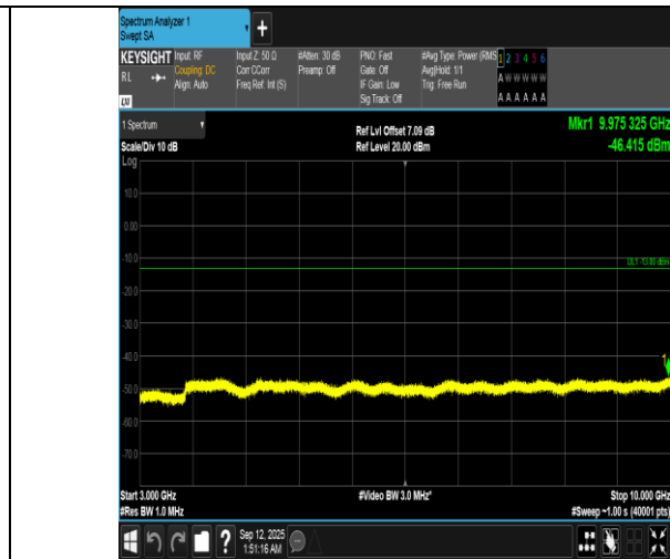
Band12-1.4MHz-QPSK-23017-1RB#5-3000-10000-PASS
