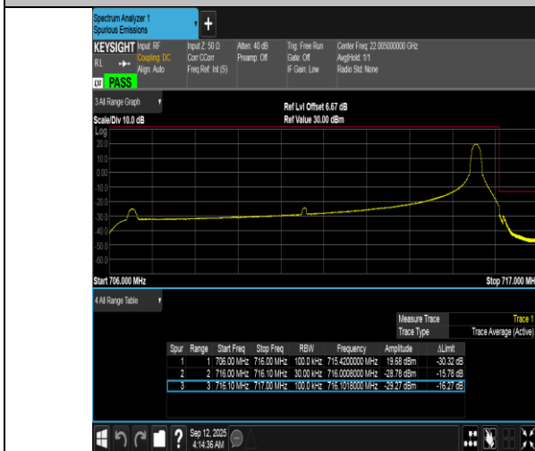
Band12-10MHz-16QAM-23130-1RB#49-PASS
