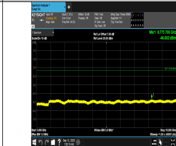
Band12-1.4MHz-16QAM-23017-1RB#0-3000~10000-PASS
