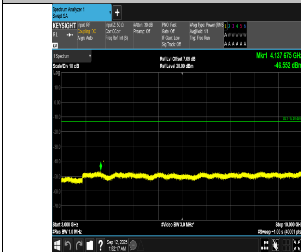
Band12-1.4MHz-16QAM-23017-1RB#5-3000~10000-PASS
