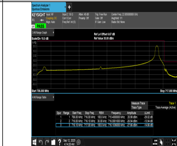
Band12-10MHz-QPSK-23130-1RB#49-PASS
