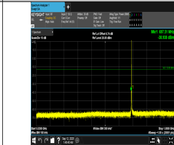
Band12-1.4MHz-16QAM-23017-1RB#0-30~1000-PASS
