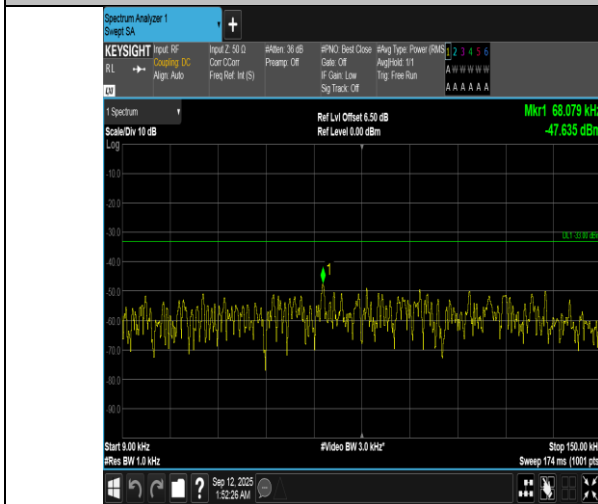
Band12-1.4MHz-QPSK-23017-6RB#0-0.009-0.15-PASS
