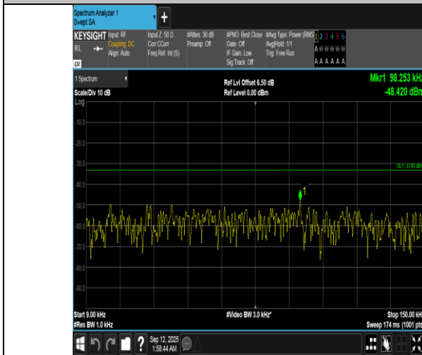
Band12-1.4MHz-QPSK-23095-6RB#0-0.009-0.15-PASS
