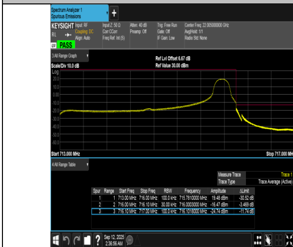
Band12-3MHz-16QAM-23165-1RB#14-PASS
