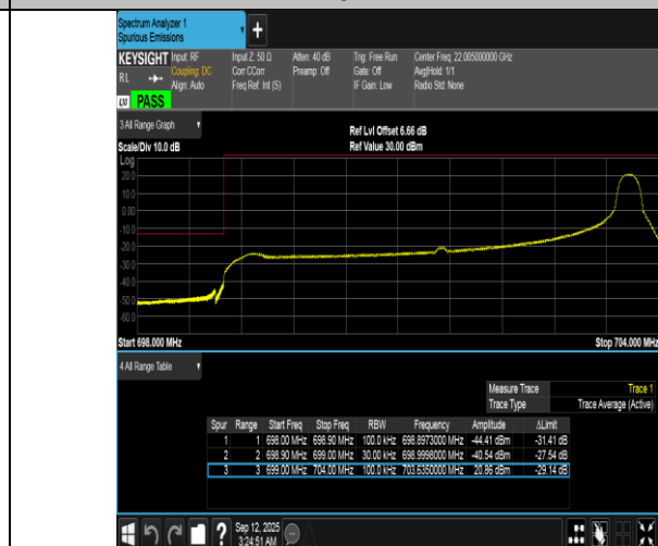
Band12-5MHz-QPSK-23035-1RB#24-PASS
