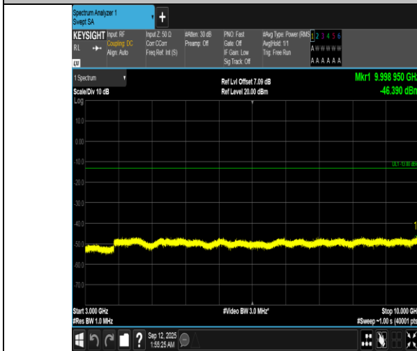
Band12-1.4MHz-QPSK-23095-1RB#0-3000~10000-PASS
