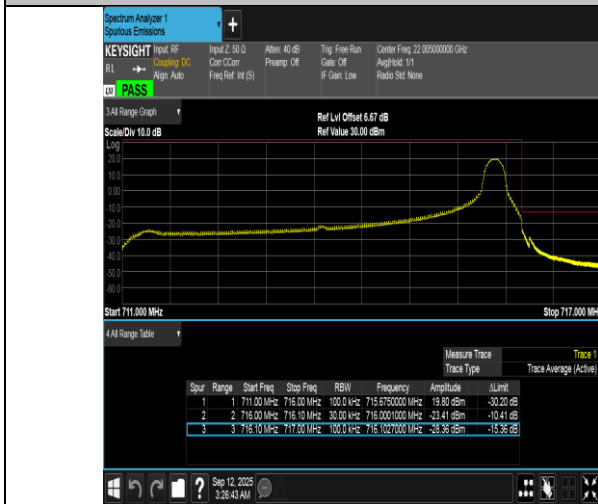
Band12-5MHz-16QAM-23155-1RB#24-PASS
