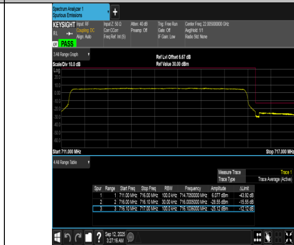
Band12-5MHz-16QAM-23155-25RB#0-PASS
