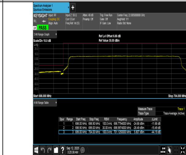
Band12-5MHz-16QAM-23035-25RB#0-PASS
