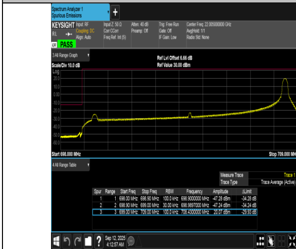
Band12-10MHz-16QAM-23060-1RB#49-PASS
