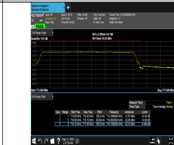
Band12-3MHz-16QAM-23165-15RB#0-PASS
