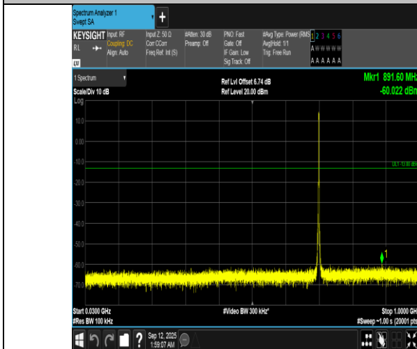
Band12-1.4MHz-QPSK-23095-6RB#0-30-1000-PASS
