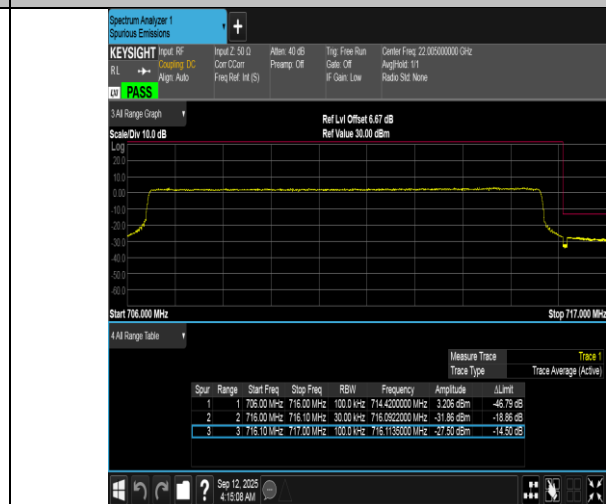
Band12-10MHz-16QAM-23130-50RB#0-PASS
