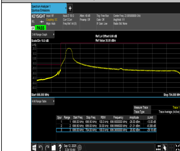
Band12-5MHz-QPSK-23035-1RB#0-PASS
