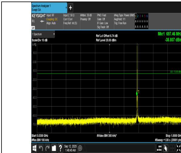
Band12-1.4MHz-QPSK-23017-1RB#0-30~1000-PASS
