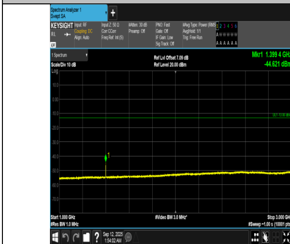
Band12-1.4MHz-16QAM-23017-6RB#0-1000~3000-PASS
