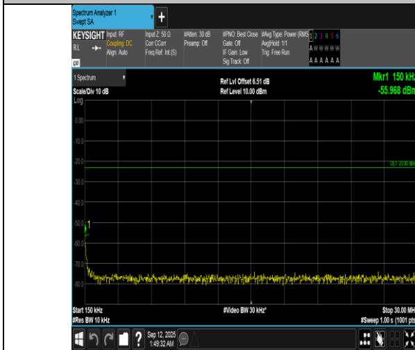
Band12-1.4MHz-16QAM-23017-1RB#0-0.15~30-PASS
