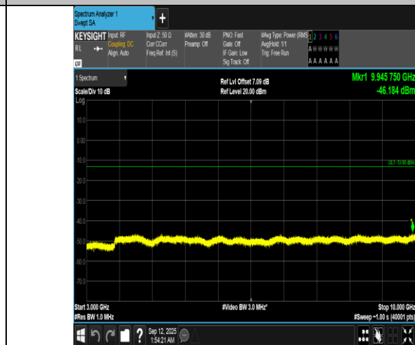
Band12-1.4MHz-16QAM-23017-6RB#0-3000~10000-PASS
