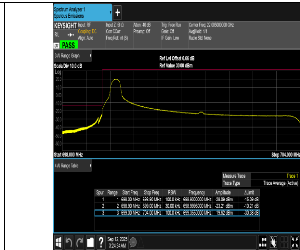
Band12-5MHz-16QAM-23035-1RB#0-PASS
