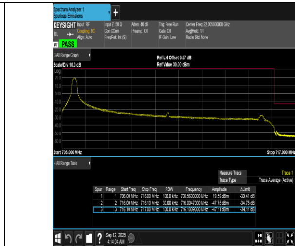
Band12-10MHz-16QAM-23130-1RB#0-PASS
