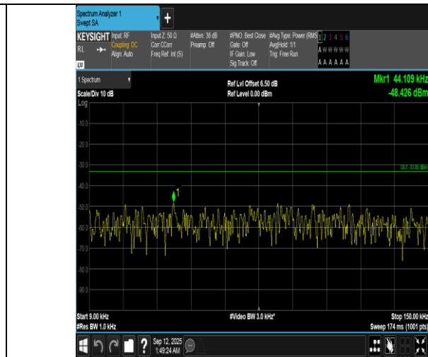
Band12-1.4MHz-16QAM-23017-1RB#0-0.009~0.15-PASS
