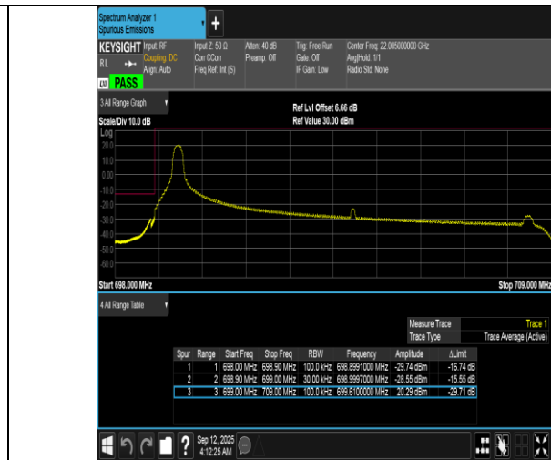
Band12-10MHz-16QAM-23060-1RB#0-PASS
