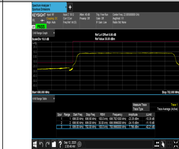
Band12-3MHz-16QAM-23025-15RB#0-PASS
