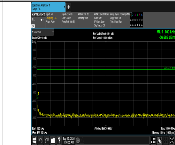
Band12-1.4MHz-QPSK-23095-6RB#0-0.15-30-PASS
