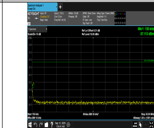
Band12-1.4MHz-QPSK-23095-1RB#0-0.15~30-PASS
