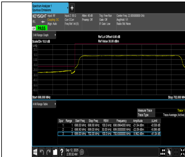
Band12-3MHz-QPSK-23025-15RB#0-PASS
