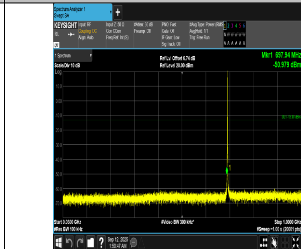
Band12-1.4MHz-QPSK-23017-1RB#5-30~1000-PASS
