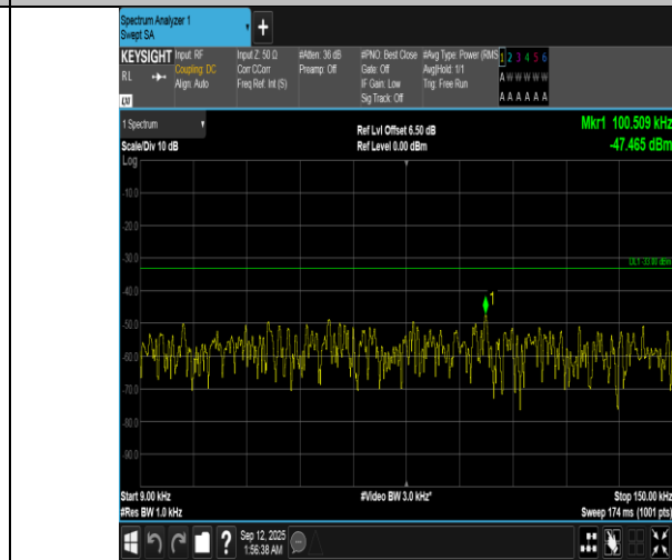
Band12-1.4MHz-QPSK-23095-1RB#5-0.009~0.15-PASS
