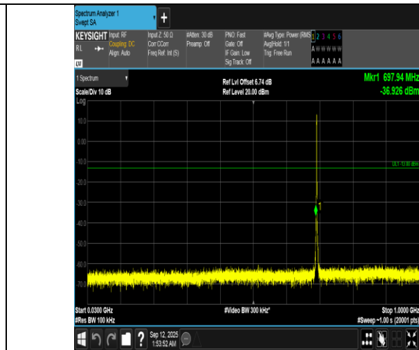
Band12-1.4MHz-16QAM-23017-6RB#0-30~1000-PASS
