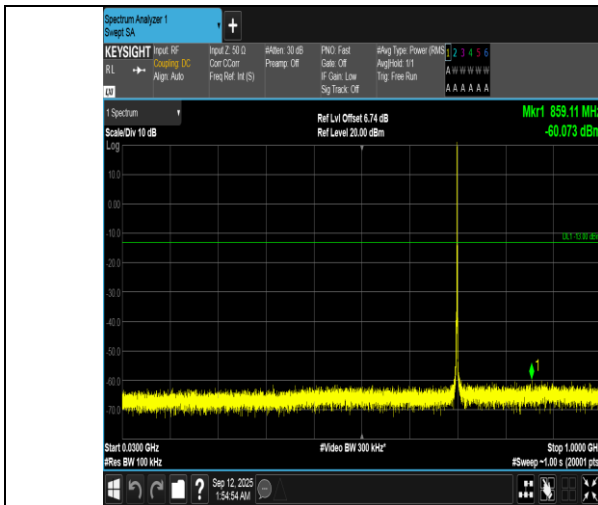
Band12-1.4MHz-QPSK-23095-1RB#0-30~1000-PASS
