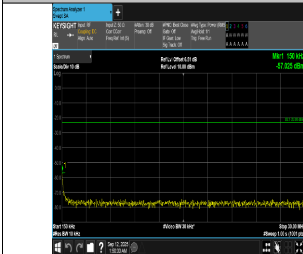
Band12-1.4MHz-QPSK-23017-1RB#5-0.15~30-PASS
