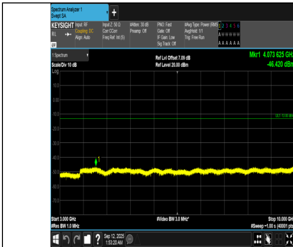
Band12-1.4MHz-QPSK-23017-6RB#0-3000~10000-PASS
