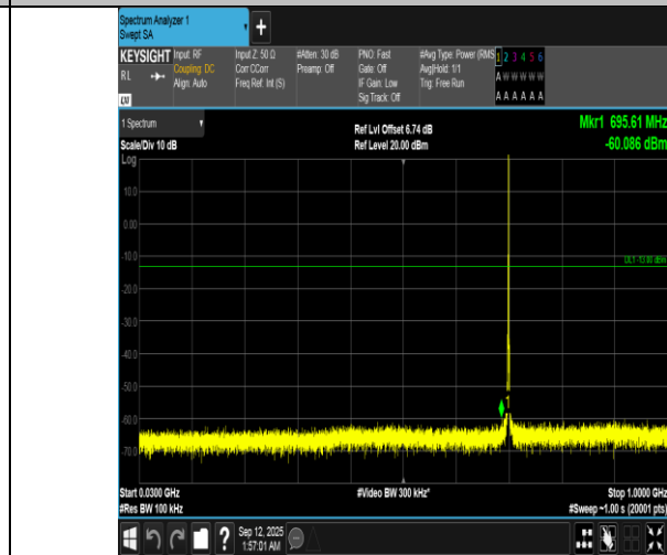
Band12-1.4MHz-QPSK-23095-1RB#5-30~1000-PASS
