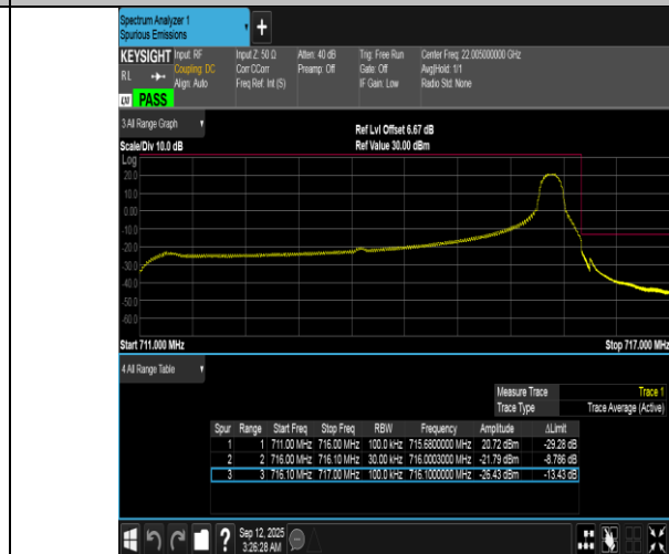
Band12-5MHz-QPSK-23155-1RB#24-PASS
