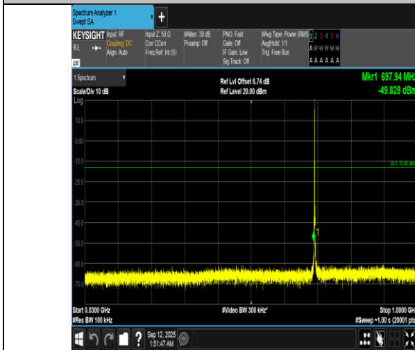
Band12-1.4MHz-16QAM-23017-1RB#5-30~1000-PASS
