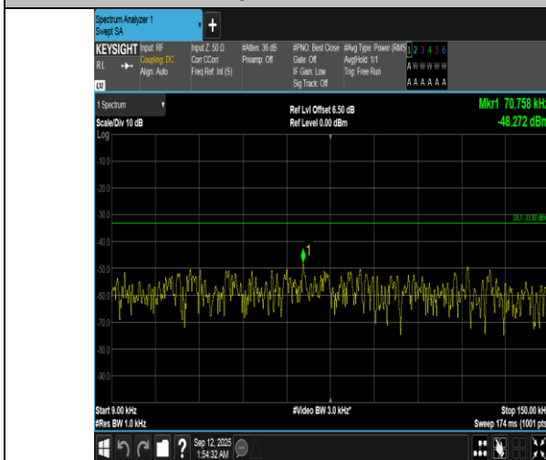
Band12-1.4MHz-QPSK-23095-1RB#0-0.009~0.15-PASS
