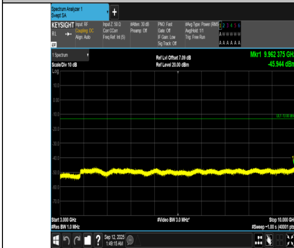
Band12-1.4MHz-QPSK-23017-1RB#0-3000~10000-PASS
