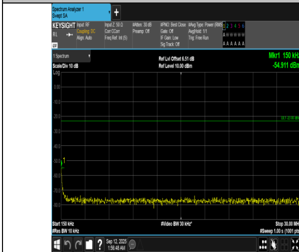
Band12-1.4MHz-QPSK-23095-1RB#5-0.15~30-PASS
