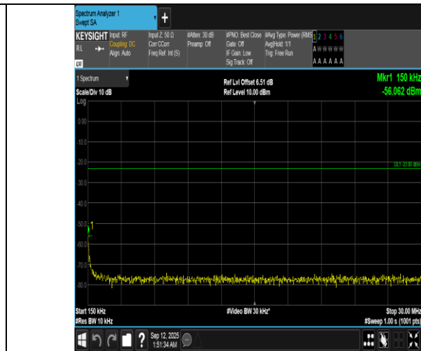
Band12-1.4MHz-16QAM-23017-1RB#5-0.15~30-PASS
