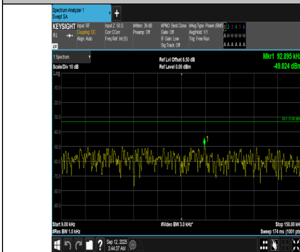
Band12-5MHz-QPSK-23155-25RB#0-0.009~0.15-PASS
