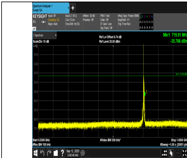
Band12-5MHz-QPSK-23155-1RB#0-30~1000-PASS
