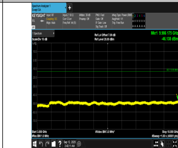
Band12-5MHz-16QAM-23095-25RB#0-3000~10000-PASS
