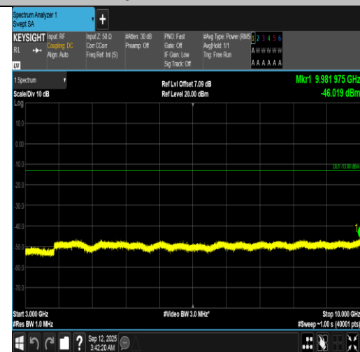
Band12-5MHz-16QAM-23155-1RB#0-3000~10000-PASS
