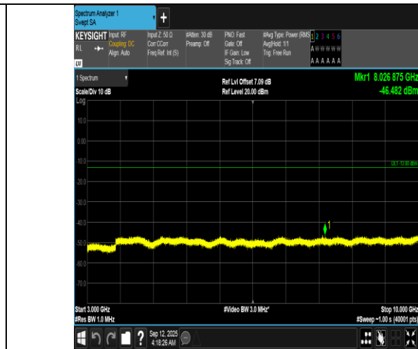
Band12-10MHz-QPSK-23060-1RB#49-3000~10000-PASS
