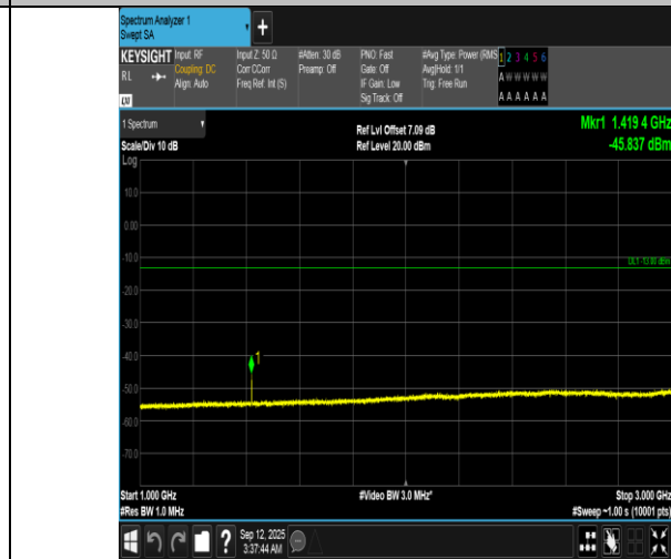
Band12-5MHz-16QAM-23095-1RB#24-1000~3000-PASS
