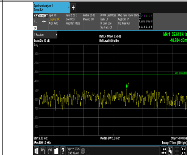
Band12-5MHz-16QAM-23155-25RB#0-0.009~0.15-PASS
