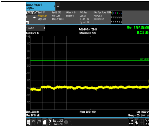
Band12-10MHz-QPSK-23060-50RB#0-3000~10000-PASS
