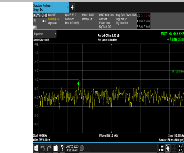
Band12-10MHz-QPSK-23095-1RB#49-0.009~0.15-PASS
