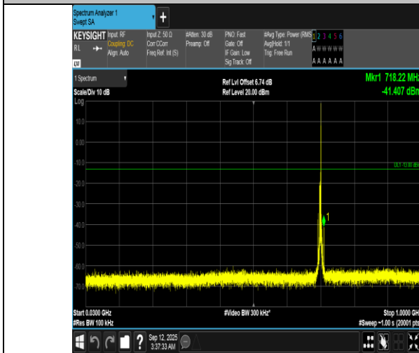
Band12-5MHz-16QAM-23095-1RB#24-30~1000-PASS
