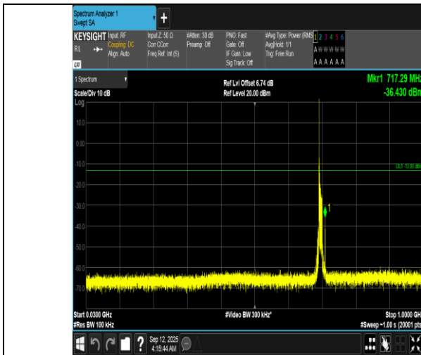
Band12-10MHz-QPSK-23060-1RB#0-30~1000-PASS
