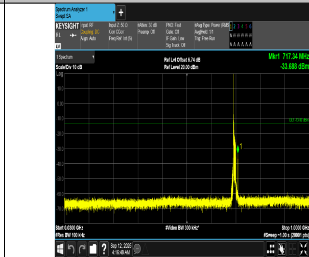
Band12-10MHz-16QAM-23060-1RB#0-30~1000-PASS
