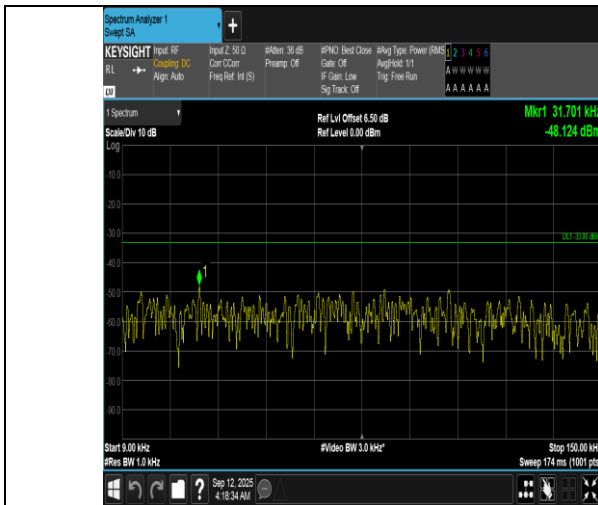
Band12-10MHz-16QAM-23060-1RB#49-0.009~0.15-PASS
