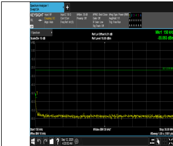
Band12-10MHz-16QAM-23060-50RB#0-0.15~30-PASS
