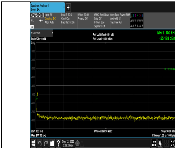
Band12-5MHz-16QAM-23095-25RB#0-0.15~30-PASS
