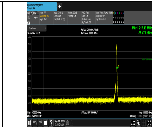
Band12-5MHz-16QAM-23155-25RB#0-30~1000-PASS
