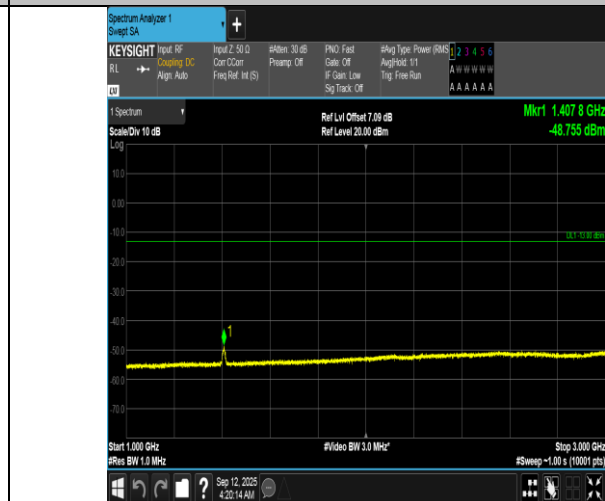
Band12-10MHz-QPSK-23060-50RB#0-1000~3000-PASS
