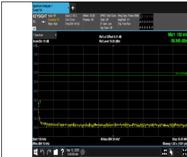
Band12-5MHz-16QAM-23155-25RB#0-0.15~30-PASS
