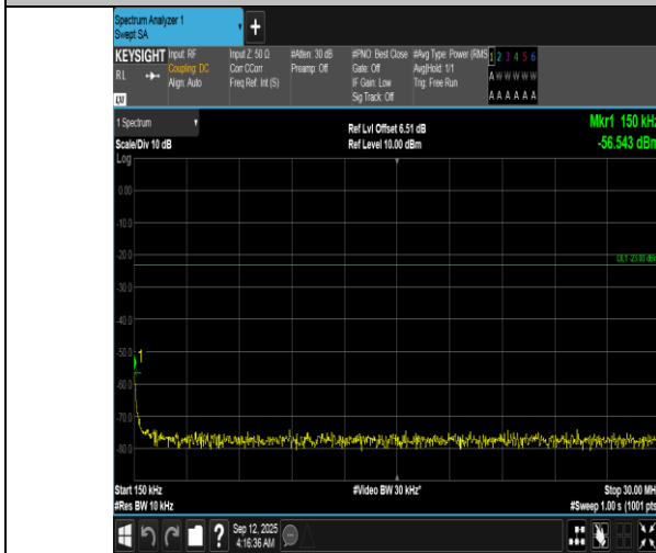
Band12-10MHz-16QAM-23060-1RB#0-0.15~30-PASS
