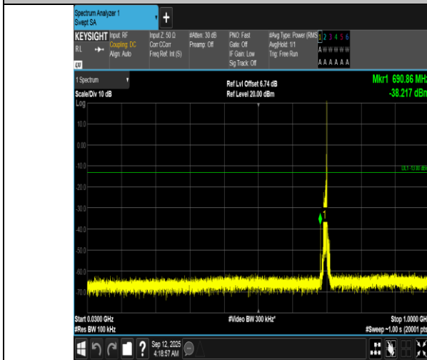
Band12-10MHz-16QAM-23060-1RB#49-30~1000-PASS
