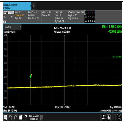
Band12-10MHz-QPSK-23060-1RB#0-1000~3000-PASS
