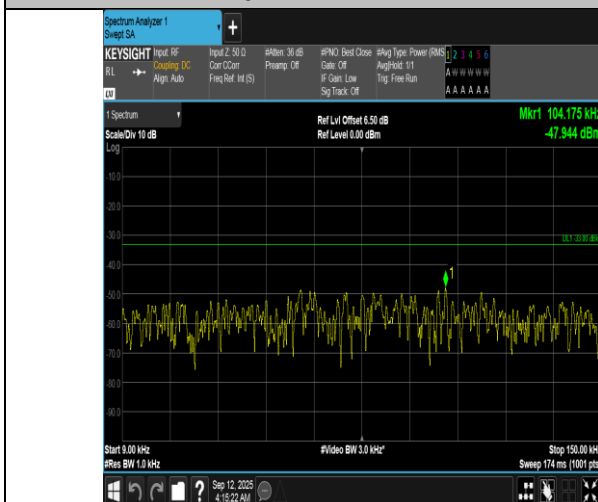
Band12-10MHz-QPSK-23060-1RB#0-0.009~0.15-PASS
