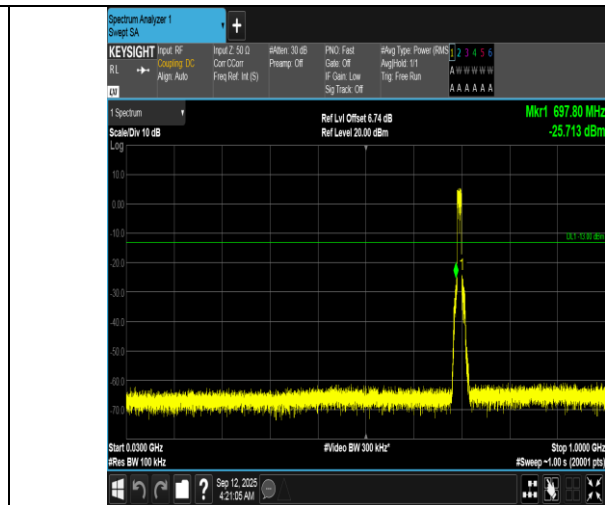
Band12-10MHz-16QAM-23060-50RB#0-30~1000-PASS
