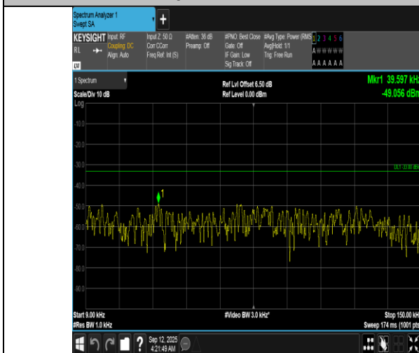
Band12-10MHz-QPSK-23095-1RB#0-0.009~0.15-PASS
