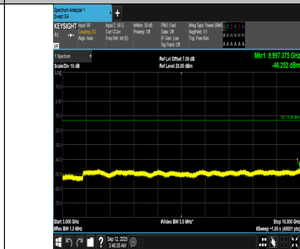
Band12-5MHz-16QAM-23155-25RB#0-3000~10000-PASS
