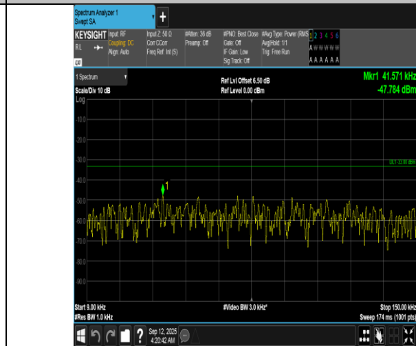
Band12-10MHz-16QAM-23060-50RB#0-0.009~0.15-PASS
