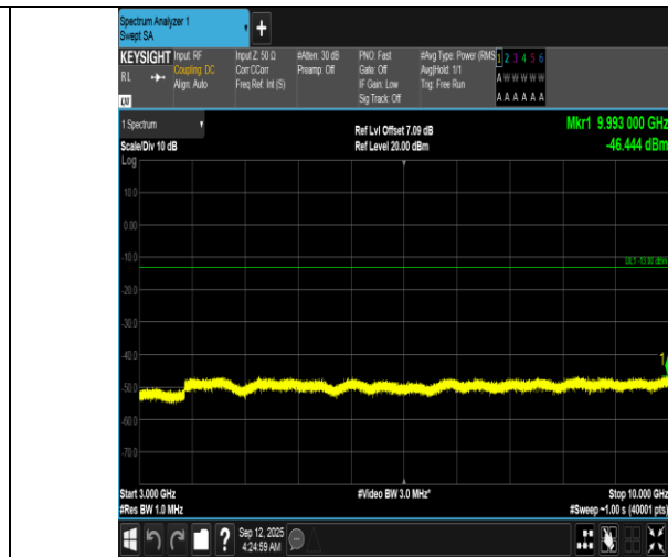
Band12-10MHz-QPSK-23095-1RB#49-3000~10000-PASS
