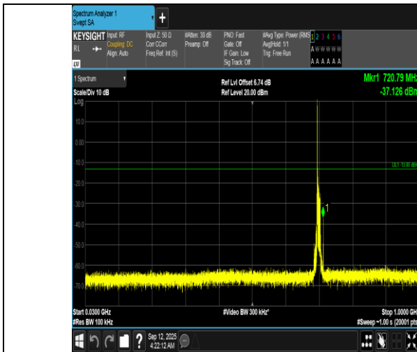
Band12-10MHz-QPSK-23095-1RB#0-30~1000-PASS
