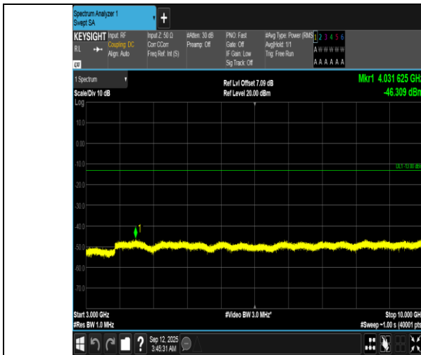
Band12-5MHz-QPSK-23155-25RB#0-3000~10000-PASS
