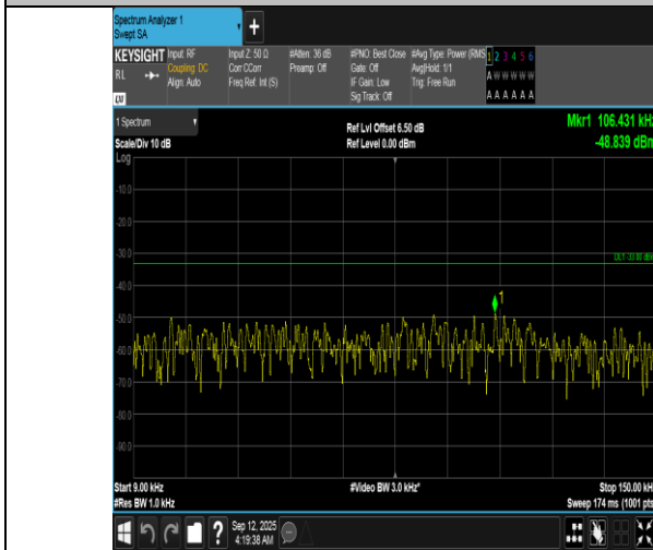
Band12-10MHz-QPSK-23060-50RB#0-0.009~0.15-PASS
