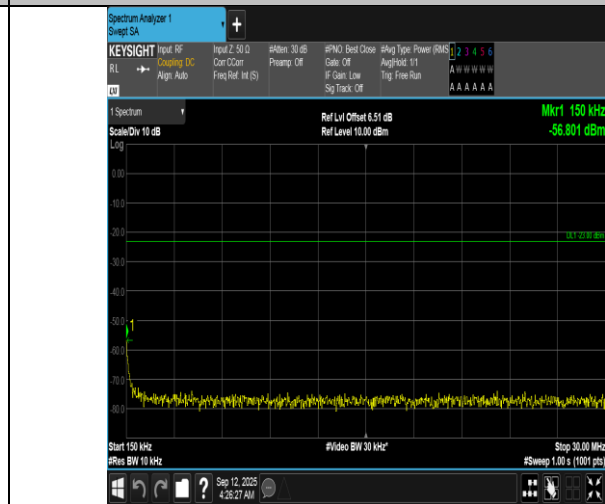
Band12-10MHz-QPSK-23095-50RB#0-0.15~30-PASS
