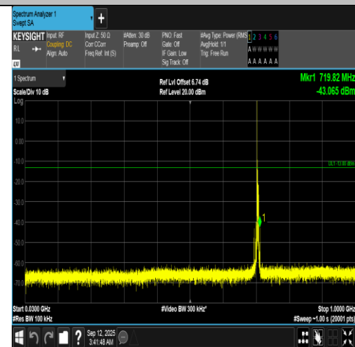
Band12-5MHz-16QAM-23155-1RB#0-30~1000-PASS
