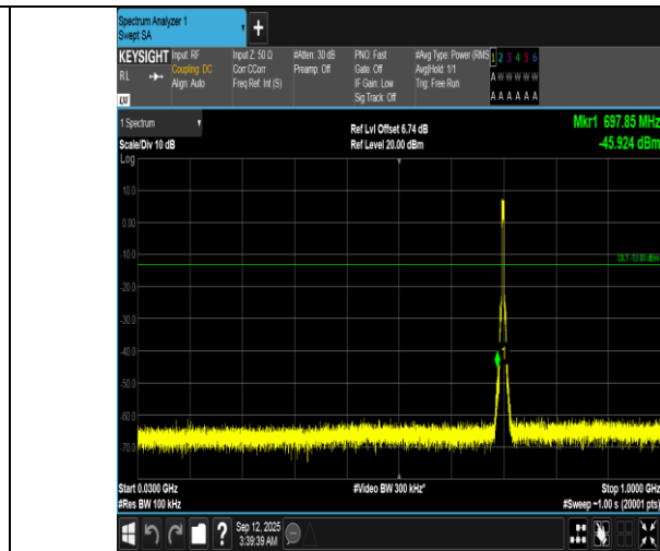
Band12-5MHz-16QAM-23095-25RB#0-30~1000-PASS
