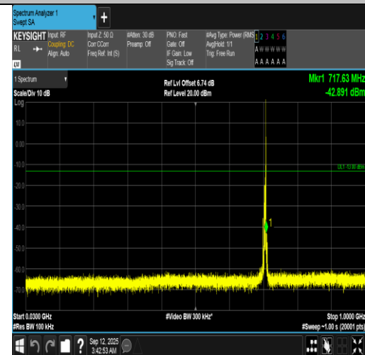
Band12-5MHz-QPSK-23155-1RB#24-30~1000-PASS
