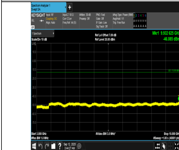
Band12-5MHz-16QAM-23155-1RB#24-3000~10000-PASS
