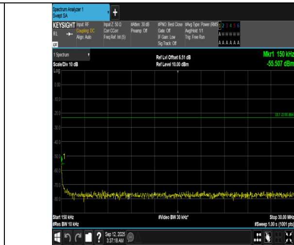
Band12-5MHz-16QAM-23095-1RB#24-0.15~30-PASS
