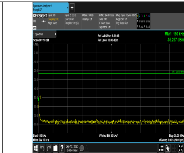
Band12-5MHz-16QAM-23155-1RB#24-0.15~30-PASS
