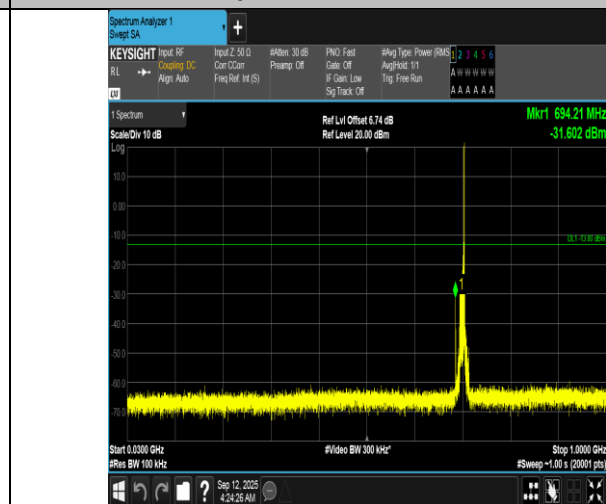
Band12-10MHz-QPSK-23095-1RB#49-30~1000-PASS
