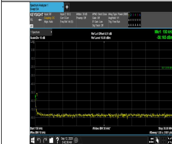
Band12-5MHz-QPSK-23155-1RB#24-0.15~30-PASS
