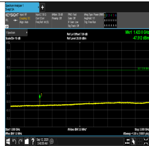
Band12-5MHz-QPSK-23155-1RB#0-1000~3000-PASS
