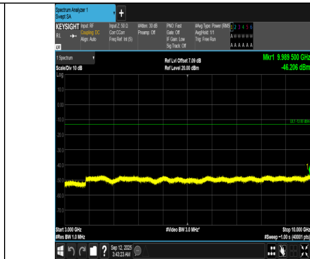
Band12-5MHz-QPSK-23155-1RB#24-3000~10000-PASS
