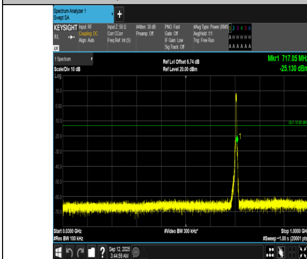
Band12-5MHz-QPSK-23155-25RB#0-30~1000-PASS
