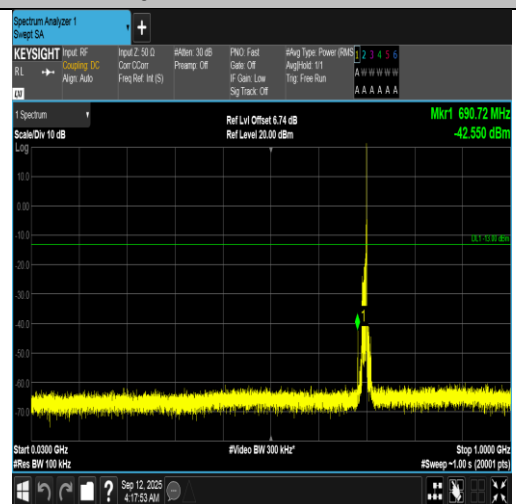
Band12-10MHz-QPSK-23060-1RB#49-30~1000-PASS
