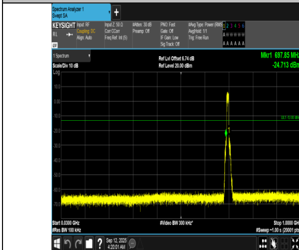
Band12-10MHz-QPSK-23060-50RB#0-30~1000-PASS
