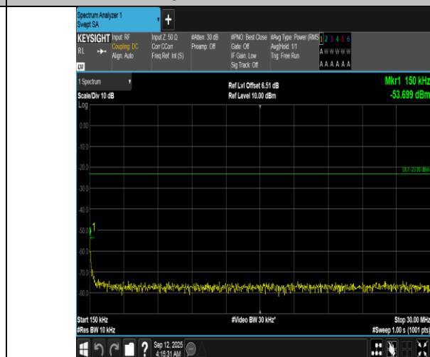
Band12-10MHz-QPSK-23060-1RB#0-0.15~30-PASS
