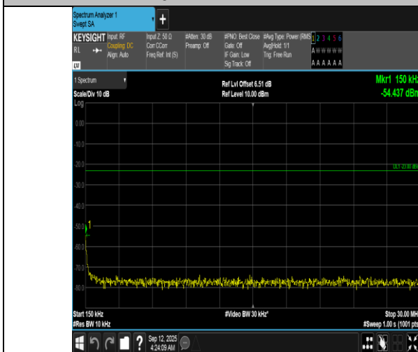
Band12-10MHz-QPSK-23095-1RB#49-0.15~30-PASS
