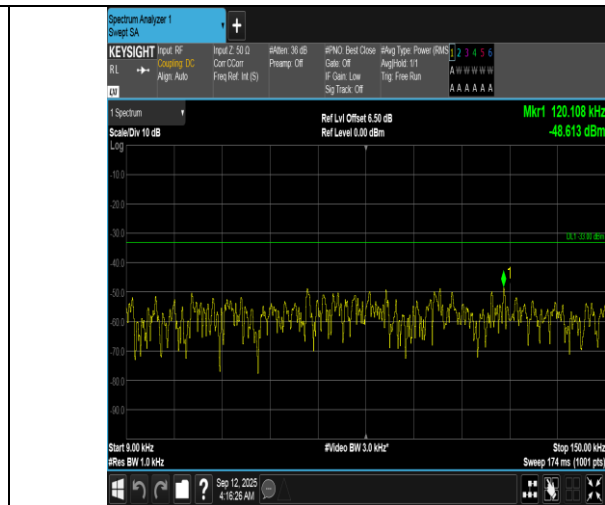
Band12-10MHz-16QAM-23060-1RB#0-0.009~0.15-PASS
