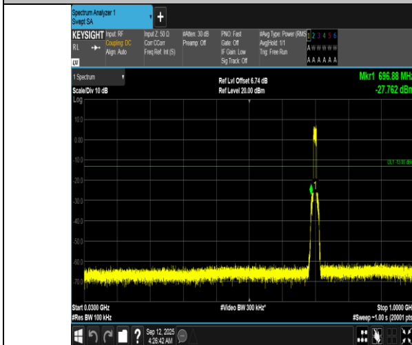
Band12-10MHz-QPSK-23095-50RB#0-30~1000-PASS
