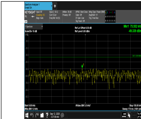
Band12-5MHz-16QAM-23095-1RB#24-0.009~0.15-PASS
