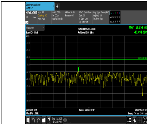
Band12-5MHz-16QAM-23155-1RB#24-0.009~0.15-PASS
