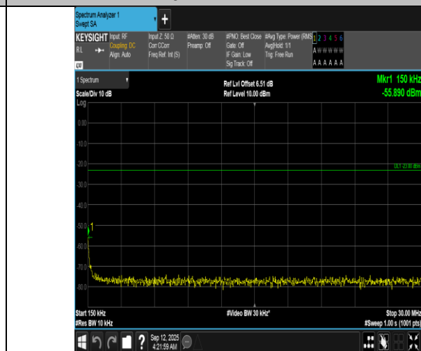
Band12-10MHz-QPSK-23095-1RB#0-0.15~30-PASS
