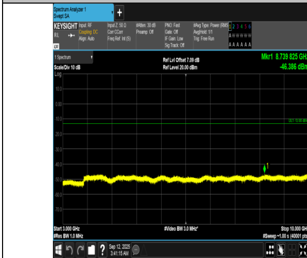
Band12-5MHz-QPSK-23155-1RB#0-3000~10000-PASS
