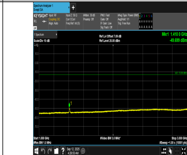
Band12-10MHz-QPSK-23095-50RB#0-1000~3000-PASS
