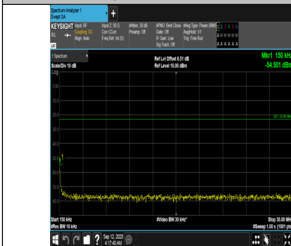
Band12-10MHz-QPSK-23060-1RB#49-0.15~30-PASS
