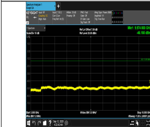
Band12-10MHz-QPSK-23095-1RB#0-3000~10000-PASS
