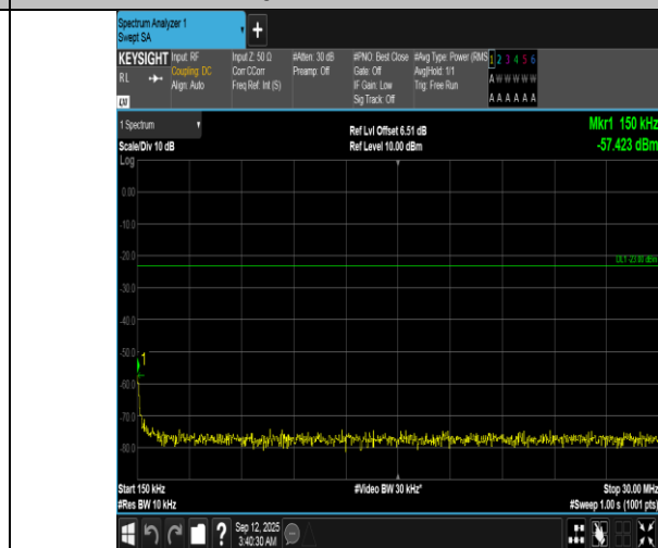
Band12-5MHz-QPSK-23155-1RB#0-0.15~30-PASS
