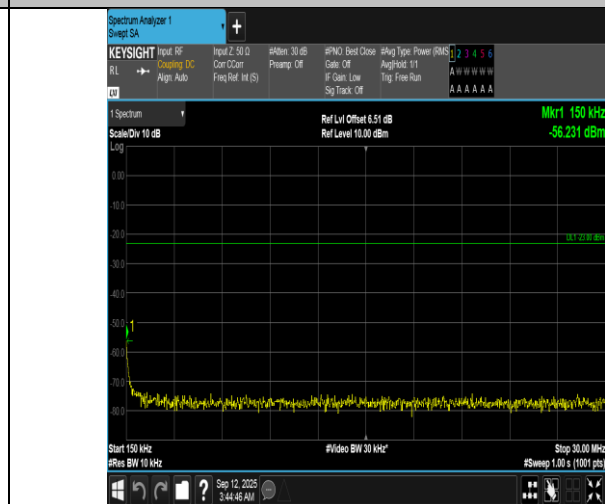
Band12-5MHz-QPSK-23155-25RB#0-0.15~30-PASS
