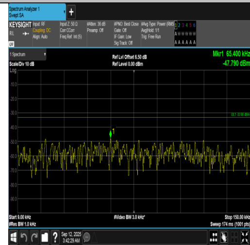
Band12-5MHz-QPSK-23155-1RB#24-0.009~0.15-PASS
