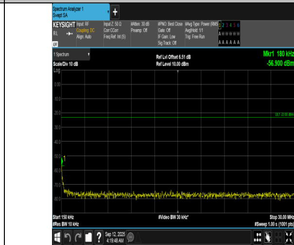
Band12-10MHz-QPSK-23060-50RB#0-0.15~30-PASS
