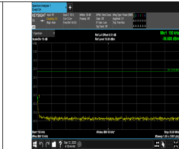
Band12-10MHz-16QAM-23060-1RB#49-0.15~30-PASS
