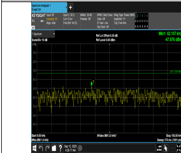
Band12-10MHz-QPSK-23095-50RB#0-0.009~0.15-PASS
