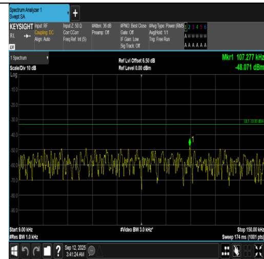
Band12-5MHz-16QAM-23155-1RB#0-0.009~0.15-PASS
