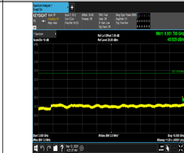
Band12-10MHz-16QAM-23060-50RB#0-3000~10000-PASS
