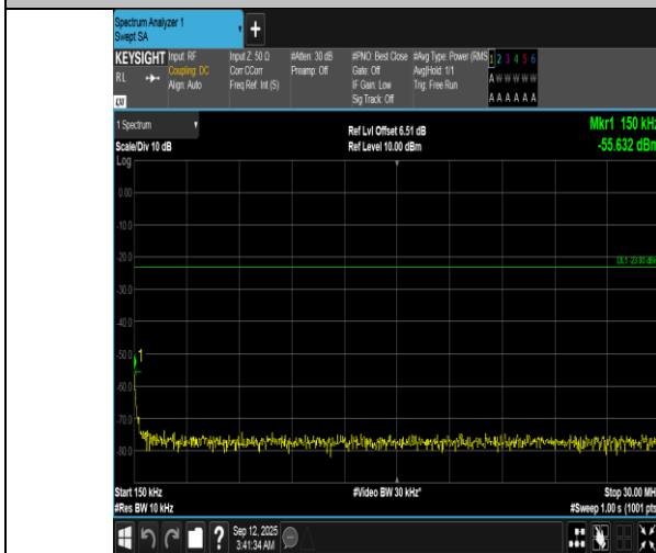
Band12-5MHz-16QAM-23155-1RB#0-0.15~30-PASS
