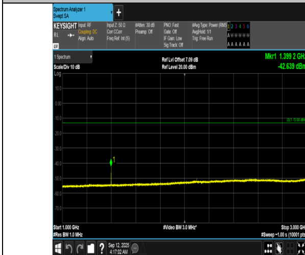
Band12-10MHz-16QAM-23060-1RB#0-1000~3000-PASS
