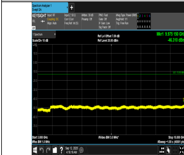
Band12-10MHz-QPSK-23060-1RB#0-3000~10000-PASS
