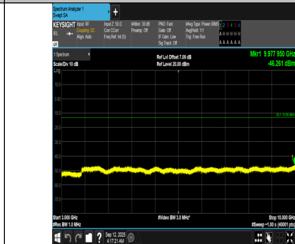
Band12-10MHz-16QAM-23060-1RB#0-3000~10000-PASS
