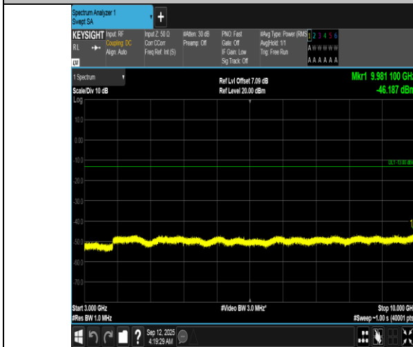
Band12-10MHz-16QAM-23060-1RB#49-3000~10000-PASS
