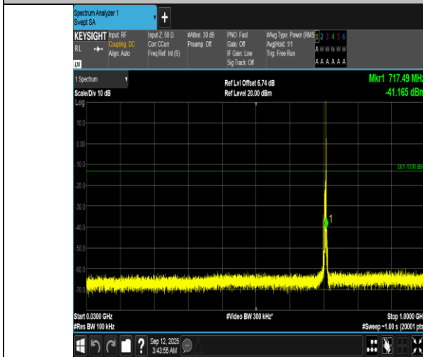
Band12-5MHz-16QAM-23155-1RB#24-30~1000-PASS
