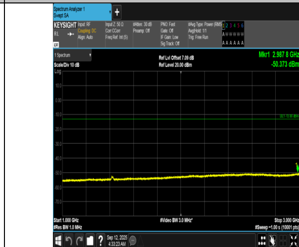
Band12-10MHz-QPSK-23130-50RB#0-1000~3000-PASS
