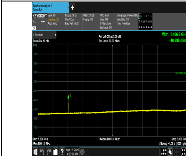
Band12-10MHz-16QAM-23095-1RB#0-1000~3000-PASS
