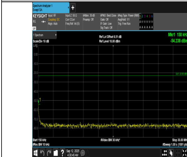
Band12-10MHz-QPSK-23130-1RB#49-0.15~30-PASS
