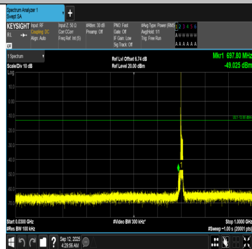
Band12-10MHz-16QAM-23130-1RB#0-30~1000-PASS
