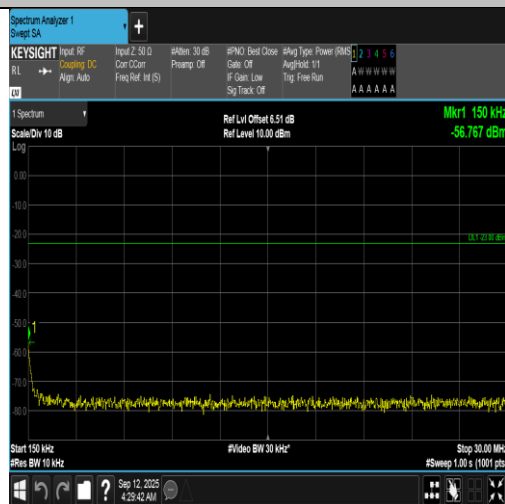
Band12-10MHz-16QAM-23130-1RB#0-0.15~30-PASS
