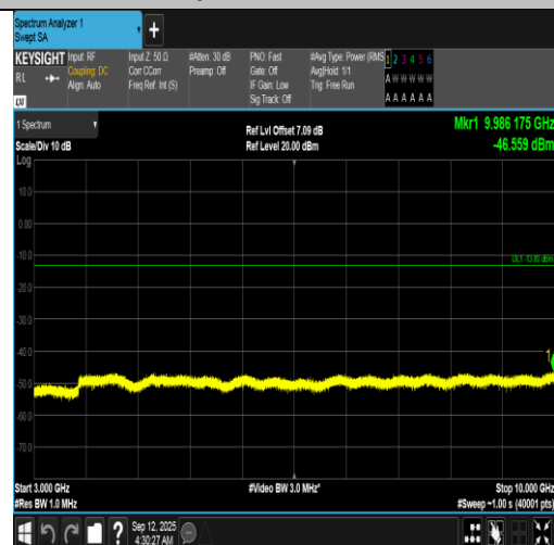
Band12-10MHz-16QAM-23130-1RB#0-3000~10000-PASS
