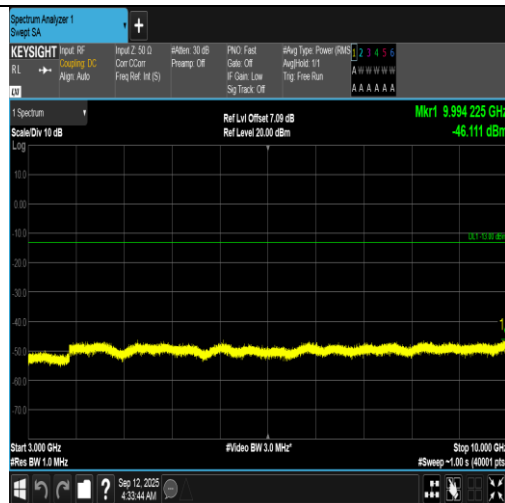
Band12-10MHz-QPSK-23130-50RB#0-3000~10000-PASS
