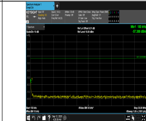
Band12-10MHz-QPSK-23130-1RB#0-0.15~30-PASS
