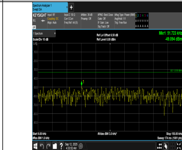
Band12-10MHz-16QAM-23130-50RB#0-0.009~0.15-PASS
