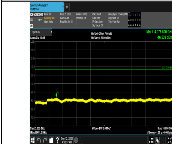
Band12-10MHz-16QAM-23130-1RB#49-3000~10000-PASS
