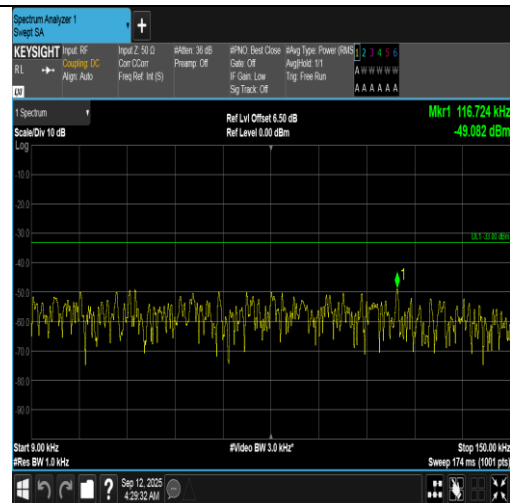
Band12-10MHz-16QAM-23130-1RB#0-0.009~0.15-PASS
