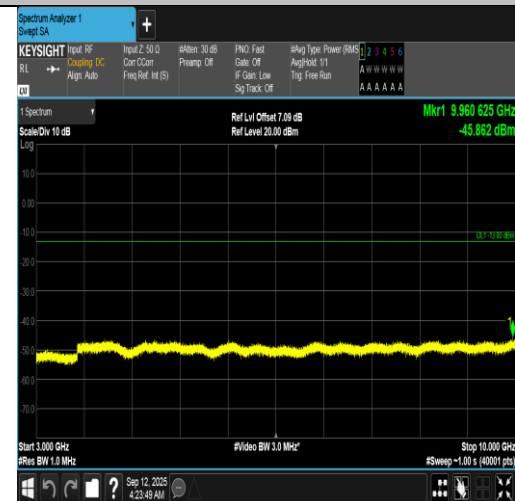
Band12-10MHz-16QAM-23095-1RB#0-3000~10000-PASS
