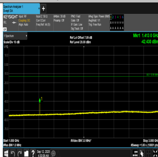
Band12-10MHz-16QAM-23130-1RB#0-1000~3000-PASS
