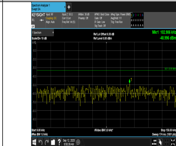
Band17-10MHz-QPSK-23800-1RB#49-0.009~0.15-PASS
