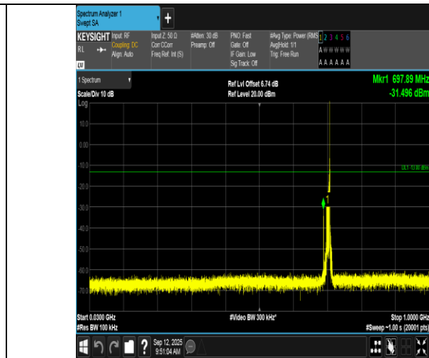
Band17-10MHz-QPSK-23800-1RB#49-30~1000-PASS
