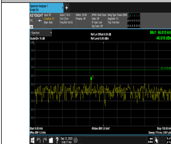
Band17-10MHz-QPSK-23790-50RB#0-0.009~0.15-PASS
