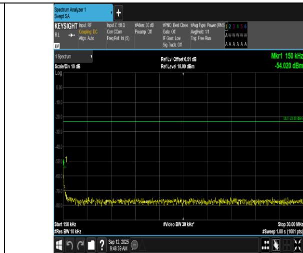
Band17-10MHz-QPSK-23800-1RB#0-0.15~30-PASS
