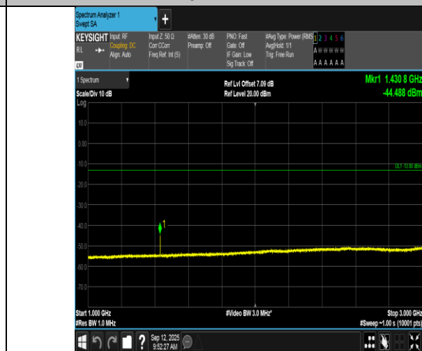
Band17-10MHz-16QAM-23800-1RB#49-1000~3000-PASS
