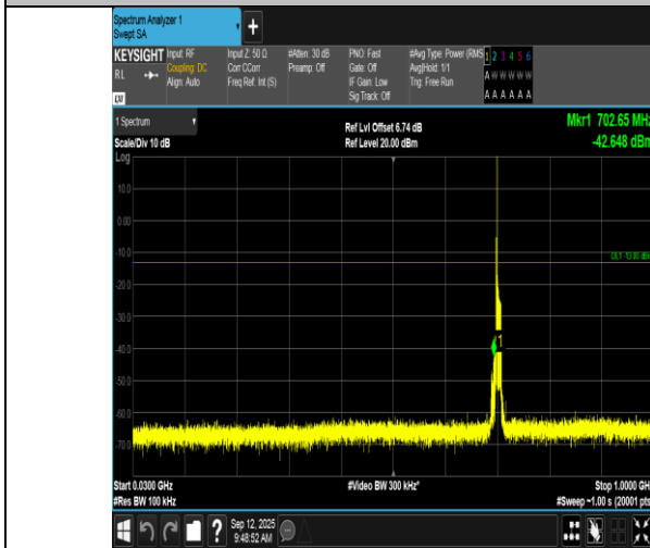
Band17-10MHz-QPSK-23800-1RB#0-30~1000-PASS
