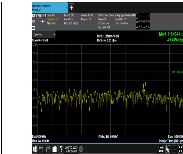
Band17-10MHz-QPSK-23800-1RB#0-0.009~0.15-PASS
