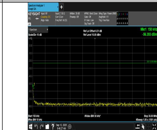
Band17-10MHz-QPSK-23790-50RB#0-0.15~30-PASS
