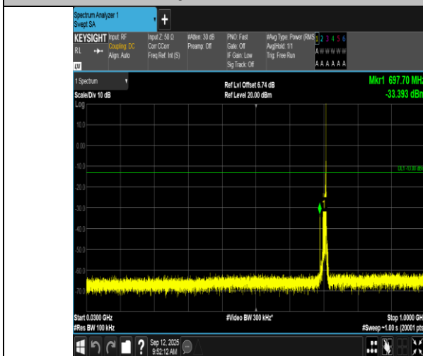
Band17-10MHz-16QAM-23800-1RB#49-30~1000-PASS
