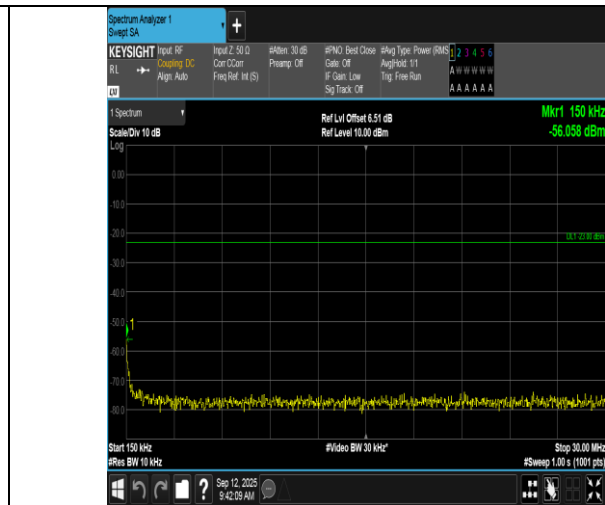
Band17-10MHz-QPSK-23790-1RB#0-0.15~30-PASS
