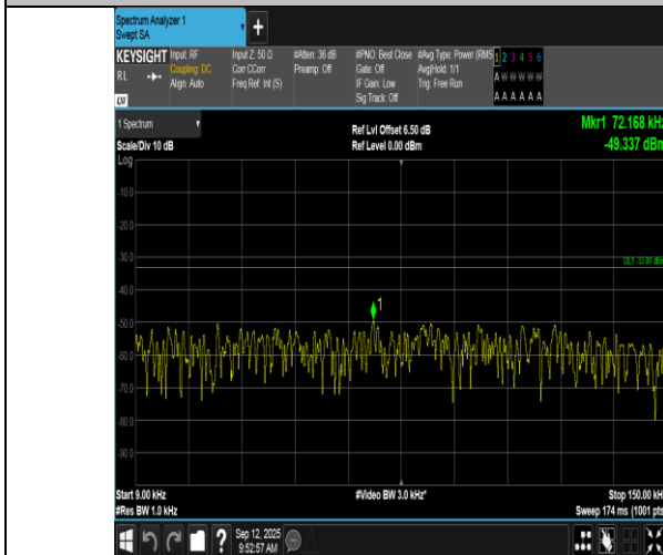
Band17-10MHz-QPSK-23800-50RB#0-0.009~0.15-PASS
