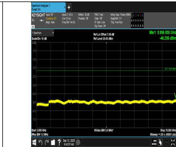
Band17-10MHz-16QAM-23790-1RB#0-3000~10000-PASS
