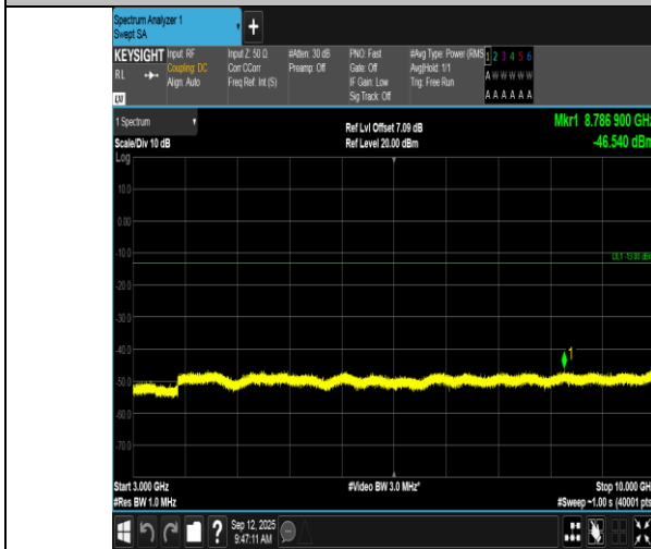
Band17-10MHz-QPSK-23790-50RB#0-3000~10000-PASS
