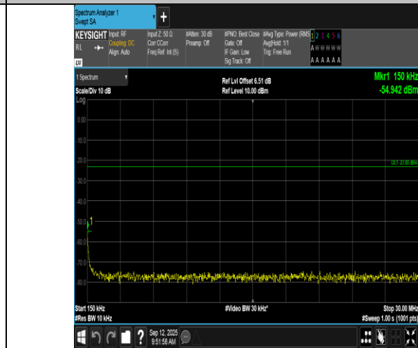
Band17-10MHz-16QAM-23800-1RB#49-0.15~30-PASS
