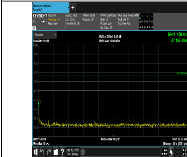
Band17-10MHz-16QAM-23780-50RB#0-0.15~30-PASS
