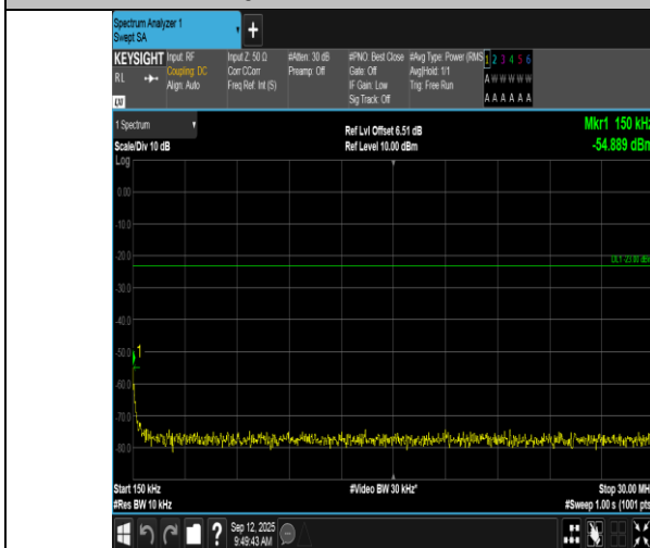
Band17-10MHz-16QAM-23800-1RB#0-0.15~30-PASS
