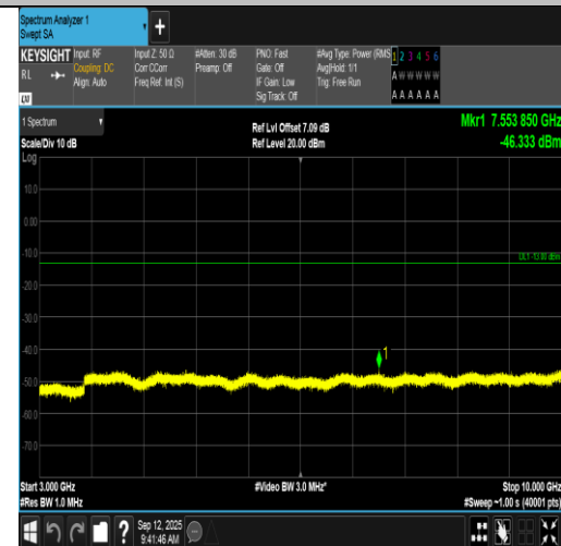
Band17-10MHz-16QAM-23780-50RB#0-3000~10000-PASS
