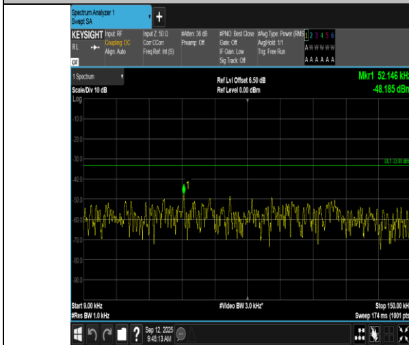
Band17-10MHz-16QAM-23790-1RB#49-0.009~0.15-PASS
