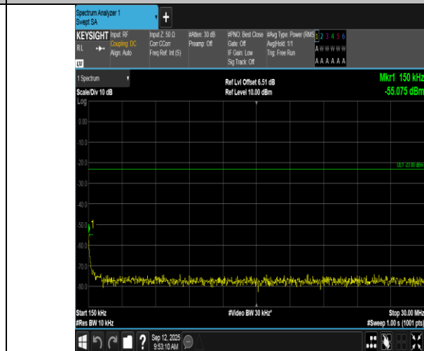
Band17-10MHz-QPSK-23800-50RB#0-0.15~30-PASS
