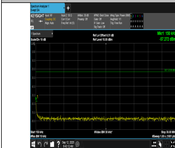
Band17-10MHz-16QAM-23790-1RB#0-0.15~30-PASS
