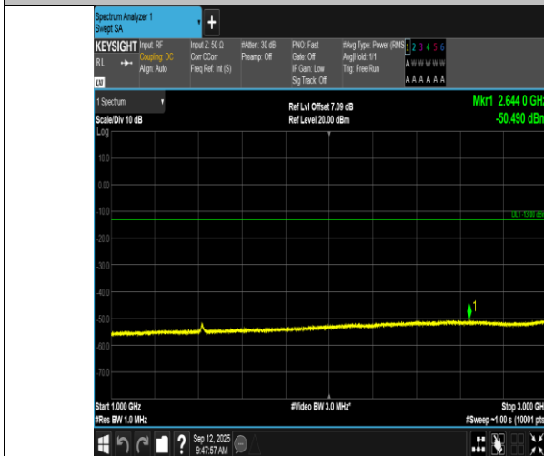
Band17-10MHz-16QAM-23790-50RB#0-1000~3000-PASS
