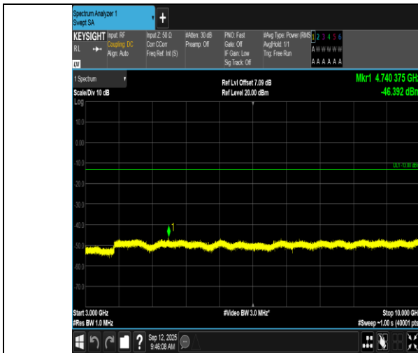
Band17-10MHz-16QAM-23790-1RB#49-3000~10000-PASS
