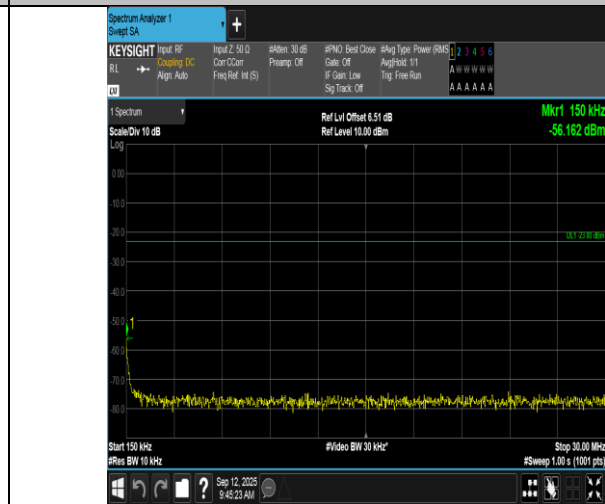
Band17-10MHz-16QAM-23790-1RB#49-0.15~30-PASS
