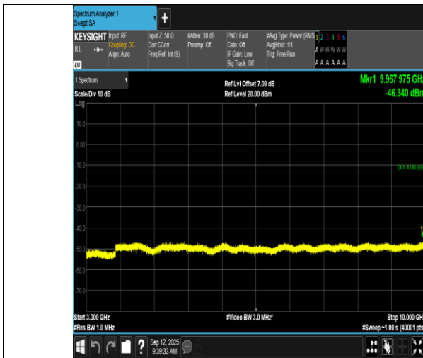
Band17-10MHz-16QAM-23780-1RB#49-3000~10000-PASS
