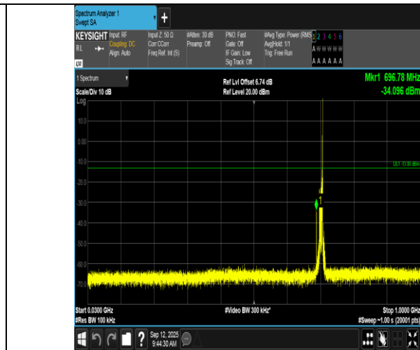
Band17-10MHz-QPSK-23790-1RB#49-30~1000-PASS
