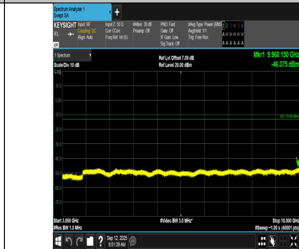
Band17-10MHz-QPSK-23800-1RB#49-3000~10000-PASS
