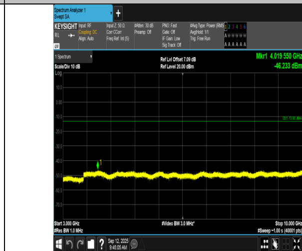
Band17-10MHz-QPSK-23790-1RB#49-3000~10000-PASS
