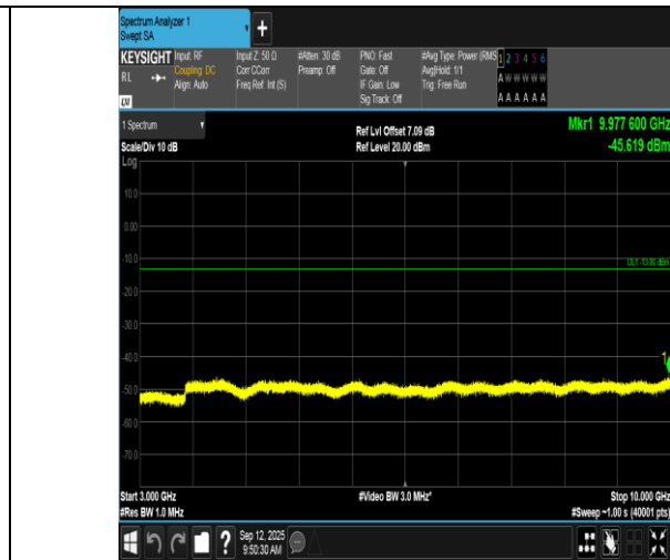
Band17-10MHz-16QAM-23800-1RB#0-3000~10000-PASS
