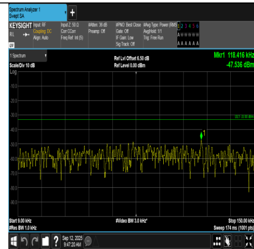
Band17-10MHz-16QAM-23790-50RB#0-0.009~0.15-PASS
