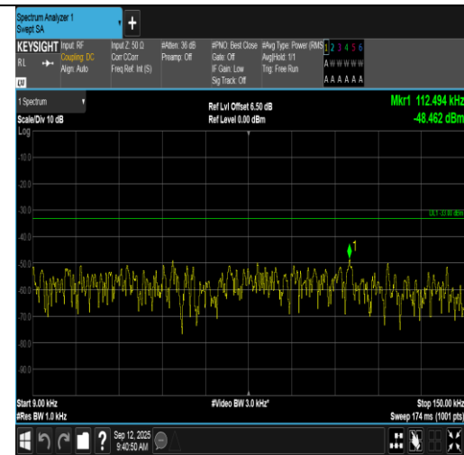
Band17-10MHz-16QAM-23780-50RB#0-0.009~0.15-PASS
