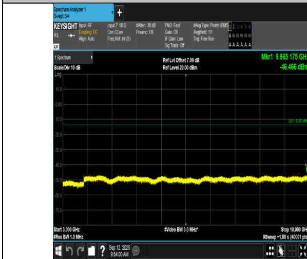
Band17-10MHz-QPSK-23800-50RB#0-3000~10000-PASS
