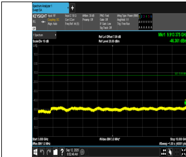
Band17-10MHz-16QAM-23800-1RB#49-3000~10000-PASS
