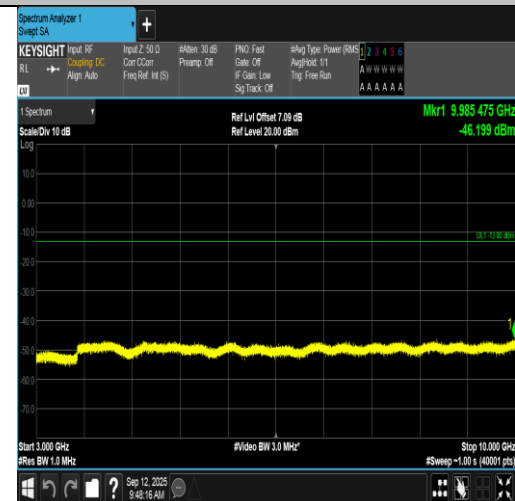
Band17-10MHz-16QAM-23790-50RB#0-3000~10000-PASS
