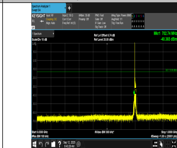
Band17-10MHz-16QAM-23790-1RB#0-30~1000-PASS
