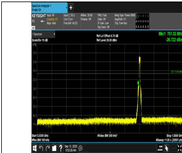
Band17-10MHz-QPSK-23800-50RB#0-30~1000-PASS
