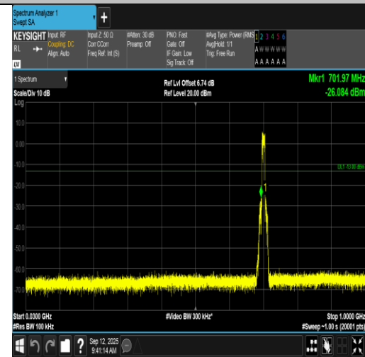
Band17-10MHz-16QAM-23780-50RB#0-30~1000-PASS
