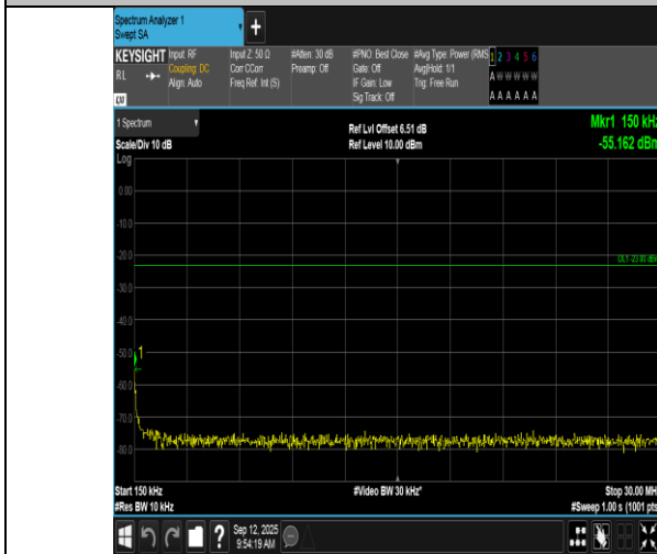
Band17-10MHz-16QAM-23800-50RB#0-0.15~30-PASS
