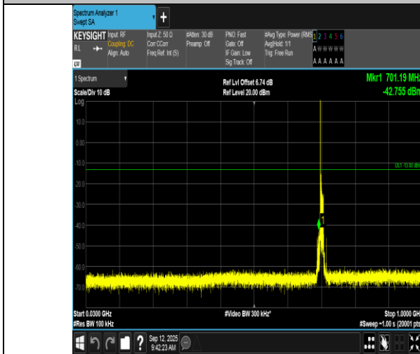
Band17-10MHz-QPSK-23790-1RB#0-30~1000-PASS
