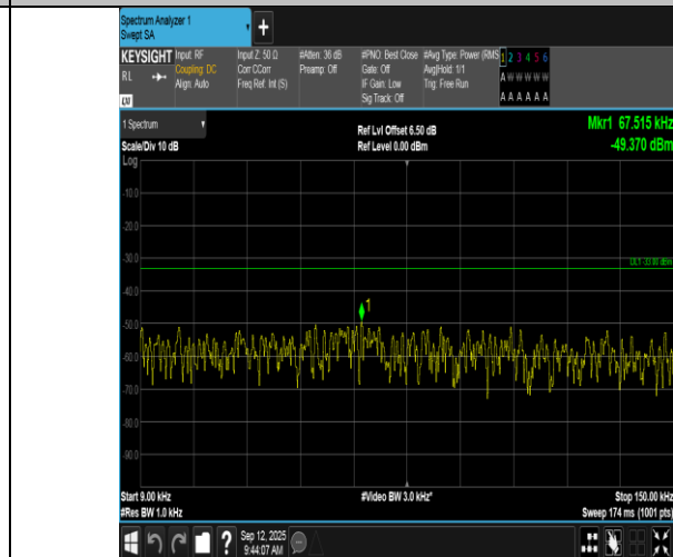
Band17-10MHz-QPSK-23790-1RB#49-0.009~0.15-PASS
