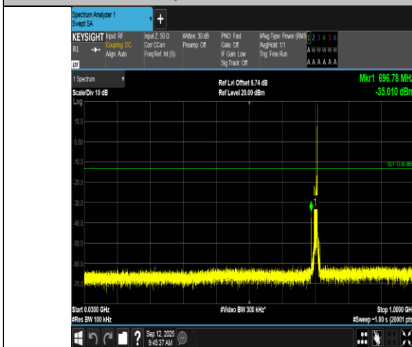
Band17-10MHz-16QAM-23790-1RB#49-30~1000-PASS
