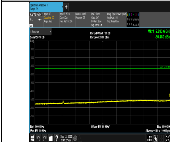
Band17-10MHz-16QAM-23780-50RB#0-1000~3000-PASS
