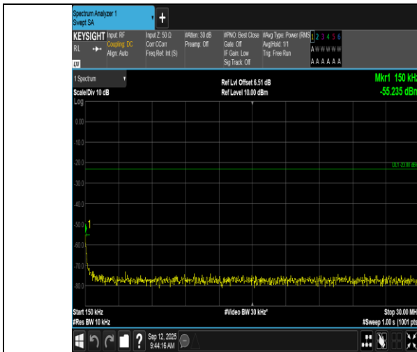
Band17-10MHz-QPSK-23790-1RB#49-0.15~30-PASS
