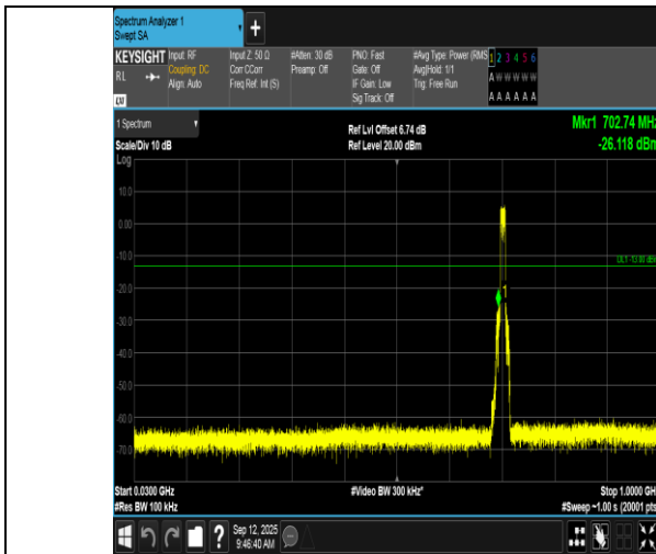
Band17-10MHz-QPSK-23790-50RB#0-30~1000-PASS
