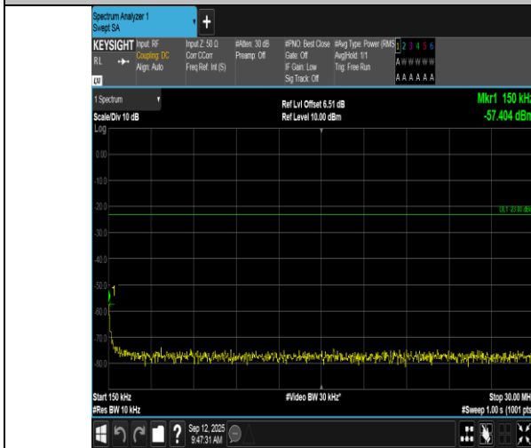
Band17-10MHz-16QAM-23790-50RB#0-0.15~30-PASS
