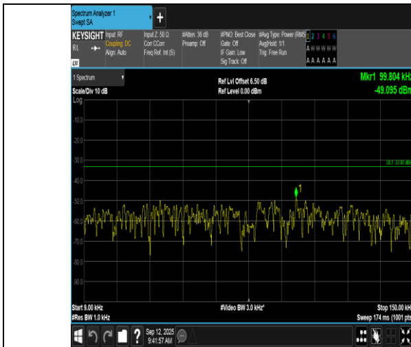
Band17-10MHz-QPSK-23790-1RB#0-0.009~0.15-PASS
