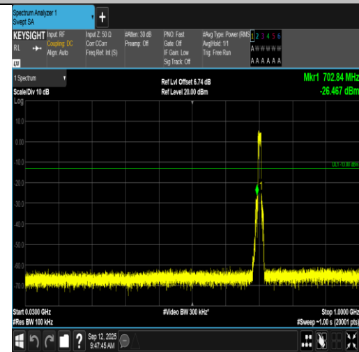
Band17-10MHz-16QAM-23790-50RB#0-30~1000-PASS
