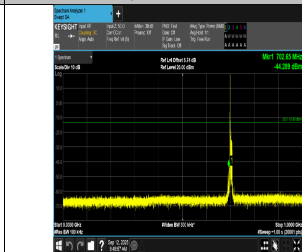
Band17-10MHz-16QAM-23800-1RB#0-30~1000-PASS
