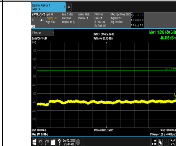
Band17-10MHz-16QAM-23800-50RB#0-3000~10000-PASS
