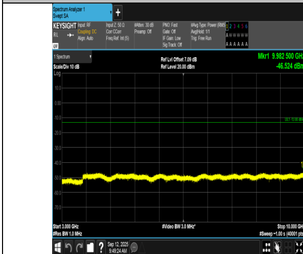
Band17-10MHz-QPSK-23800-1RB#0-3000~10000-PASS
