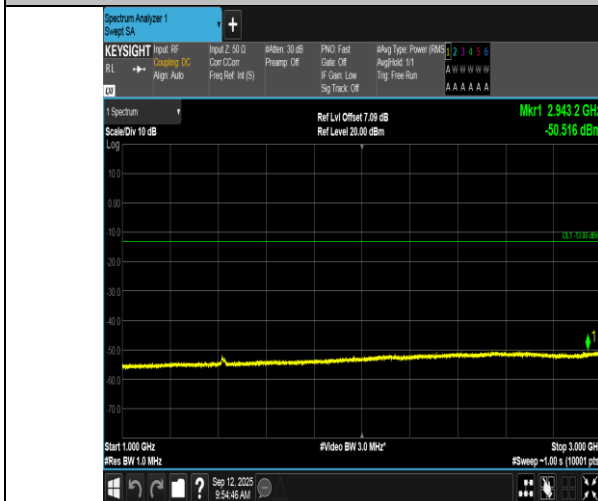
Band17-10MHz-16QAM-23800-50RB#0-1000~3000-PASS
