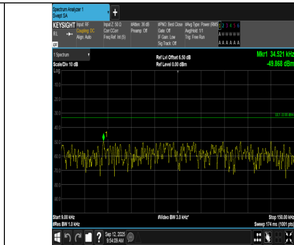
Band17-10MHz-16QAM-23800-50RB#0-0.009~0.15-PASS
