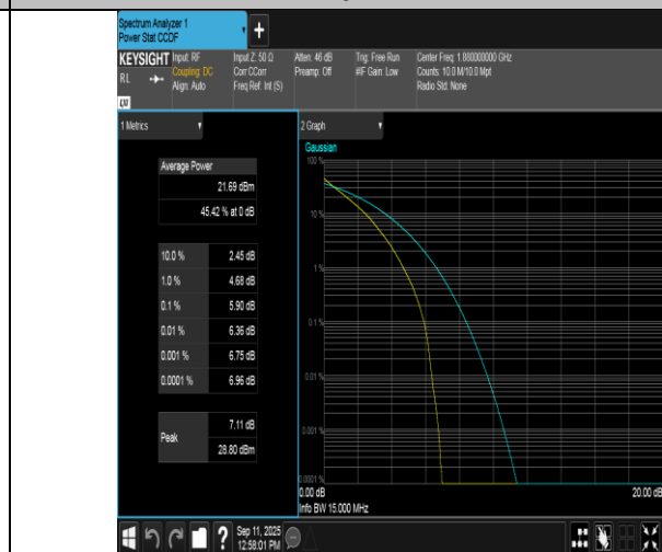
Band2-15MHz-QPSK-18900-75RB#0-PASS
