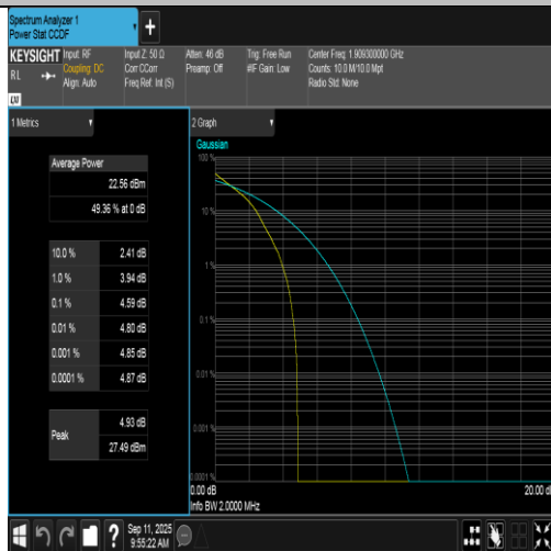
Band2-1.4MHz-QPSK-19193-1RB#0-PASS
