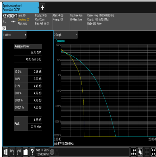
Band2-15MHz-QPSK-19125-1RB#0-PASS
