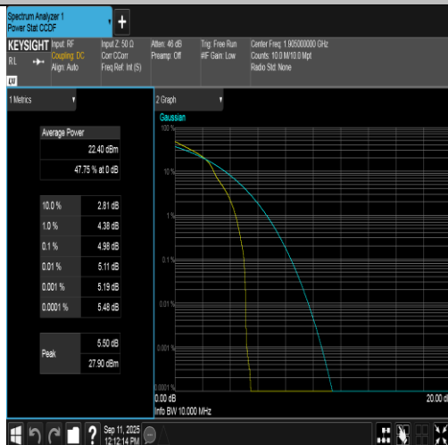
Band2-10MHz-16QAM-19150-1RB#0-PASS
