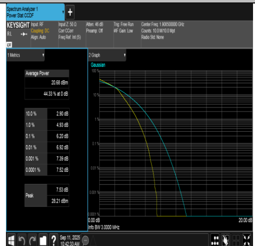
Band2-3MHz-16QAM-19185-15RB#0-PASS
