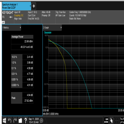
Band2-3MHz-QPSK-19185-1RB#0-PASS
