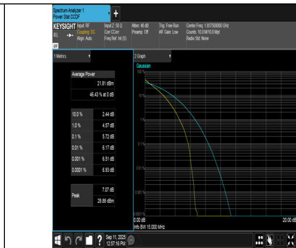
Band2-15MHz-QPSK-18675-75RB#0-PASS
