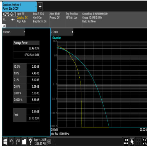
Band2-15MHz-16QAM-19125-1RB#0-PASS
