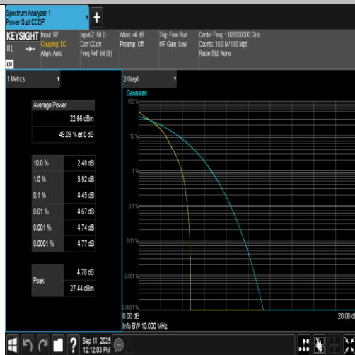
Band2-10MHz-QPSK-19150-1RB#0-PASS
