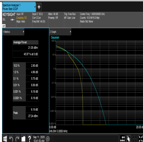
Band2-3MHz-16QAM-19185-1RB#0-PASS
