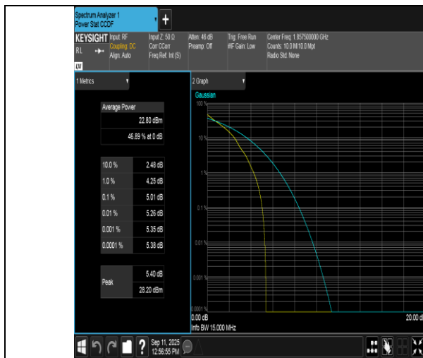
Band2-15MHz-QPSK-18675-1RB#0-PASS
