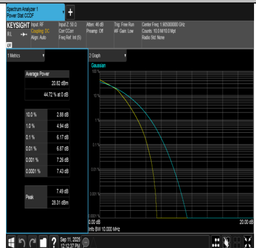
Band2-10MHz-16QAM-19150-50RB#0-PASS
