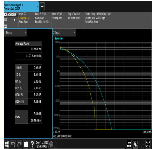
Band2-1.4MHz-16QAM-18900-6RB#0-PASS
