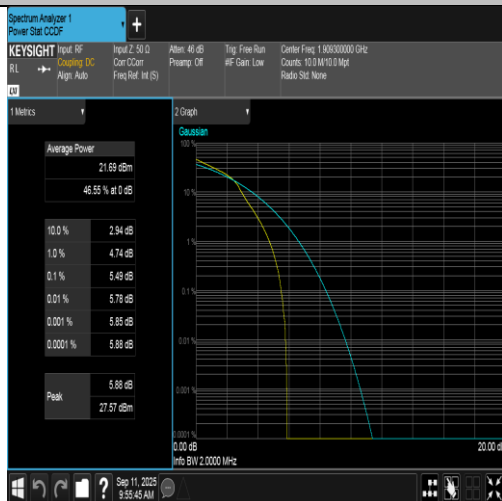
Band2-1.4MHz-16QAM-19193-1RB#0-PASS
