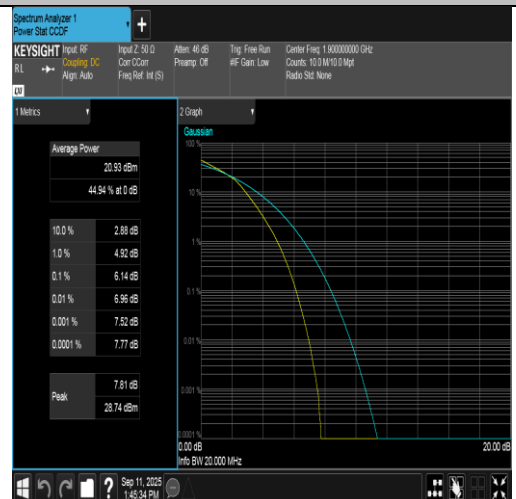
Band2-20MHz-16QAM-19100-100RB#0-PASS
