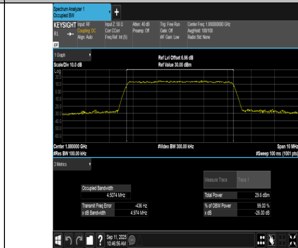
Band2-5MHz-16QAM-18900-25RB#0-PASS
