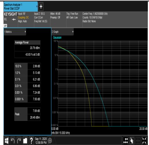
Band2-15MHz-16QAM-19125-75RB#0-PASS
