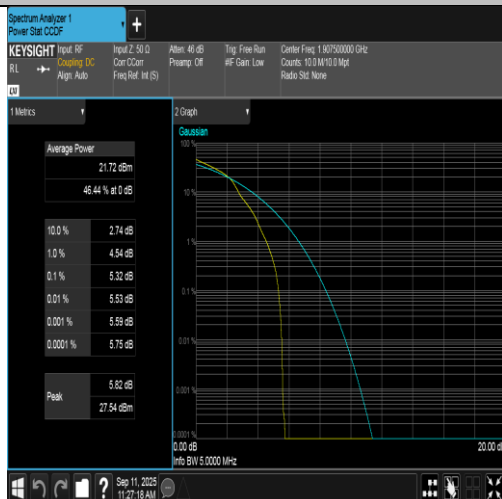
Band2-5MHz-16QAM-19175-1RB#0-PASS
