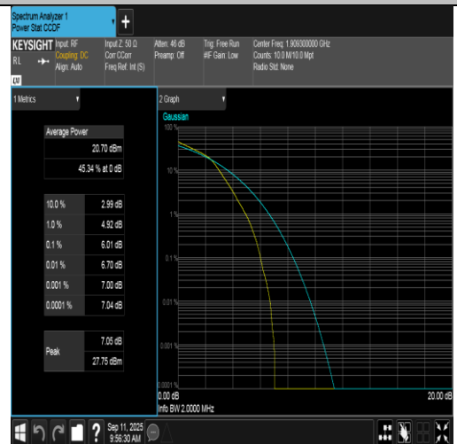
Band2-1.4MHz-16QAM-19193-6RB#0-PASS
