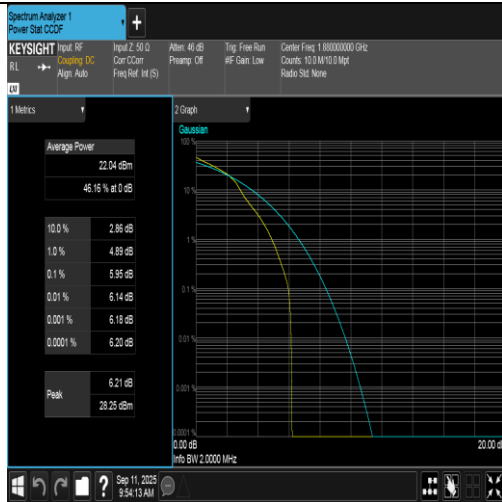
Band2-1.4MHz-16QAM-18900-1RB#0-PASS
