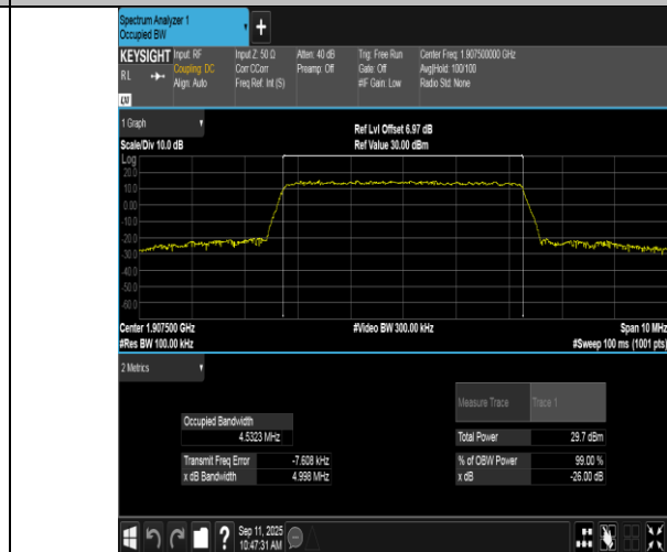
Band2-5MHz-16QAM-19175-25RB#0-PASS
