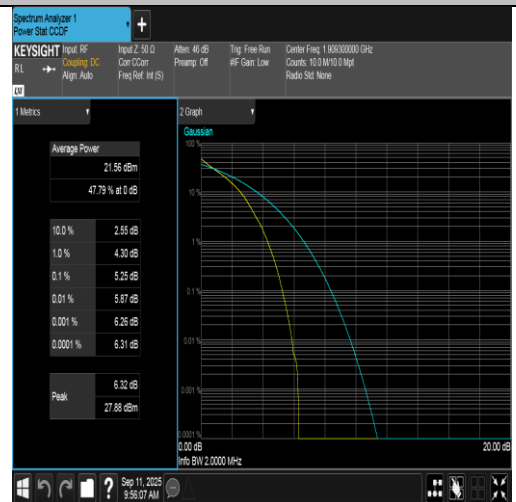
Band2-1.4MHz-QPSK-19193-6RB#0-PASS
