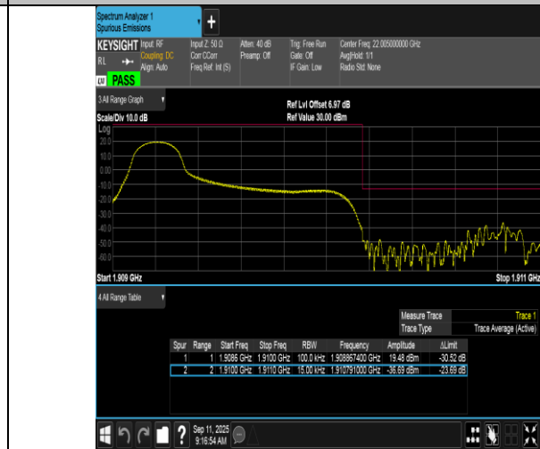
Band2-1.4MHz-16QAM-19193-1RB#0-PASS
