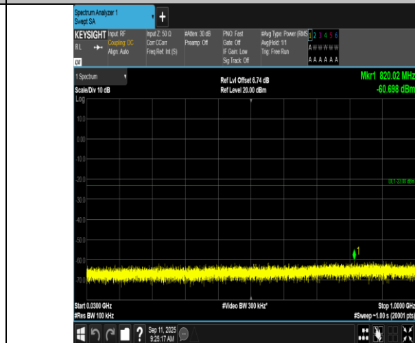
Band2-1.4MHz-16QAM-18900-1RB#0-30~1000-PASS
