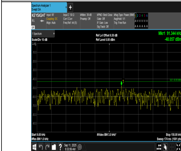
Band2-1.4MHz-QPSK-19193-6RB#0-0.009~0.15-PASS
