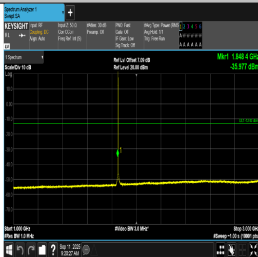
Band2-1.4MHz-QPSK-18607-1RB#5-1000~3000-PASS
