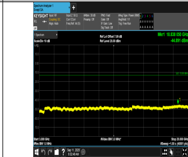
Band2-1.4MHz-QPSK-19193-1RB#5-3000~20000-PASS
