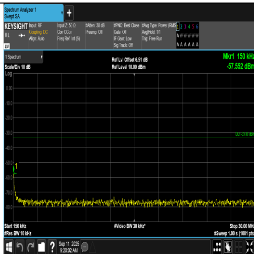
Band2-1.4MHz-QPSK-18607-1RB#5-0.15~30-PASS
