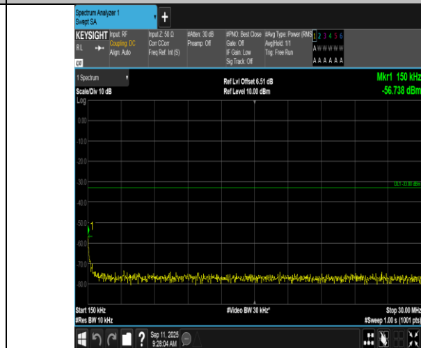
Band2-1.4MHz-QPSK-18900-6RB#0-0.15~30-PASS
