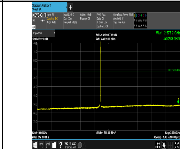
Band2-1.4MHz-16QAM-18900-1RB#5-1000-3000-PASS
