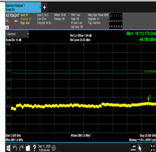
Band2-1.4MHz-16QAM-18900-6RB#0-3000~20000-PASS
