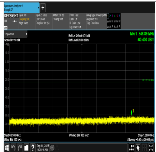
Band2-1.4MHz-QPSK-18607-1RB#5-30~1000-PASS
