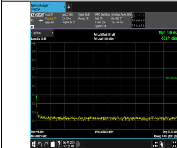
Band2-1.4MHz-16QAM-19193-1RB#0-0.15~30-PASS
