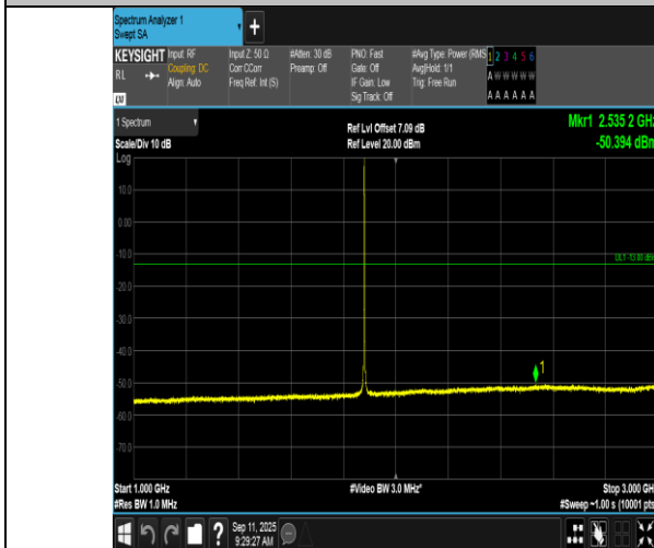
Band2-1.4MHz-16QAM-18900-6RB#0-1000~3000-PASS
