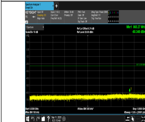
Band2-1.4MHz-16QAM-18607-1RB#5-30-1000-PASS
