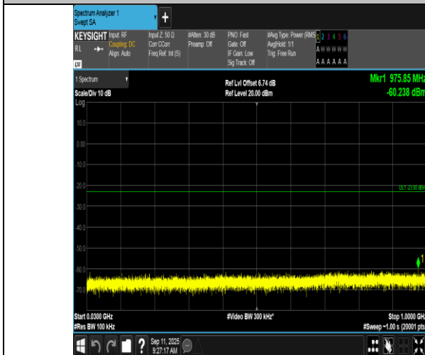
Band2-1.4MHz-16QAM-18900-1RB#5-30-1000-PASS
