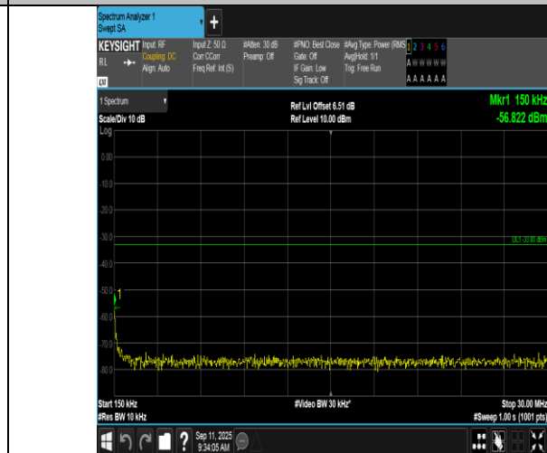
Band2-1.4MHz-QPSK-19193-6RB#0-0.15~30-PASS
