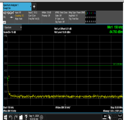
Band2-1.4MHz-QPSK-18607-6RB#0-0.15~30-PASS
