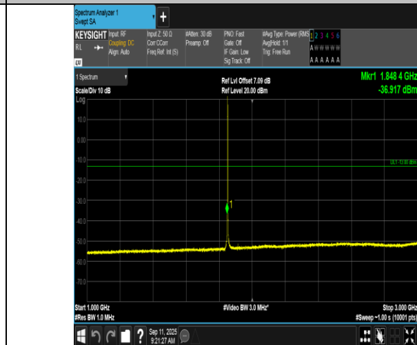
Band2-1.4MHz-16QAM-18607-1RB#5-1000-3000-PASS
