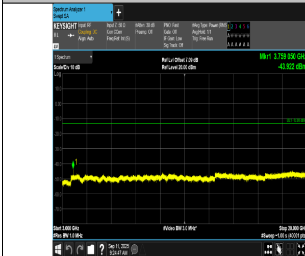
Band2-1.4MHz-QPSK-18900-1RB#0-3000~20000-PASS
