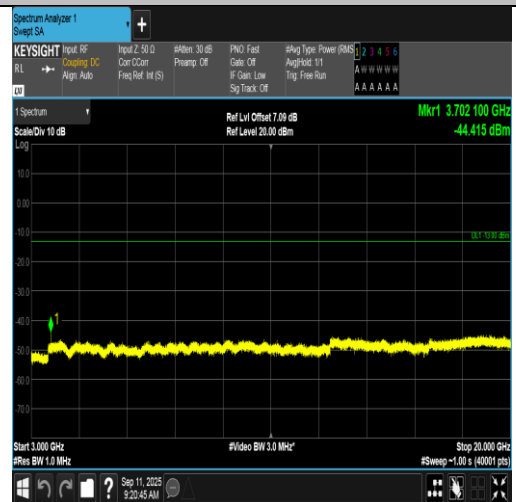
Band2-1.4MHz-QPSK-18607-1RB#5-3000~20000-PASS
