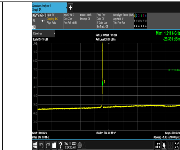
Band2-1.4MHz-QPSK-19193-6RB#0-1000~3000-PASS
