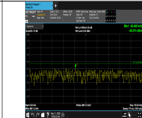
Band2-3MHz-QPSK-18615-1RB#14-0.009~0.15-PASS
