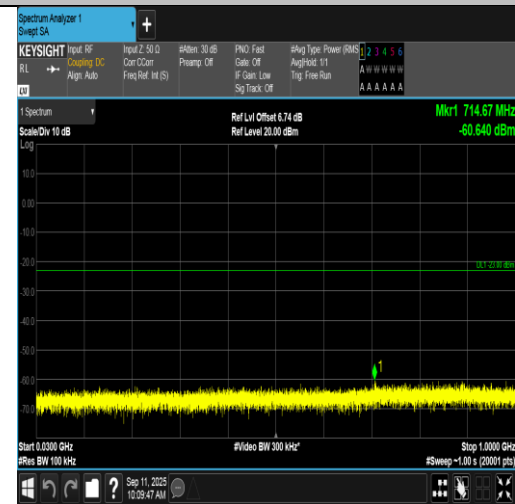
Band2-3MHz-16QAM-18615-15RB#0-30~1000-PASS
