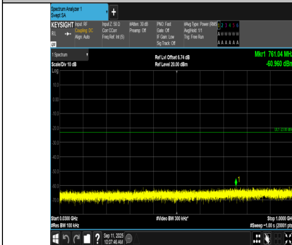
Band2-3MHz-16QAM-18615-1RB#14-30~1000-PASS
