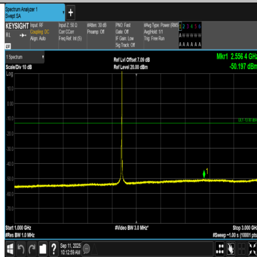
Band2-3MHz-QPSK-18900-1RB#14-1000~3000-PASS
