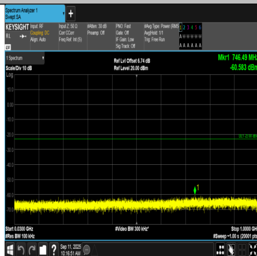
Band2-3MHz-QPSK-19185-1RB#0-30~1000-PASS
