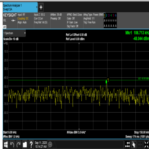
Band2-3MHz-QPSK-18900-15RB#0-0.009~0.15-PASS
