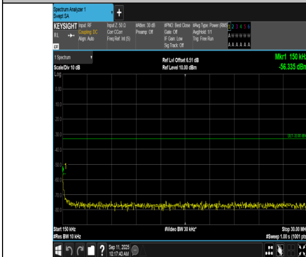
Band2-3MHz-16QAM-19185-1RB#0-0.15~30-PASS
