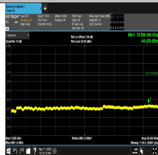
Band2-3MHz-16QAM-18615-15RB#0-3000~20000-PASS
