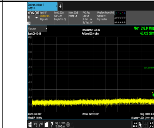
Band2-3MHz-16QAM-18615-1RB#0-30~1000-PASS
