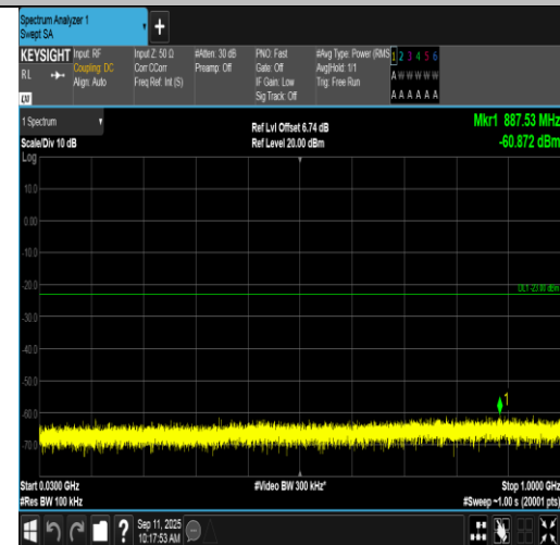
Band2-3MHz-16QAM-19185-1RB#0-30~1000-PASS
