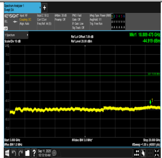
Band2-3MHz-QPSK-18900-1RB#14-3000~20000-PASS
