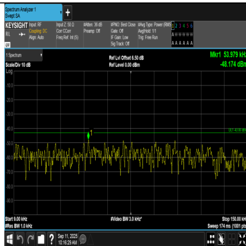
Band2-3MHz-QPSK-19185-1RB#0-0.009~0.15-PASS
