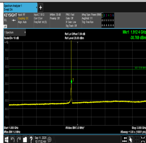
Band2-3MHz-QPSK-19185-1RB#0-1000~3000-PASS
