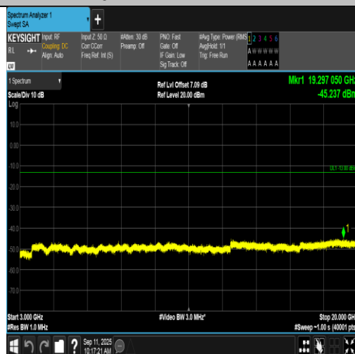
Band2-3MHz-QPSK-19185-1RB#0-3000~20000-PASS
