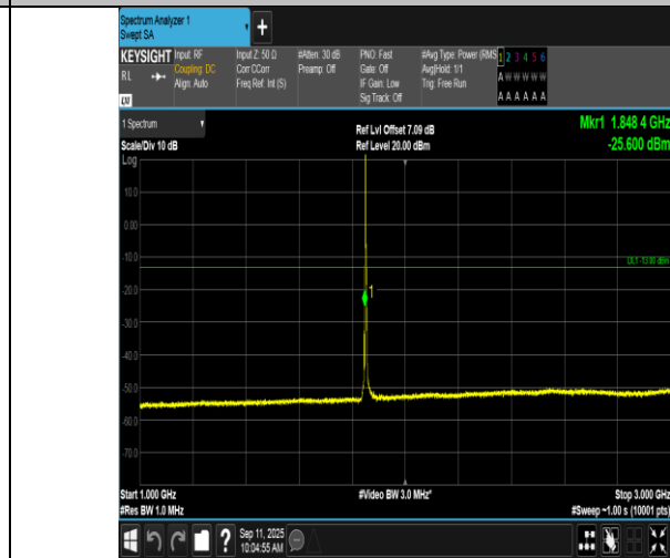
Band2-3MHz-QPSK-18615-1RB#0-1000~3000-PASS
