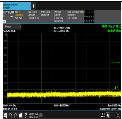
Band2-3MHz-QPSK-18900-1RB#14-30~1000-PASS
