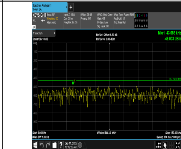
Band2-3MHz-QPSK-18900-1RB#14-0.009~0.15-PASS
