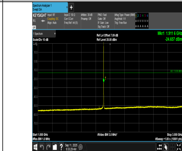
Band2-1.4MHz-16QAM-19193-1RB#5-1000~3000-PASS
