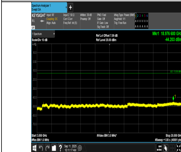
Band2-3MHz-QPSK-18900-1RB#0-3000~20000-PASS
