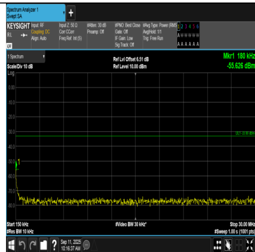
Band2-3MHz-QPSK-19185-1RB#0-0.15~30-PASS
