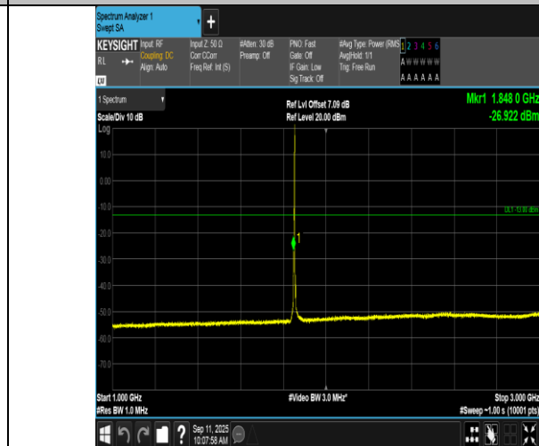
Band2-3MHz-16QAM-18615-1RB#14-1000~3000-PASS
