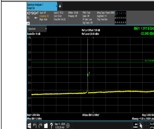
Band2-1.4MHz-16QAM-19193-6RB#0-1000~3000-PASS
