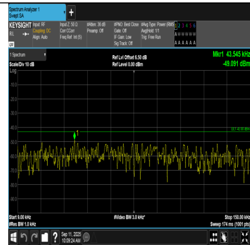
Band2-3MHz-16QAM-18615-15RB#0-0.009~0.15-PASS
