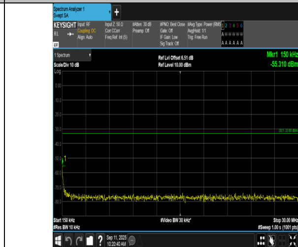
Band2-3MHz-QPSK-19185-15RB#0-0.15~30-PASS
