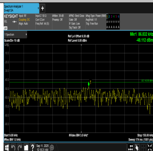
Band2-3MHz-QPSK-19185-1RB#14-0.009~0.15-PASS
