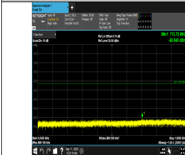
Band2-1.4MHz-16QAM-19193-1RB#5-30~1000-PASS
