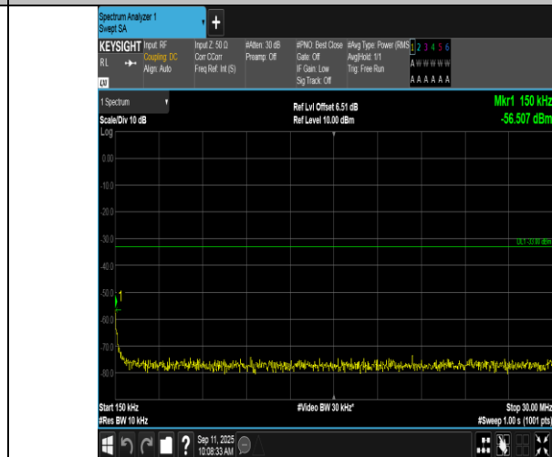
Band2-3MHz-QPSK-18615-15RB#0-0.15~30-PASS
