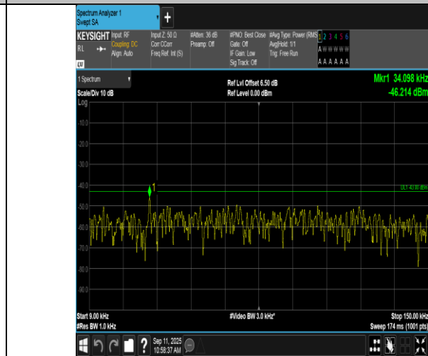
Band2-5MHz-QPSK-18900-1RB#24-0.009~0.15-PASS
