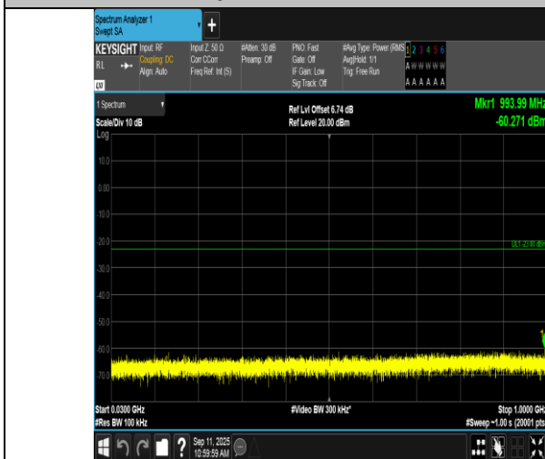
Band2-5MHz-16QAM-18900-1RB#24-30~1000-PASS
