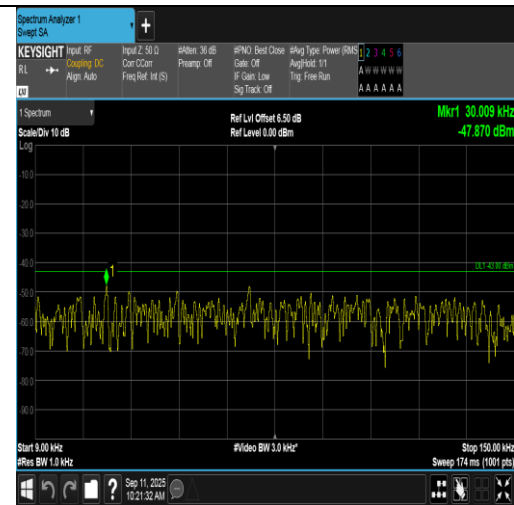
Band2-3MHz-16QAM-19185-15RB#0-0.009~0.15-PASS
