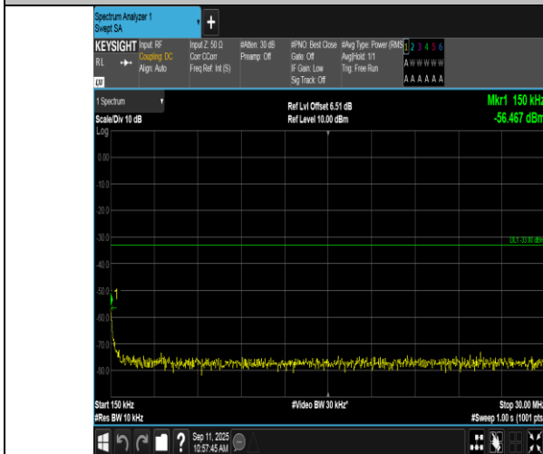
Band2-5MHz-16QAM-18900-1RB#0-0.15~30-PASS
