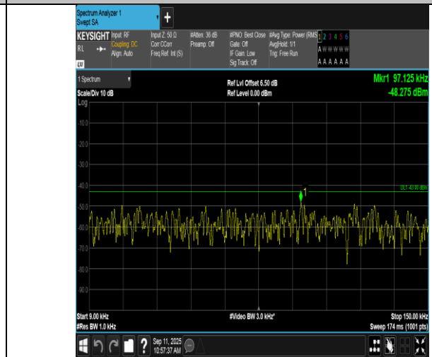
Band2-5MHz-16QAM-18900-1RB#0-0.009~0.15-PASS
