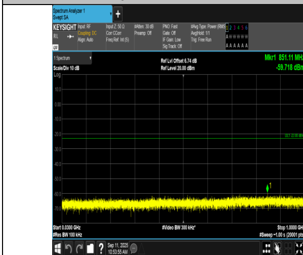
Band2-5MHz-16QAM-18625-1RB#24-30~1000-PASS
