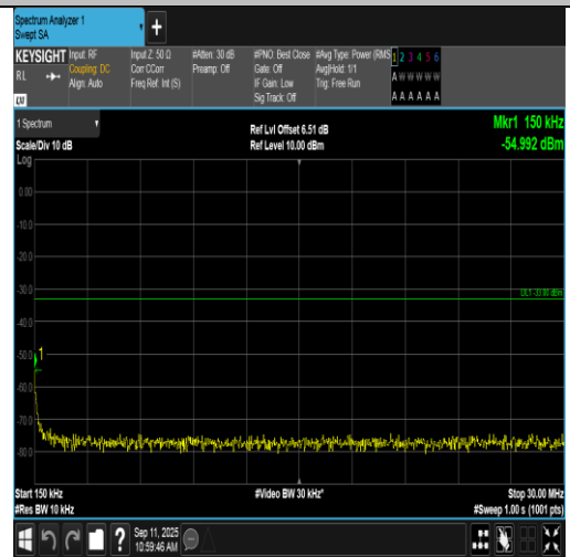
Band2-5MHz-16QAM-18900-1RB#24-0.15~30-PASS
