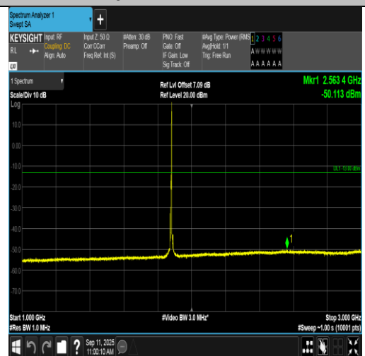
Band2-5MHz-16QAM-18900-1RB#24-1000~3000-PASS
