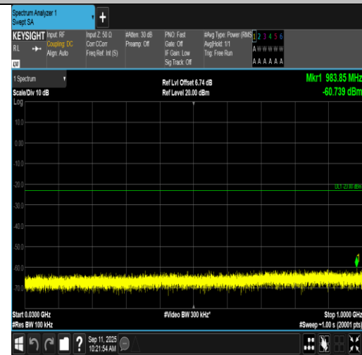
Band2-3MHz-16QAM-19185-15RB#0-30~1000-PASS
