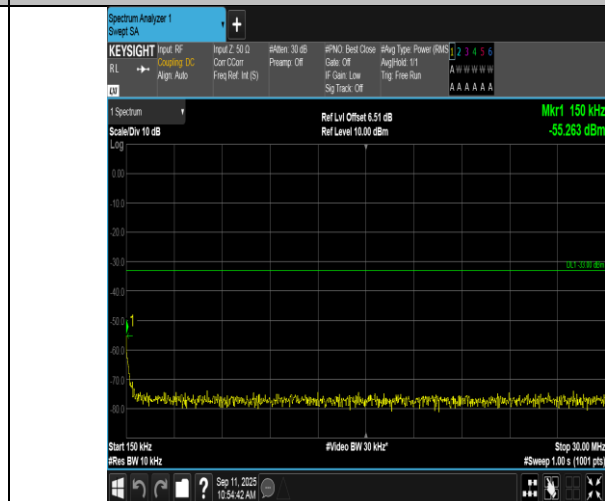
Band2-5MHz-QPSK-18625-25RB#0-0.15~30-PASS
