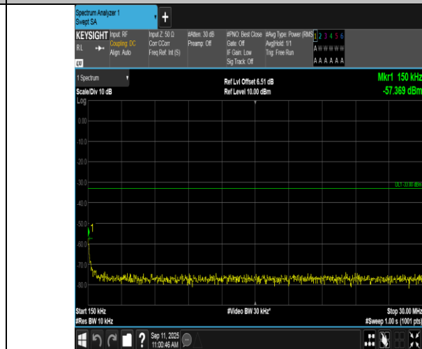
Band2-5MHz-QPSK-18900-25RB#0-0.15~30-PASS
