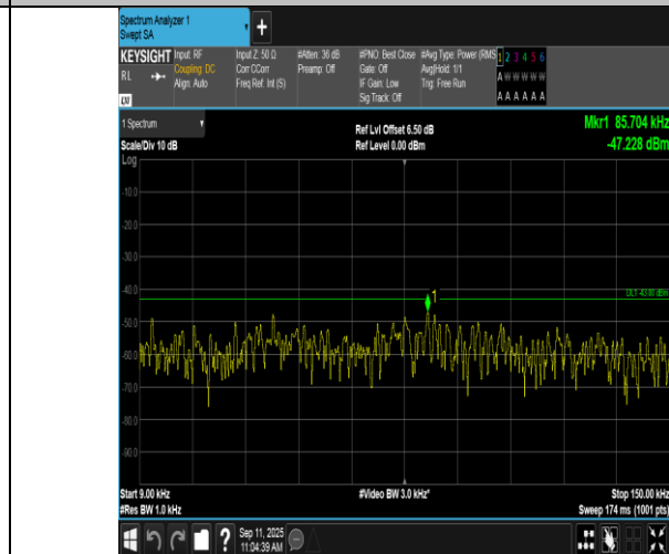
Band2-5MHz-QPSK-19175-1RB#24-0.009~0.15-PASS
