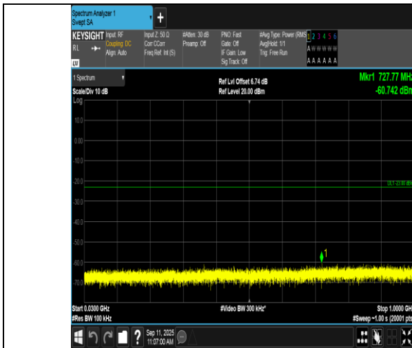
Band2-5MHz-QPSK-19175-25RB#0-30~1000-PASS
