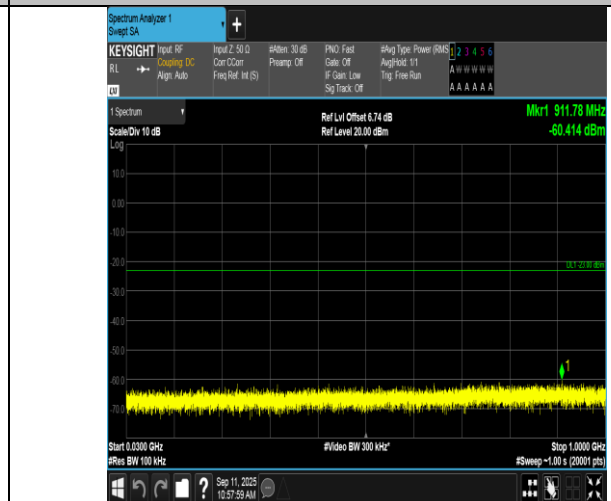
Band2-5MHz-16QAM-18900-1RB#0-30~1000-PASS
