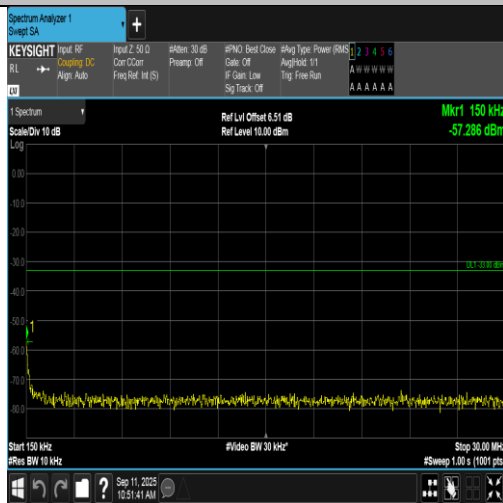
Band2-5MHz-16QAM-18625-1RB#0-0.15~30-PASS
