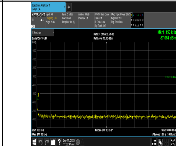
Band2-5MHz-QPSK-19175-25RB#0-0.15~30-PASS
