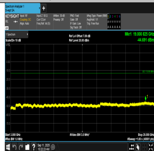
Band2-3MHz-16QAM-19185-15RB#0-3000~20000-PASS
