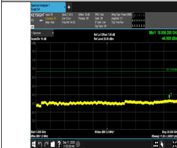
Band2-5MHz-QPSK-19175-1RB#0-3000~20000-PASS
