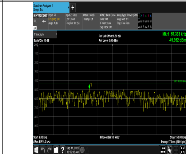
Band2-5MHz-QPSK-18625-1RB#24-0.009~0.15-PASS
