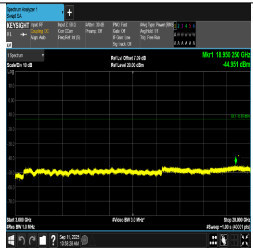
Band2-5MHz-16QAM-18900-1RB#0-3000~20000-PASS
