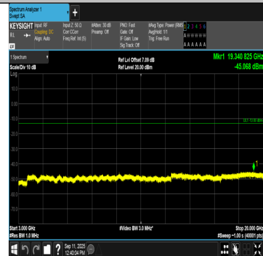
Band2-15MHz-16QAM-19125-75RB#0-3000~20000-PASS
