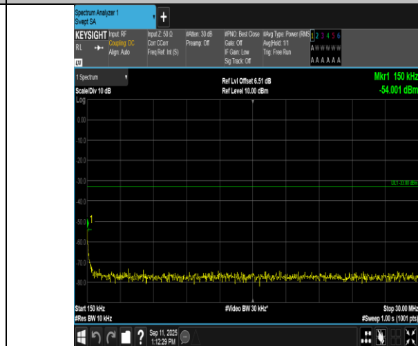
Band2-20MHz-QPSK-18700-100RB#0-0.15~30-PASS
