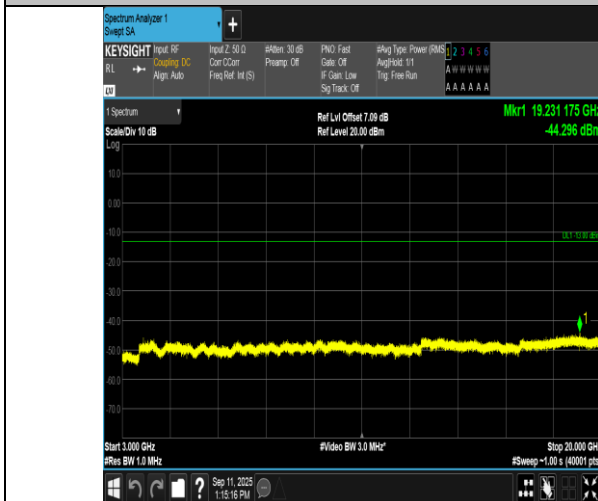
Band2-20MHz-QPSK-18900-1RB#0-3000~20000-PASS
