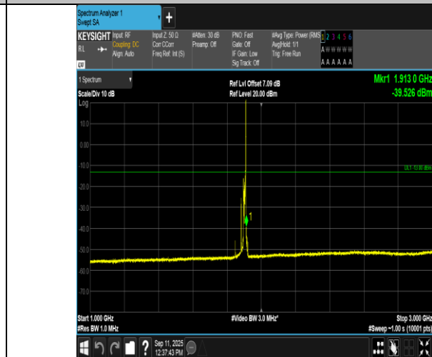
Band2-15MHz-16QAM-19125-1RB#74-1000~3000-PASS
