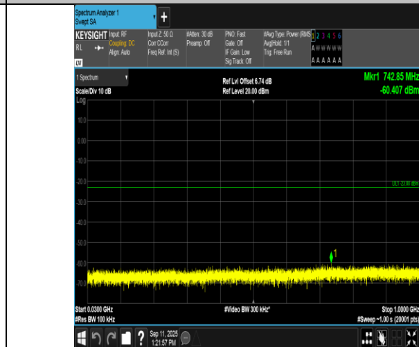
Band2-20MHz-16QAM-19100-1RB#0-30~1000-PASS
