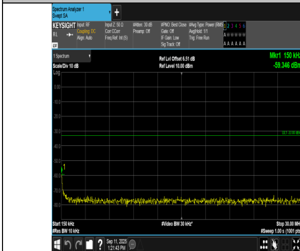
Band2-20MHz-16QAM-19100-1RB#0-0.15~30-PASS
