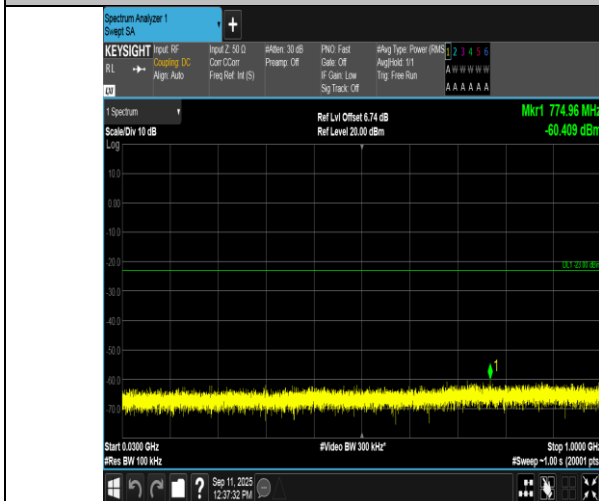
Band2-15MHz-16QAM-19125-1RB#74-30~1000-PASS
