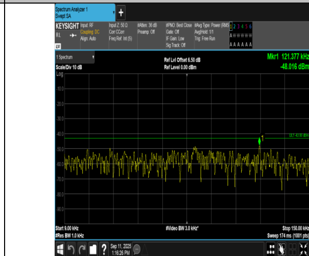
Band2-20MHz-QPSK-18900-1RB#99-0.009~0.15-PASS
