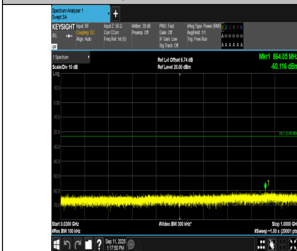
Band2-20MHz-16QAM-18900-1RB#99-30~1000-PASS
