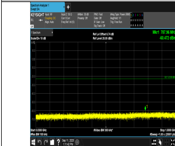
Band2-20MHz-16QAM-18700-1RB#99-30~1000-PASS
