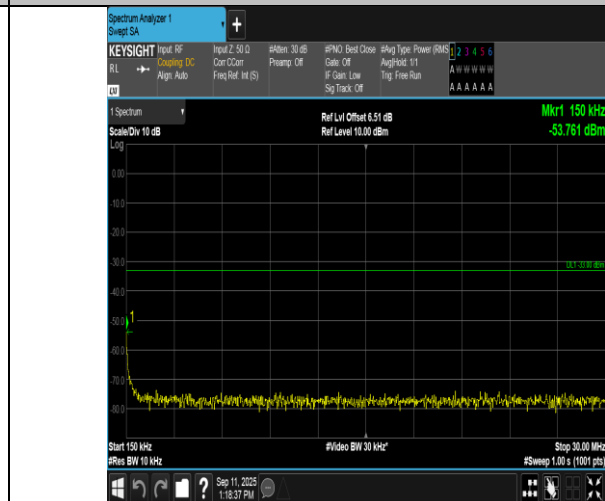
Band2-20MHz-QPSK-18900-100RB#0-0.15~30-PASS
