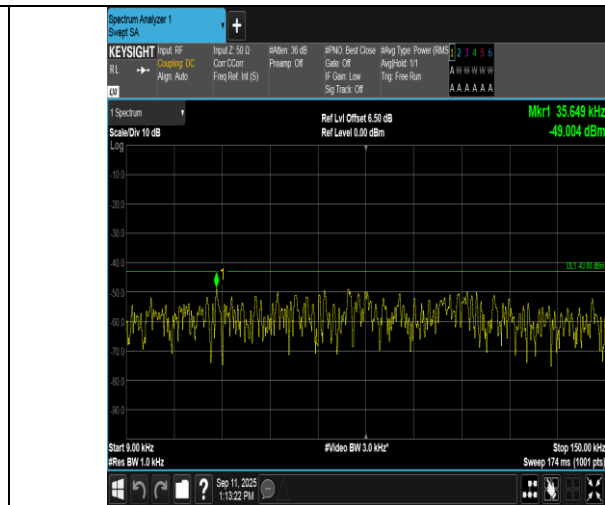
Band2-20MHz-16QAM-18700-100RB#0-0.009~0.15-PASS
