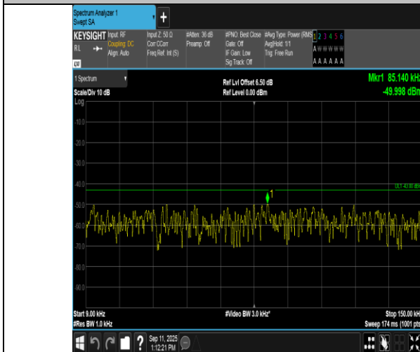
Band2-20MHz-QPSK-18700-100RB#0-0.009~0.15-PASS
