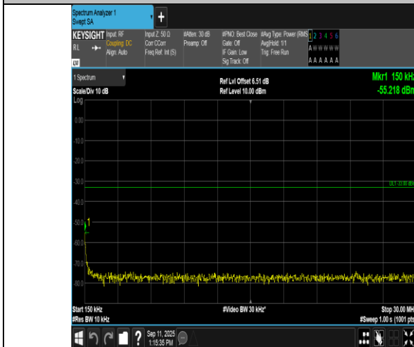
Band2-20MHz-16QAM-18900-1RB#0-0.15~30-PASS
