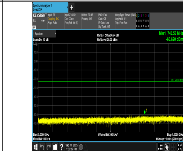
Band2-20MHz-16QAM-18700-1RB#0-30~1000-PASS
