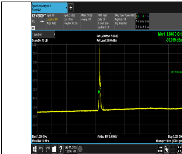
Band2-20MHz-16QAM-18700-1RB#0-1000~3000-PASS
