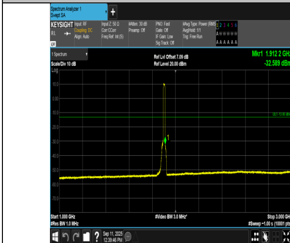
Band2-15MHz-16QAM-19125-75RB#0-1000~3000-PASS
