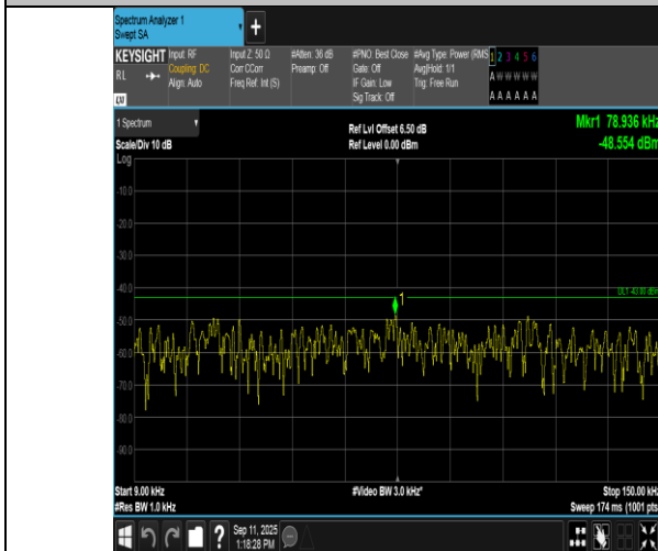
Band2-20MHz-QPSK-18900-100RB#0-0.009~0.15-PASS
