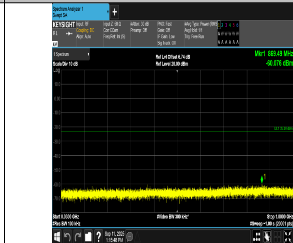
Band2-20MHz-16QAM-18900-1RB#0-30~1000-PASS
