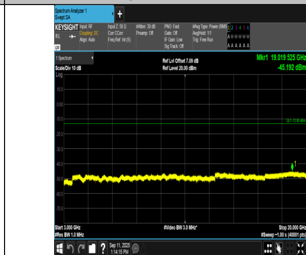
Band2-20MHz-16QAM-18700-100RB#0-3000~20000-PASS
