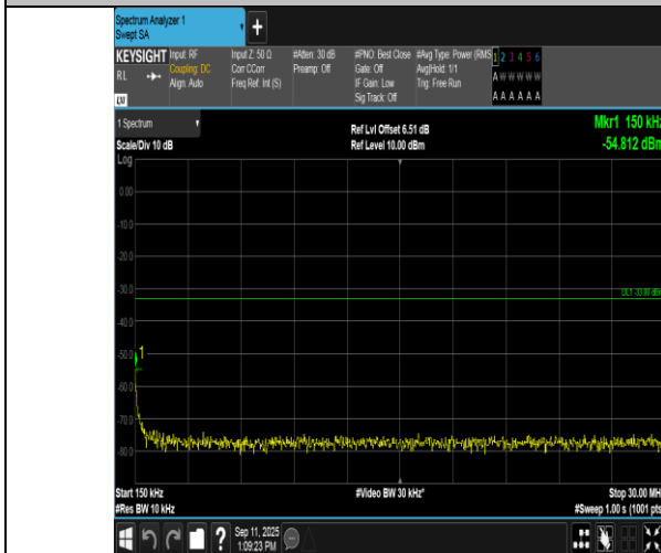
Band2-20MHz-16QAM-18700-1RB#0-0.15~30-PASS
