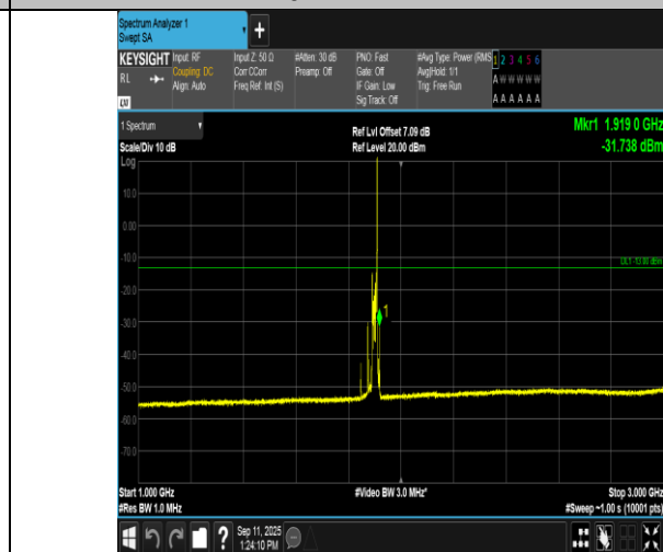
Band2-20MHz-16QAM-19100-1RB#99-1000~3000-PASS
