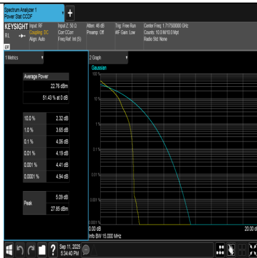
Band4-15MHz-QPSK-20025-1RB#0-PASS
