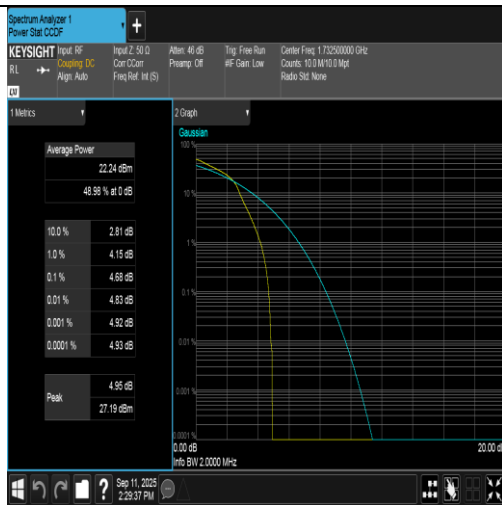
Band4-1.4MHz-16QAM-20175-1RB#0-PASS
