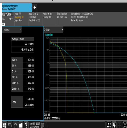
Band4-1.4MHz-16QAM-20393-1RB#0-PASS
