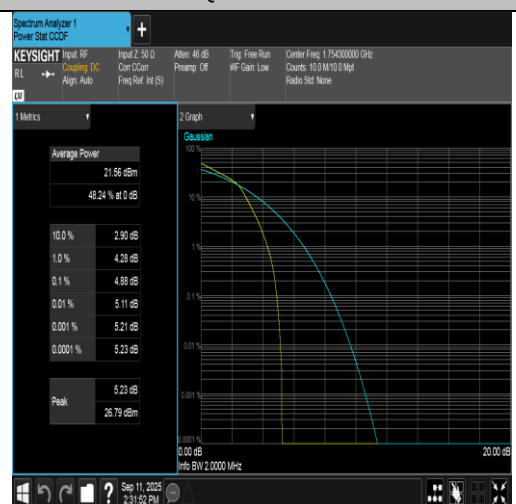
Band4-1.4MHz-16QAM-20393-6RB#0-PASS
