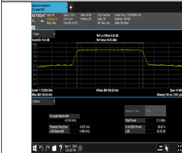
Band4-5MHz-QPSK-20175-25RB#0-PASS
