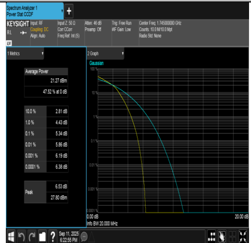
Band4-20MHz-16QAM-20300-100RB#0-PASS
