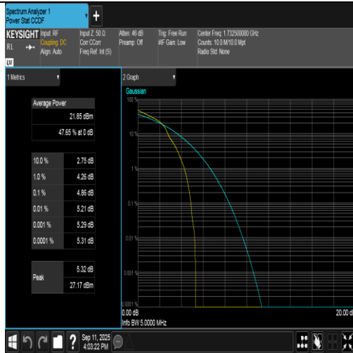
Band4-5MHz-16QAM-20175-1RB#0-PASS
