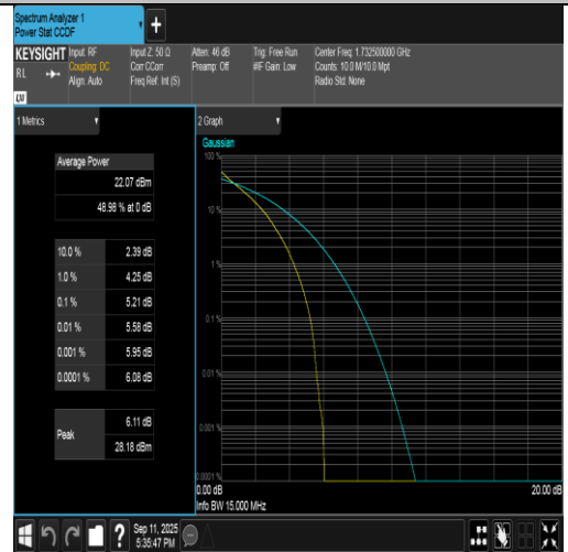
Band4-15MHz-QPSK-20175-75RB#0-PASS
