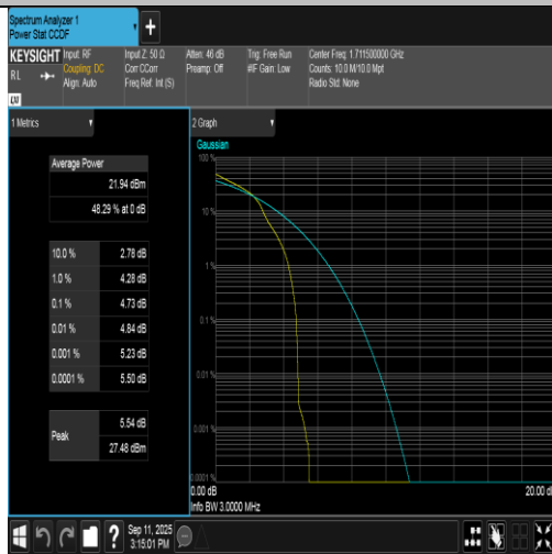
Band4-3MHz-16QAM-19965-1RB#0-PASS
