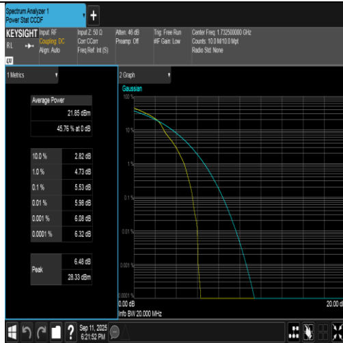
Band4-20MHz-16QAM-20175-1RB#0-PASS
