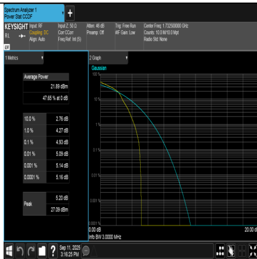
Band4-3MHz-16QAM-20175-1RB#0-PASS
