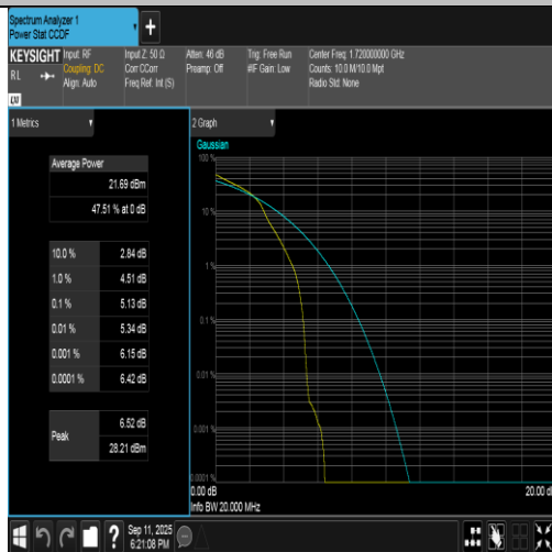
Band4-20MHz-16QAM-20050-1RB#0-PASS
