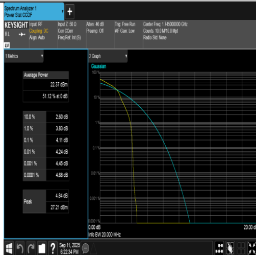
Band4-20MHz-16QAM-20300-1RB#0-PASS
