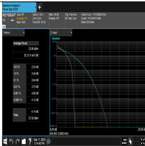
Band4-3MHz-QPSK-19965-1RB#0-PASS
