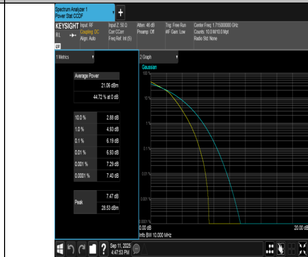
Band4-10MHz-16QAM-20000-50RB#0-PASS
