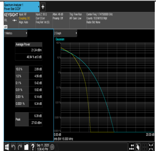
Band4-15MHz-16QAM-20325-75RB#0-PASS
