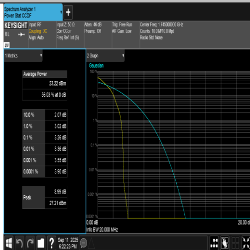
Band4-20MHz-QPSK-20300-1RB#0-PASS
