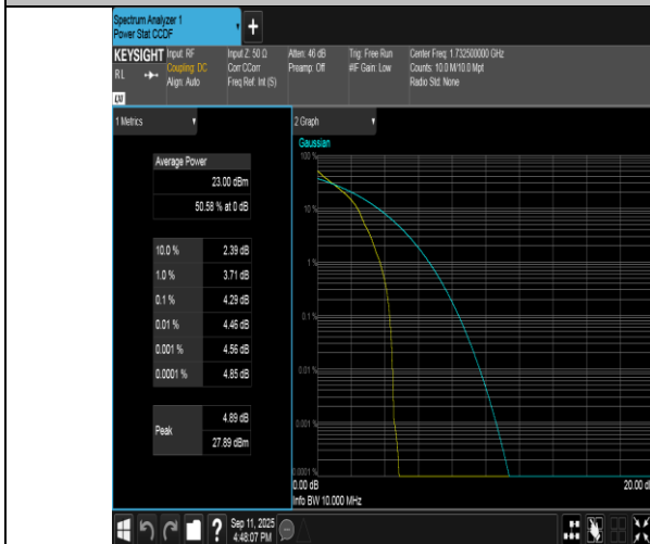
Band4-10MHz-QPSK-20175-1RB#0-PASS
