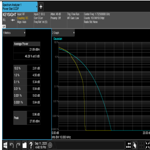
Band4-10MHz-16QAM-20175-1RB#0-PASS
