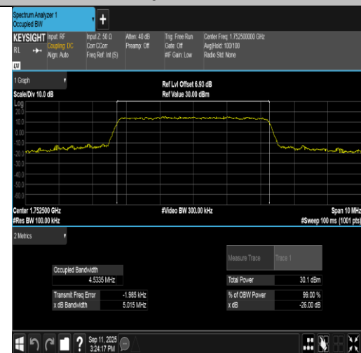
Band4-5MHz-16QAM-20375-25RB#0-PASS
