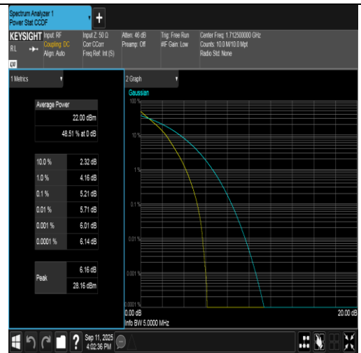
Band4-5MHz-QPSK-19975-25RB#0-PASS
