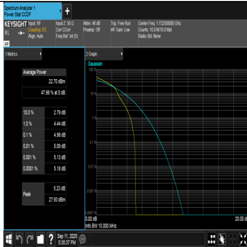
Band4-15MHz-16QAM-20175-1RB#0-PASS
