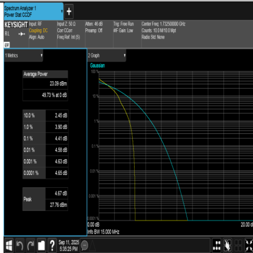
Band4-15MHz-QPSK-20175-1RB#0-PASS
