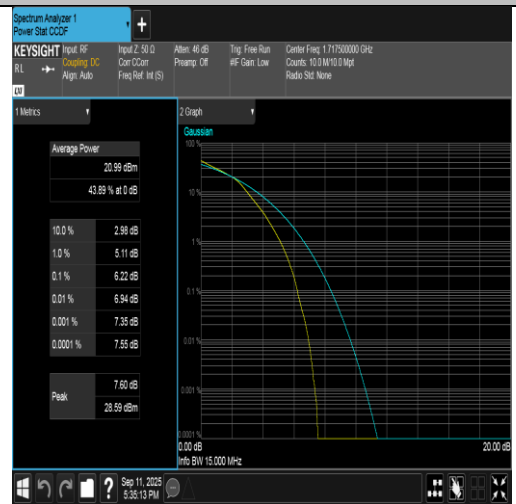
Band4-15MHz-16QAM-20025-75RB#0-PASS
