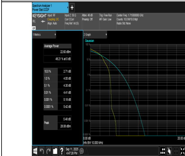
Band4-10MHz-16QAM-20000-1RB#0-PASS
