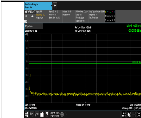
Band4-3MHz-16QAM-20175-1RB#0-0.15~30-PASS
