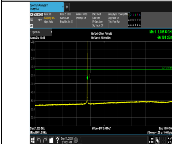
Band4-1.4MHz-16QAM-20393-6RB#0-1000~3000-PASS
