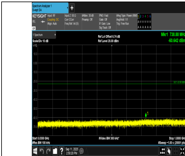
Band4-3MHz-QPSK-20175-15RB#0-30~1000-PASS
