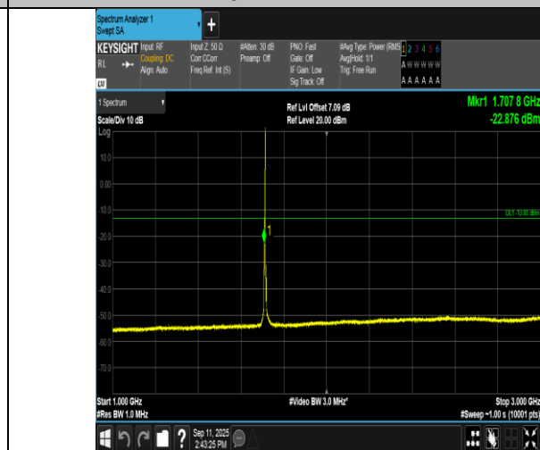
Band4-3MHz-16QAM-19965-1RB#14-1000~3000-PASS
