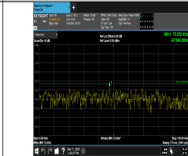
Band4-3MHz-16QAM-20175-1RB#0-0.009~0.15-PASS
