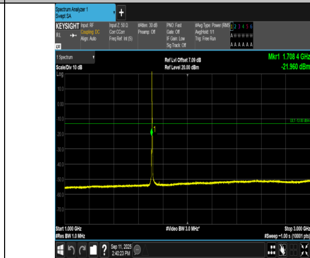
Band4-3MHz-QPSK-19965-1RB#0-1000~3000-PASS
