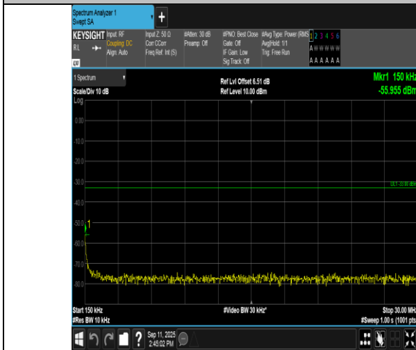
Band4-3MHz-16QAM-19965-15RB#0-0.15~30-PASS
