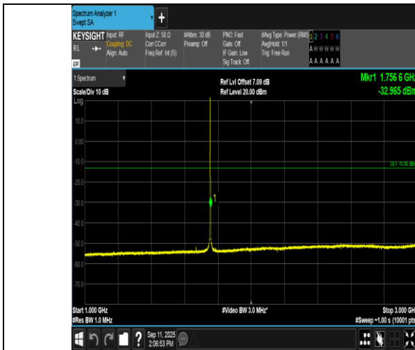
Band4-1.4MHz-16QAM-20393-1RB#0-1000~3000-PASS
