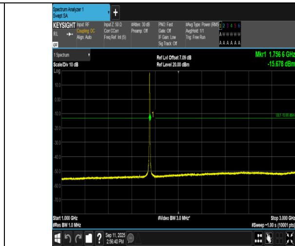
Band4-3MHz-QPSK-20385-15RB#0-1000~3000-PASS
