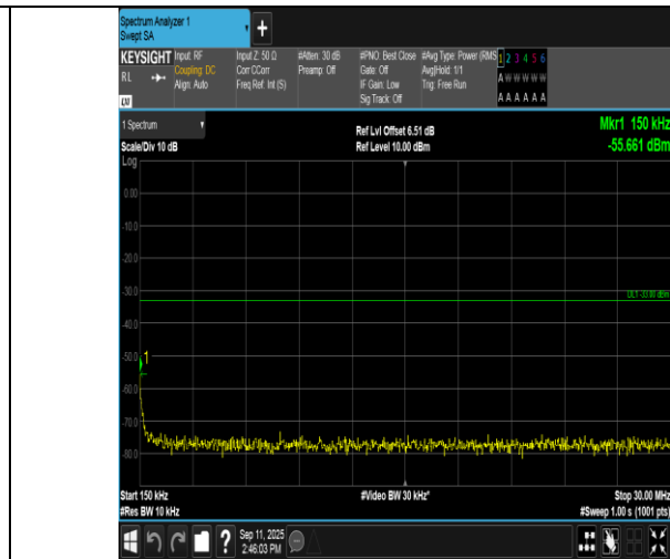
Band4-3MHz-QPSK-20175-1RB#0-0.15~30-PASS
