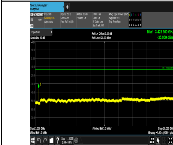
Band4-3MHz-QPSK-19965-15RB#0-3000~20000-PASS
