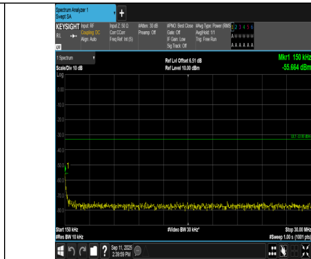
Band4-3MHz-QPSK-19965-1RB#0-0.15~30-PASS
