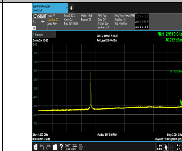
Band4-3MHz-16QAM-20175-1RB#14-1000~3000-PASS
