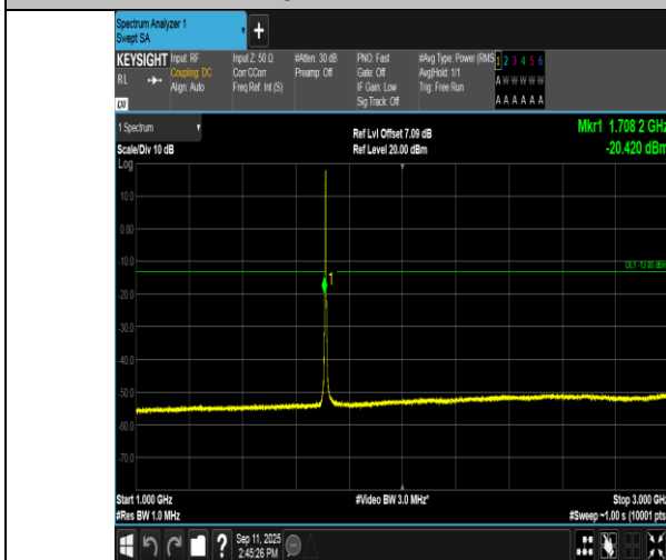
Band4-3MHz-16QAM-19965-15RB#0-1000~3000-PASS
