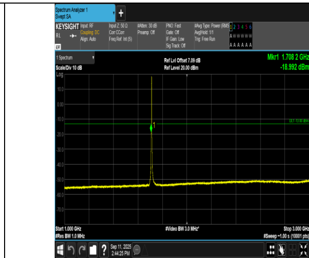
Band4-3MHz-QPSK-19965-15RB#0-1000~3000-PASS
