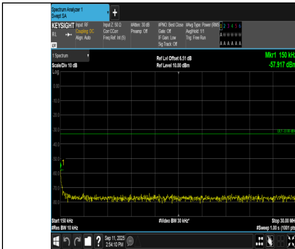
Band4-3MHz-QPSK-20385-1RB#14-0.15~30-PASS
