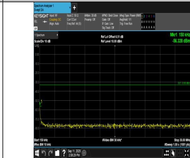
Band4-1.4MHz-16QAM-20393-1RB#5-0.15~30-PASS
