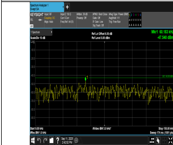
Band4-3MHz-16QAM-19965-1RB#14-0.009~0.15-PASS
