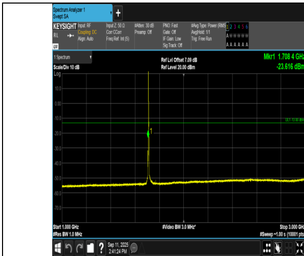
Band4-3MHz-16QAM-19965-1RB#0-1000~3000-PASS
