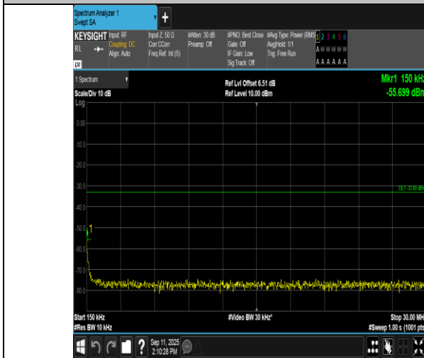
Band4-1.4MHz-16QAM-20393-6RB#0-0.15~30-PASS
