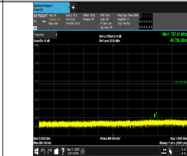
Band4-3MHz-16QAM-20175-1RB#0-30~1000-PASS
