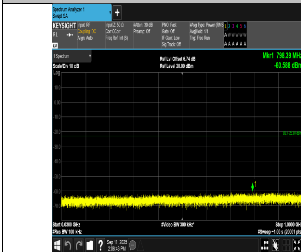
Band4-1.4MHz-16QAM-20393-1RB#5-30~1000-PASS
