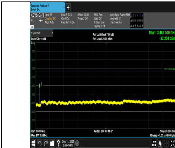
Band4-3MHz-16QAM-20175-1RB#14-3000~20000-PASS
