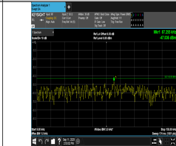
Band4-3MHz-16QAM-20385-1RB#0-0.009~0.15-PASS
