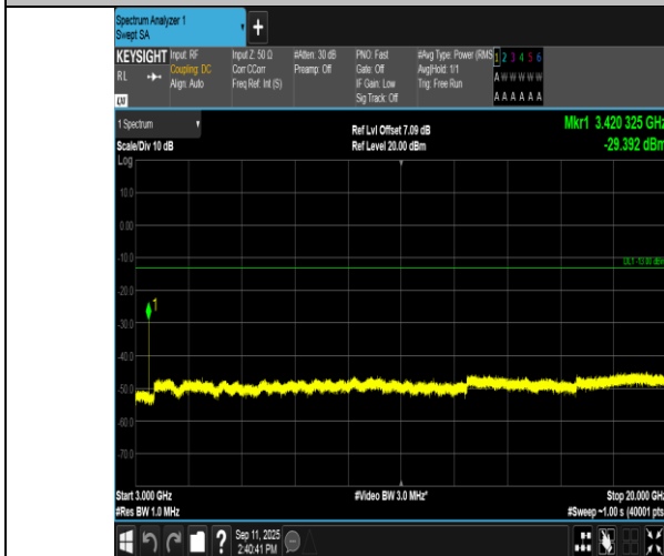
Band4-3MHz-QPSK-19965-1RB#0-3000~20000-PASS
