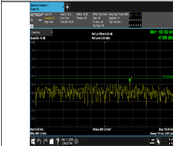
Band4-3MHz-16QAM-20175-1RB#14-0.009~0.15-PASS
