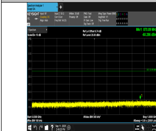
Band4-3MHz-16QAM-20175-1RB#14-30~1000-PASS
