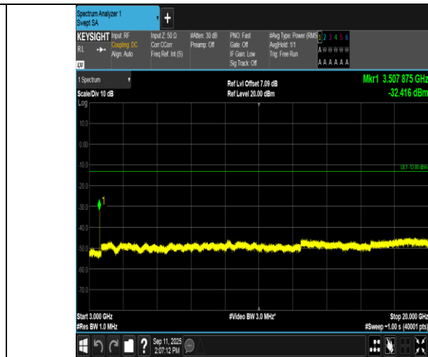
Band4-1.4MHz-16QAM-20393-1RB#0-3000~20000-PASS
