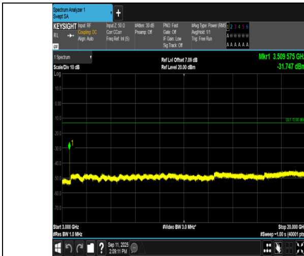
Band4-1.4MHz-16QAM-20393-1RB#5-3000~20000-PASS
