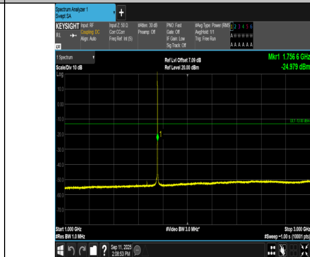
Band4-1.4MHz-16QAM-20393-1RB#5-1000~3000-PASS
