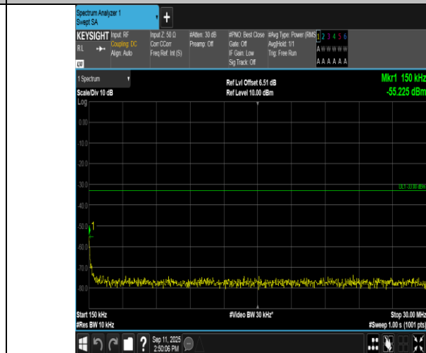
Band4-3MHz-QPSK-20175-15RB#0-0.15~30-PASS
