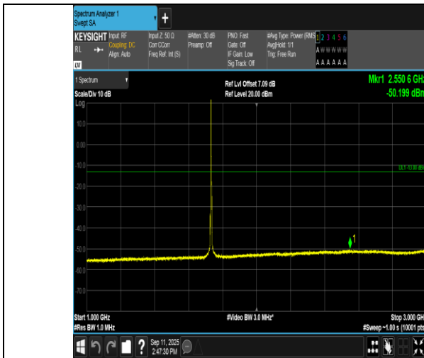
Band4-3MHz-16QAM-20175-1RB#0-1000~3000-PASS
