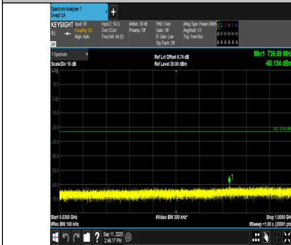
Band4-3MHz-QPSK-20175-1RB#0-30~1000-PASS
