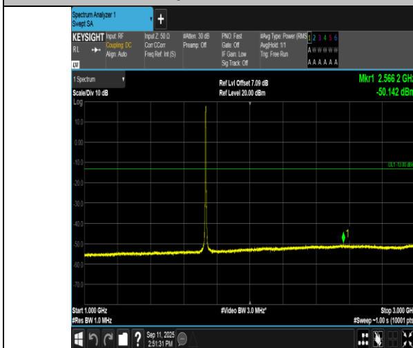
Band4-3MHz-16QAM-20175-15RB#0-1000~3000-PASS
