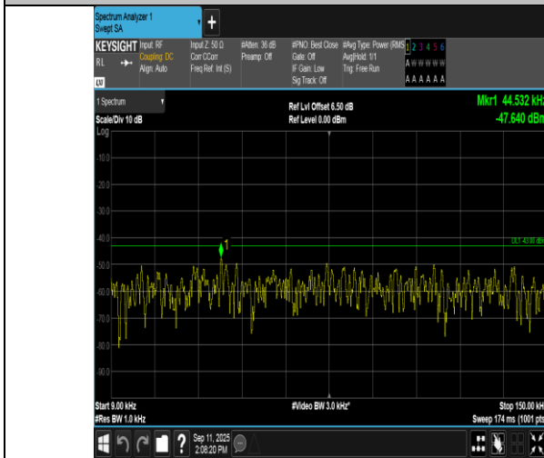
Band4-1.4MHz-16QAM-20393-1RB#5-0.009~0.15-PASS
