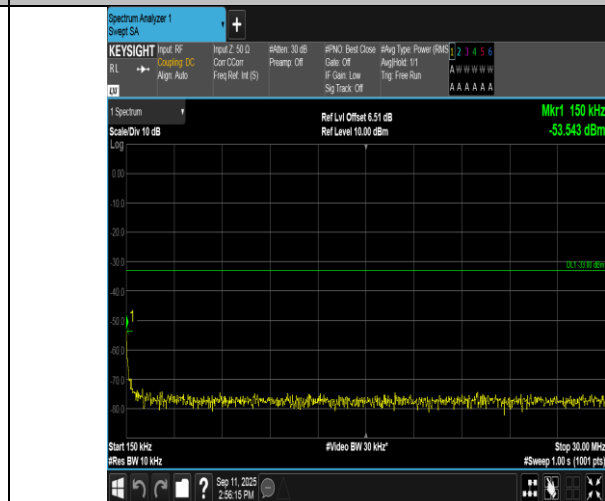
Band4-3MHz-QPSK-20385-15RB#0-0.15~30-PASS
