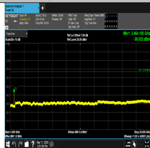
Band4-3MHz-16QAM-20175-15RB#0-3000~20000-PASS
