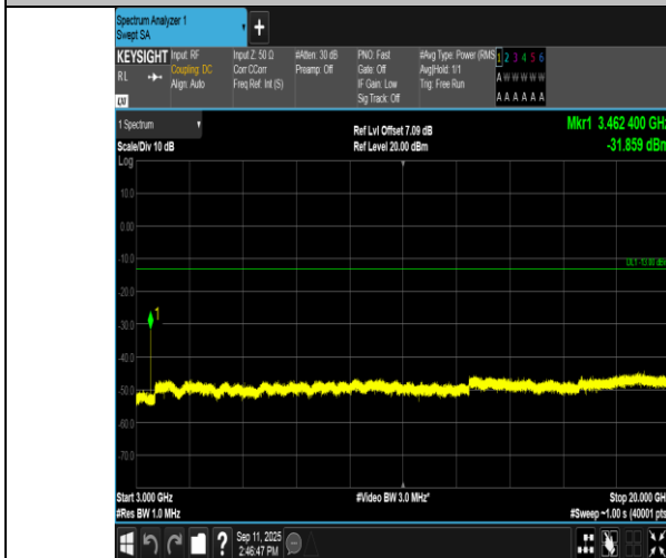
Band4-3MHz-QPSK-20175-1RB#0-3000~20000-PASS
