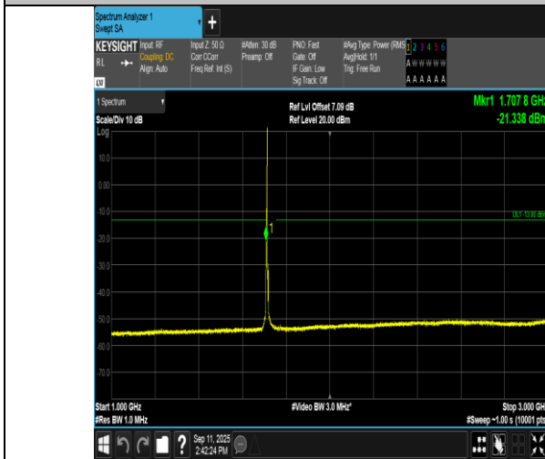
Band4-3MHz-QPSK-19965-1RB#14-1000~3000-PASS
