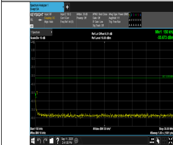
Band4-3MHz-16QAM-19965-1RB#0-0.15~30-PASS
