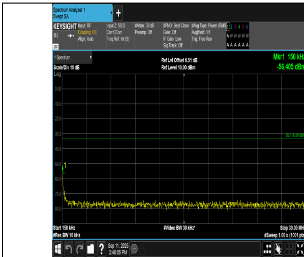
Band4-3MHz-QPSK-20175-1RB#14-0.15~30-PASS
