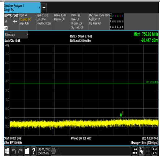
Band4-3MHz-16QAM-19965-15RB#0-30~1000-PASS
