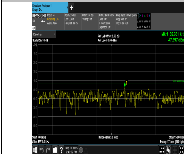
Band4-3MHz-QPSK-19965-15RB#0-0.009~0.15-PASS
