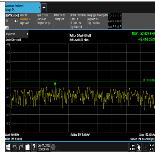
Band4-3MHz-16QAM-20175-15RB#0-0.009~0.15-PASS
