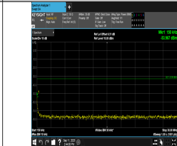
Band4-3MHz-QPSK-19965-15RB#0-0.15~30-PASS
