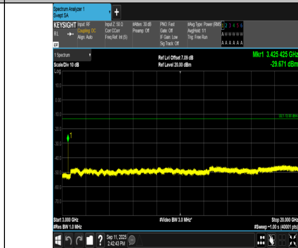
Band4-3MHz-QPSK-19965-1RB#14-3000~20000-PASS
