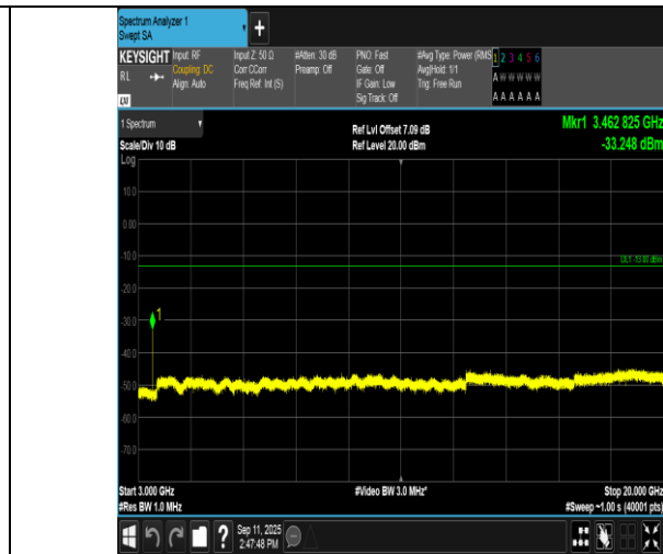
Band4-3MHz-16QAM-20175-1RB#0-3000~20000-PASS
