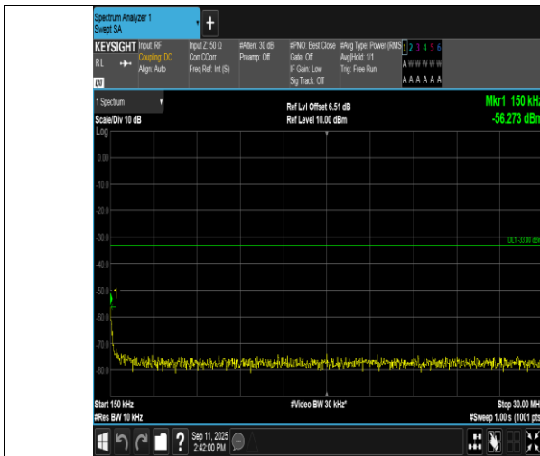
Band4-3MHz-QPSK-19965-1RB#14-0.15~30-PASS
