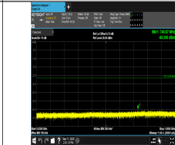
Band4-3MHz-16QAM-19965-1RB#0-30~1000-PASS
