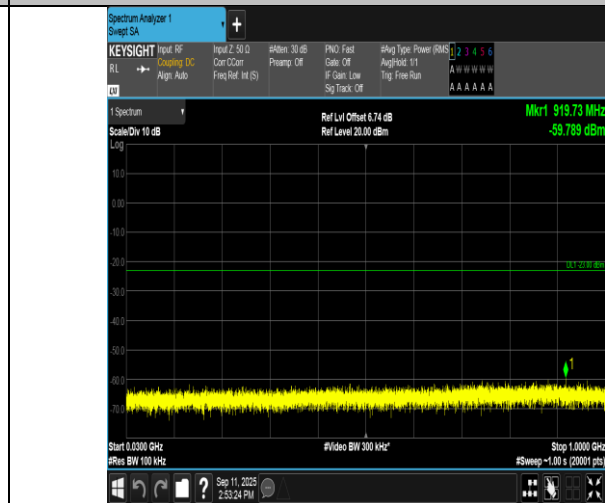
Band4-3MHz-16QAM-20385-1RB#0-30~1000-PASS
