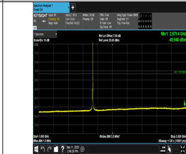
Band4-3MHz-QPSK-20175-1RB#0-1000~3000-PASS
