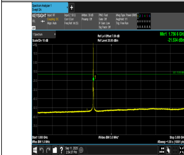
Band4-3MHz-QPSK-20385-1RB#14-1000~3000-PASS
