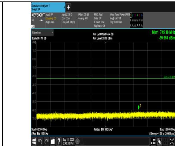
Band4-3MHz-QPSK-20175-1RB#14-30~1000-PASS
