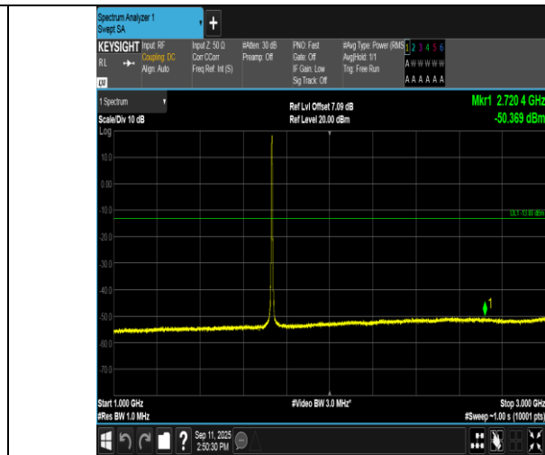
Band4-3MHz-QPSK-20175-15RB#0-1000~3000-PASS
