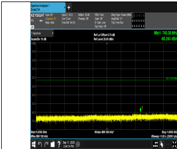
Band4-3MHz-QPSK-19965-15RB#0-30~1000-PASS
