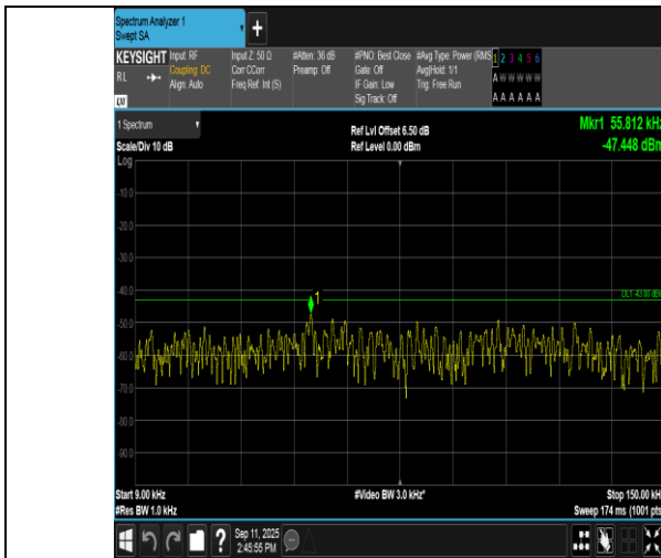
Band4-3MHz-QPSK-20175-1RB#0-0.009~0.15-PASS
