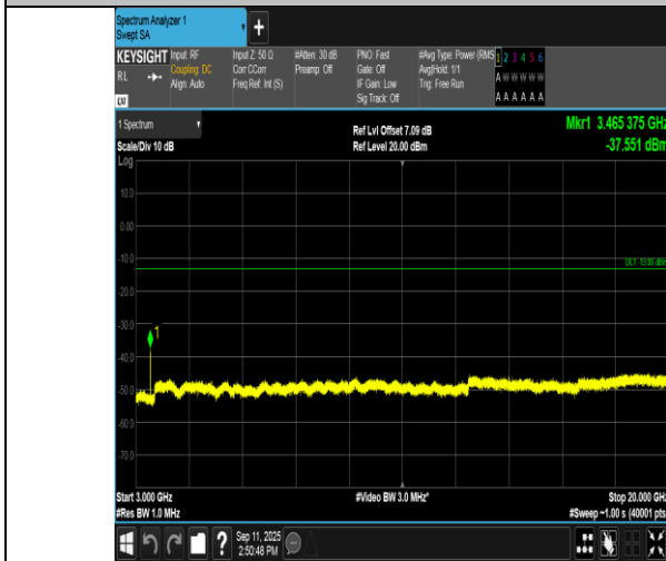
Band4-3MHz-QPSK-20175-15RB#0-3000~20000-PASS
