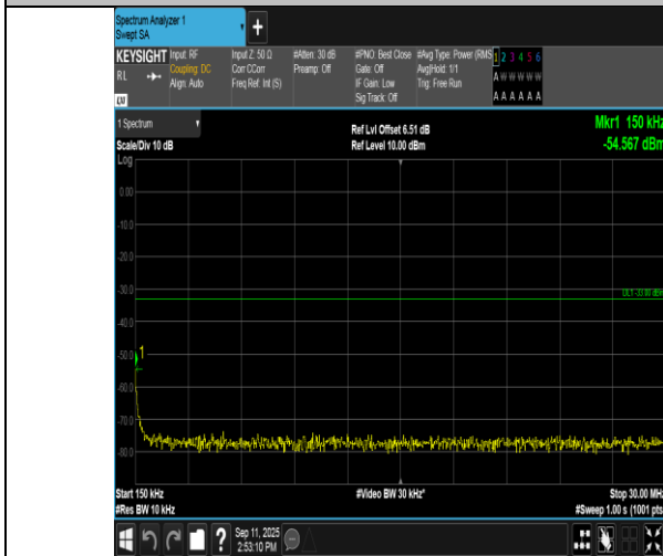
Band4-3MHz-16QAM-20385-1RB#0-0.15~30-PASS
