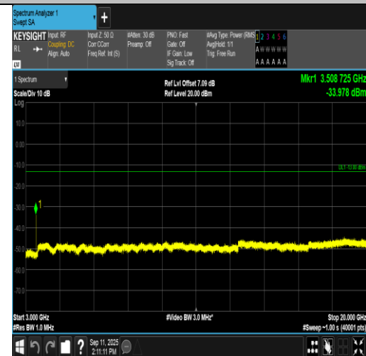
Band4-1.4MHz-16QAM-20393-6RB#0-3000~20000-PASS
