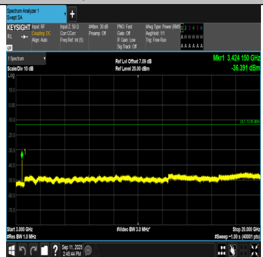
Band4-3MHz-16QAM-19965-15RB#0-3000~20000-PASS
