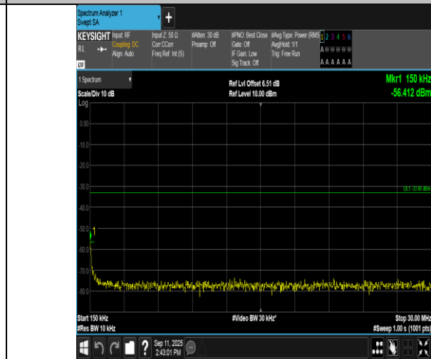
Band4-3MHz-16QAM-19965-1RB#14-0.15~30-PASS
