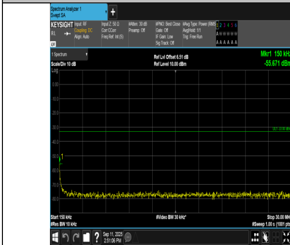
Band4-3MHz-16QAM-20175-15RB#0-0.15~30-PASS
