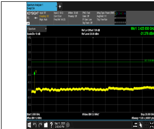
Band4-3MHz-16QAM-19965-1RB#14-3000~20000-PASS
