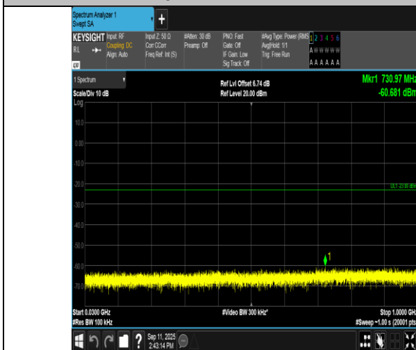
Band4-3MHz-16QAM-19965-1RB#14-30~1000-PASS
