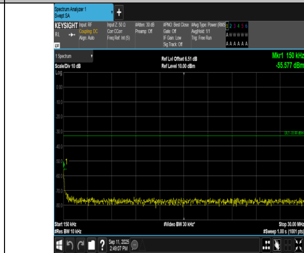
Band4-3MHz-16QAM-20175-1RB#14-0.15~30-PASS
