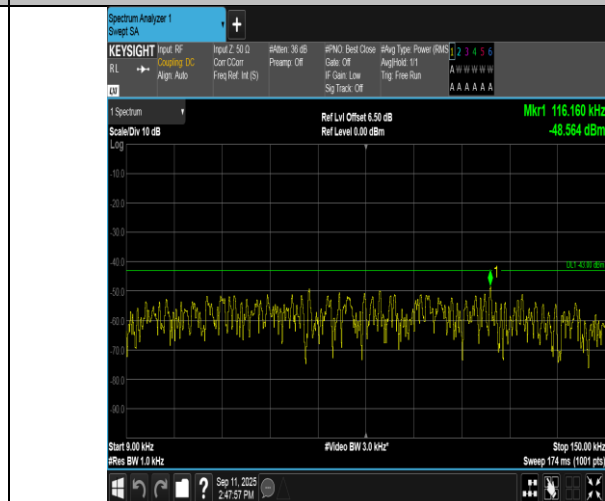
Band4-3MHz-QPSK-20175-1RB#14-0.009~0.15-PASS
