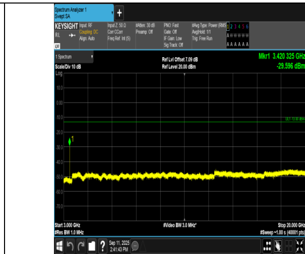
Band4-3MHz-16QAM-19965-1RB#0-3000~20000-PASS
