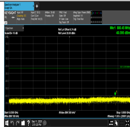
Band4-3MHz-16QAM-20175-15RB#0-30~1000-PASS
