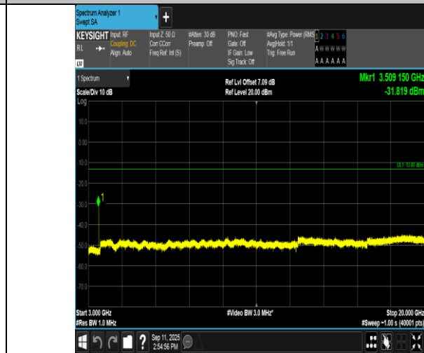
Band4-3MHz-QPSK-20385-1RB#14-3000~20000-PASS
