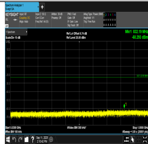
Band4-1.4MHz-16QAM-20393-6RB#0-30~1000-PASS
