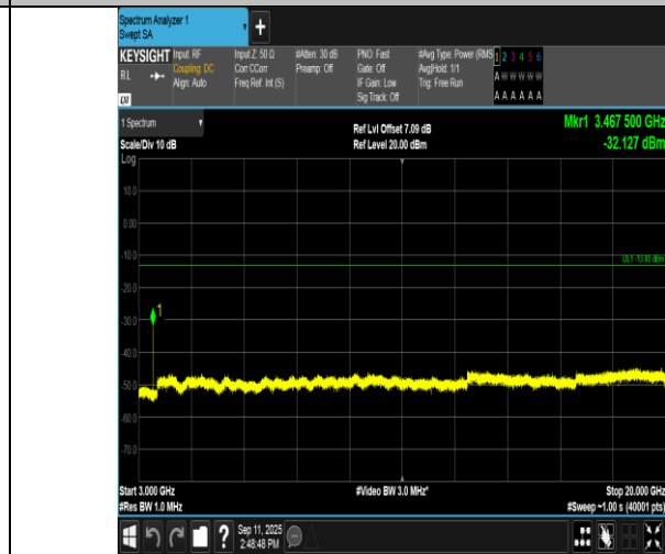
Band4-3MHz-QPSK-20175-1RB#14-3000~20000-PASS
