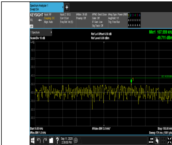
Band4-3MHz-QPSK-19965-1RB#0-0.009~0.15-PASS
