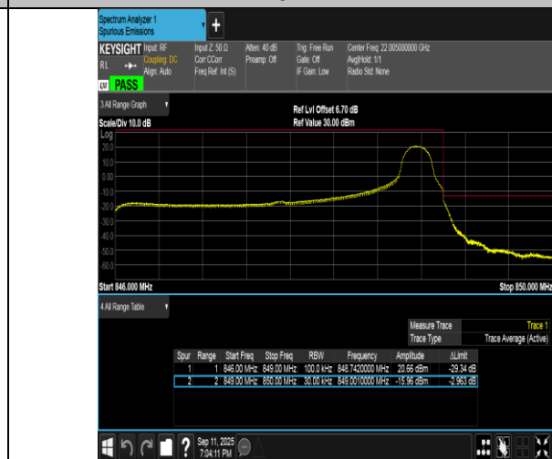
Band5-3MHz-QPSK-20635-1RB#14-PASS
