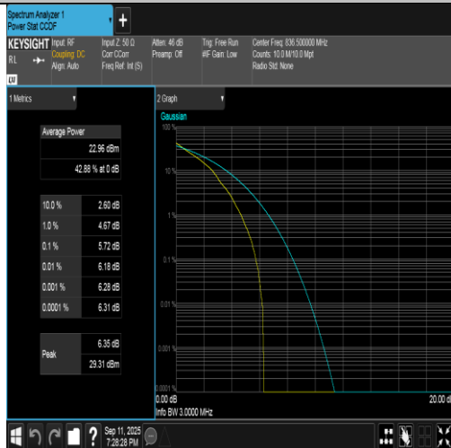
Band5-3MHz-QPSK-20525-1RB#0-PASS
