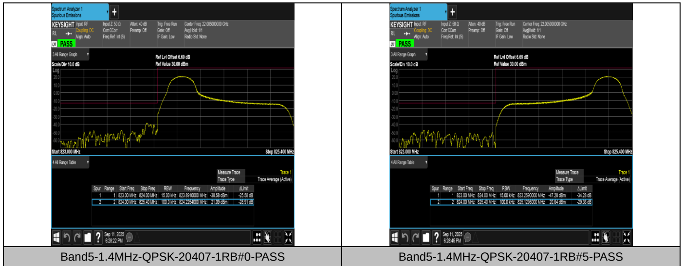
Band5-1.4MHz-QPSK-20407-1RB#0-PASS Band5-1.4MHz-QPSK-20407-1RB#5-PASS
