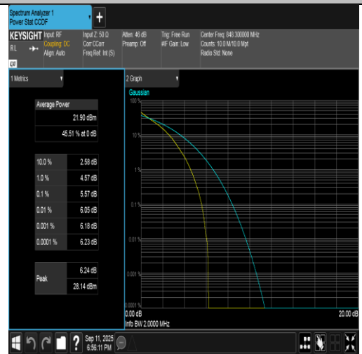
Band5-1.4MHz-QPSK-20643-6RB#0-PASS
