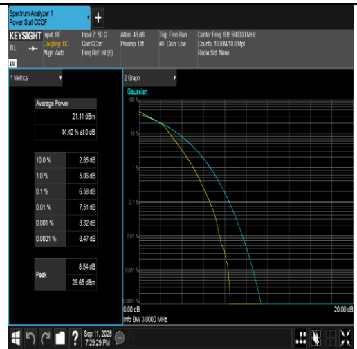
Band5-3MHz-16QAM-20525-15RB#0-PASS
