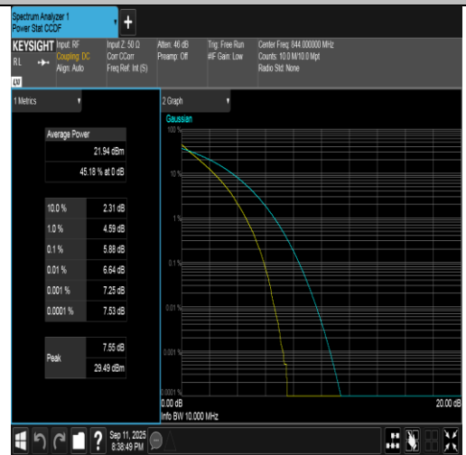
Band5-10MHz-QPSK-20600-50RB#0-PASS
