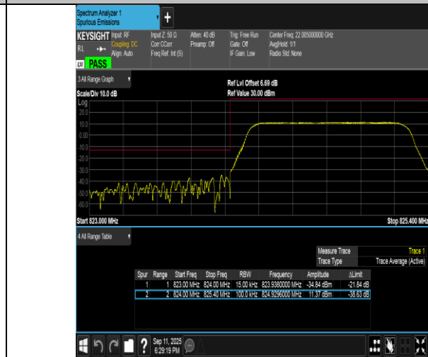
Band5-1.4MHz-16QAM-20407-6RB#0-PASS
