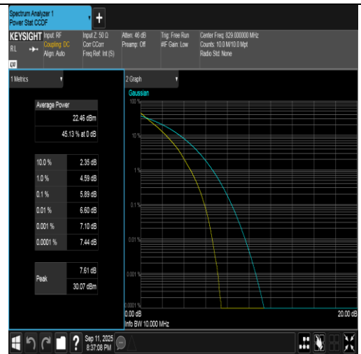
Band5-10MHz-QPSK-20450-50RB#0-PASS
