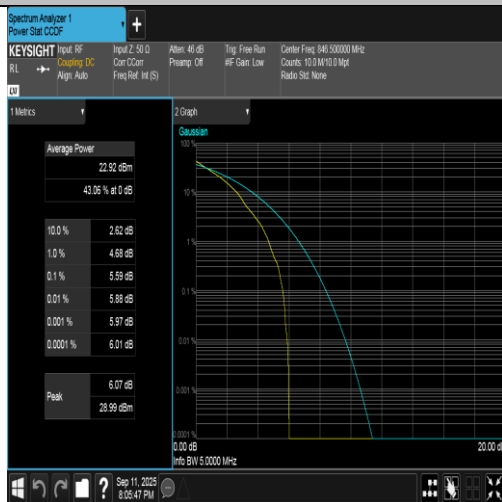
Band5-5MHz-QPSK-20625-1RB#0-PASS
