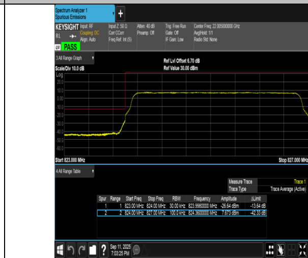
Band5-3MHz-16QAM-20415-15RB#0-PASS
