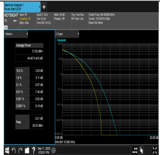
Band5-10MHz-16QAM-20600-50RB#0-PASS
