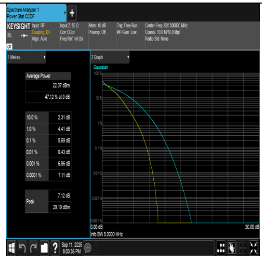
Band5-5MHz-QPSK-20425-25RB#0-PASS
