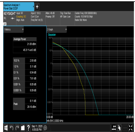
Band5-1.4MHz-16QAM-20525-6RB#0-PASS
