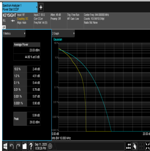
Band5-10MHz-QPSK-20600-1RB#0-PASS
