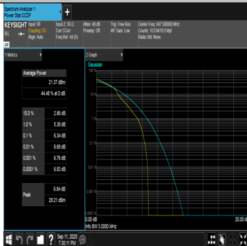
Band5-3MHz-16QAM-20635-1RB#0-PASS
