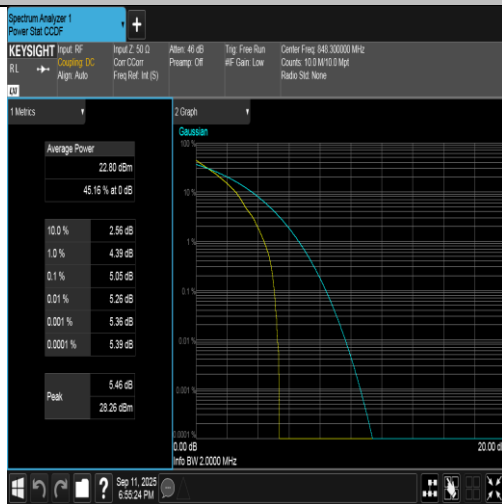
Band5-1.4MHz-QPSK-20643-1RB#0-PASS
