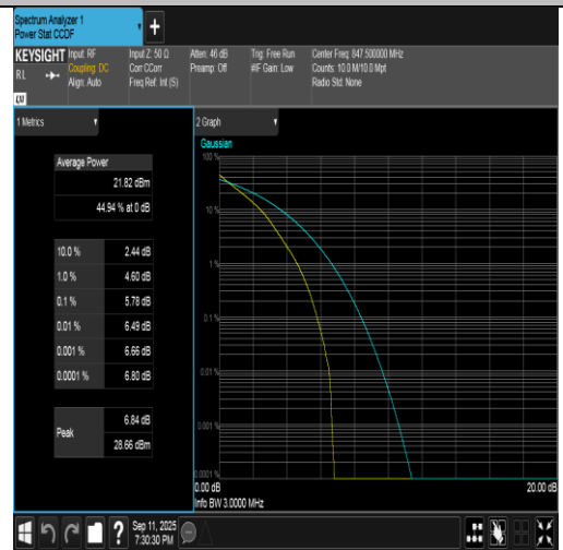
Band5-3MHz-QPSK-20635-15RB#0-PASS
