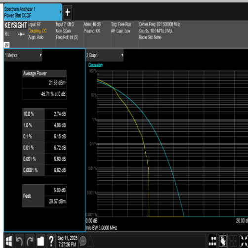
Band5-3MHz-16QAM-20415-1RB#0-PASS
