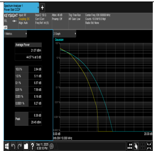
Band5-10MHz-16QAM-20525-50RB#0-PASS
