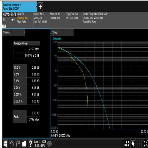
Band5-1.4MHz-16QAM-20643-1RB#0-PASS
