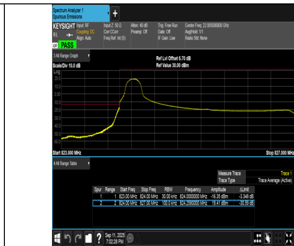
Band5-3MHz-16QAM-20415-1RB#0-PASS
