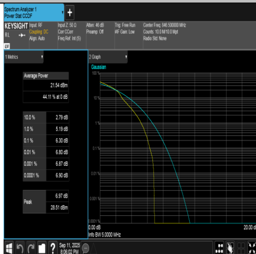
Band5-5MHz-16QAM-20625-1RB#0-PASS
