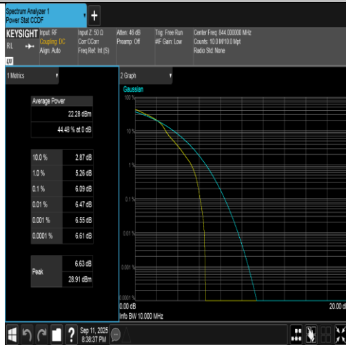
Band5-10MHz-16QAM-20600-1RB#0-PASS
