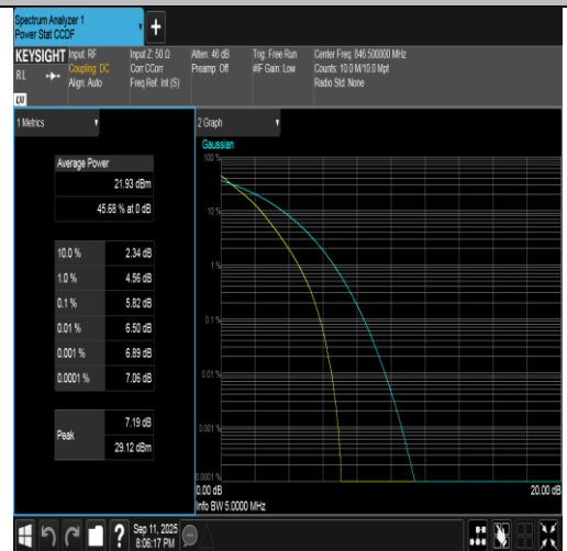
Band5-5MHz-QPSK-20625-25RB#0-PASS
