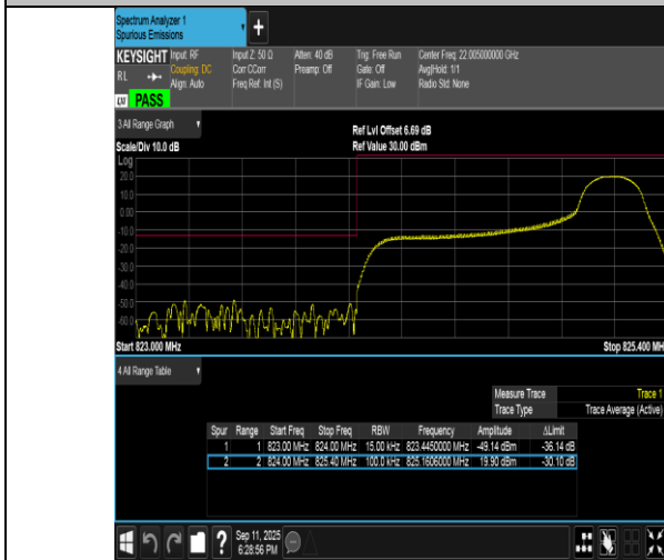
Band5-1.4MHz-16QAM-20407-1RB#5-PASS
