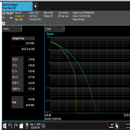
Band5-10MHz-16QAM-20450-1RB#0-PASS
