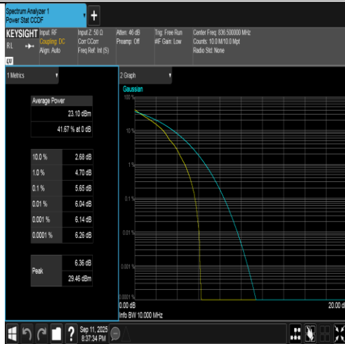
Band5-10MHz-QPSK-20525-1RB#0-PASS
