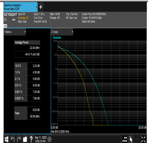
Band5-5MHz-QPSK-20525-25RB#0-PASS
