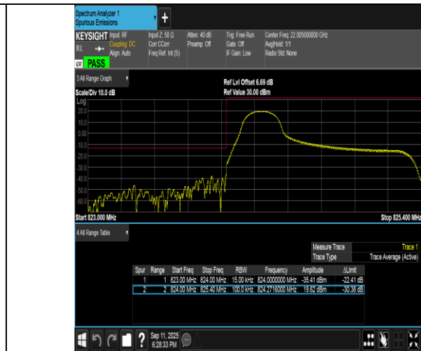
Band5-1.4MHz-16QAM-20407-1RB#0-PASS
