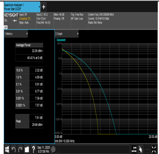
Band5-10MHz-QPSK-20525-50RB#0-PASS
