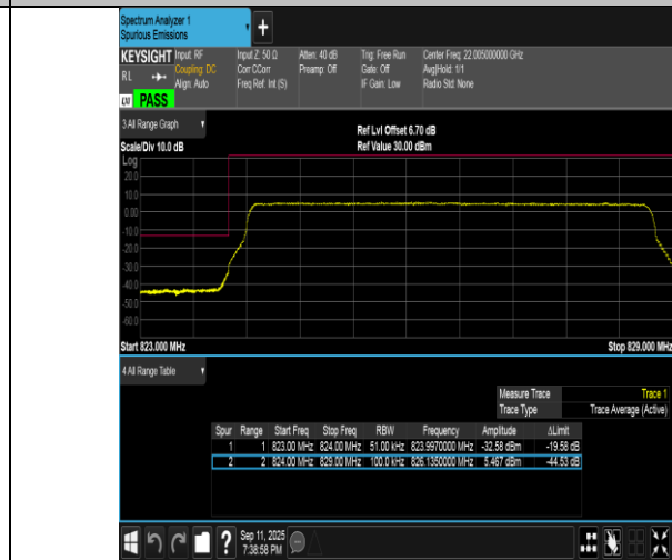
Band5-5MHz-16QAM-20425-25RB#0-PASS
