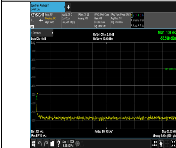
Band5-1.4MHz-QPSK-20525-1RB#5-0.15~30-PASS
