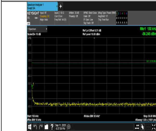
Band5-1.4MHz-16QAM-20525-1RB#0-0.15~30-PASS
