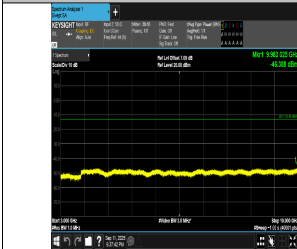
Band5-1.4MHz-QPSK-20525-1RB#0-3000~10000-PASS
