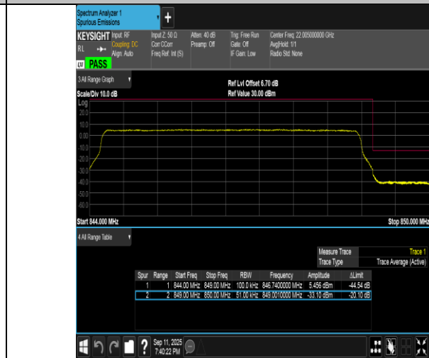
Band5-5MHz-16QAM-20625-25RB#0-PASS
