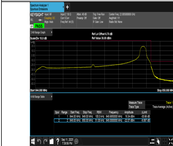
Band5-5MHz-16QAM-20625-1RB#24-PASS
