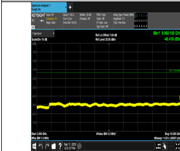
Band5-1.4MHz-QPSK-20407-1RB#0-3000~10000-PASS
