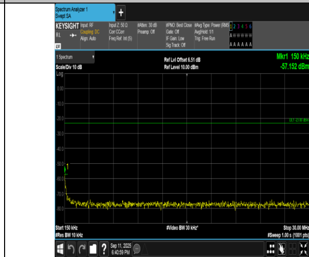
Band5-1.4MHz-QPSK-20525-6RB#0-0.15~30-PASS
