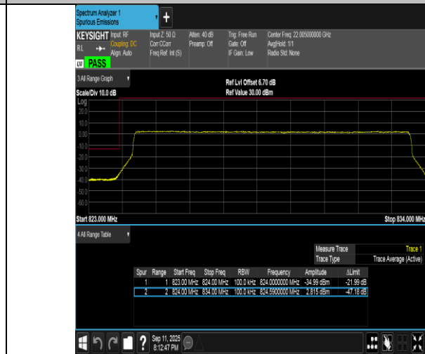
Band5-10MHz-16QAM-20450-50RB#0-PASS
