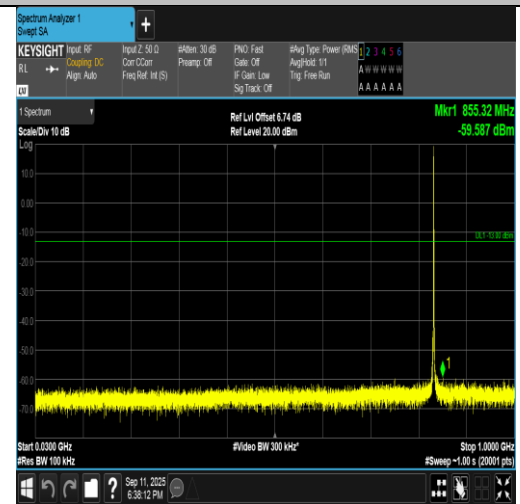
Band5-1.4MHz-16QAM-20525-1RB#0-30~1000-PASS
