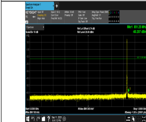
Band5-1.4MHz-QPSK-20525-6RB#0-30~1000-PASS
