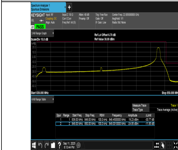
Band5-10MHz-16QAM-20600-1RB#49-PASS
