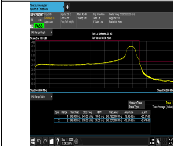
Band5-3MHz-16QAM-20635-1RB#14-PASS
