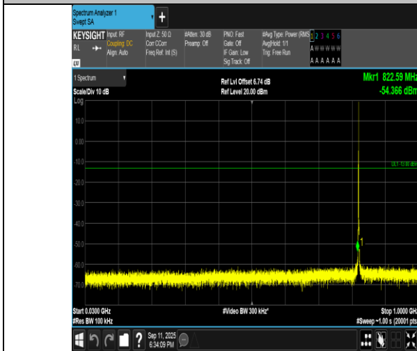
Band5-1.4MHz-16QAM-20407-1RB#5-30~1000-PASS
