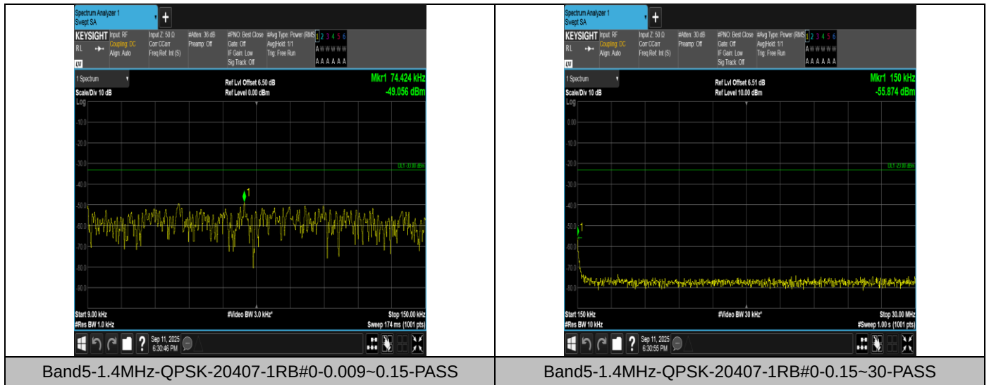
Band5-1.4MHz-QPSK-20407-1RB#0-0.009~0.15-PASS Band5-1.4MHz-QPSK-20407-1RB#0-0.15~30-PASS
