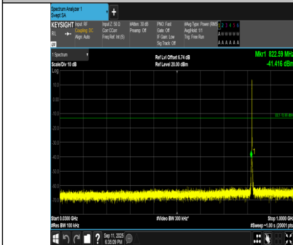
Band5-1.4MHz-QPSK-20407-6RB#0-30~1000-PASS
