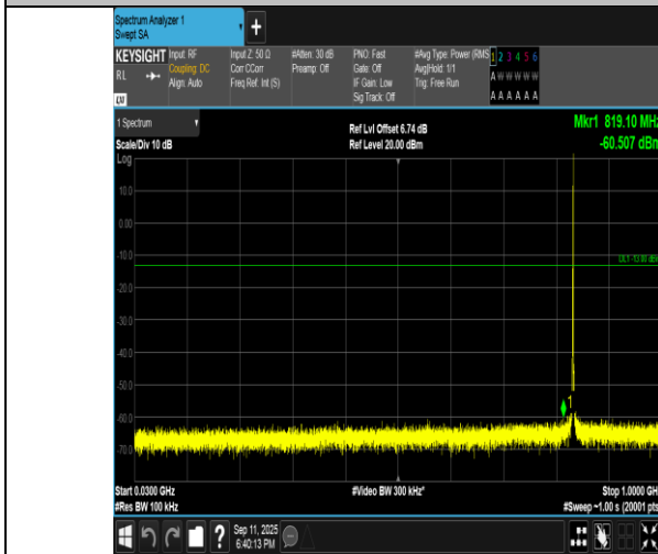
Band5-1.4MHz-16QAM-20525-1RB#5-30~1000-PASS
