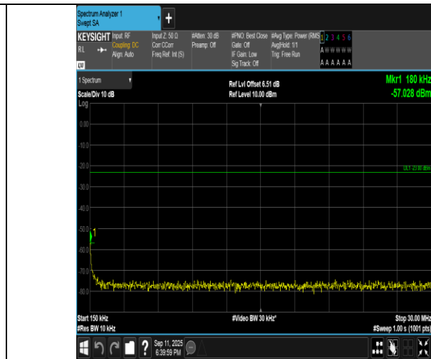
Band5-1.4MHz-16QAM-20525-1RB#5-0.15~30-PASS
