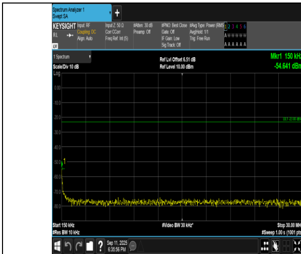
Band5-1.4MHz-16QAM-20407-6RB#0-0.15~30-PASS
