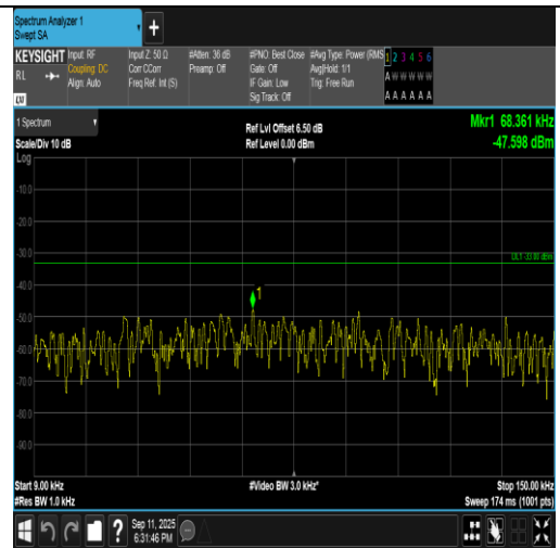
Band5-1.4MHz-16QAM-20407-1RB#0-0.009~0.15-PASS
