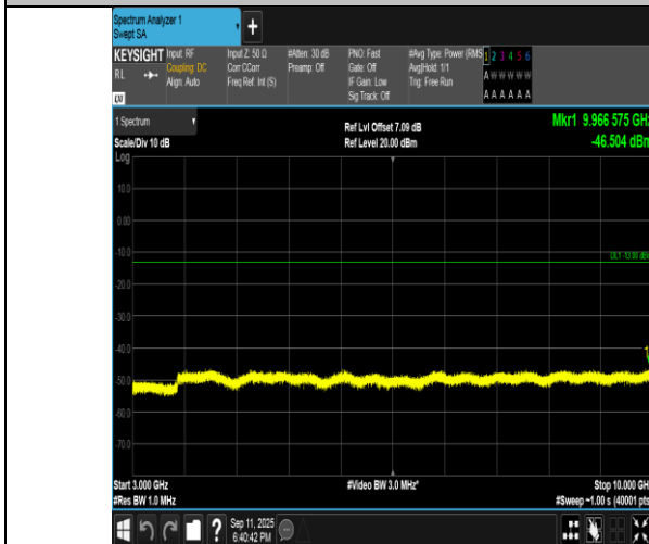
Band5-1.4MHz-16QAM-20525-1RB#5-3000~10000-PASS
