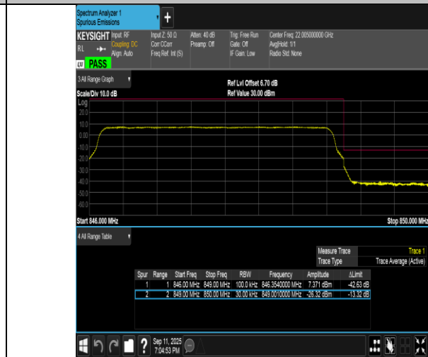
Band5-3MHz-16QAM-20635-15RB#0-PASS
