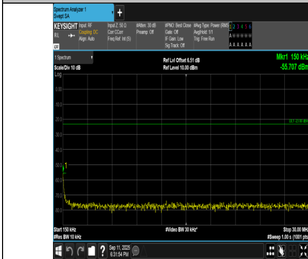
Band5-1.4MHz-16QAM-20407-1RB#0-0.15~30-PASS
