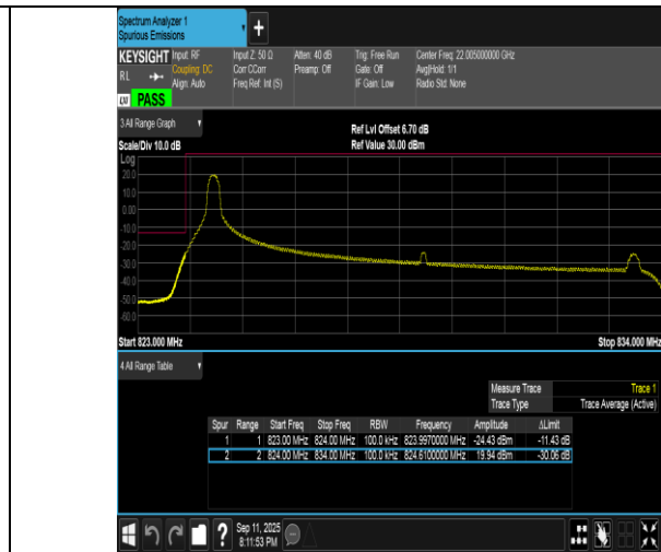
Band5-10MHz-16QAM-20450-1RB#0-PASS
