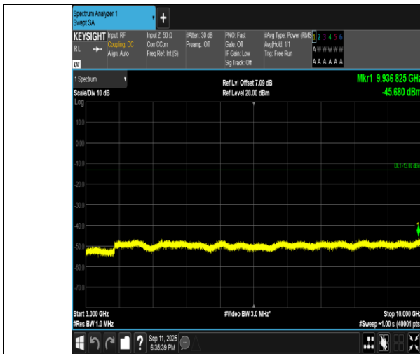
Band5-1.4MHz-QPSK-20407-6RB#0-3000~10000-PASS
