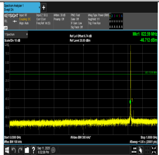
Band5-1.4MHz-16QAM-20407-1RB#0-30~1000-PASS
