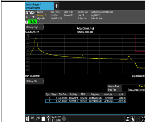
Band5-10MHz-QPSK-20600-1RB#0-PASS
