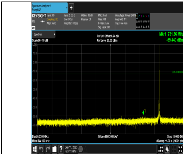
Band5-1.4MHz-QPSK-20525-1RB#0-30~1000-PASS
