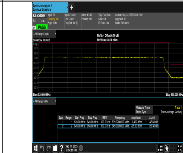
Band5-10MHz-16QAM-20600-50RB#0-PASS
