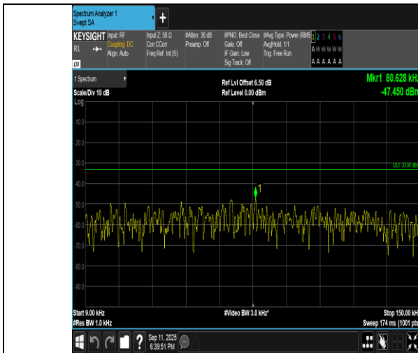
Band5-1.4MHz-16QAM-20525-1RB#5-0.009~0.15-PASS
