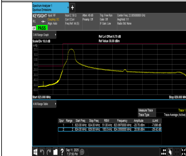
Band5-5MHz-QPSK-20425-1RB#0-PASS
