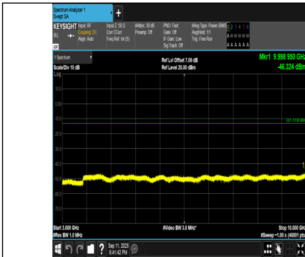
Band5-1.4MHz-QPSK-20525-6RB#0-3000~10000-PASS
