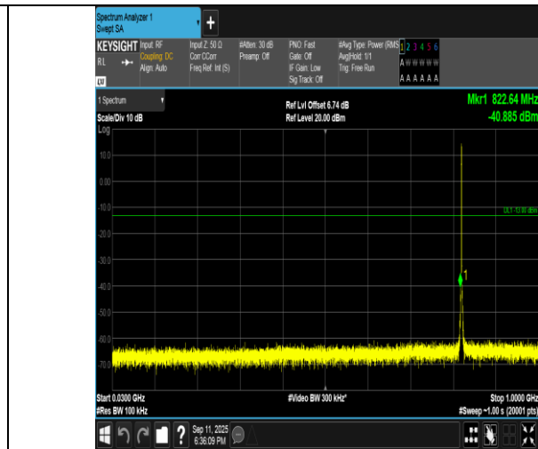
Band5-1.4MHz-16QAM-20407-6RB#0-30~1000-PASS
