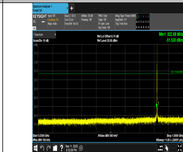
Band5-1.4MHz-QPSK-20407-1RB#5-30~1000-PASS
