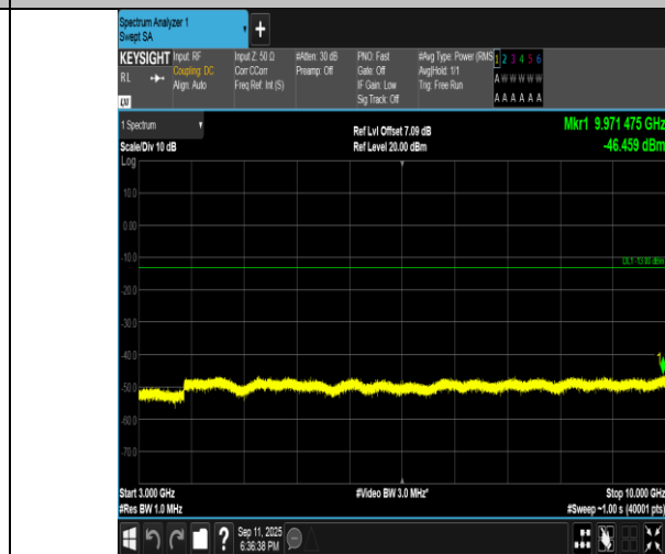
Band5-1.4MHz-16QAM-20407-6RB#0-3000~10000-PASS
