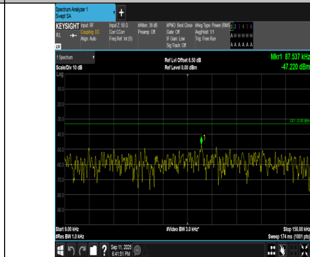
Band5-1.4MHz-16QAM-20525-6RB#0-0.009~0.15-PASS
