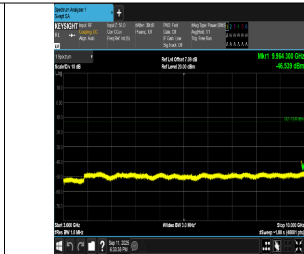
Band5-1.4MHz-QPSK-20407-1RB#5-3000~10000-PASS
