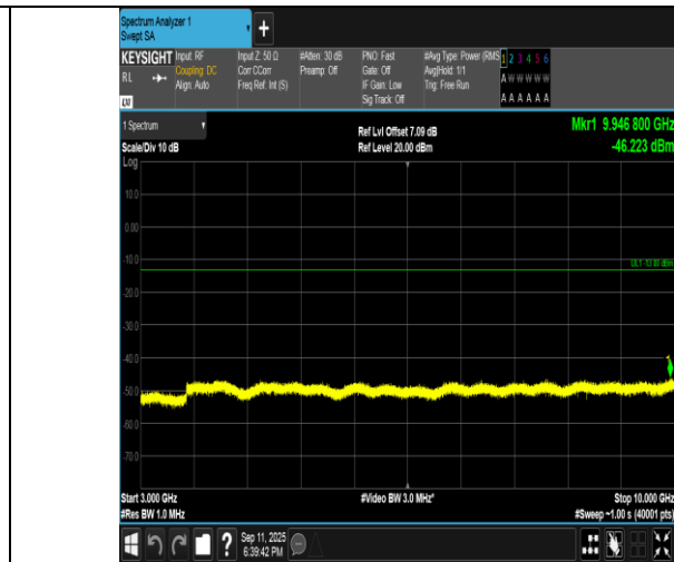
Band5-1.4MHz-QPSK-20525-1RB#5-3000~10000-PASS
