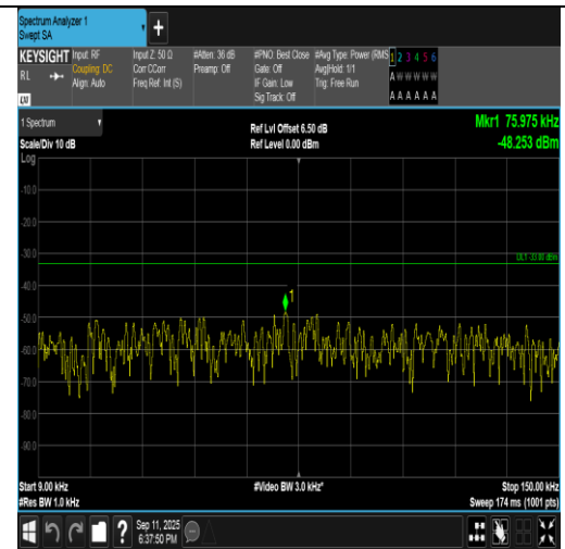
Band5-1.4MHz-16QAM-20525-1RB#0-0.009~0.15-PASS
