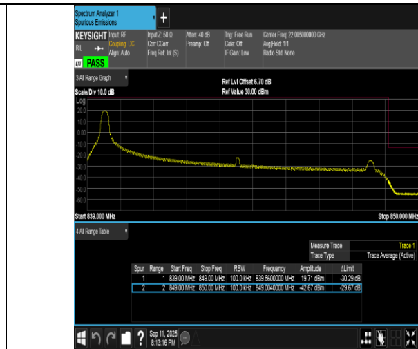
Band5-10MHz-16QAM-20600-1RB#0-PASS
