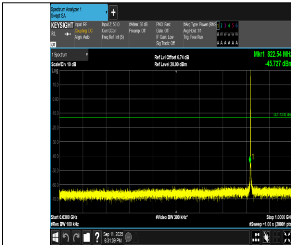
Band5-1.4MHz-QPSK-20407-1RB#0-30~1000-PASS
