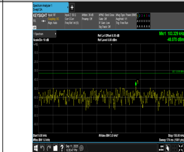
Band5-1.4MHz-16QAM-20407-6RB#0-0.009~0.15-PASS
