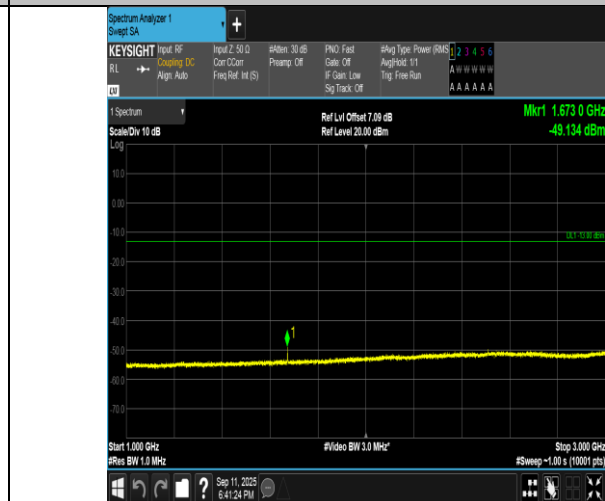
Band5-1.4MHz-QPSK-20525-6RB#0-1000~3000-PASS
