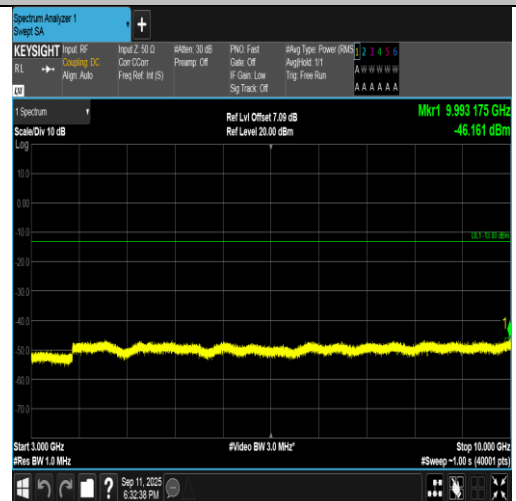
Band5-1.4MHz-16QAM-20407-1RB#0-3000~10000-PASS
