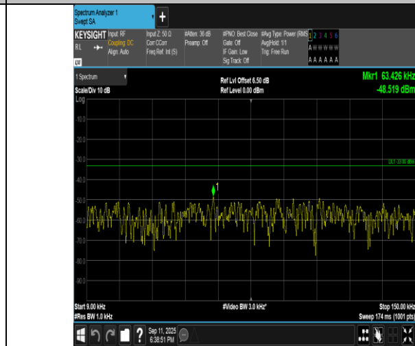
Band5-1.4MHz-QPSK-20525-1RB#5-0.009~0.15-PASS
