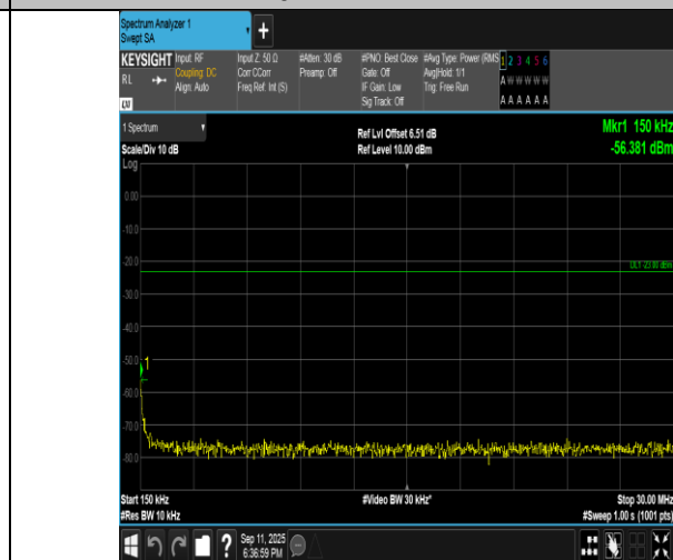
Band5-1.4MHz-QPSK-20525-1RB#0-0.15~30-PASS
