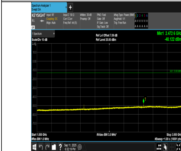
Band5-1.4MHz-16QAM-20407-1RB#0-1000~3000-PASS
