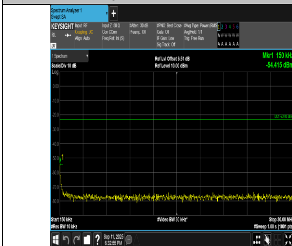
Band5-1.4MHz-QPSK-20407-1RB#5-0.15~30-PASS
