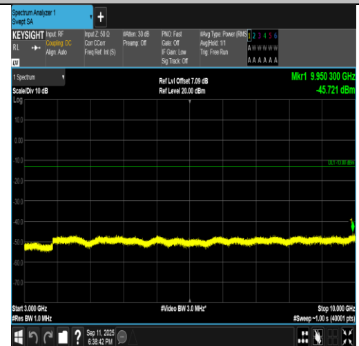
Band5-1.4MHz-16QAM-20525-1RB#0-3000~10000-PASS
