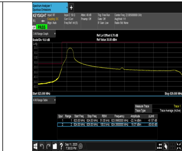
Band5-5MHz-16QAM-20425-1RB#0-PASS
