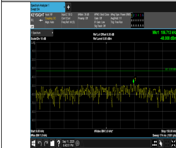
Band5-1.4MHz-QPSK-20525-6RB#0-0.009~0.15-PASS
