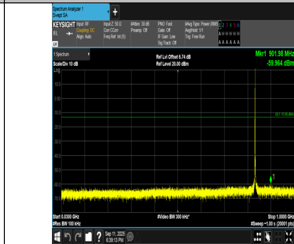
Band5-1.4MHz-QPSK-20525-1RB#5-30~1000-PASS
