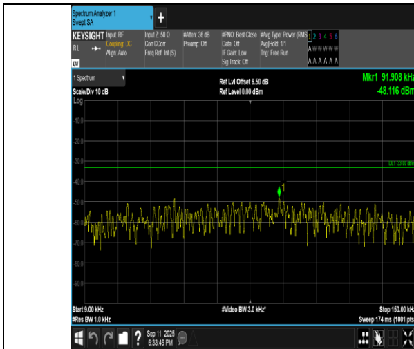
Band5-1.4MHz-16QAM-20407-1RB#5-0.009~0.15-PASS
