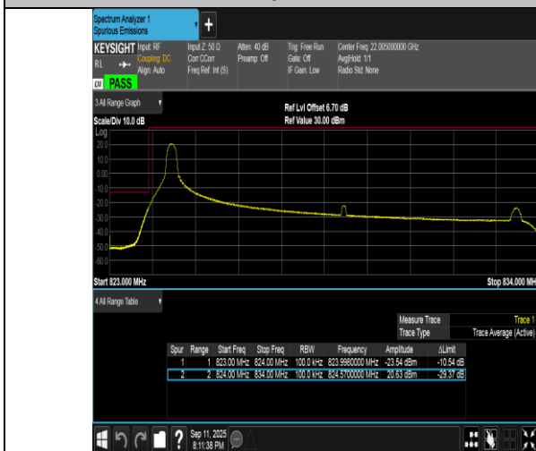
Band5-10MHz-QPSK-20450-1RB#0-PASS
