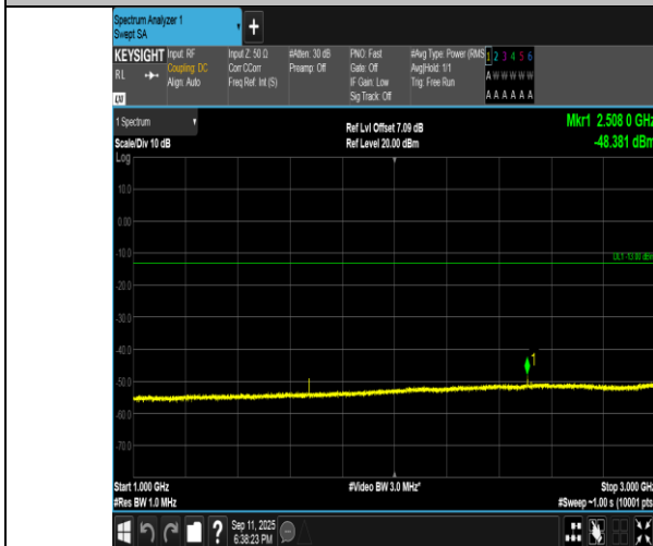
Band5-1.4MHz-16QAM-20525-1RB#0-1000~3000-PASS
