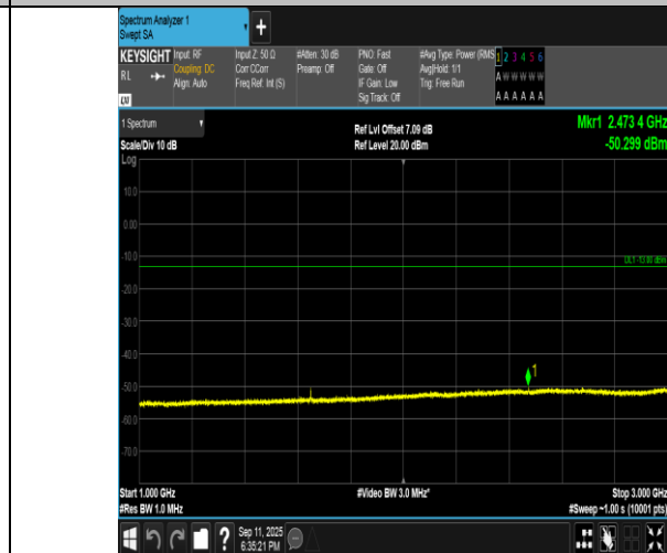
Band5-1.4MHz-QPSK-20407-6RB#0-1000~3000-PASS
