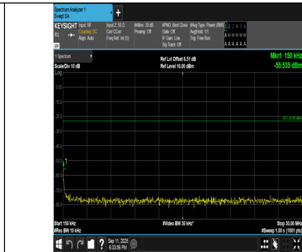
Band5-1.4MHz-16QAM-20407-1RB#5-0.15~30-PASS
