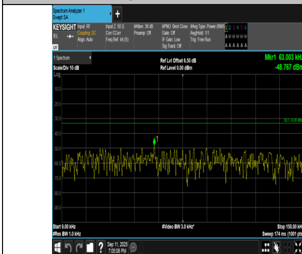
Band5-3MHz-QPSK-20415-1RB#0-0.009~0.15-PASS
