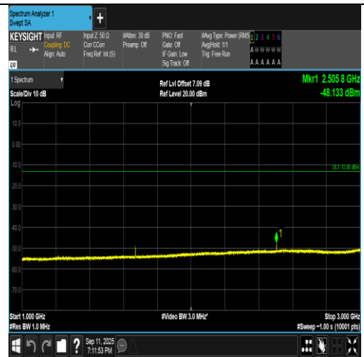
Band5-3MHz-QPSK-20525-1RB#0-1000~3000-PASS
