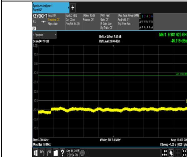
Band5-3MHz-16QAM-20415-1RB#14-3000~10000-PASS
