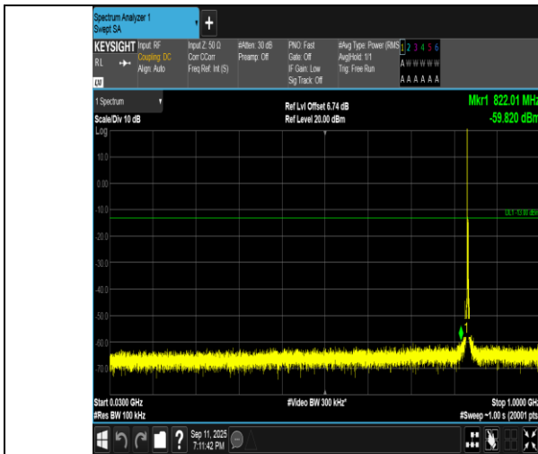
Band5-3MHz-QPSK-20525-1RB#0-30~1000-PASS
