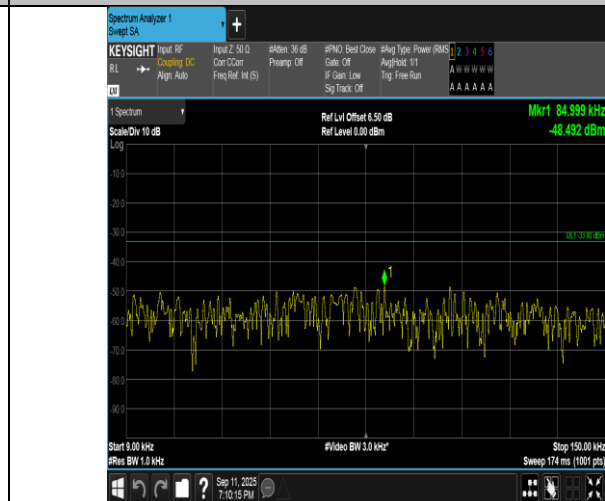
Band5-3MHz-16QAM-20415-15RB#0-0.009~0.15-PASS
