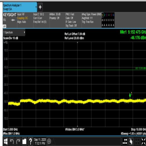
Band5-3MHz-QPSK-20525-1RB#0-3000~10000-PASS
