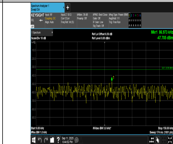
Band5-1.4MHz-QPSK-20643-1RB#5-0.009~0.15-PASS
