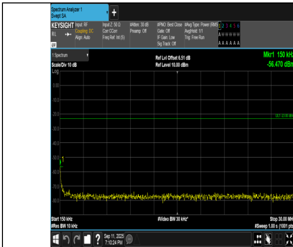
Band5-3MHz-16QAM-20415-15RB#0-0.15~30-PASS
