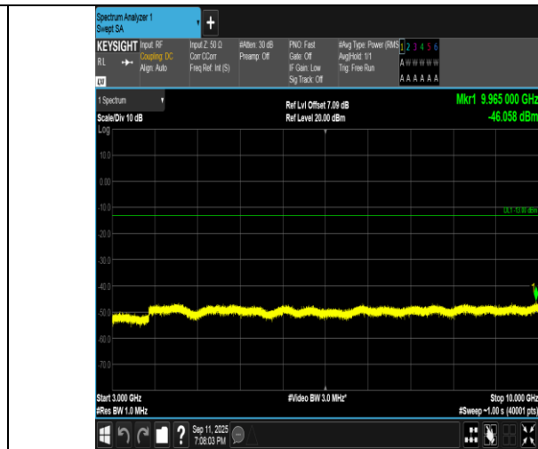
Band5-3MHz-QPSK-20415-1RB#14-3000~10000-PASS
