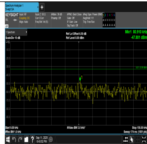
Band5-1.4MHz-16QAM-20643-1RB#0-0.009~0.15-PASS
