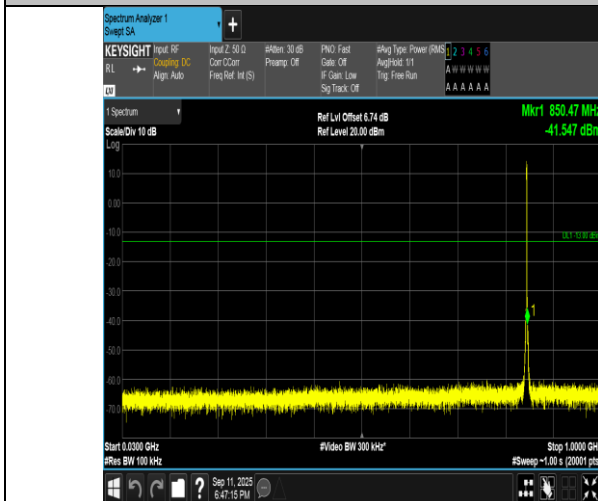
Band5-1.4MHz-QPSK-20643-6RB#0-30~1000-PASS
