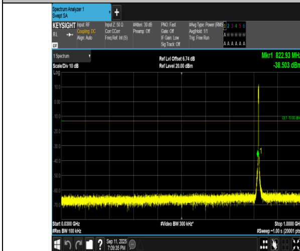
Band5-3MHz-QPSK-20415-15RB#0-30~1000-PASS
