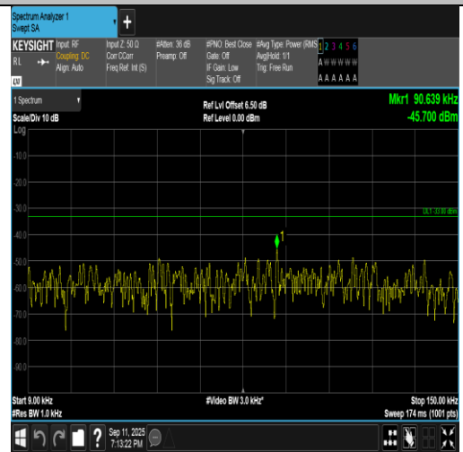
Band5-3MHz-QPSK-20525-1RB#14-0.009~0.15-PASS
