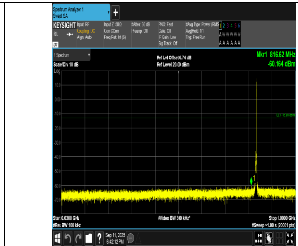
Band5-1.4MHz-16QAM-20525-6RB#0-30~1000-PASS
