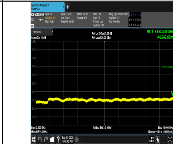
Band5-1.4MHz-16QAM-20643-6RB#0-3000~10000-PASS
