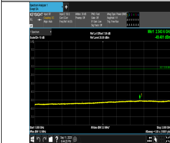
Band5-1.4MHz-16QAM-20643-1RB#0-1000~3000-PASS
