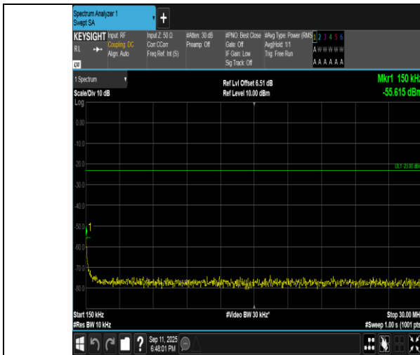
Band5-1.4MHz-16QAM-20643-6RB#0-0.15~30-PASS
