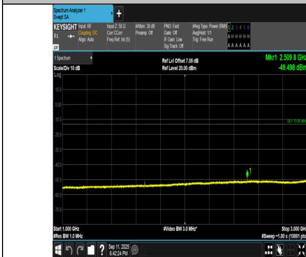
Band5-1.4MHz-16QAM-20525-6RB#0-1000~3000-PASS
