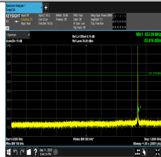
Band5-1.4MHz-16QAM-20643-1RB#0-30~1000-PASS
