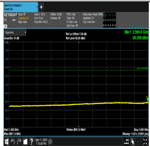
Band5-3MHz-QPSK-20525-15RB#0-1000~3000-PASS
