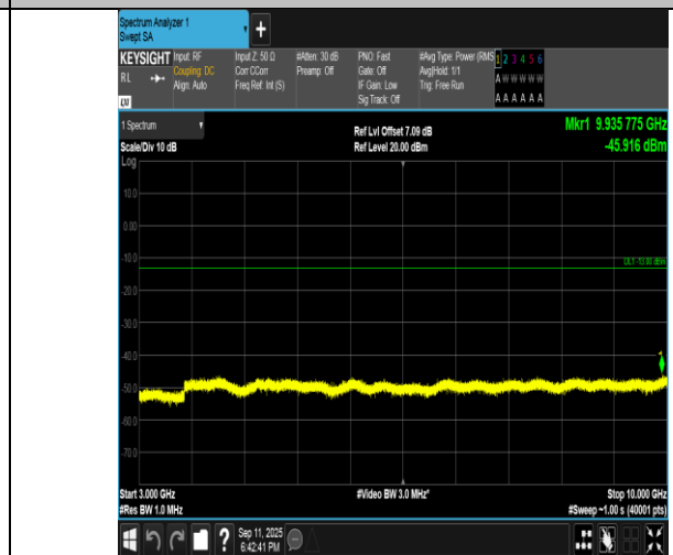
Band5-1.4MHz-16QAM-20525-6RB#0-3000~10000-PASS
