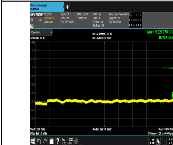
Band5-3MHz-16QAM-20525-1RB#14-3000~10000-PASS
