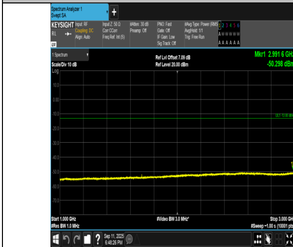
Band5-1.4MHz-16QAM-20643-6RB#0-1000~3000-PASS
