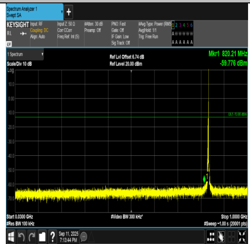
Band5-3MHz-QPSK-20525-1RB#14-30~1000-PASS
