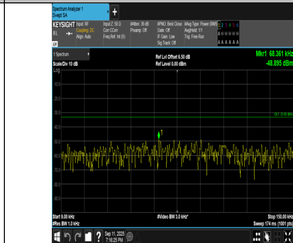
Band5-3MHz-16QAM-20525-15RB#0-0.009~0.15-PASS
