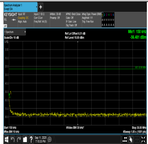
Band5-3MHz-QPSK-20525-15RB#0-0.15~30-PASS
