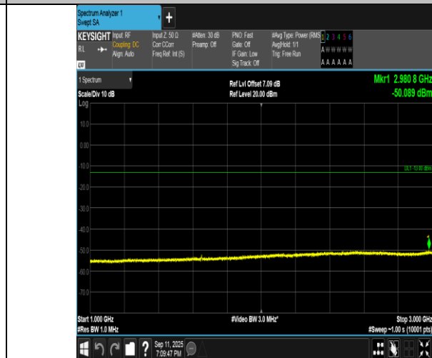
Band5-3MHz-QPSK-20415-15RB#0-1000~3000-PASS
