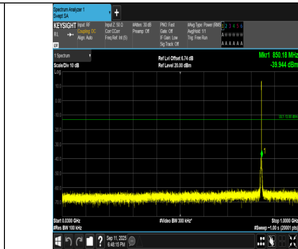
Band5-1.4MHz-16QAM-20643-6RB#0-30~1000-PASS
