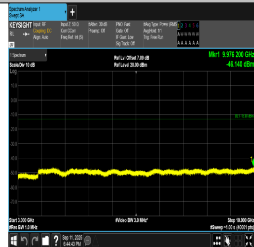
Band5-1.4MHz-16QAM-20643-1RB#0-3000~10000-PASS
