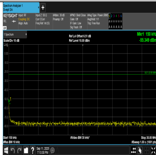
Band5-3MHz-QPSK-20525-1RB#14-0.15~30-PASS
