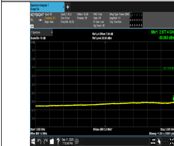
Band5-3MHz-16QAM-20415-15RB#0-1000~3000-PASS
