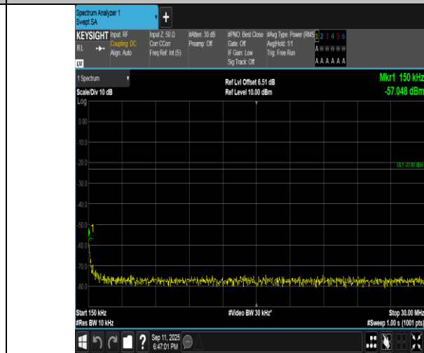
Band5-1.4MHz-QPSK-20643-6RB#0-0.15~30-PASS
