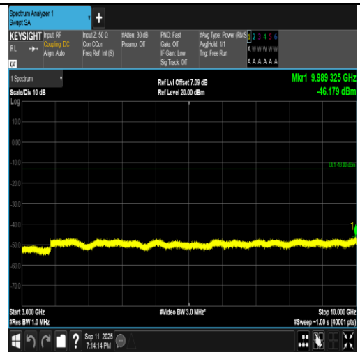
Band5-3MHz-QPSK-20525-1RB#14-3000~10000-PASS
