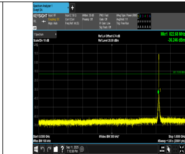
Band5-3MHz-16QAM-20415-15RB#0-30~1000-PASS
