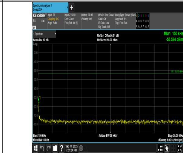
Band5-5MHz-QPSK-20525-25RB#0-0.15~30-PASS
