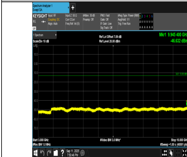
Band5-5MHz-16QAM-20525-1RB#24-3000~10000-PASS
