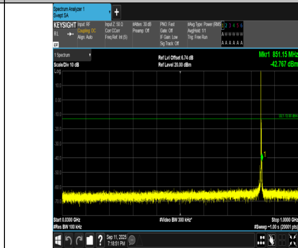
Band5-3MHz-16QAM-20635-1RB#0-30~1000-PASS
