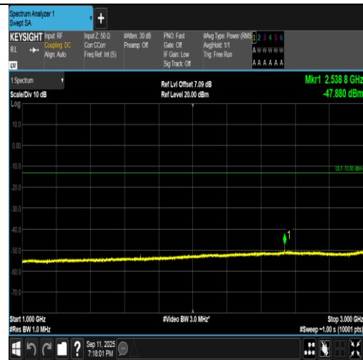
Band5-3MHz-QPSK-20635-1RB#0-1000~3000-PASS
