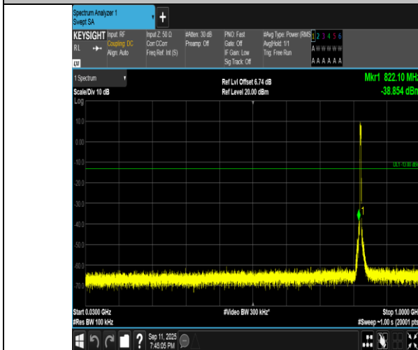
Band5-5MHz-QPSK-20425-25RB#0-30~1000-PASS
