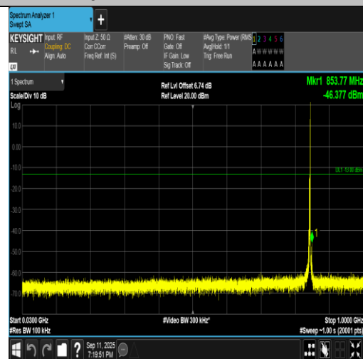
Band5-3MHz-QPSK-20635-1RB#14-30~1000-PASS
