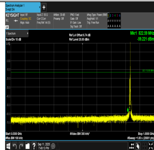
Band5-5MHz-QPSK-20525-1RB#24-30~1000-PASS
