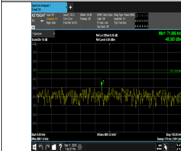
Band5-5MHz-QPSK-20425-1RB#0-0.009~0.15-PASS
