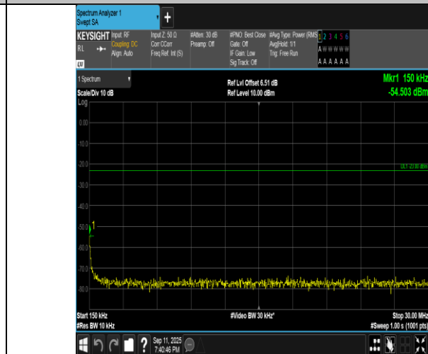
Band5-5MHz-QPSK-20425-1RB#0-0.15~30-PASS
