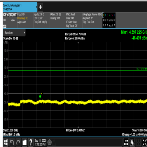
Band5-3MHz-QPSK-20635-1RB#0-3000~10000-PASS
