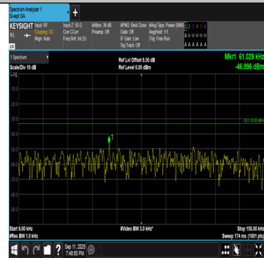
Band5-5MHz-QPSK-20525-1RB#24-0.009~0.15-PASS
