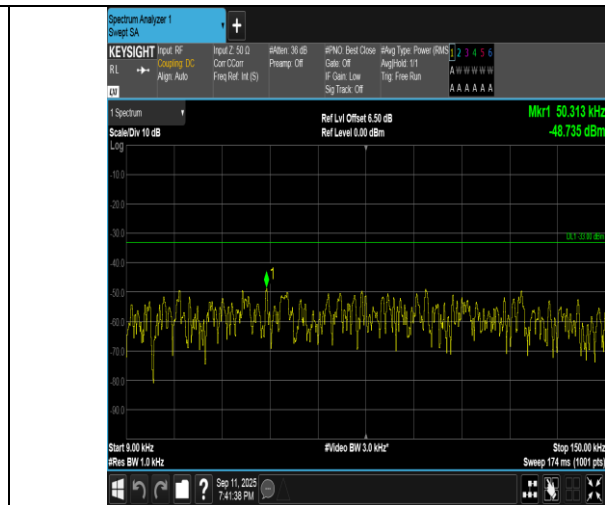
Band5-5MHz-16QAM-20425-1RB#0-0.009~0.15-PASS
