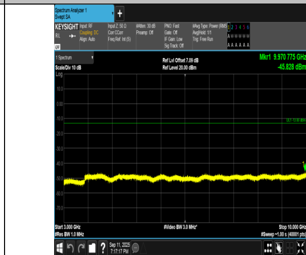
Band5-3MHz-16QAM-20525-15RB#0-3000~10000-PASS
