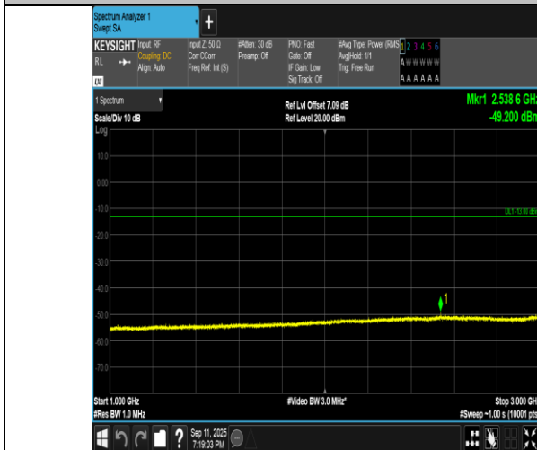
Band5-3MHz-16QAM-20635-1RB#0-1000~3000-PASS
