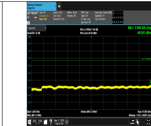
Band5-5MHz-QPSK-20525-1RB#24-3000~10000-PASS
