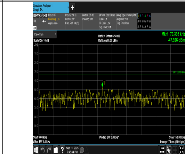
Band5-5MHz-16QAM-20425-25RB#0-0.009~0.15-PASS
