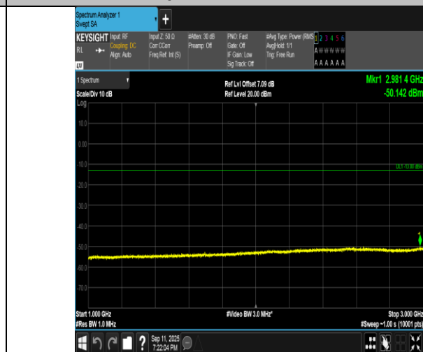
Band5-3MHz-QPSK-20635-15RB#0-1000~3000-PASS
