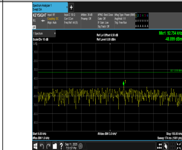
Band5-5MHz-16QAM-20525-25RB#0-0.009~0.15-PASS
