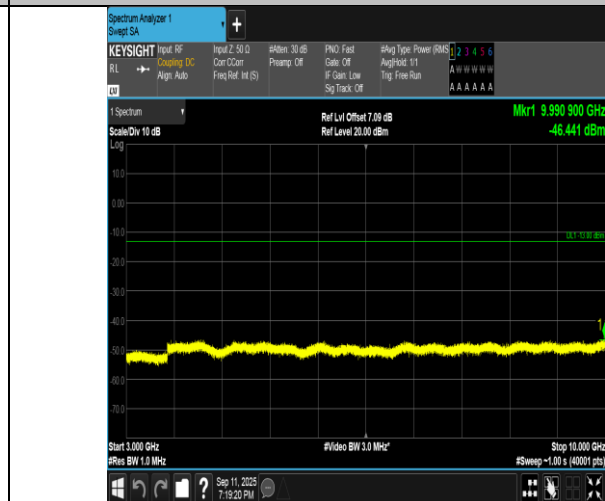
Band5-3MHz-16QAM-20635-1RB#0-3000~10000-PASS
