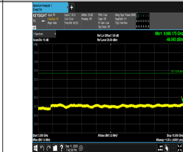
Band5-5MHz-16QAM-20425-1RB#0-3000~10000-PASS
