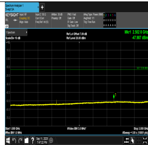
Band5-5MHz-QPSK-20525-1RB#0-1000~3000-PASS
