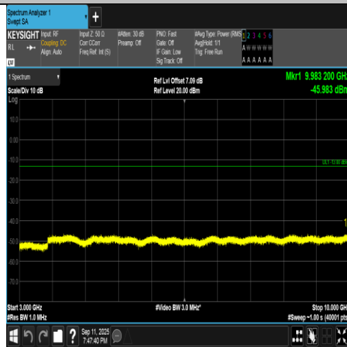
Band5-5MHz-QPSK-20525-1RB#0-3000~10000-PASS
