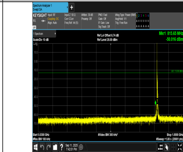
Band5-5MHz-16QAM-20425-1RB#0-30~1000-PASS
