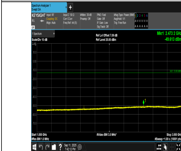
Band5-5MHz-16QAM-20425-1RB#0-1000~3000-PASS
