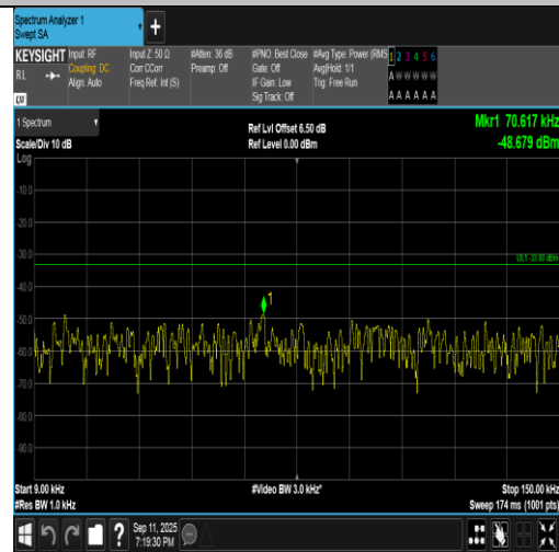
Band5-3MHz-QPSK-20635-1RB#14-0.009~0.15-PASS
