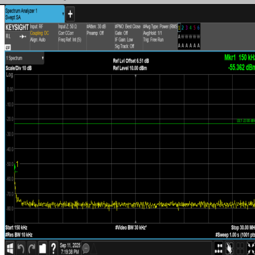
Band5-3MHz-QPSK-20635-1RB#14-0.15~30-PASS
