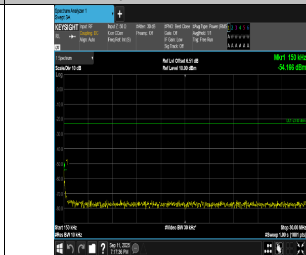
Band5-3MHz-QPSK-20635-1RB#0-0.15~30-PASS
