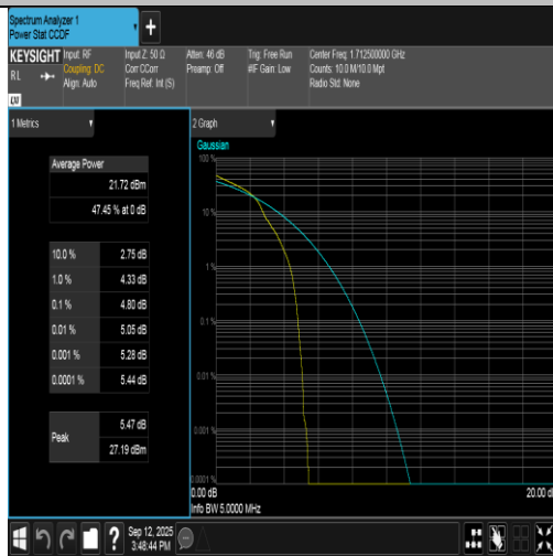
Band66-5MHz-16QAM-131997-1RB#0-PASS
