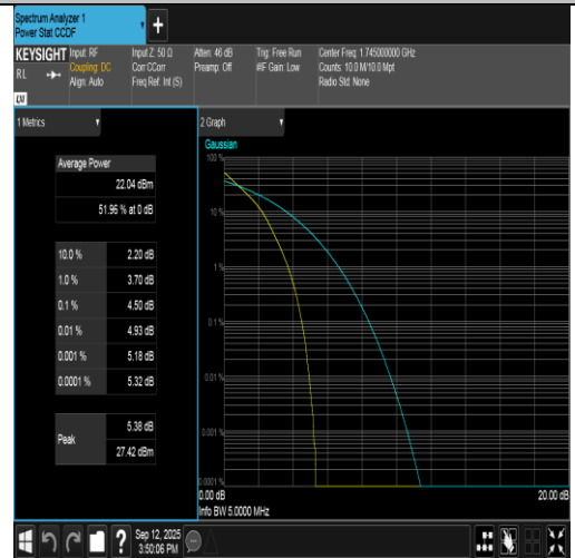
Band66-5MHz-QPSK-132322-25RB#0-PASS
