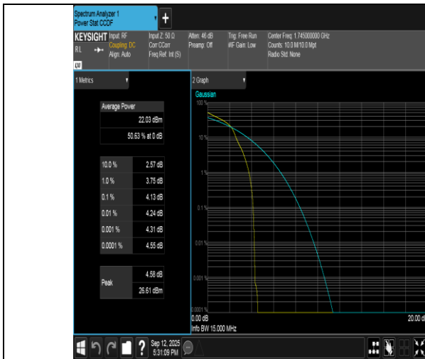
Band66-15MHz-16QAM-132322-1RB#0-PASS
