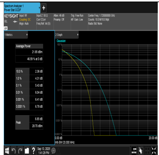
Band66-20MHz-QPSK-132072-100RB#0-PASS
