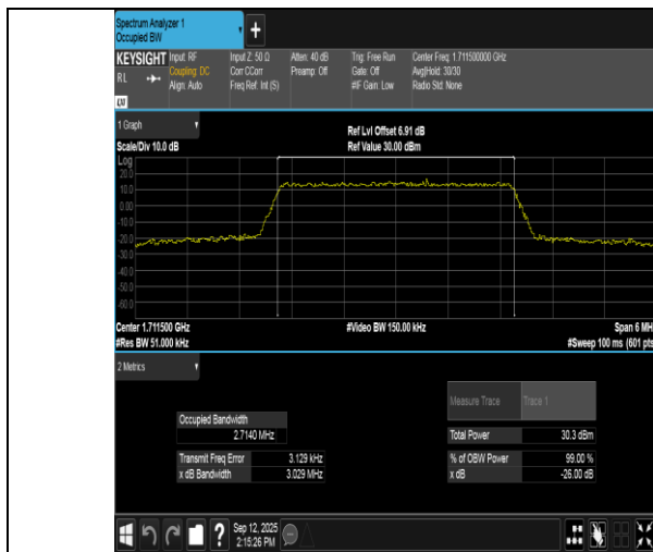
Band66-3MHz-QPSK-131987-15RB#0-PASS
