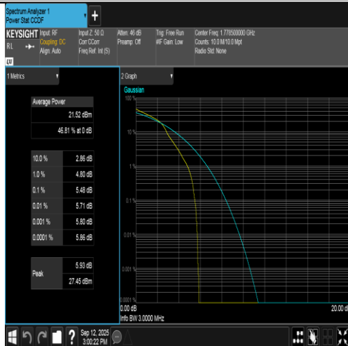
Band66-3MHz-16QAM-132657-1RB#0-PASS
