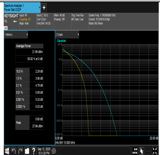
Band66-15MHz-QPSK-132322-75RB#0-PASS
