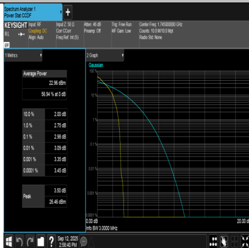
Band66-3MHz-QPSK-132322-1RB#0-PASS
