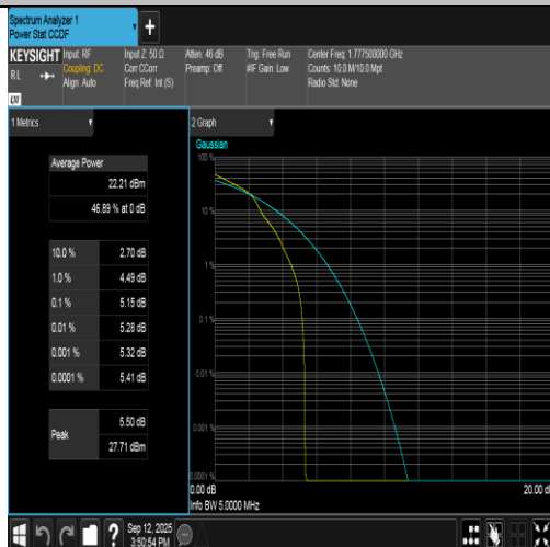
Band66-5MHz-16QAM-132647-1RB#0-PASS
