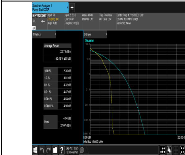
Band66-15MHz-QPSK-132597-1RB#0-PASS
