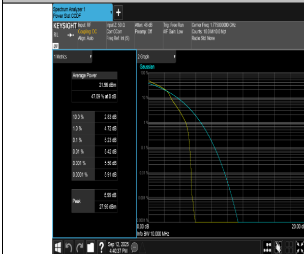
Band66-10MHz-16QAM-132622-1RB#0-PASS
