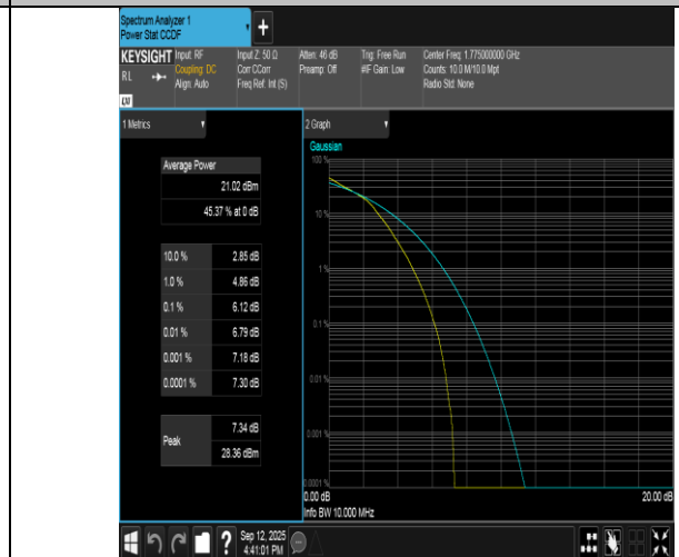
Band66-10MHz-16QAM-132622-50RB#0-PASS
