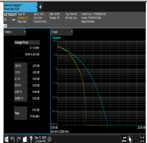
Band66-1.4MHz-16QAM-132665-6RB#0-PASS
