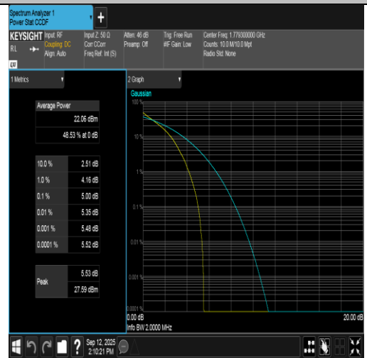
Band66-1.4MHz-QPSK-132665-6RB#0-PASS
