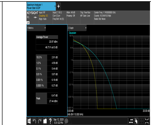
Band66-15MHz-16QAM-132322-75RB#0-PASS
