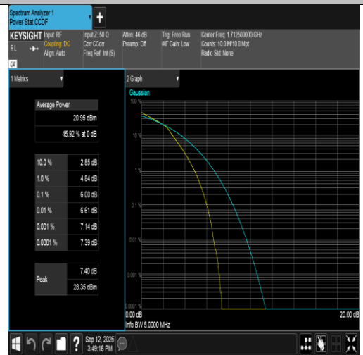
Band66-5MHz-16QAM-131997-25RB#0-PASS
