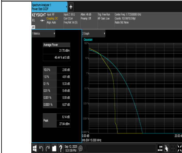
Band66-15MHz-16QAM-132597-1RB#0-PASS
