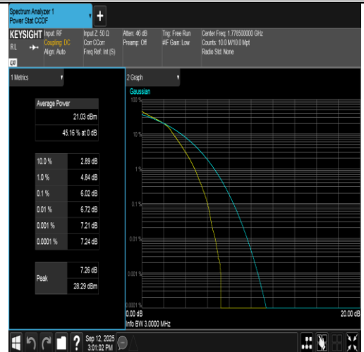
Band66-3MHz-16QAM-132657-15RB#0-PASS
