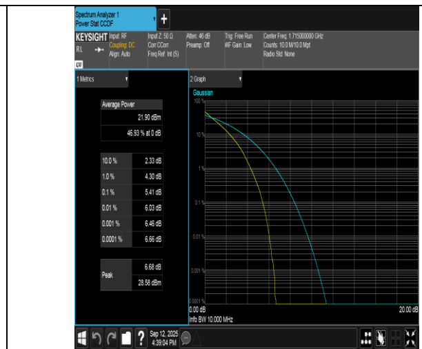
Band66-10MHz-QPSK-132022-50RB#0-PASS
