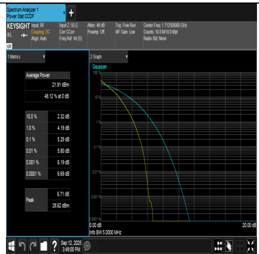
Band66-5MHz-QPSK-131997-25RB#0-PASS
