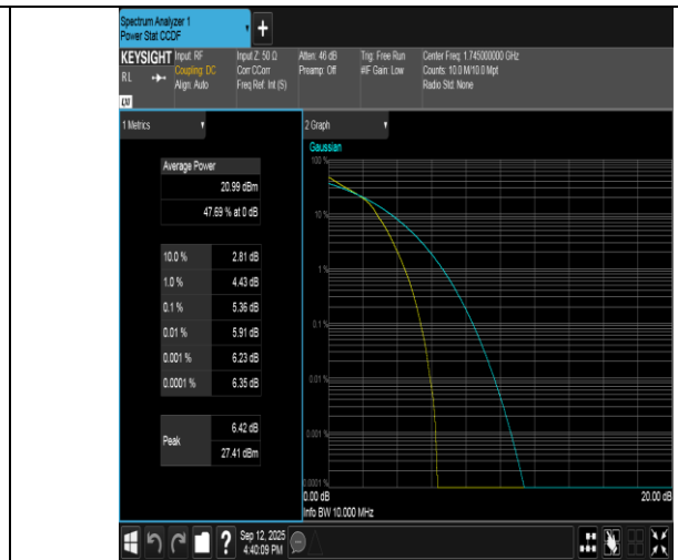
Band66-10MHz-16QAM-132322-50RB#0-PASS
