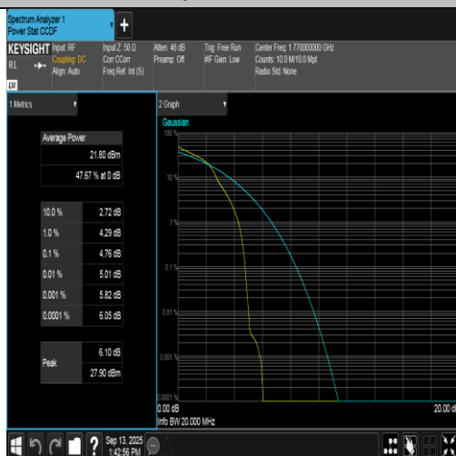
Band66-20MHz-16QAM-132572-1RB#0-PASS
