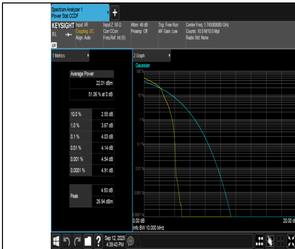
Band66-10MHz-16QAM-132322-1RB#0-PASS
