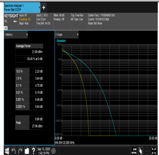
Band66-20MHz-QPSK-132322-100RB#0-PASS
