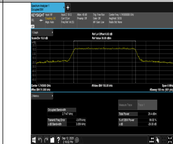
Band66-3MHz-16QAM-132322-15RB#0-PASS
