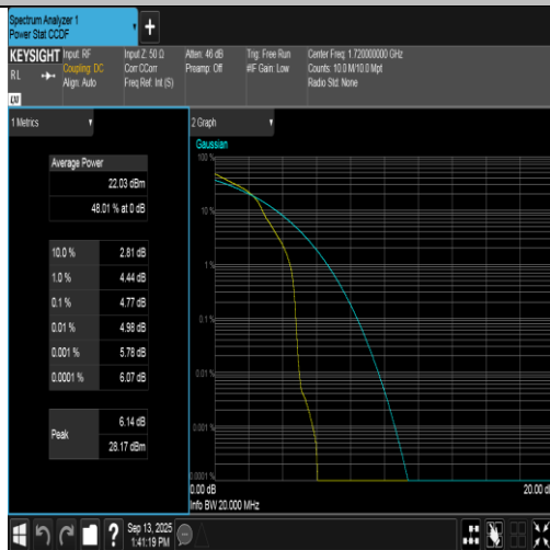
Band66-20MHz-16QAM-132072-1RB#0-PASS
