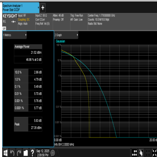
Band66-1.4MHz-16QAM-132665-1RB#0-PASS
