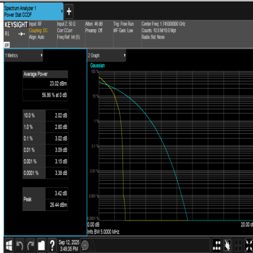
Band66-5MHz-QPSK-132322-1RB#0-PASS
