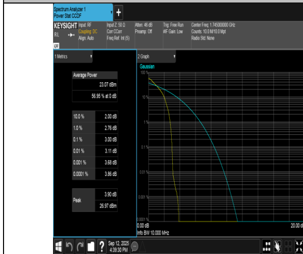
Band66-10MHz-QPSK-132322-1RB#0-PASS
