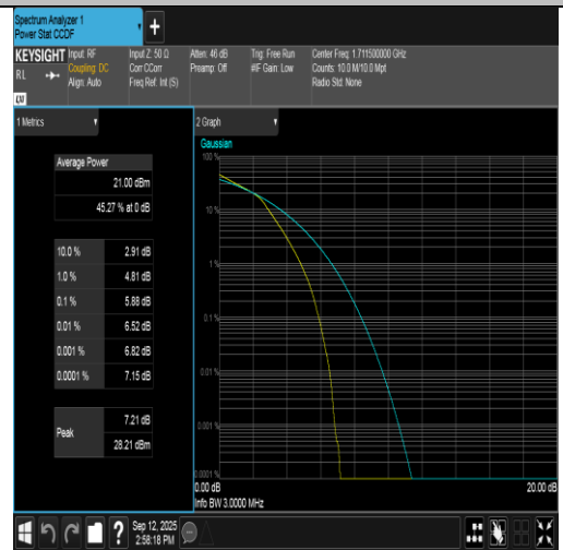
Band66-3MHz-16QAM-131987-15RB#0-PASS
