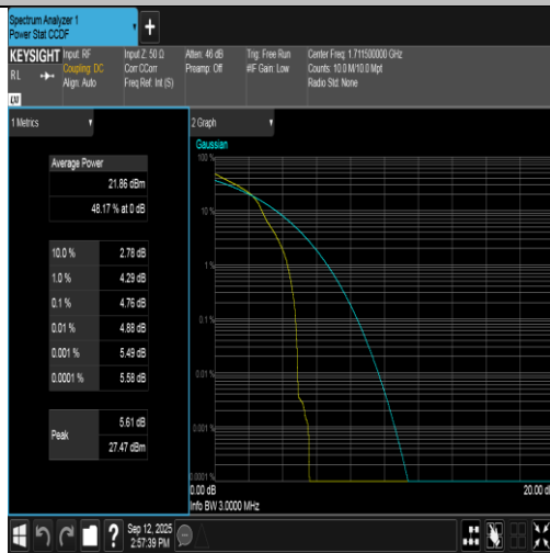
Band66-3MHz-16QAM-131987-1RB#0-PASS
