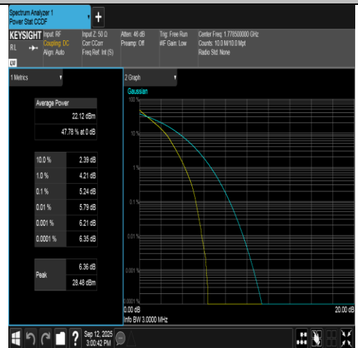
Band66-3MHz-QPSK-132657-15RB#0-PASS
