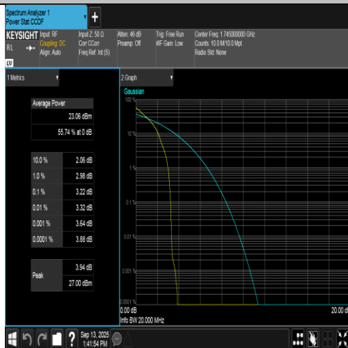
Band66-20MHz-QPSK-132322-1RB#0-PASS
