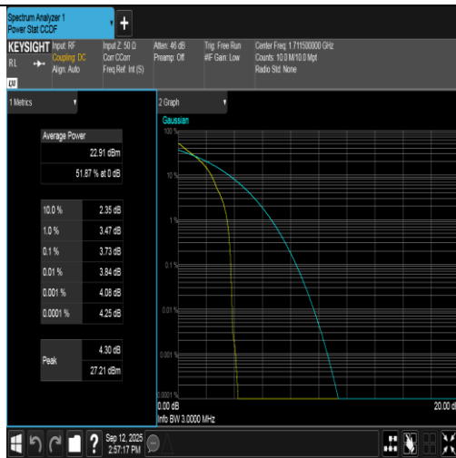
Band66-3MHz-QPSK-131987-1RB#0-PASS
