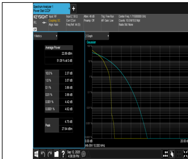
Band66-10MHz-QPSK-132022-1RB#0-PASS
