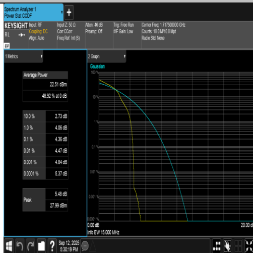
Band66-15MHz-16QAM-132047-1RB#0-PASS
