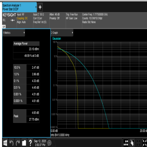
Band66-5MHz-QPSK-132647-1RB#0-PASS
