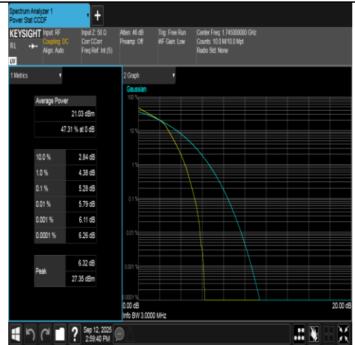
Band66-3MHz-16QAM-132322-15RB#0-PASS
