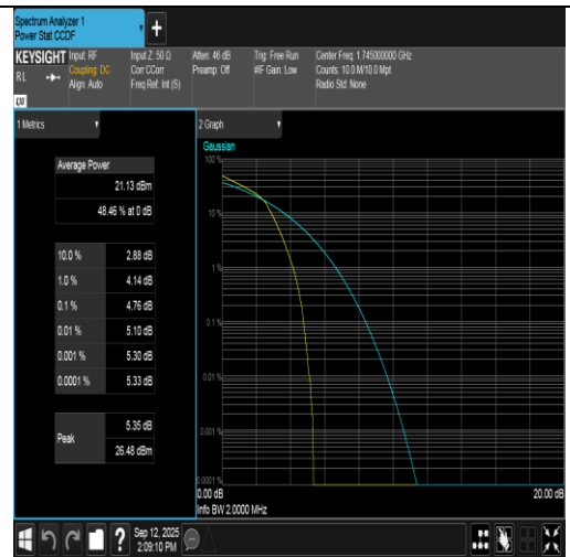
Band66-1.4MHz-16QAM-132322-6RB#0-PASS
