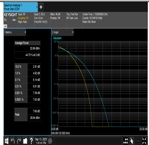
Band66-20MHz-16QAM-132072-100RB#0-PASS
