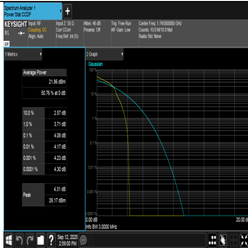
Band66-3MHz-16QAM-132322-1RB#0-PASS
