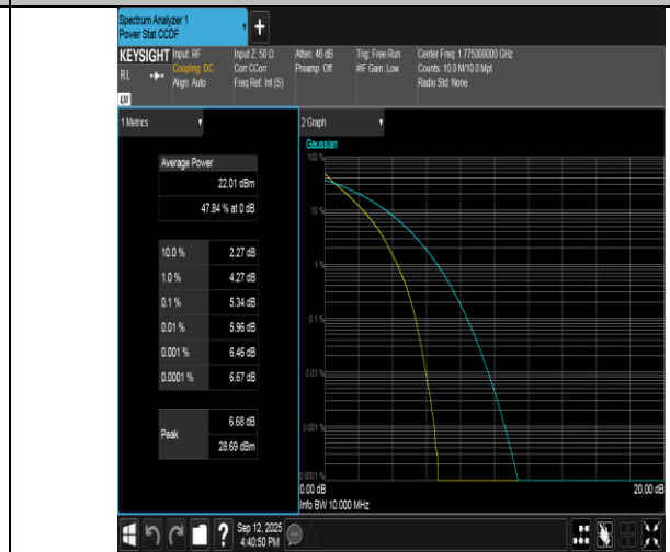
Band66-10MHz-QPSK-132622-50RB#0-PASS
