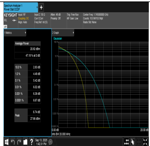
Band66-20MHz-16QAM-132322-100RB#0-PASS
