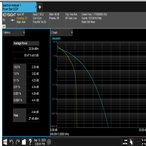
Band66-3MHz-QPSK-132657-1RB#0-PASS
