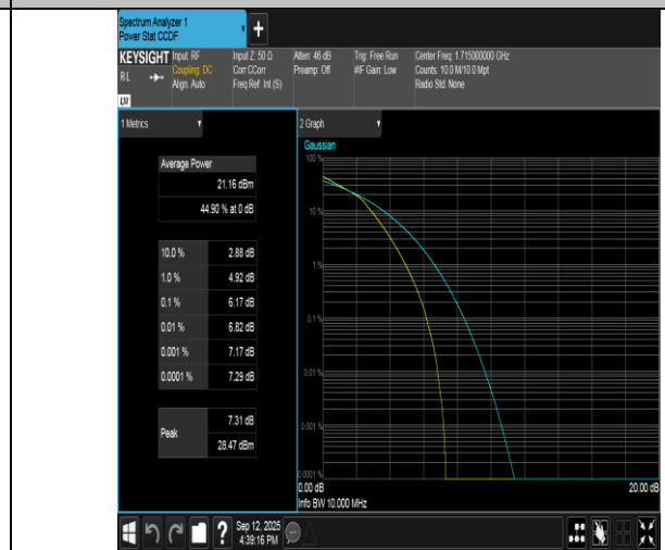
Band66-10MHz-16QAM-132022-50RB#0-PASS
