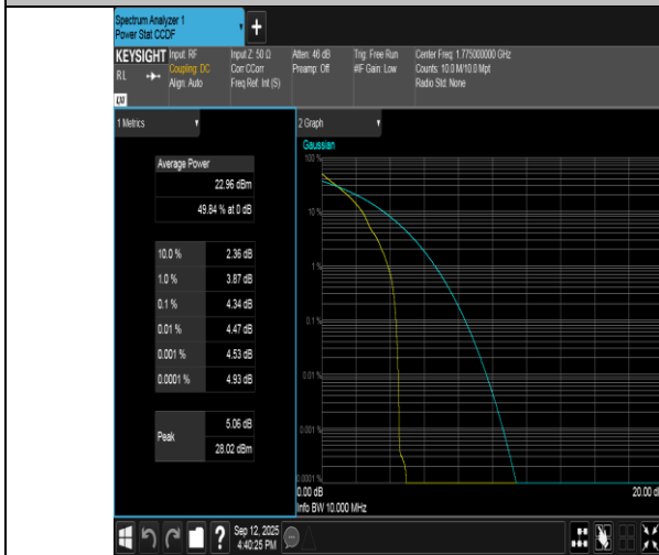
Band66-10MHz-QPSK-132622-1RB#0-PASS
