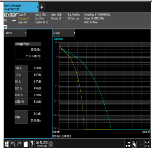
Band66-3MHz-QPSK-132322-15RB#0-PASS
