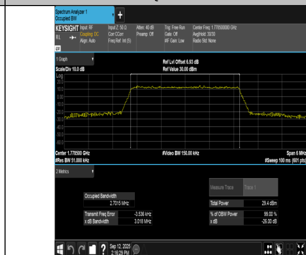
Band66-3MHz-16QAM-132657-15RB#0-PASS
