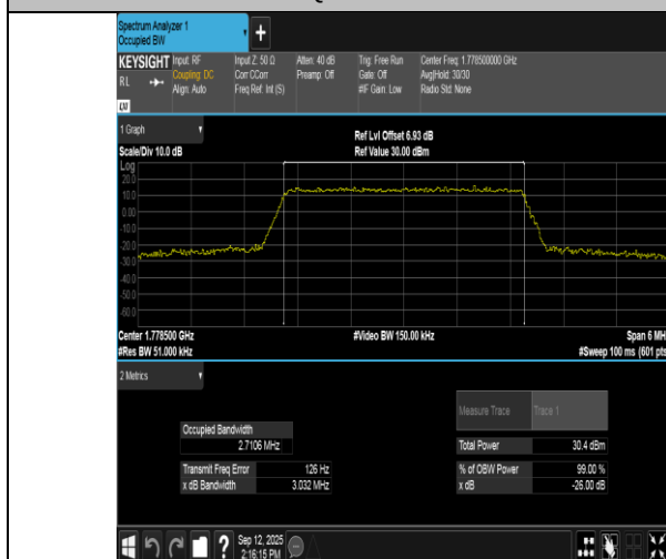
Band66-3MHz-QPSK-132657-15RB#0-PASS
