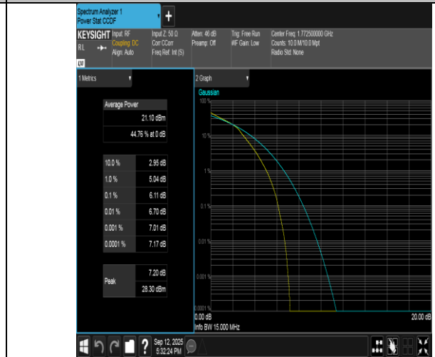
Band66-15MHz-16QAM-132597-75RB#0-PASS
