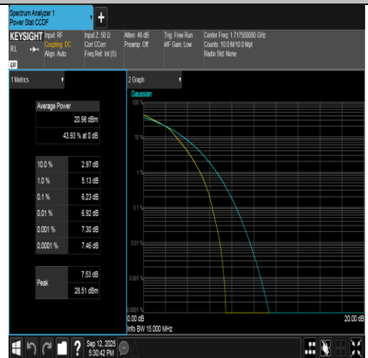
Band66-15MHz-16QAM-132047-75RB#0-PASS
