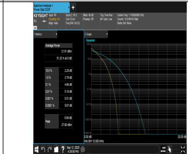
Band66-10MHz-QPSK-132322-50RB#0-PASS
