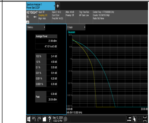
Band66-15MHz-QPSK-132597-75RB#0-PASS
