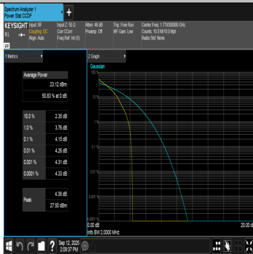
Band66-1.4MHz-QPSK-132665-1RB#0-PASS
