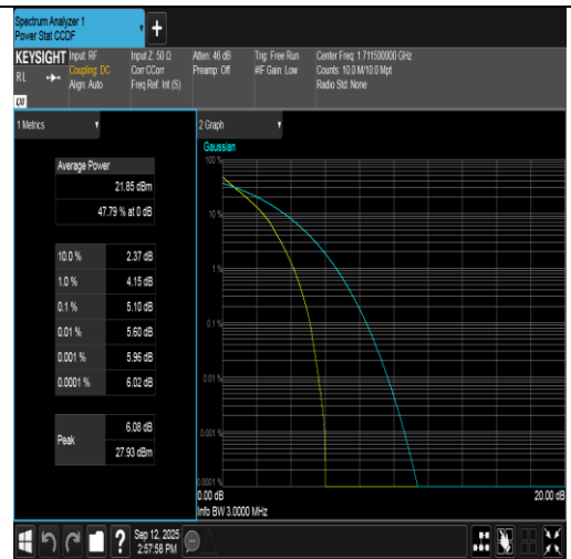
Band66-3MHz-QPSK-131987-15RB#0-PASS
