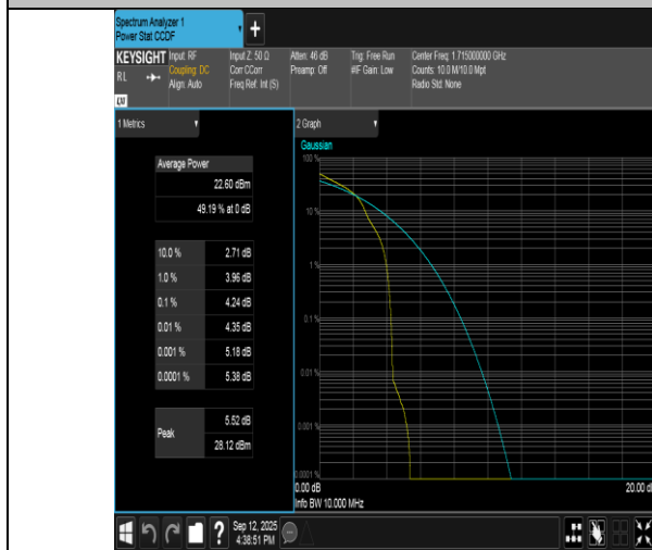
Band66-10MHz-16QAM-132022-1RB#0-PASS
