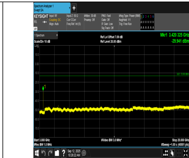
Band66-1.4MHz-16QAM-131979-1RB#0-3000~20000-PASS
