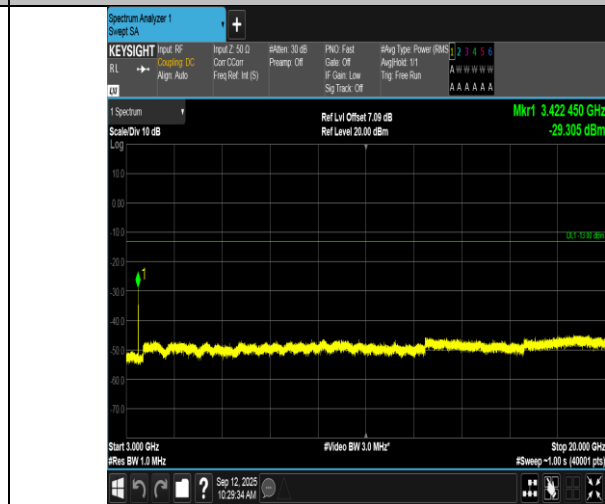
Band66-1.4MHz-QPSK-131979-1RB#5-3000~20000-PASS
