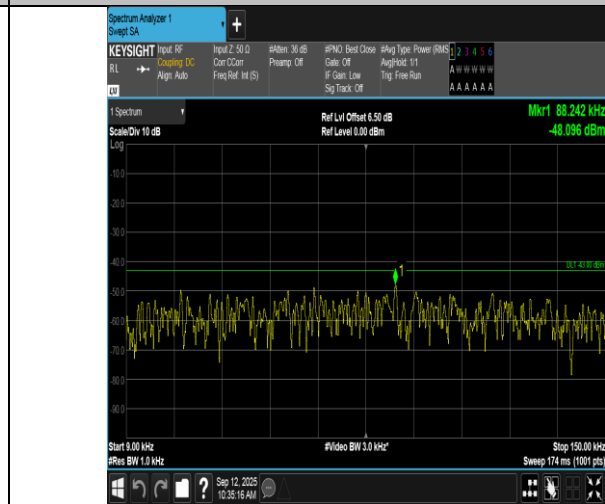
Band66-1.4MHz-16QAM-132322-1RB#0-0.009~0.15-PASS
