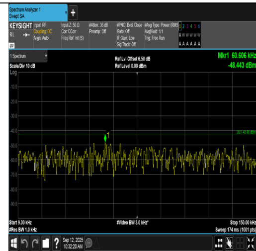
Band66-1.4MHz-16QAM-131979-6RB#0-0.009~0.15-PASS
