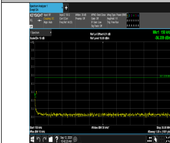
Band66-1.4MHz-16QAM-132665-1RB#0-0.15~30-PASS
