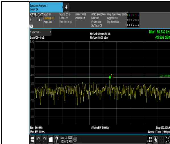
Band66-1.4MHz-QPSK-132322-1RB#0-0.009~0.15-PASS
