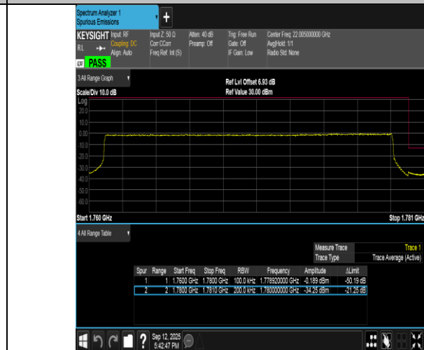
Band66-20MHz-16QAM-132572-100RB#0-PASS
