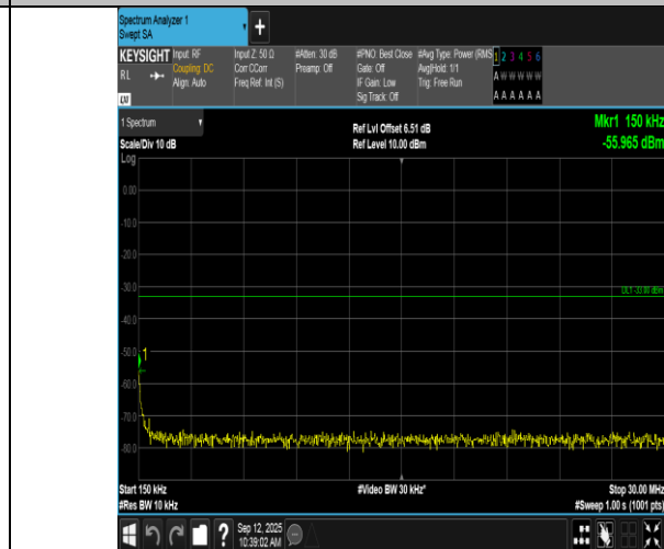
Band66-1.4MHz-QPSK-132322-6RB#0-0.15~30-PASS
