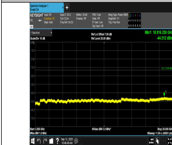
Band66-1.4MHz-QPSK-132665-6RB#0-3000~20000-PASS
