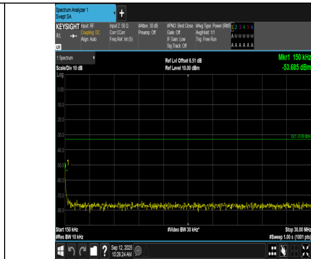
Band66-1.4MHz-QPSK-131979-1RB#0-0.15~30-PASS
