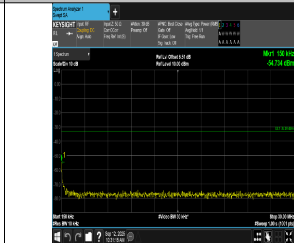
Band66-1.4MHz-QPSK-131979-6RB#0-0.15~30-PASS
