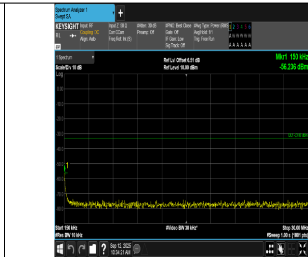
Band66-1.4MHz-QPSK-132322-1RB#0-0.15~30-PASS
