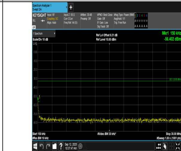
Band66-1.4MHz-16QAM-132322-1RB#5-0.15~30-PASS
