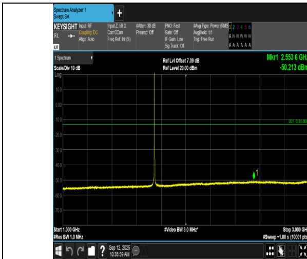
Band66-1.4MHz-16QAM-132322-1RB#0-1000~3000-PASS
