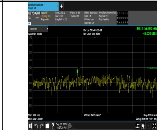
Band66-1.4MHz-16QAM-131979-1RB#0-0.009~0.15-PASS
