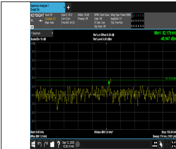
Band66-1.4MHz-QPSK-131979-1RB#0-0.009~0.15-PASS
