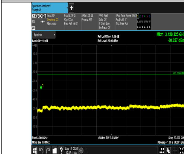
Band66-1.4MHz-QPSK-131979-1RB#0-3000~20000-PASS
