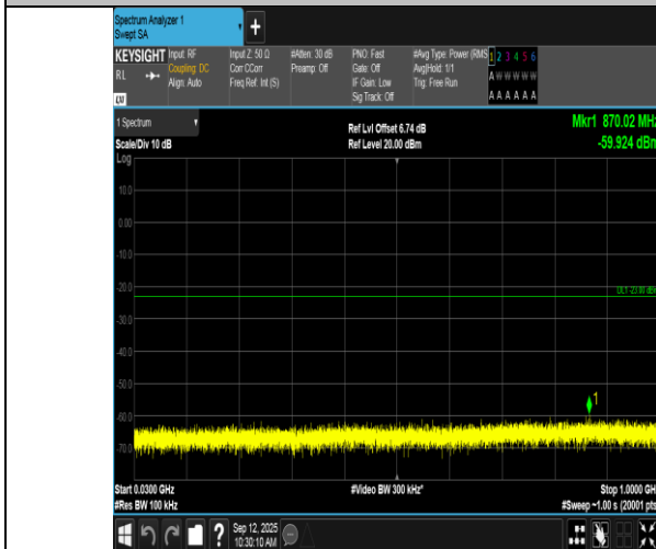
Band66-1.4MHz-16QAM-131979-1RB#5-30~1000-PASS
