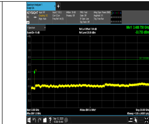
Band66-1.4MHz-16QAM-132322-1RB#0-3000~20000-PASS
