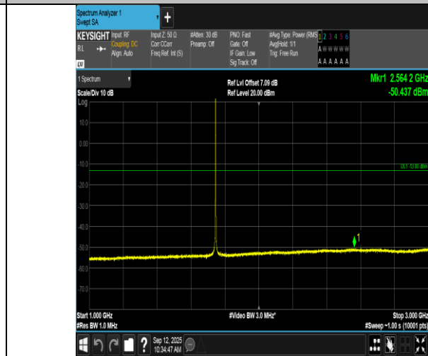
Band66-1.4MHz-QPSK-132322-1RB#0-1000~3000-PASS
