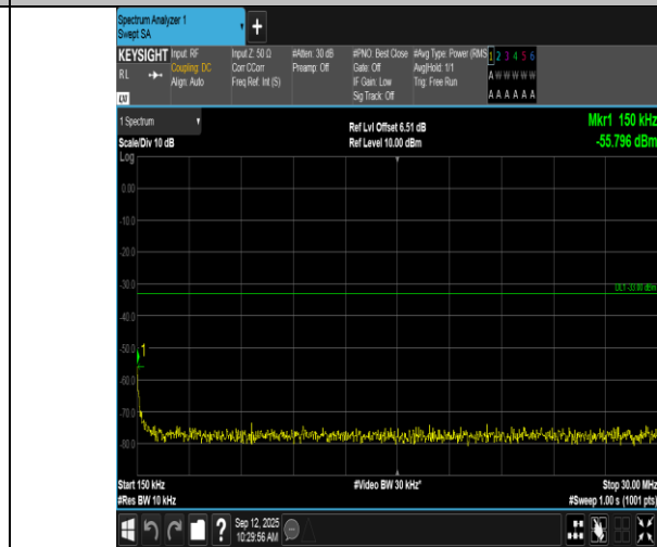
Band66-1.4MHz-16QAM-131979-1RB#5-0.15~30-PASS
