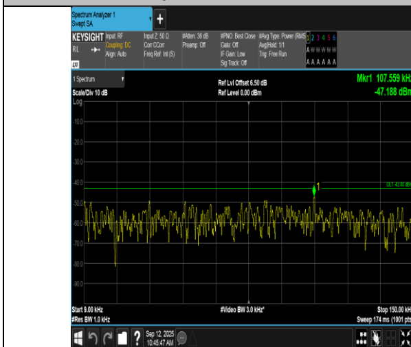
Band66-1.4MHz-QPSK-132665-6RB#0-0.009~0.15-PASS
