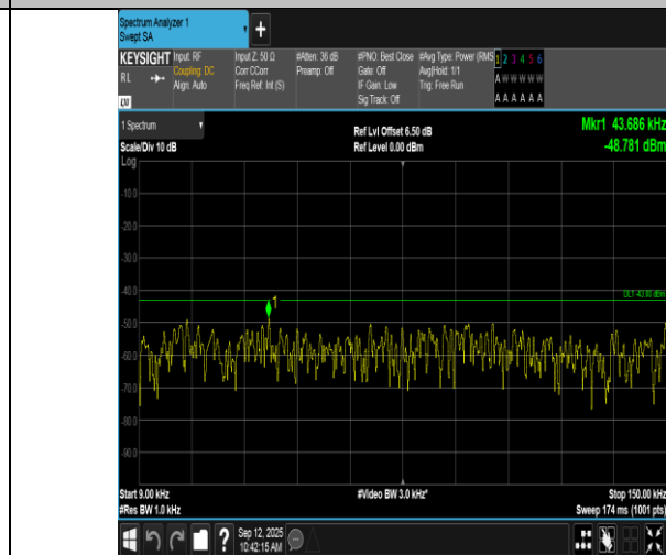
Band66-1.4MHz-16QAM-132665-1RB#0-0.009~0.15-PASS
