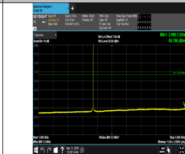
Band66-1.4MHz-16QAM-132322-1RB#5-1000~3000-PASS
