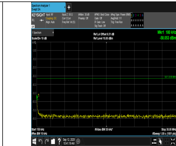
Band66-1.4MHz-QPSK-132665-1RB#0-0.15~30-PASS
