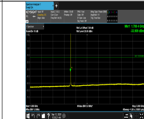
Band66-1.4MHz-16QAM-131979-1RB#5-1000~3000-PASS
