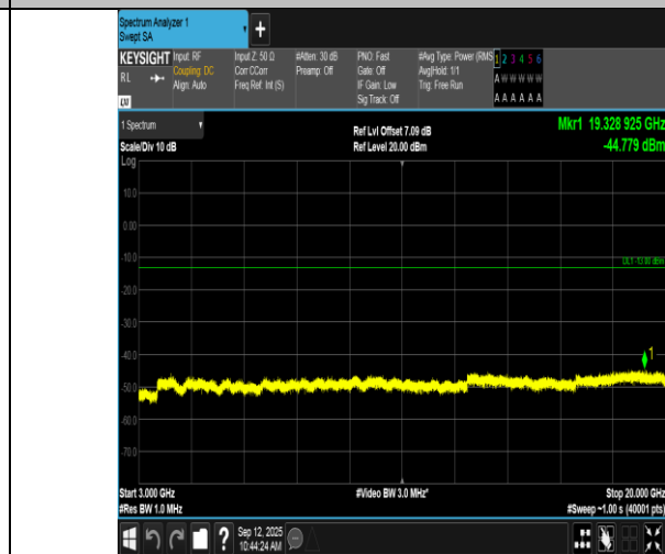
Band66-1.4MHz-QPSK-132665-1RB#5-3000~20000-PASS
