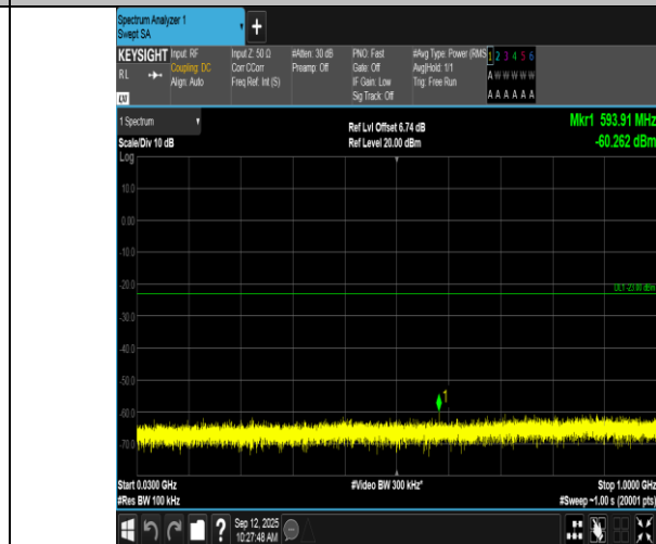
Band66-1.4MHz-16QAM-131979-1RB#0-30~1000-PASS
