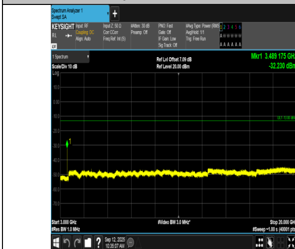
Band66-1.4MHz-QPSK-132322-1RB#0-3000~20000-PASS
