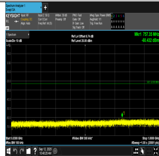
Band66-1.4MHz-16QAM-132322-6RB#0-30~1000-PASS
