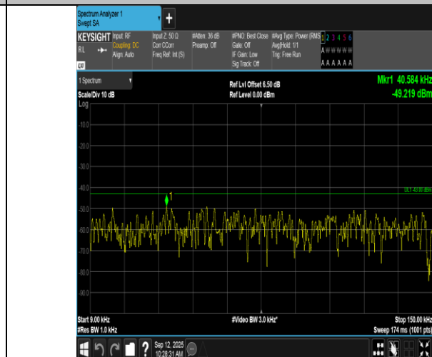
Band66-1.4MHz-QPSK-131979-1RB#5-0.009~0.15-PASS
