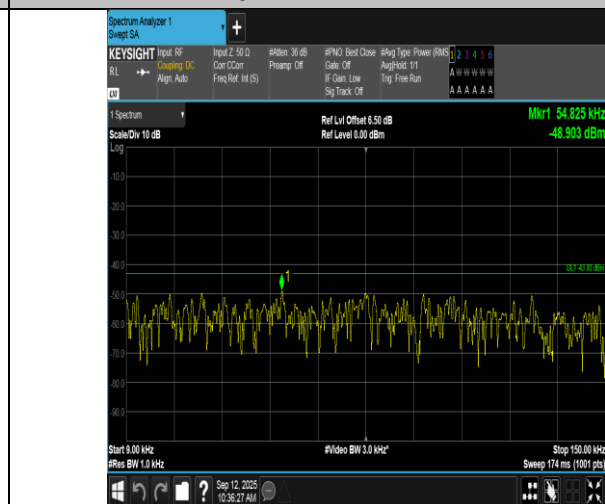
Band66-1.4MHz-QPSK-132322-1RB#5-0.009~0.15-PASS
