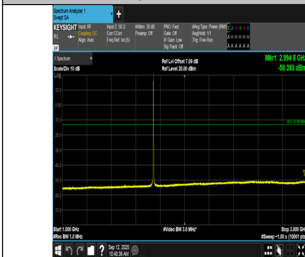
Band66-1.4MHz-16QAM-132322-6RB#0-1000~3000-PASS
