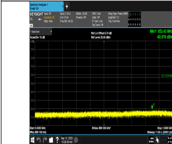
Band66-1.4MHz-QPSK-131979-1RB#0-30~1000-PASS
