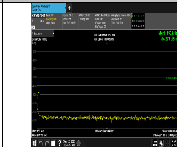
Band66-1.4MHz-QPSK-132665-6RB#0-0.15~30-PASS
