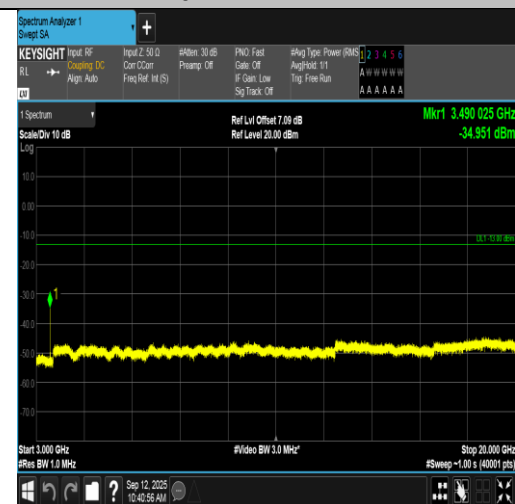
Band66-1.4MHz-16QAM-132322-6RB#0-3000~20000-PASS
