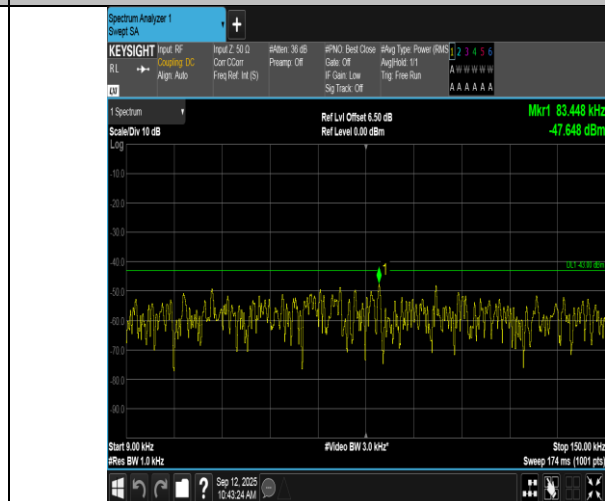
Band66-1.4MHz-QPSK-132665-1RB#5-0.009~0.15-PASS
