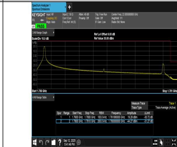
Band66-20MHz-16QAM-132572-1RB#0-PASS
