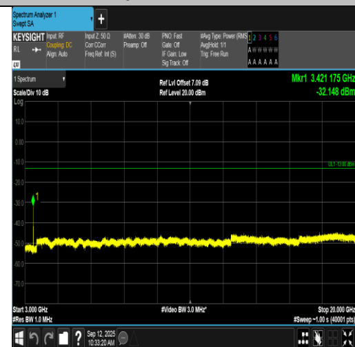
Band66-1.4MHz-16QAM-131979-6RB#0-3000~20000-PASS
