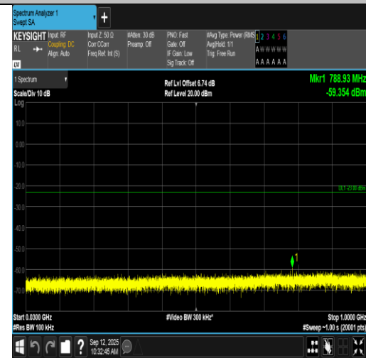
Band66-1.4MHz-16QAM-131979-6RB#0-30~1000-PASS
