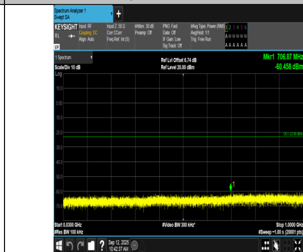
Band66-1.4MHz-16QAM-132665-1RB#0-30~1000-PASS
