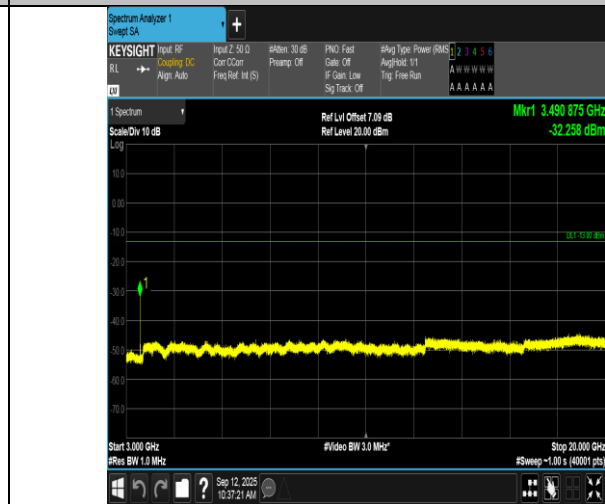
Band66-1.4MHz-QPSK-132322-1RB#5-3000~20000-PASS
