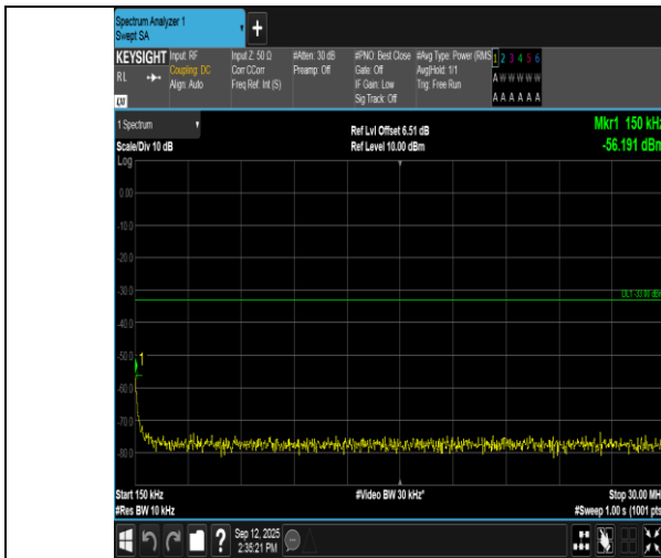
Band66-3MHz-QPSK-132657-1RB#14-0.15~30-PASS
