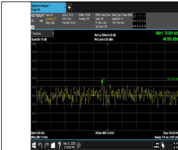
Band66-3MHz-QPSK-131987-1RB#0-0.009~0.15-PASS
