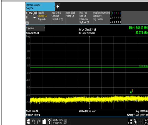
Band66-3MHz-QPSK-132657-1RB#0-30~1000-PASS
