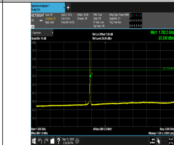
Band66-3MHz-QPSK-132657-1RB#0-1000~3000-PASS
