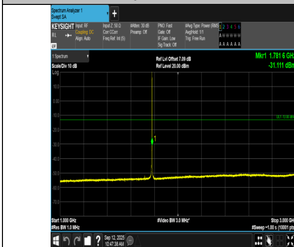
Band66-1.4MHz-16QAM-132665-6RB#0-1000~3000-PASS
