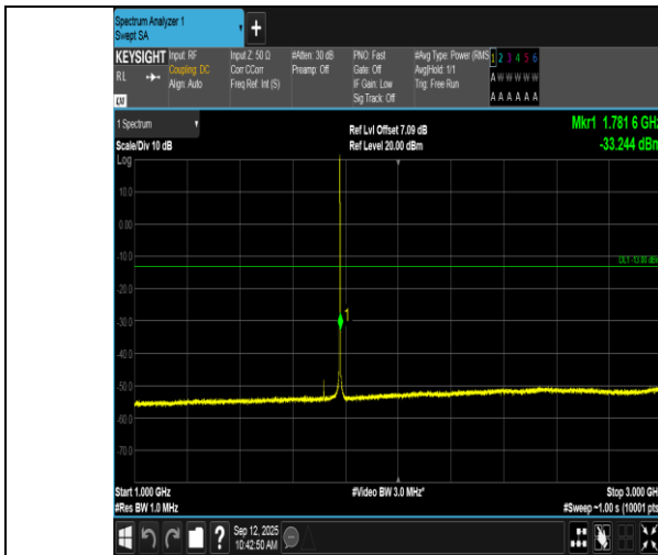
Band66-1.4MHz-16QAM-132665-1RB#0-1000~3000-PASS
