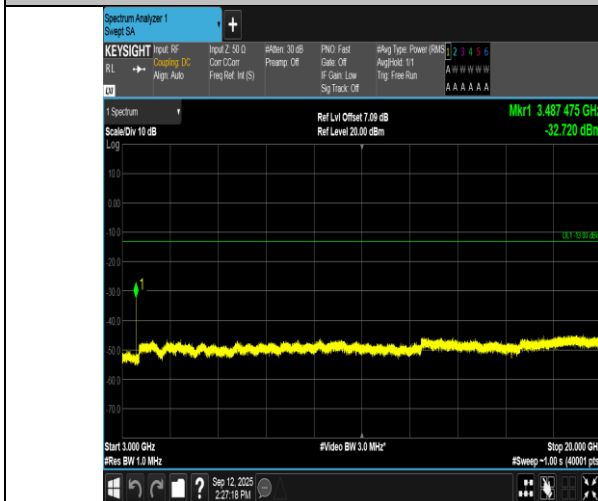
Band66-3MHz-QPSK-132322-1RB#0-3000~20000-PASS
