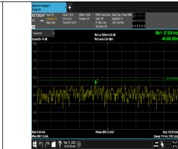
Band66-1.4MHz-16QAM-132665-6RB#0-0.009~0.15-PASS
