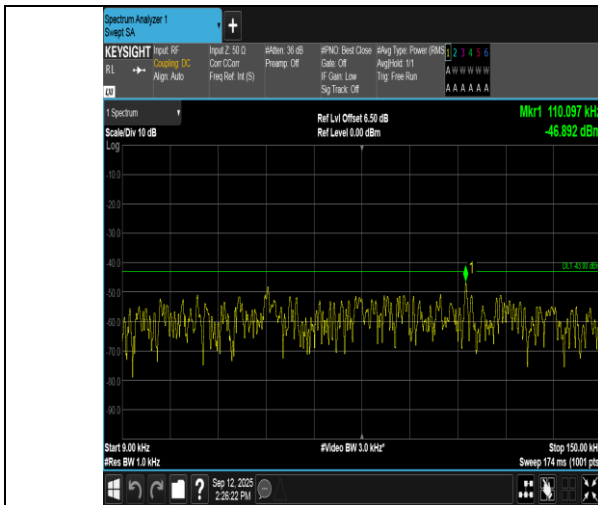
Band66-3MHz-QPSK-132322-1RB#0-0.009~0.15-PASS
