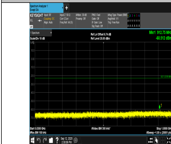
Band66-3MHz-16QAM-132322-1RB#14-30~1000-PASS
