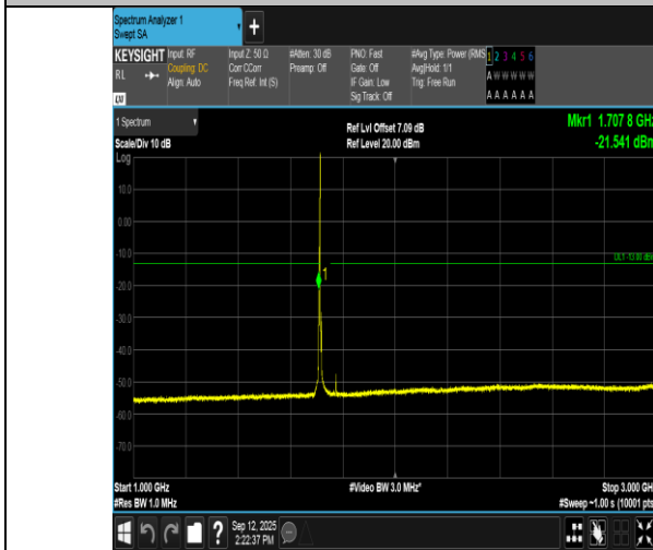
Band66-3MHz-QPSK-131987-1RB#14-1000~3000-PASS
