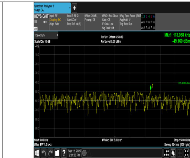
Band66-3MHz-16QAM-132322-15RB#0-0.009~0.15-PASS
