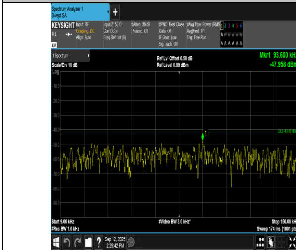
Band66-3MHz-16QAM-132322-1RB#14-0.009~0.15-PASS
