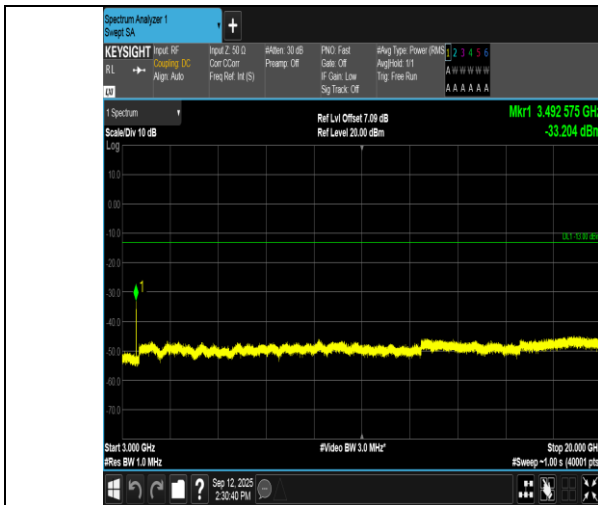
Band66-3MHz-16QAM-132322-1RB#14-3000~20000-PASS
