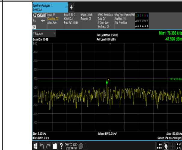
Band66-3MHz-QPSK-132322-1RB#14-0.009~0.15-PASS
