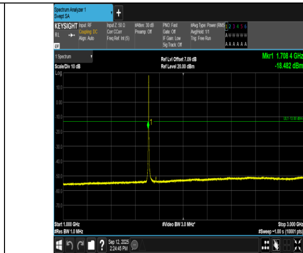
Band66-3MHz-QPSK-131987-15RB#0-1000~3000-PASS
