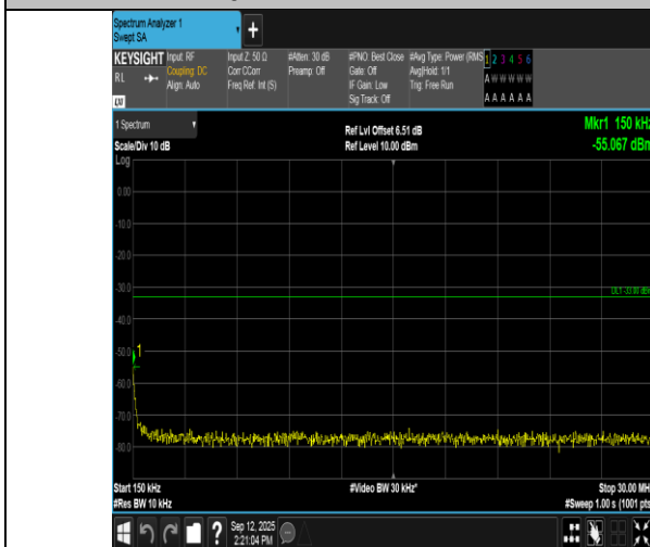
Band66-3MHz-16QAM-131987-1RB#0-0.15~30-PASS
