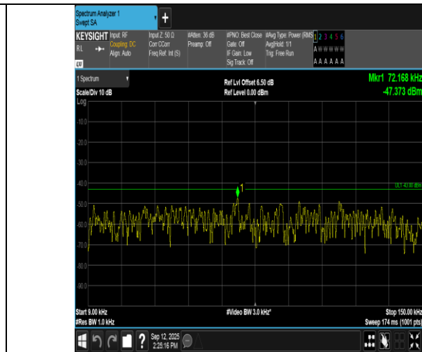
Band66-3MHz-16QAM-131987-15RB#0-0.009~0.15-PASS
