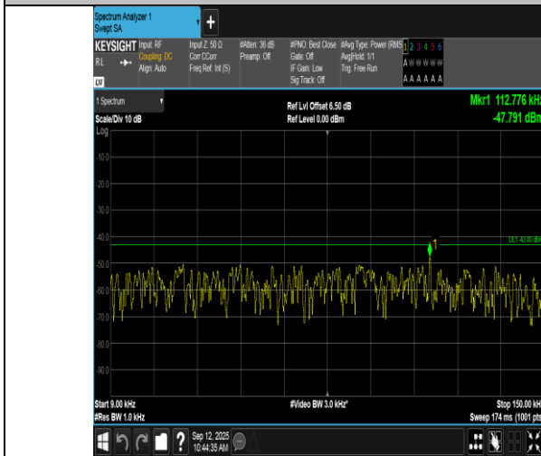
Band66-1.4MHz-16QAM-132665-1RB#5-0.009~0.15-PASS
