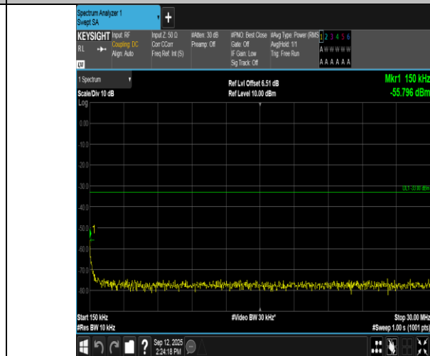
Band66-3MHz-QPSK-131987-15RB#0-0.15~30-PASS
