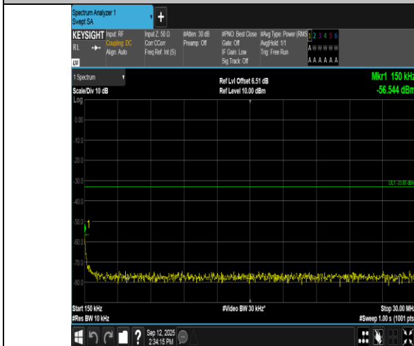
Band66-3MHz-16QAM-132657-1RB#0-0.15~30-PASS
