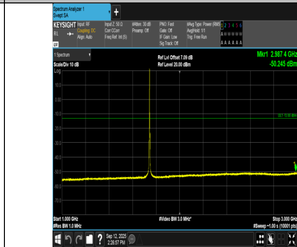
Band66-3MHz-QPSK-132322-1RB#0-1000~3000-PASS
