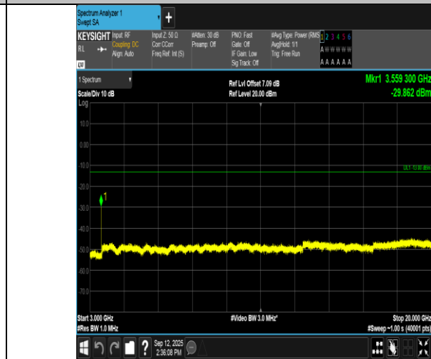
Band66-3MHz-QPSK-132657-1RB#14-3000~20000-PASS
