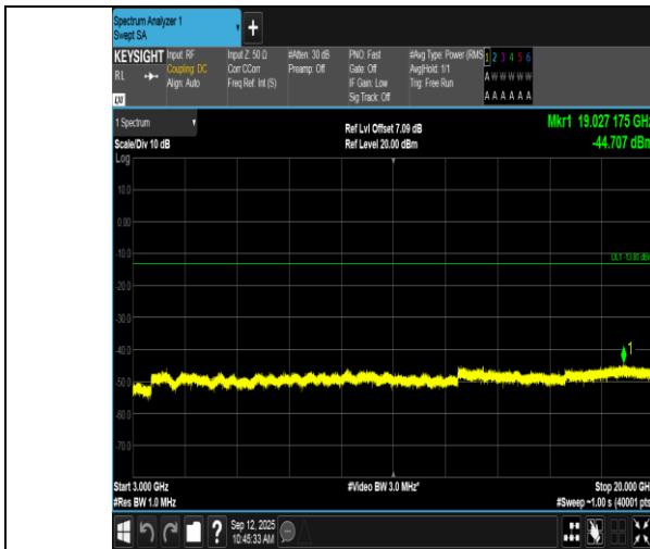
Band66-1.4MHz-16QAM-132665-1RB#5-3000~20000-PASS
