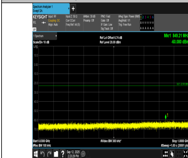
Band66-3MHz-16QAM-131987-1RB#14-30~1000-PASS
