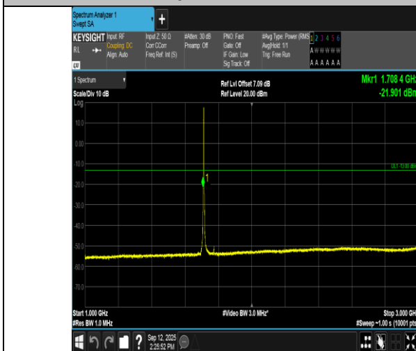
Band66-3MHz-16QAM-131987-15RB#0-1000~3000-PASS
