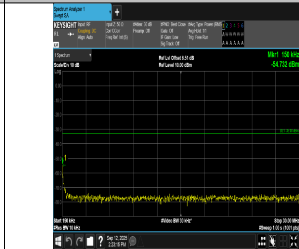
Band66-3MHz-16QAM-131987-1RB#14-0.15~30-PASS
