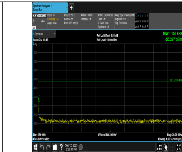
Band66-3MHz-QPSK-132322-1RB#0-0.15~30-PASS
