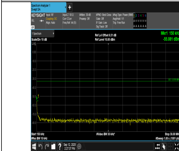
Band66-3MHz-16QAM-132322-1RB#0-0.15~30-PASS
