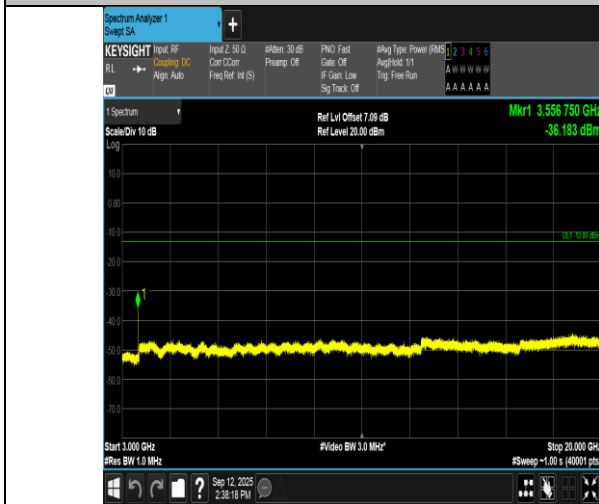
Band66-3MHz-QPSK-132657-15RB#0-3000~20000-PASS
