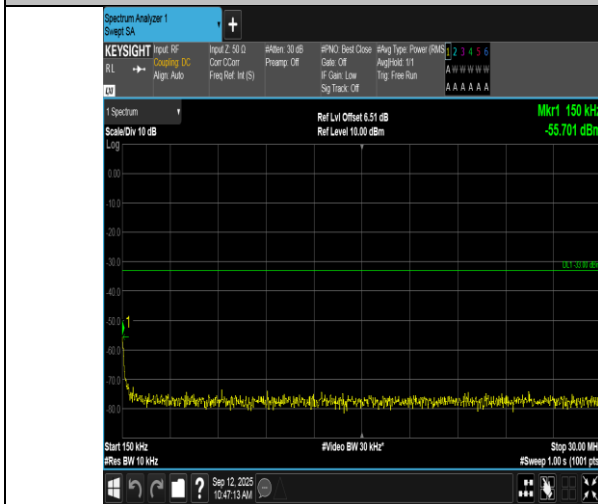
Band66-1.4MHz-16QAM-132665-6RB#0-0.15~30-PASS
