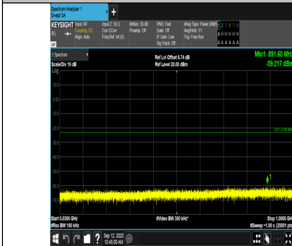
Band66-1.4MHz-16QAM-132665-1RB#5-30~1000-PASS
