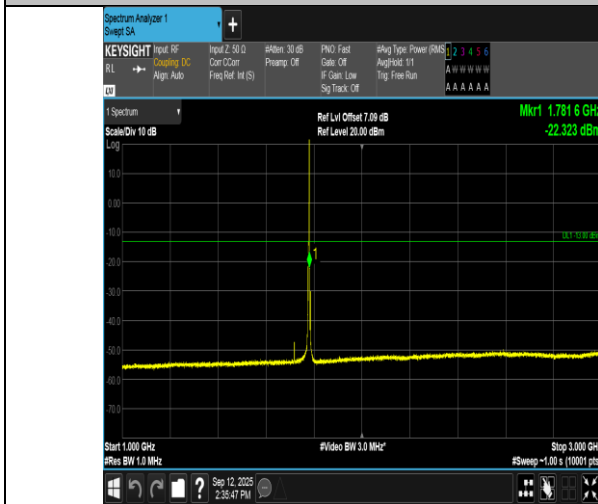
Band66-3MHz-QPSK-132657-1RB#14-1000~3000-PASS
