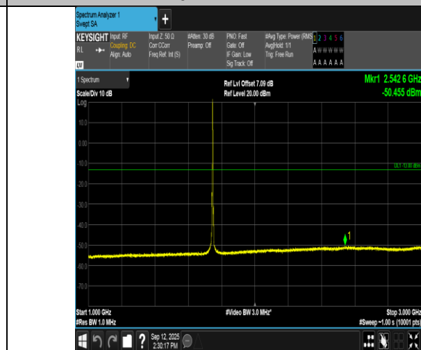
Band66-3MHz-16QAM-132322-1RB#14-1000~3000-PASS
