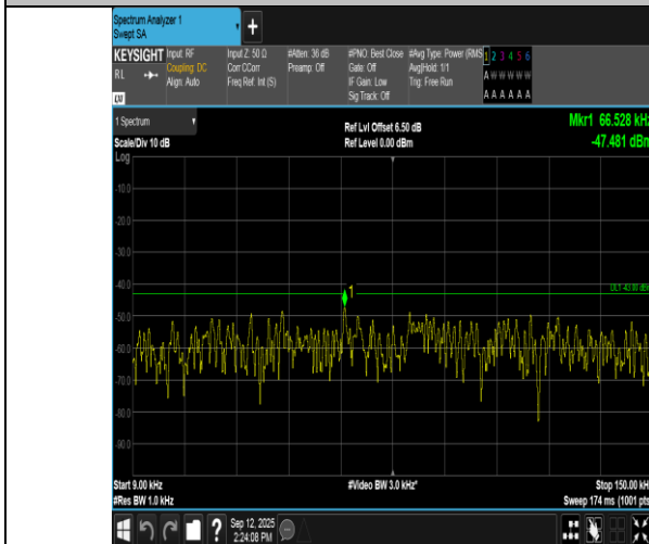
Band66-3MHz-QPSK-131987-15RB#0-0.009~0.15-PASS
