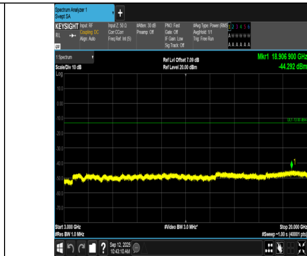
Band66-1.4MHz-16QAM-132665-1RB#0-3000~20000-PASS
