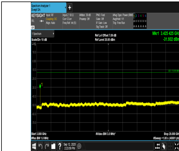
Band66-3MHz-16QAM-131987-1RB#14-3000~20000-PASS
