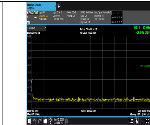
Band66-3MHz-QPSK-131987-1RB#0-0.15~30-PASS
