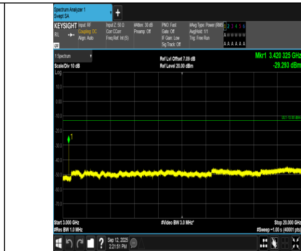
Band66-3MHz-16QAM-131987-1RB#0-3000~20000-PASS
