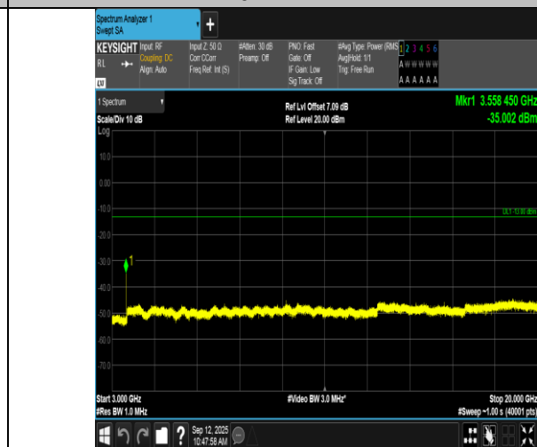
Band66-1.4MHz-16QAM-132665-6RB#0-3000~20000-PASS
