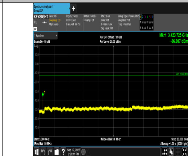
Band66-3MHz-16QAM-131987-15RB#0-3000~20000-PASS
