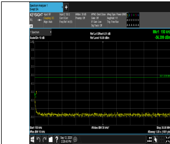
Band66-3MHz-QPSK-132322-1RB#14-0.15~30-PASS
