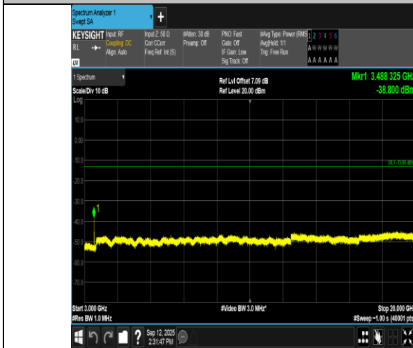
Band66-3MHz-QPSK-132322-15RB#0-3000~20000-PASS
