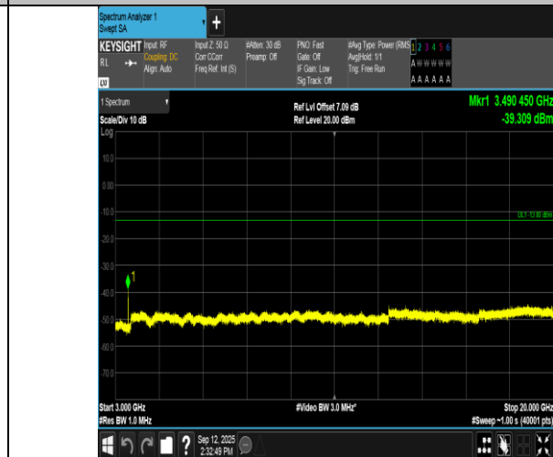
Band66-3MHz-16QAM-132322-15RB#0-3000~20000-PASS
