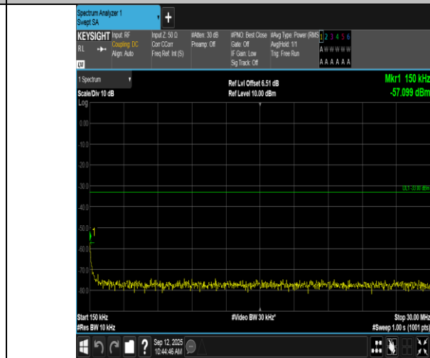
Band66-1.4MHz-16QAM-132665-1RB#5-0.15~30-PASS
