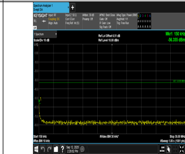
Band66-3MHz-16QAM-132322-1RB#14-0.15~30-PASS
