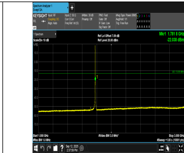
Band66-3MHz-QPSK-132657-15RB#0-1000~3000-PASS
