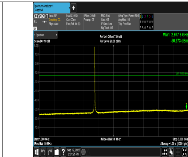
Band66-3MHz-QPSK-132322-15RB#0-1000~3000-PASS
