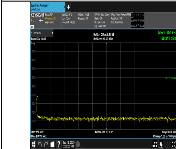
Band66-3MHz-16QAM-132322-15RB#0-0.15~30-PASS
