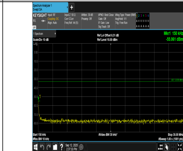
Band66-3MHz-QPSK-132657-15RB#0-0.15~30-PASS
