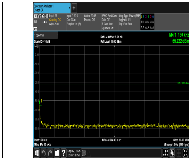
Band66-3MHz-QPSK-132657-1RB#0-0.15~30-PASS
