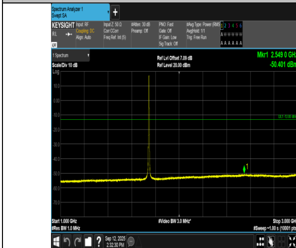
Band66-3MHz-16QAM-132322-15RB#0-1000~3000-PASS
