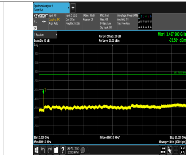
Band66-3MHz-16QAM-132322-1RB#0-3000~20000-PASS
