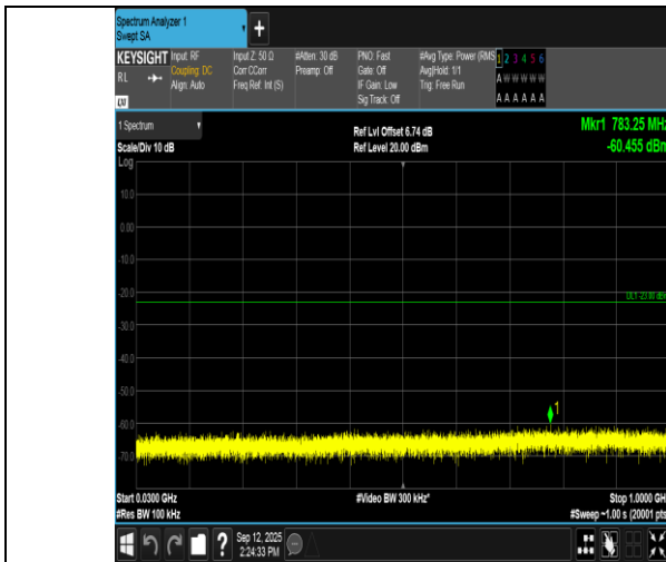
Band66-3MHz-QPSK-131987-15RB#0-30~1000-PASS
