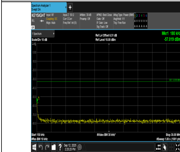
Band66-3MHz-16QAM-131987-15RB#0-0.15~30-PASS
