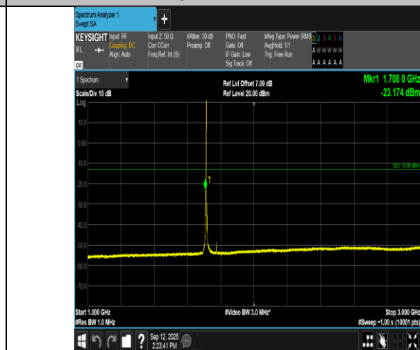
Band66-3MHz-16QAM-131987-1RB#14-1000~3000-PASS
