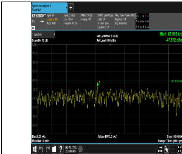
Band66-3MHz-QPSK-132657-1RB#0-0.009~0.15-PASS
