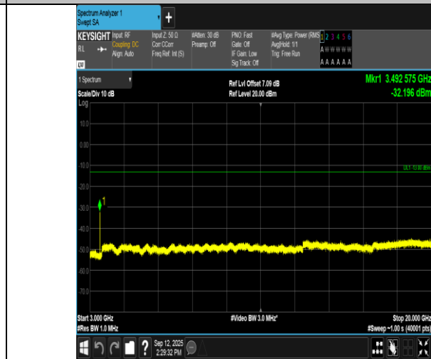
Band66-3MHz-QPSK-132322-1RB#14-3000~20000-PASS
