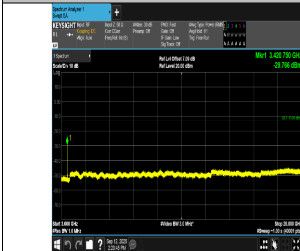
Band66-3MHz-QPSK-131987-1RB#0-3000~20000-PASS
