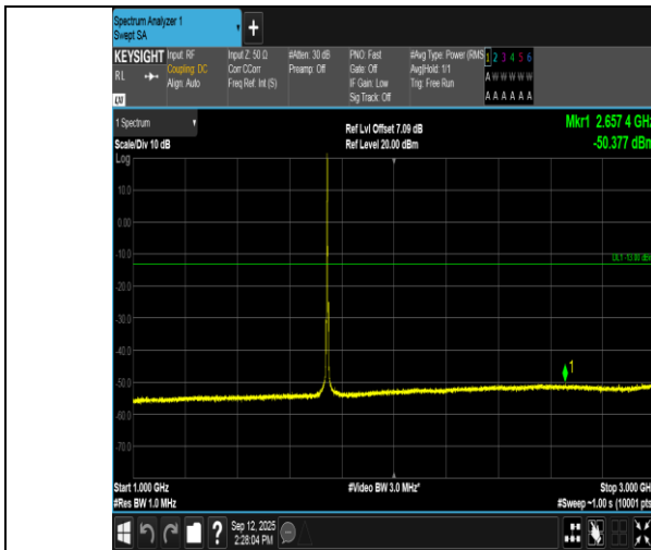
Band66-3MHz-16QAM-132322-1RB#0-1000~3000-PASS
