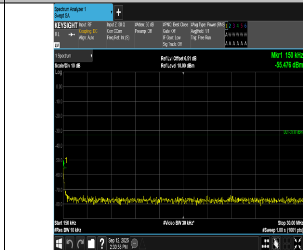
Band66-3MHz-QPSK-132322-15RB#0-0.15~30-PASS
