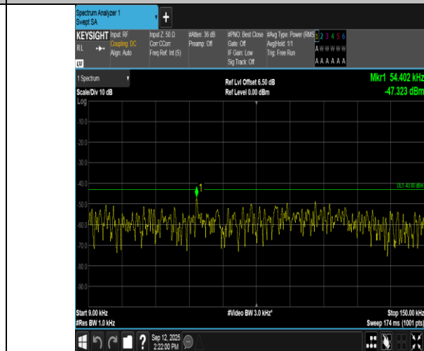
Band66-3MHz-QPSK-131987-1RB#14-0.009~0.15-PASS
