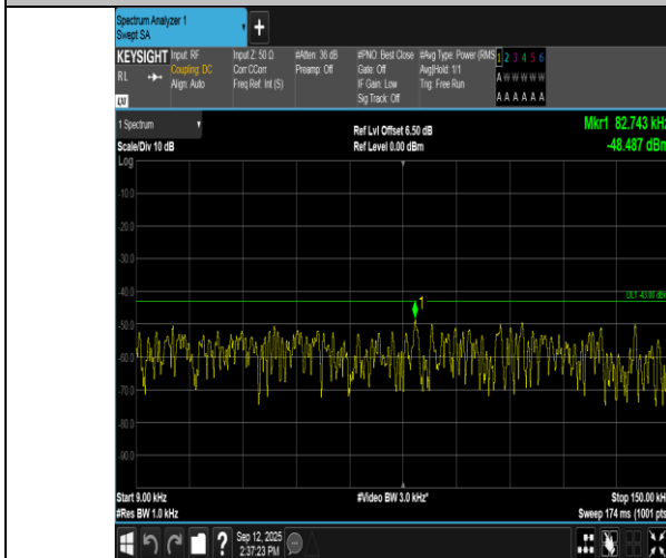
Band66-3MHz-QPSK-132657-15RB#0-0.009~0.15-PASS
