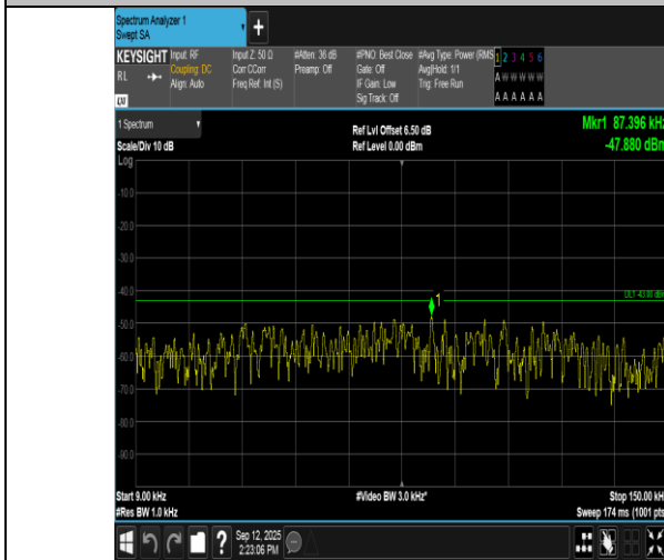
Band66-3MHz-16QAM-131987-1RB#14-0.009~0.15-PASS
