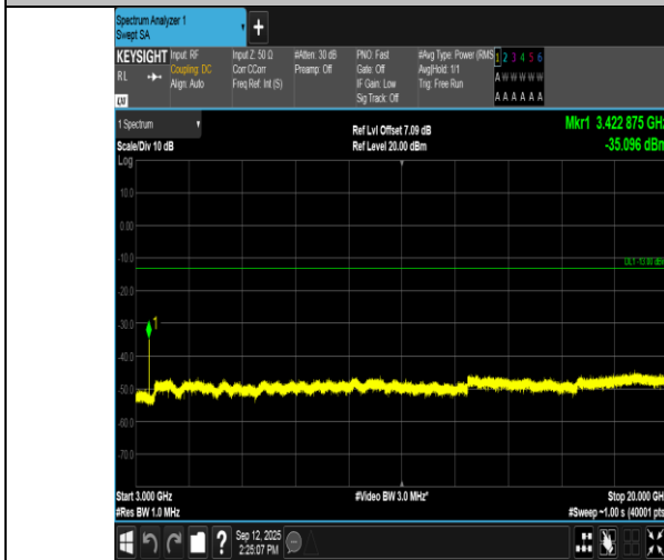
Band66-3MHz-QPSK-131987-15RB#0-3000~20000-PASS
