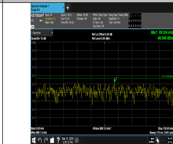
Band66-3MHz-QPSK-132657-1RB#14-0.009~0.15-PASS
