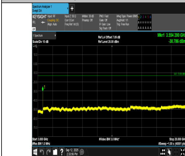
Band66-3MHz-QPSK-132657-1RB#0-3000~20000-PASS
