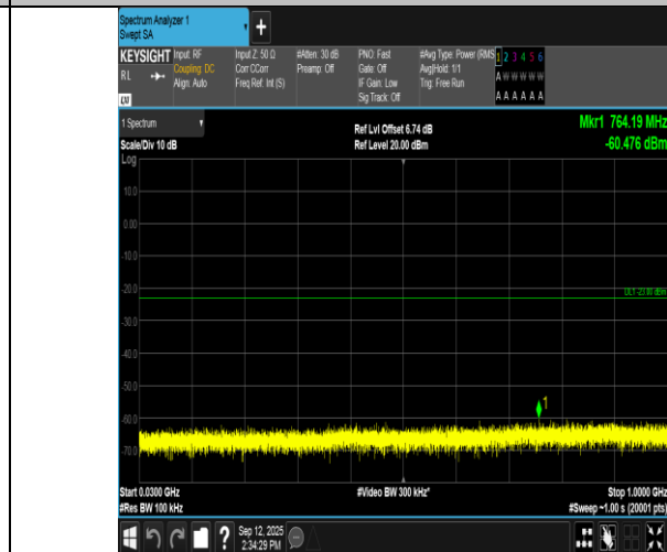
Band66-3MHz-16QAM-132657-1RB#0-30~1000-PASS
