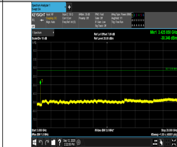
Band66-3MHz-QPSK-131987-1RB#14-3000~20000-PASS
