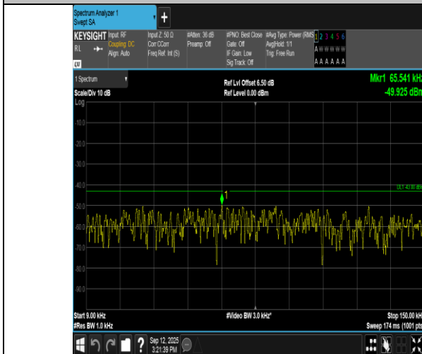
Band66-5MHz-QPSK-132322-25RB#0-0.009~0.15-PASS
