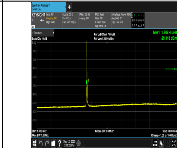
Band66-5MHz-QPSK-131997-1RB#0-1000~3000-PASS
