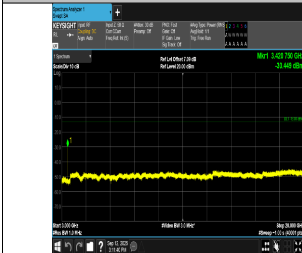
Band66-5MHz-QPSK-131997-1RB#0-3000~20000-PASS
