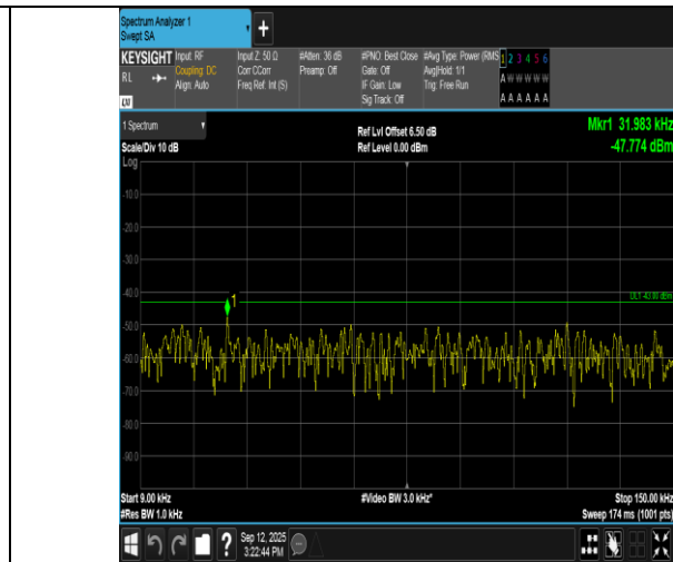
Band66-5MHz-16QAM-132322-25RB#0-0.009~0.15-PASS
