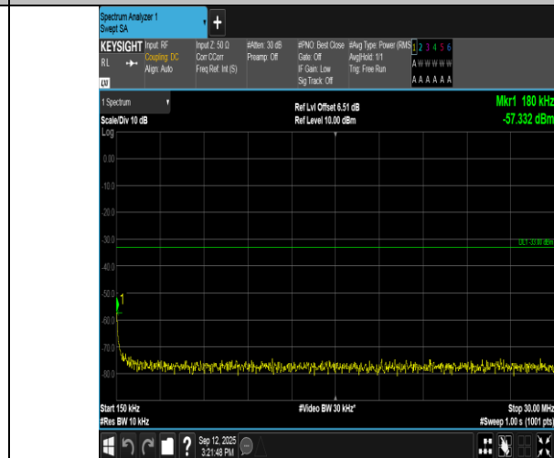
Band66-5MHz-QPSK-132322-25RB#0-0.15~30-PASS
