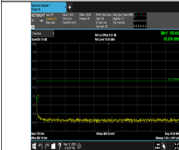
Band66-5MHz-16QAM-132322-1RB#0-0.15~30-PASS
