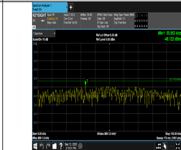
Band66-5MHz-QPSK-132322-1RB#24-0.009~0.15-PASS
