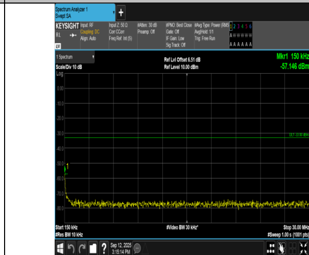
Band66-5MHz-QPSK-131997-25RB#0-0.15~30-PASS
