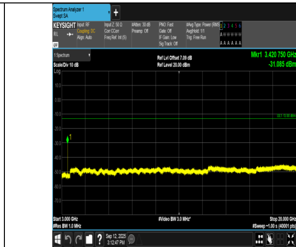
Band66-5MHz-16QAM-131997-1RB#0-3000~20000-PASS
