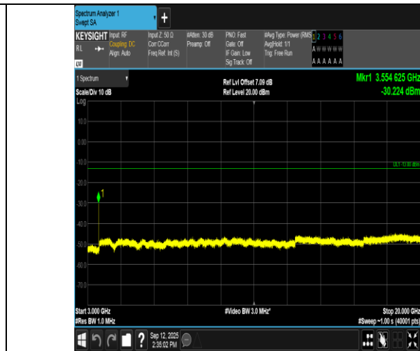
Band66-3MHz-16QAM-132657-1RB#0-3000~20000-PASS
