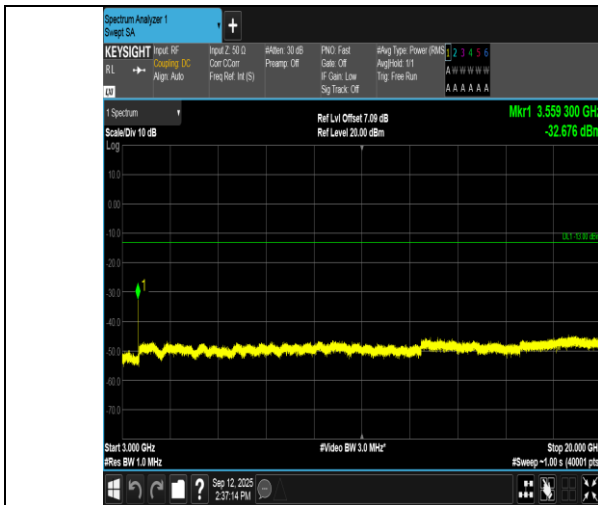
Band66-3MHz-16QAM-132657-1RB#14-3000~20000-PASS
