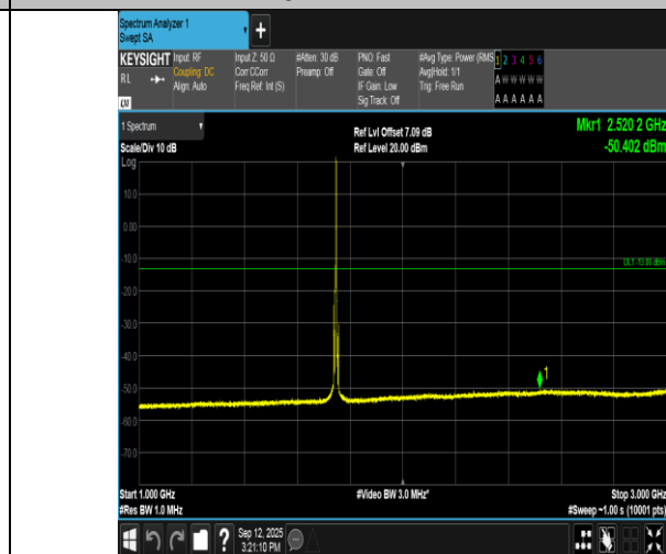
Band66-5MHz-16QAM-132322-1RB#24-1000~3000-PASS
