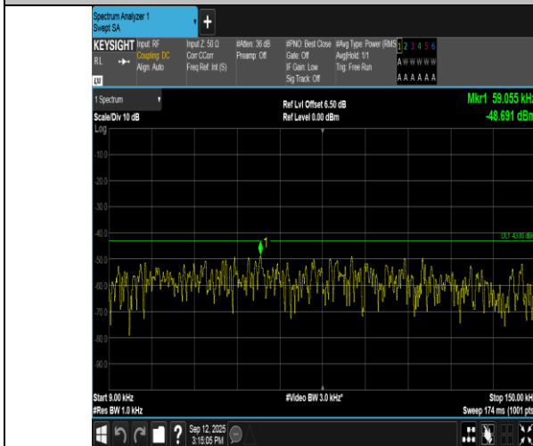
Band66-5MHz-QPSK-131997-25RB#0-0.009~0.15-PASS
