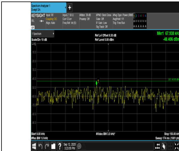
Band66-5MHz-QPSK-132647-1RB#0-0.009~0.15-PASS
