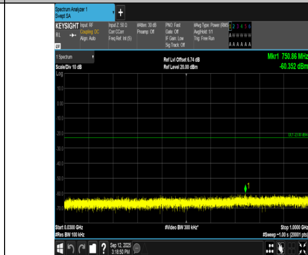
Band66-5MHz-16QAM-132322-1RB#0-30~1000-PASS
