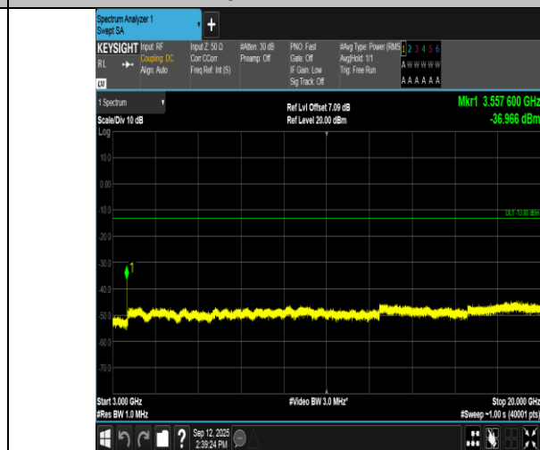
Band66-3MHz-16QAM-132657-15RB#0-3000~20000-PASS
