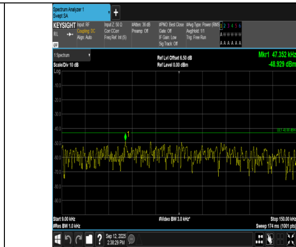
Band66-3MHz-16QAM-132657-15RB#0-0.009~0.15-PASS
