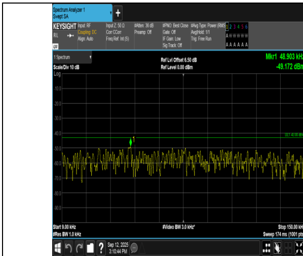
Band66-5MHz-QPSK-131997-1RB#0-0.009~0.15-PASS
