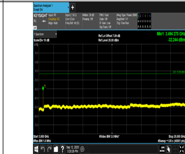
Band66-5MHz-QPSK-132322-1RB#24-3000~20000-PASS
