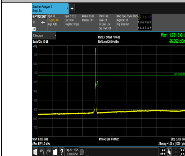
Band66-3MHz-16QAM-132657-15RB#0-1000~3000-PASS
