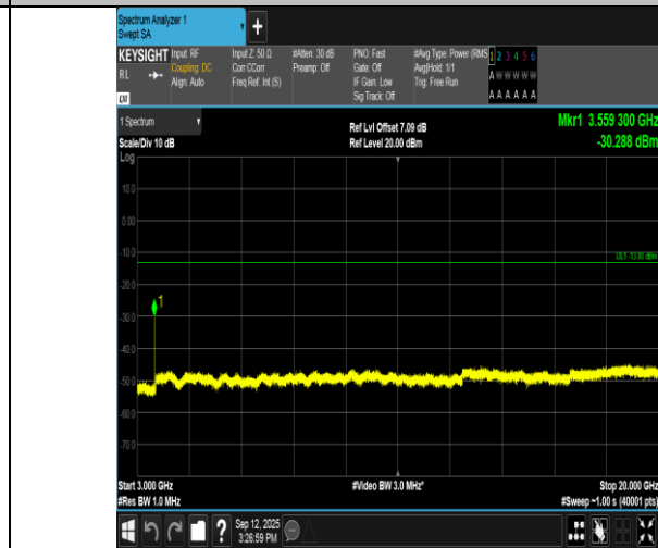
Band66-5MHz-QPSK-132647-1RB#24-3000~20000-PASS
