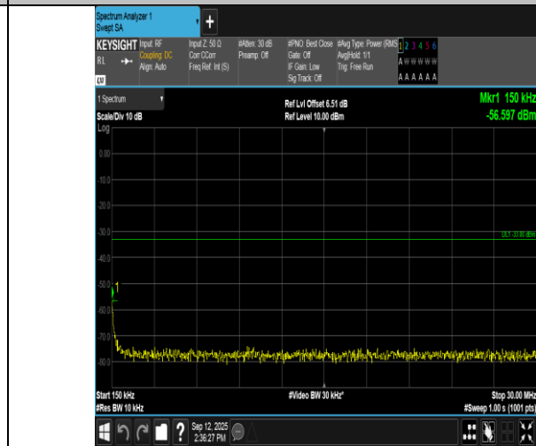
Band66-3MHz-16QAM-132657-1RB#14-0.15~30-PASS
