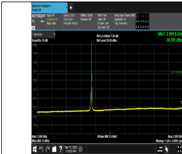
Band66-5MHz-16QAM-132322-1RB#0-1000~3000-PASS
