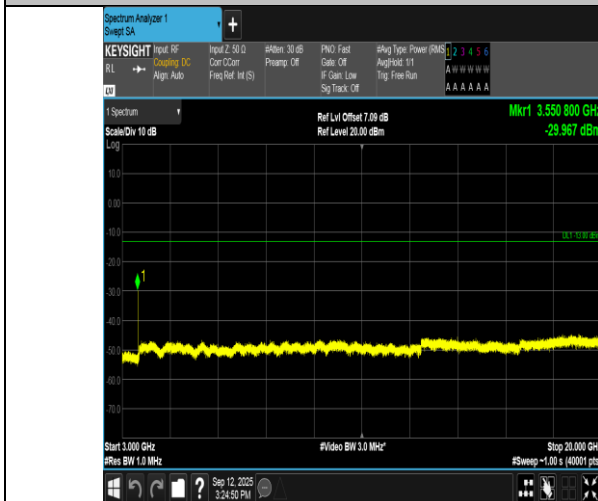
Band66-5MHz-QPSK-132647-1RB#0-3000~20000-PASS
