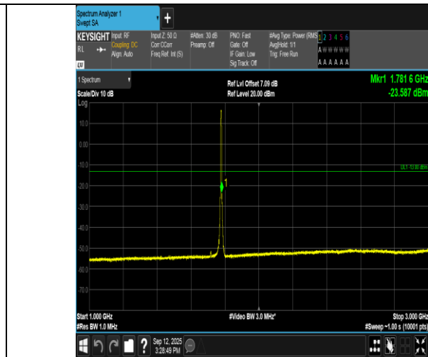
Band66-5MHz-QPSK-132647-25RB#0-1000~3000-PASS
