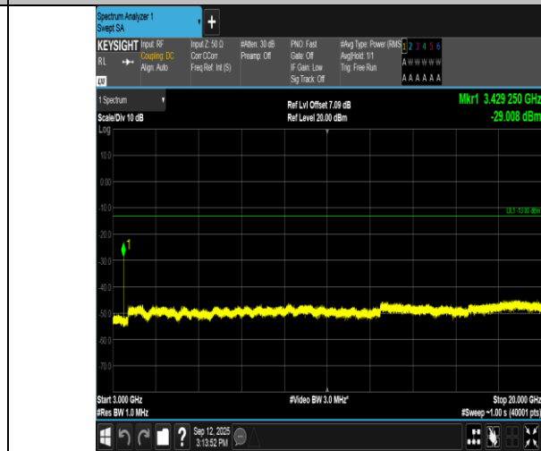
Band66-5MHz-QPSK-131997-1RB#24-3000~20000-PASS
