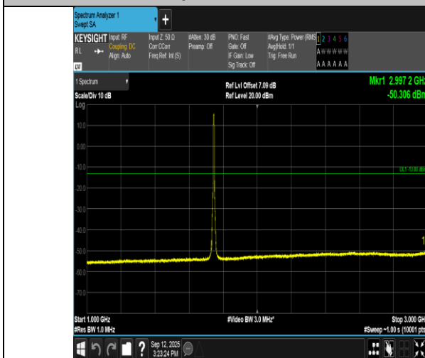
Band66-5MHz-16QAM-132322-25RB#0-1000~3000-PASS
