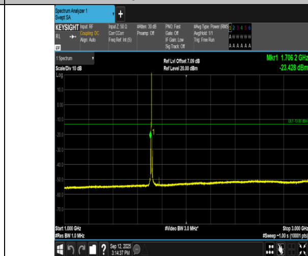
Band66-5MHz-16QAM-131997-1RB#24-1000~3000-PASS
