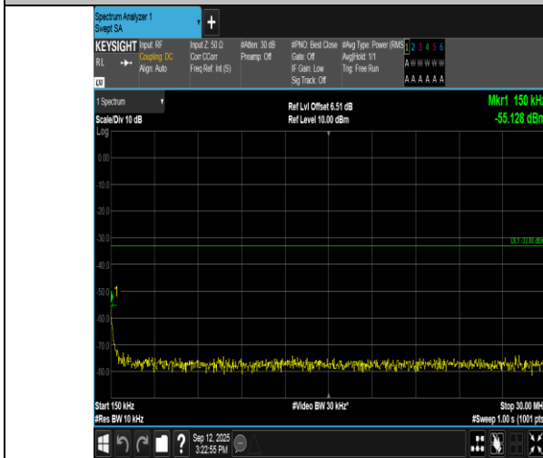
Band66-5MHz-16QAM-132322-25RB#0-0.15~30-PASS
