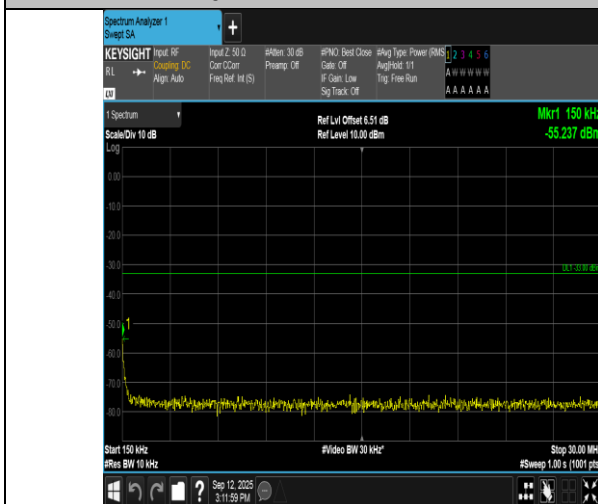
Band66-5MHz-16QAM-131997-1RB#0-0.15~30-PASS
