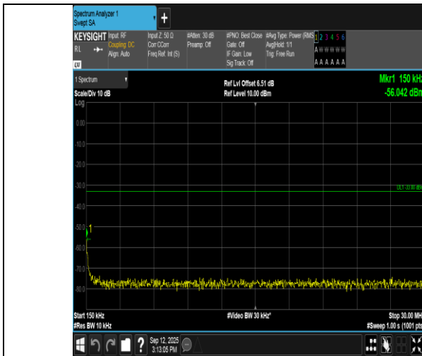
Band66-5MHz-QPSK-131997-1RB#24-0.15~30-PASS
