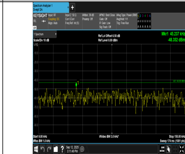
Band66-5MHz-16QAM-131997-1RB#0-0.009~0.15-PASS
