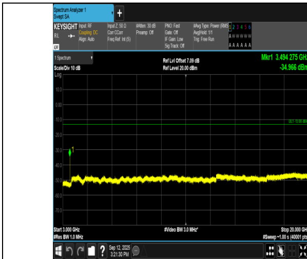
Band66-5MHz-16QAM-132322-1RB#24-3000~20000-PASS
