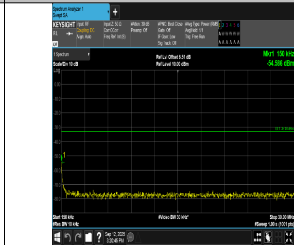
Band66-5MHz-16QAM-132322-1RB#24-0.15~30-PASS
