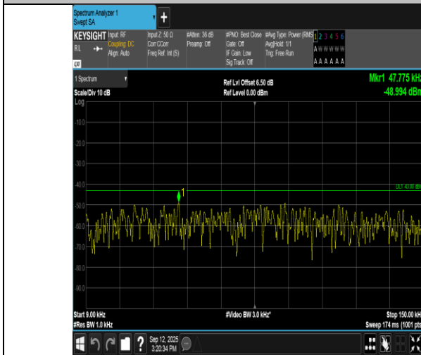
Band66-5MHz-16QAM-132322-1RB#24-0.009~0.15-PASS
