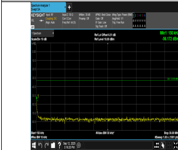
Band66-5MHz-16QAM-131997-25RB#0-0.15~30-PASS
