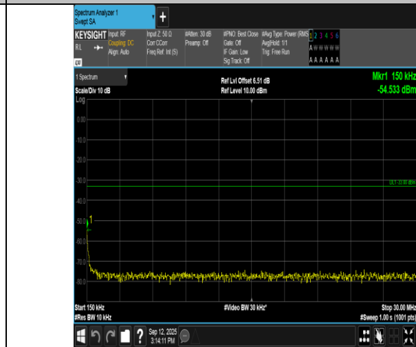
Band66-5MHz-16QAM-131997-1RB#24-0.15~30-PASS
