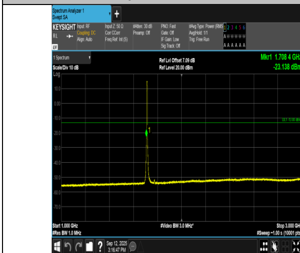
Band66-5MHz-16QAM-131997-25RB#0-1000~3000-PASS
