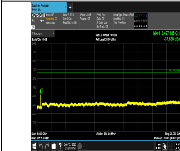
Band66-5MHz-QPSK-131997-25RB#0-3000~20000-PASS
