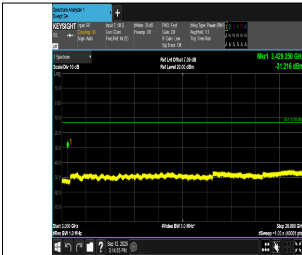
Band66-5MHz-16QAM-131997-1RB#24-3000~20000-PASS
