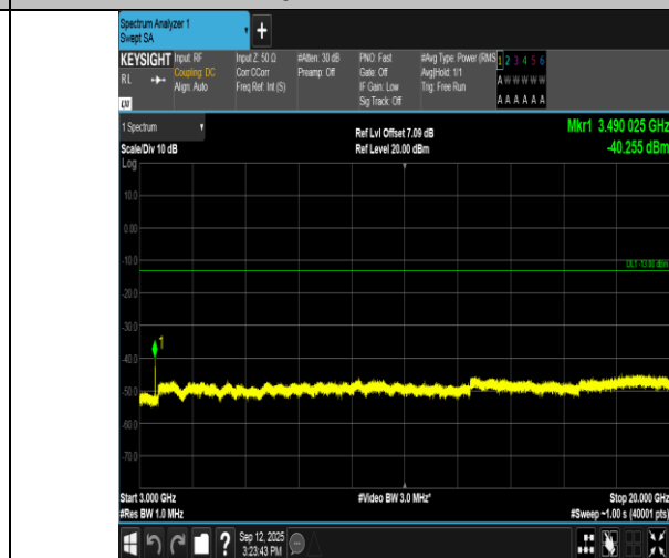
Band66-5MHz-16QAM-132322-25RB#0-3000~20000-PASS
