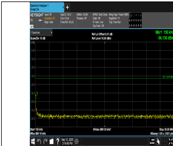
Band66-5MHz-QPSK-132322-1RB#24-0.15~30-PASS
