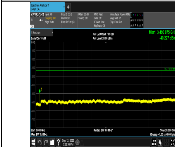
Band66-5MHz-QPSK-132322-25RB#0-3000~20000-PASS
