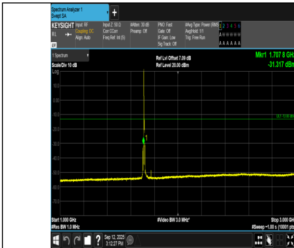
Band66-5MHz-16QAM-131997-1RB#0-1000~3000-PASS
