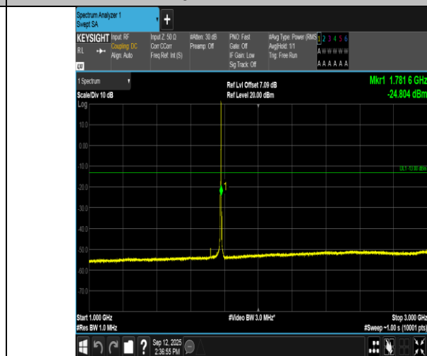
Band66-3MHz-16QAM-132657-1RB#14-1000~3000-PASS
