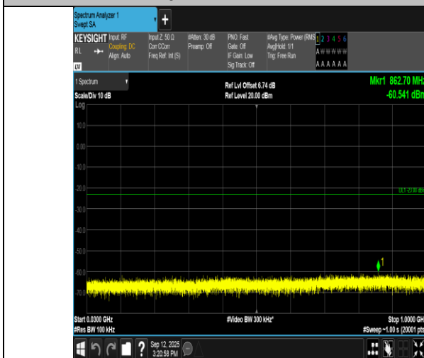
Band66-5MHz-16QAM-132322-1RB#24-30~1000-PASS
