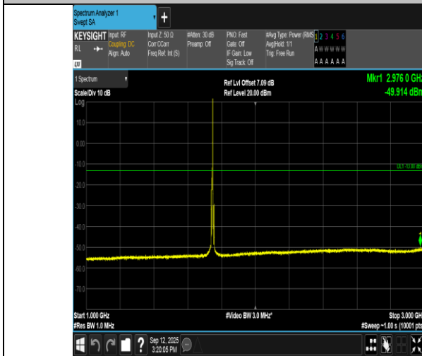
Band66-5MHz-QPSK-132322-1RB#24-1000~3000-PASS
