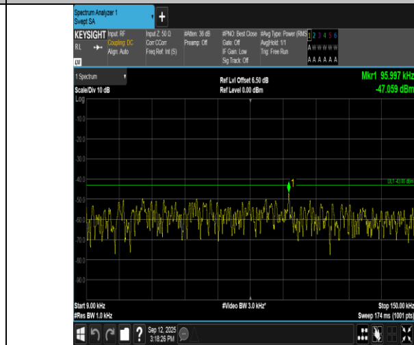
Band66-5MHz-16QAM-132322-1RB#0-0.009~0.15-PASS
