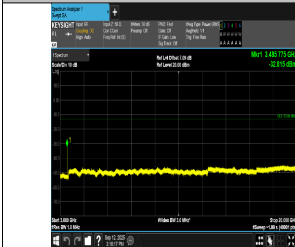
Band66-5MHz-QPSK-132322-1RB#0-3000~20000-PASS
