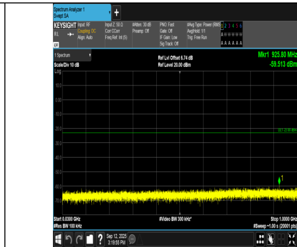
Band66-5MHz-QPSK-132322-1RB#24-30~1000-PASS
