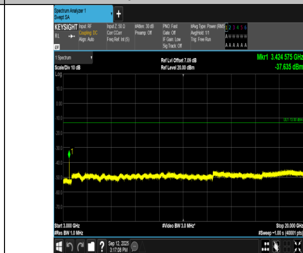
Band66-5MHz-16QAM-131997-25RB#0-3000~20000-PASS
