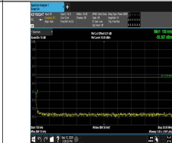
Band66-5MHz-QPSK-132647-25RB#0-0.15~30-PASS
