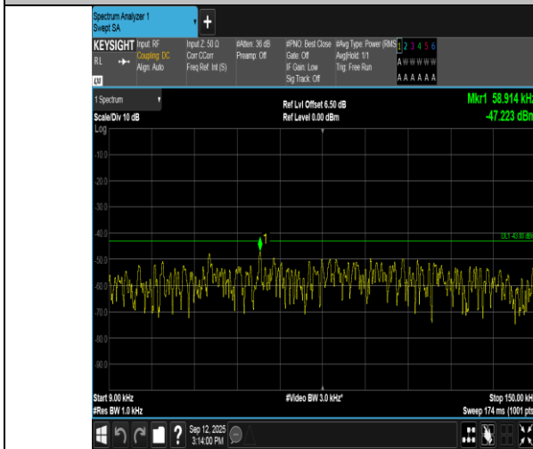
Band66-5MHz-16QAM-131997-1RB#24-0.009~0.15-PASS
