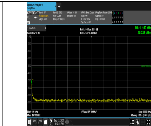
Band66-5MHz-QPSK-131997-1RB#0-0.15~30-PASS
