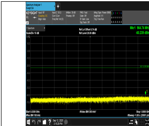
Band66-5MHz-QPSK-131997-25RB#0-30~1000-PASS
