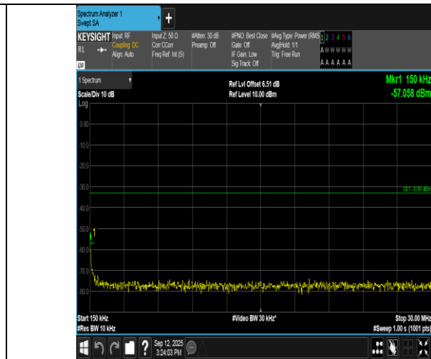
Band66-5MHz-QPSK-132647-1RB#0-0.15~30-PASS
