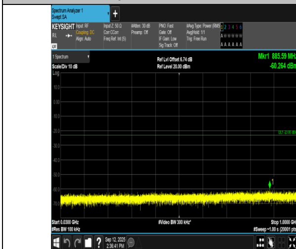
Band66-3MHz-16QAM-132657-1RB#14-30~1000-PASS
