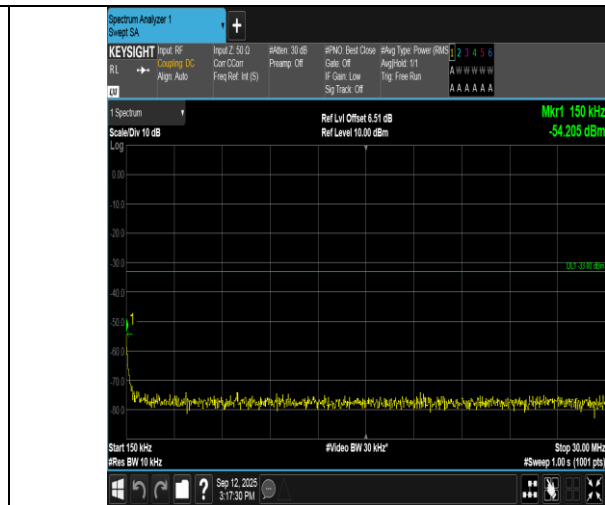
Band66-5MHz-QPSK-132322-1RB#0-0.15~30-PASS
