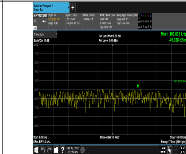
Band66-5MHz-QPSK-131997-1RB#24-0.009~0.15-PASS
