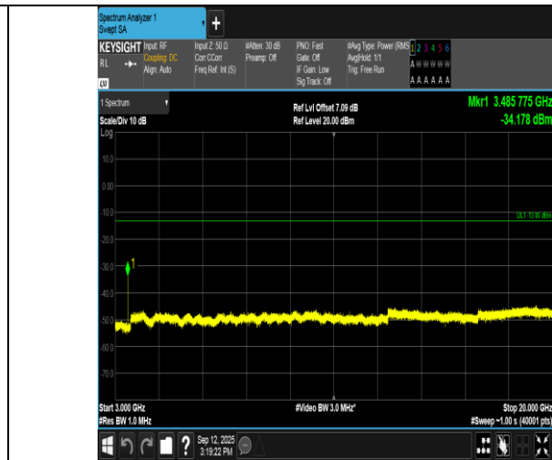
Band66-5MHz-16QAM-132322-1RB#0-3000~20000-PASS
