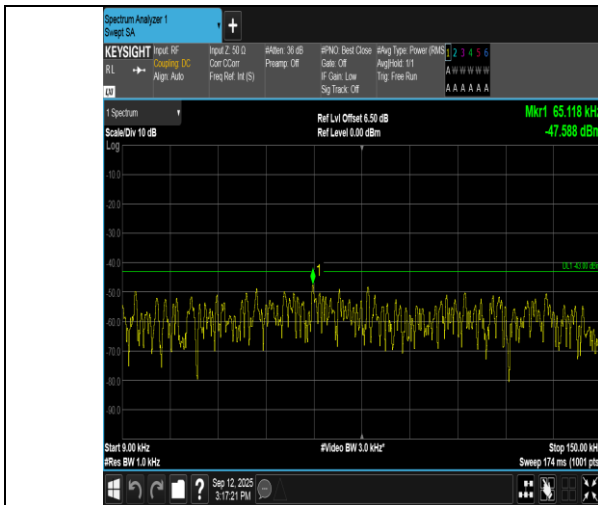
Band66-5MHz-QPSK-132322-1RB#0-0.009~0.15-PASS
