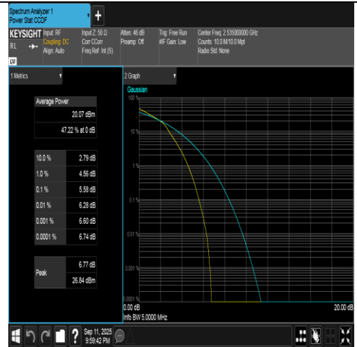
Band7-5MHz-16QAM-21100-25RB#0-PASS
