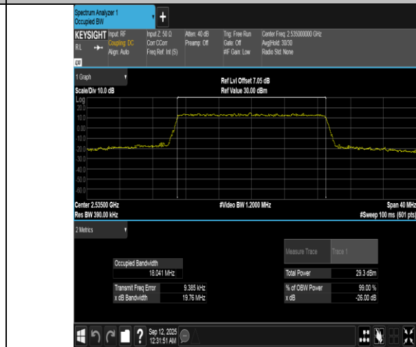
Band7-20MHz-16QAM-21100-100RB#0-PASS
