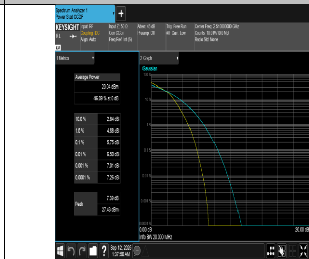
Band7-20MHz-16QAM-20850-100RB#0-PASS
