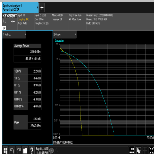
Band7-10MHz-QPSK-21100-1RB#0-PASS
