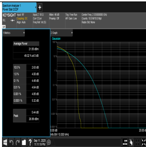
Band7-10MHz-16QAM-21100-1RB#0-PASS
