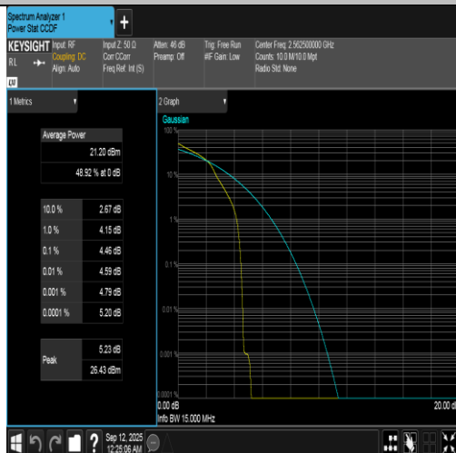
Band7-15MHz-16QAM-21375-1RB#0-PASS
