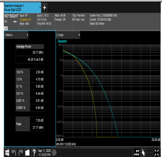
Band7-10MHz-16QAM-20800-50RB#0-PASS
