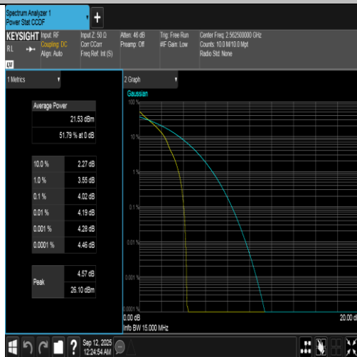
Band7-15MHz-QPSK-21375-1RB#0-PASS
