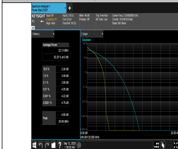
Band7-20MHz-QPSK-21100-1RB#0-PASS
