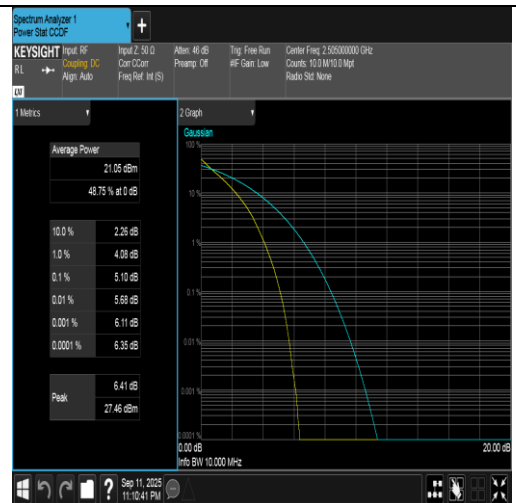
Band7-10MHz-QPSK-20800-50RB#0-PASS
