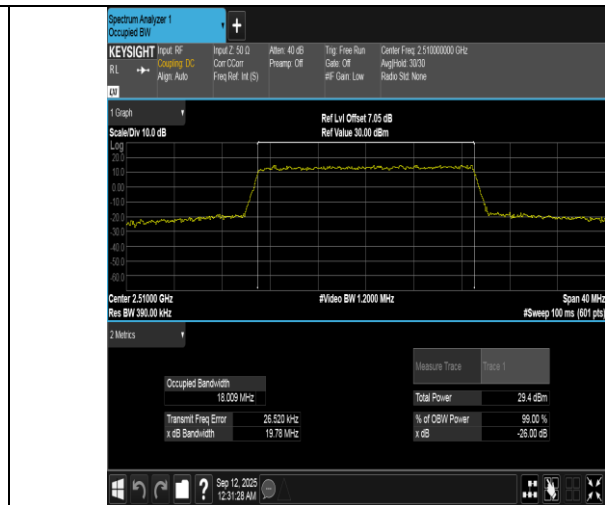
Band7-20MHz-16QAM-20850-100RB#0-PASS
