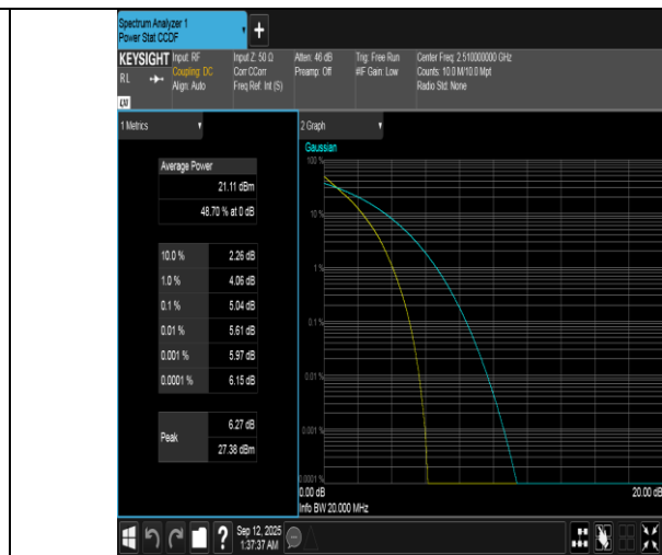
Band7-20MHz-QPSK-20850-100RB#0-PASS
