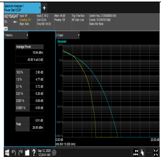
Band7-15MHz-16QAM-21100-75RB#0-PASS
