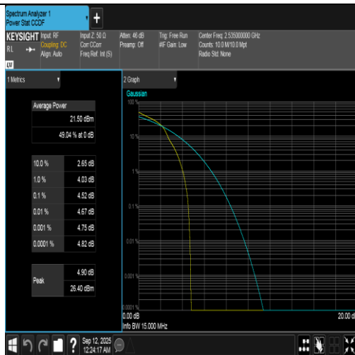
Band7-15MHz-16QAM-21100-1RB#0-PASS
