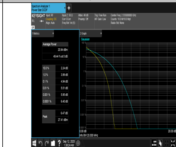
Band7-20MHz-QPSK-21100-100RB#0-PASS
