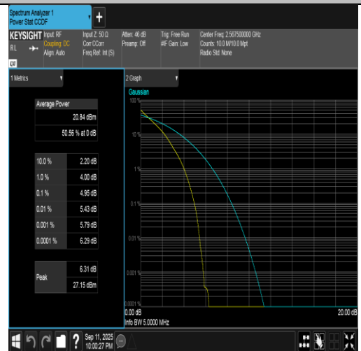
Band7-5MHz-QPSK-21425-25RB#0-PASS
