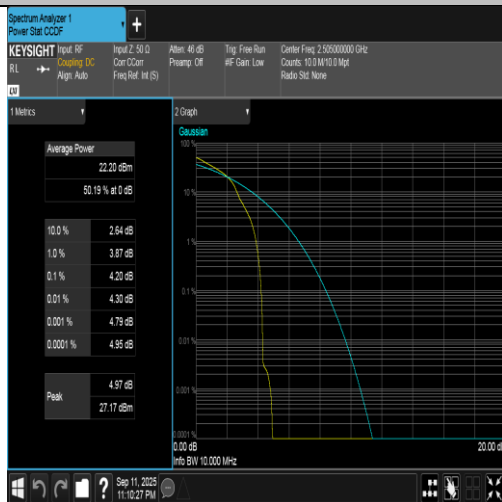
Band7-10MHz-16QAM-20800-1RB#0-PASS
