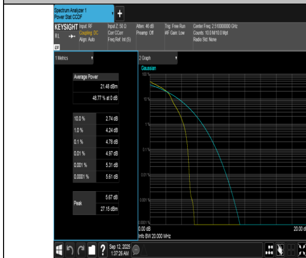
Band7-20MHz-16QAM-20850-1RB#0-PASS
