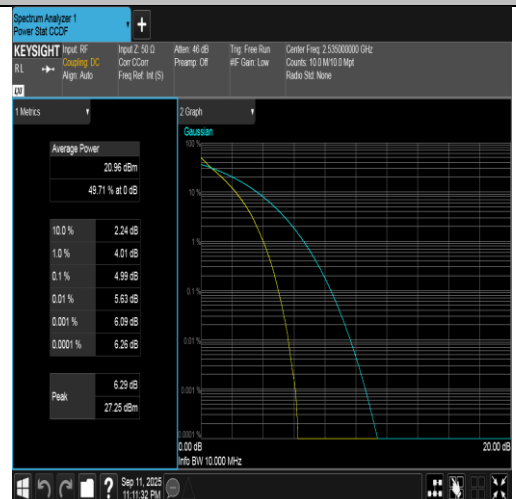
Band7-10MHz-QPSK-21100-50RB#0-PASS
