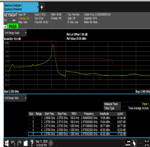
Band7-5MHz-QPSK-21425-1RB#24-PASS
