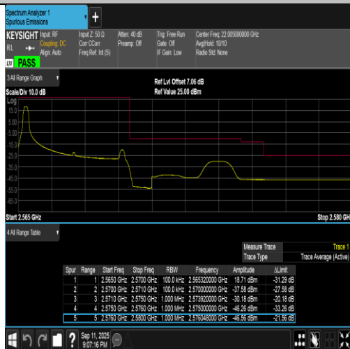
Band7-5MHz-QPSK-21425-1RB#0-PASS
