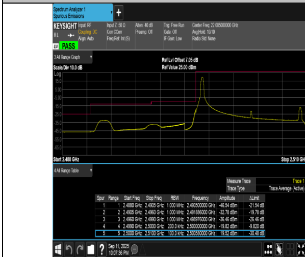
Band7-10MHz-QPSK-20800-1RB#0-PASS
