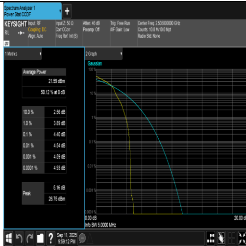
Band7-5MHz-16QAM-21100-1RB#0-PASS
