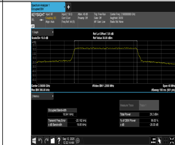
Band7-20MHz-16QAM-21350-100RB#0-PASS
