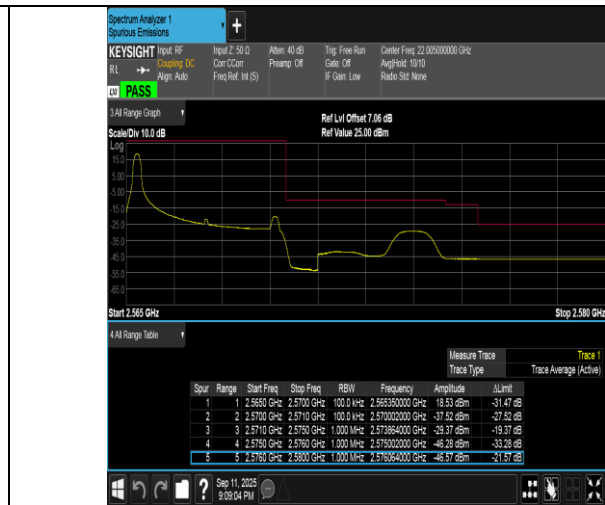
Band7-5MHz-16QAM-21425-1RB#0-PASS
