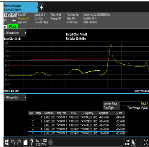
Band7-5MHz-16QAM-20775-1RB#0-PASS
