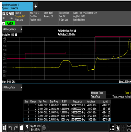
Band7-5MHz-16QAM-20775-1RB#24-PASS
