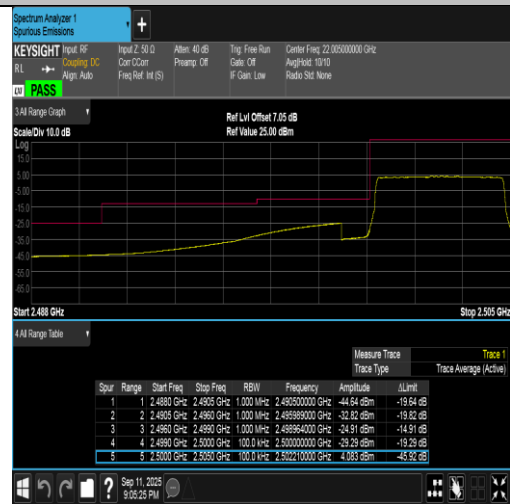
Band7-5MHz-16QAM-20775-25RB#0-PASS
