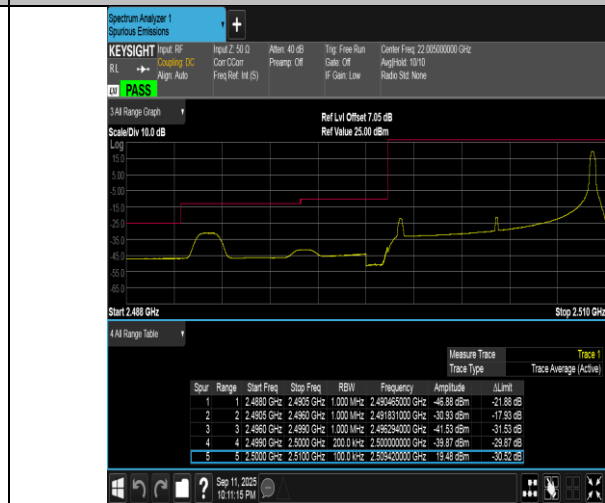
Band7-10MHz-QPSK-20800-1RB#49-PASS
