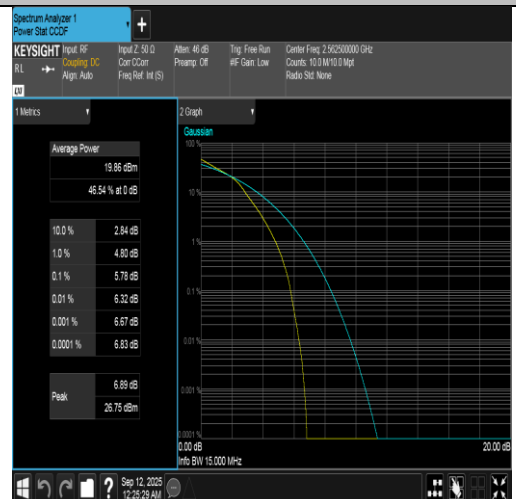
Band7-15MHz-16QAM-21375-75RB#0-PASS
