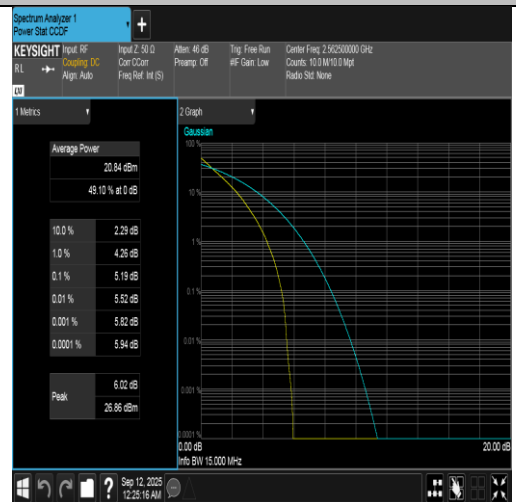
Band7-15MHz-QPSK-21375-75RB#0-PASS
