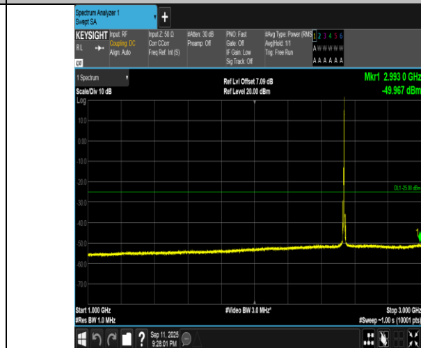
Band7-5MHz-QPSK-21100-1RB#24-1000~3000-PASS
