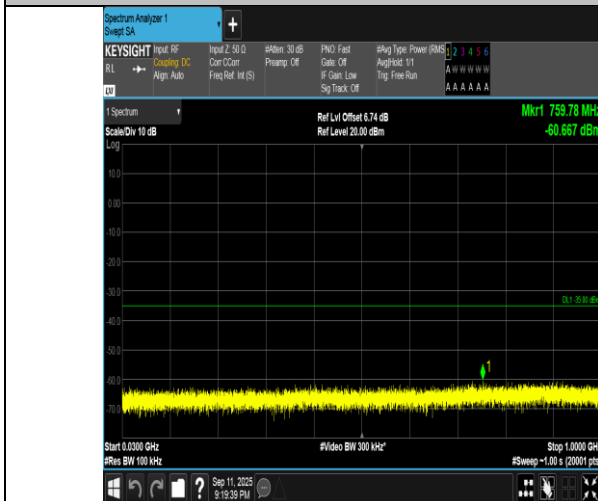
Band7-5MHz-QPSK-20775-1RB#24-30~1000-PASS
