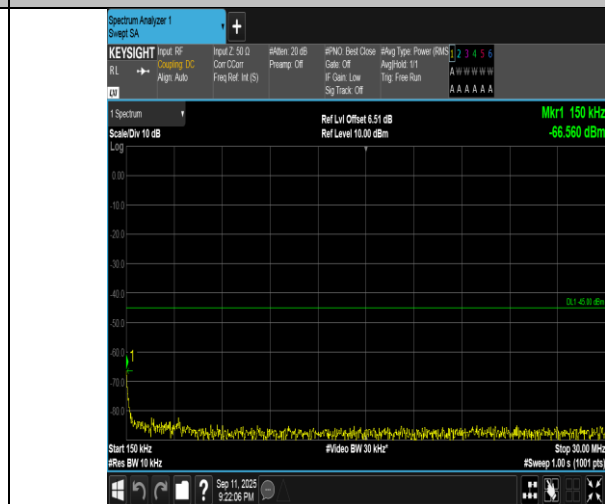
Band7-5MHz-QPSK-20775-25RB#0-0.15~30-PASS
