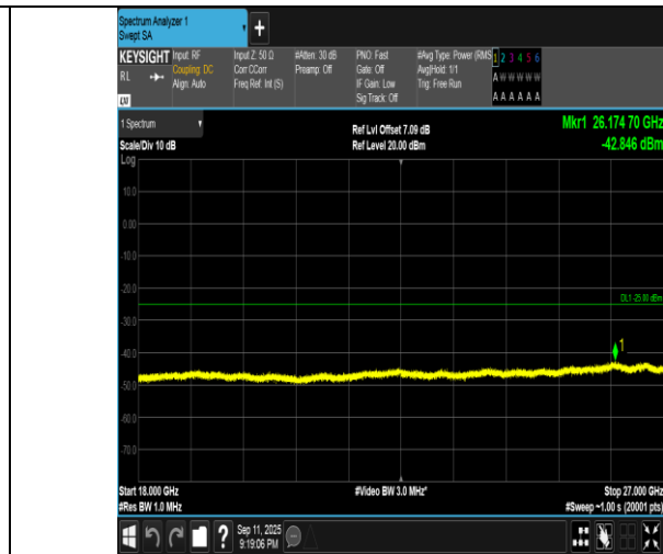
Band7-5MHz-16QAM-20775-1RB#0-18000~27000-PASS
