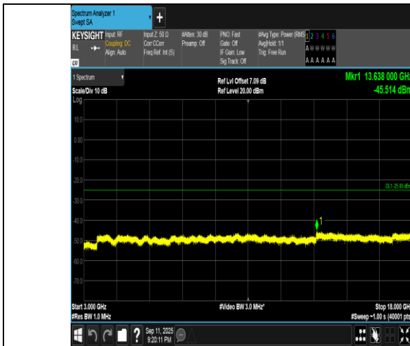
Band7-5MHz-QPSK-20775-1RB#24-3000~18000-PASS
