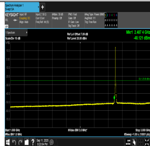
Band7-5MHz-16QAM-20775-25RB#0-1000~3000-PASS
