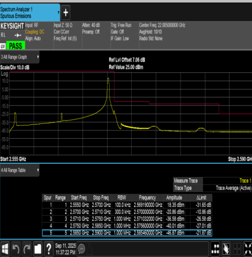
Band7-15MHz-16QAM-21375-1RB#74-PASS
