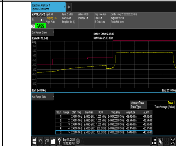
Band7-10MHz-16QAM-20800-50RB#0-PASS
