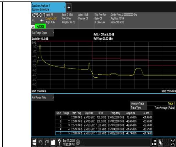
Band7-10MHz-16QAM-21400-1RB#0-PASS
