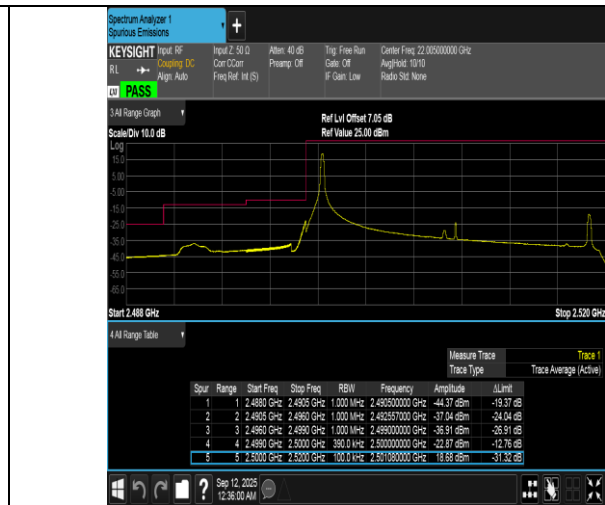
Band7-20MHz-16QAM-20850-1RB#0-PASS
