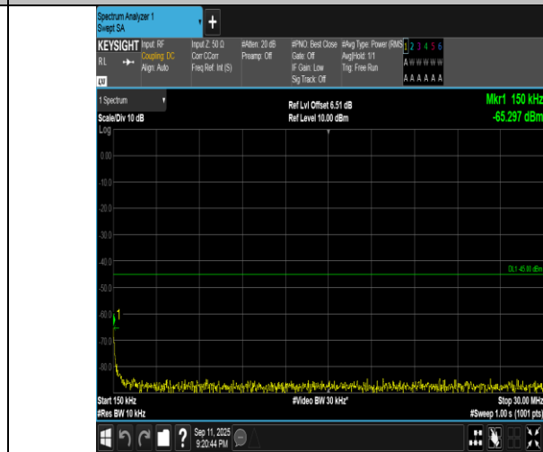
Band7-5MHz-16QAM-20775-1RB#24-0.15~30-PASS
