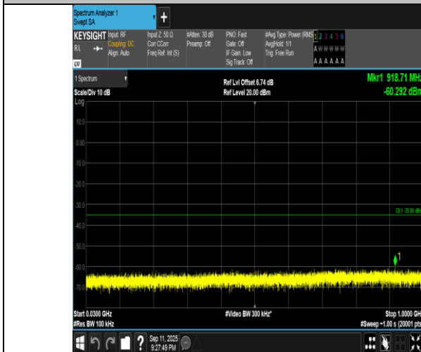
Band7-5MHz-QPSK-21100-1RB#24-30~1000-PASS
