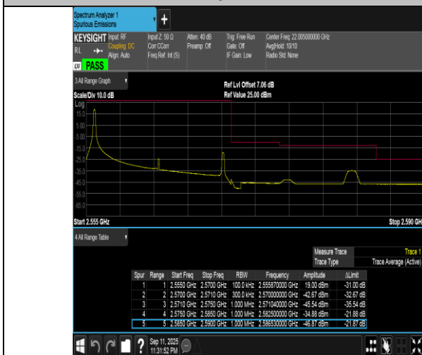
Band7-15MHz-QPSK-21375-1RB#0-PASS
