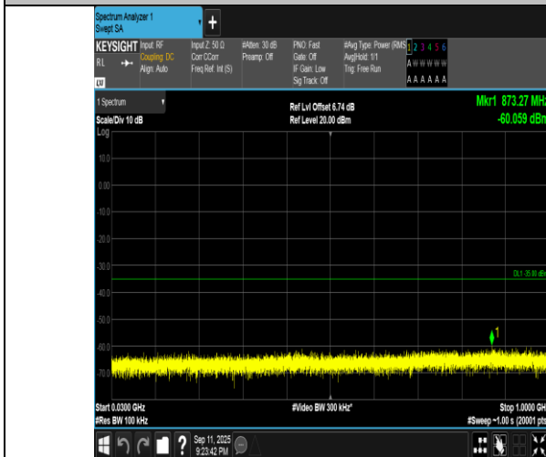
Band7-5MHz-16QAM-20775-25RB#0-30~1000-PASS
