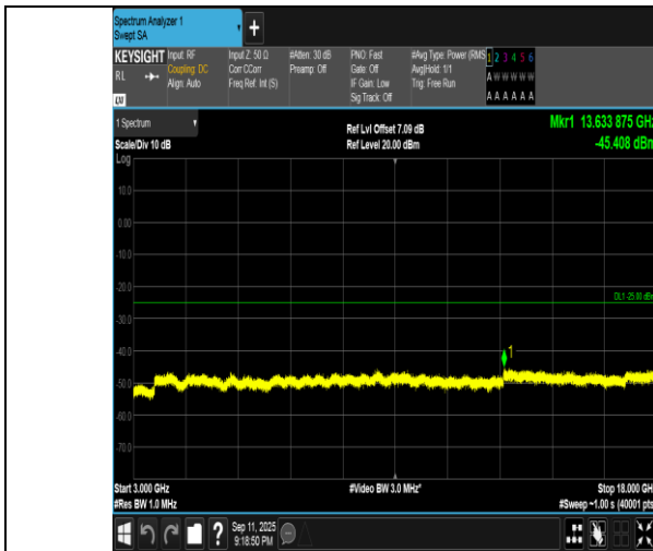
Band7-5MHz-16QAM-20775-1RB#0-3000~18000-PASS
