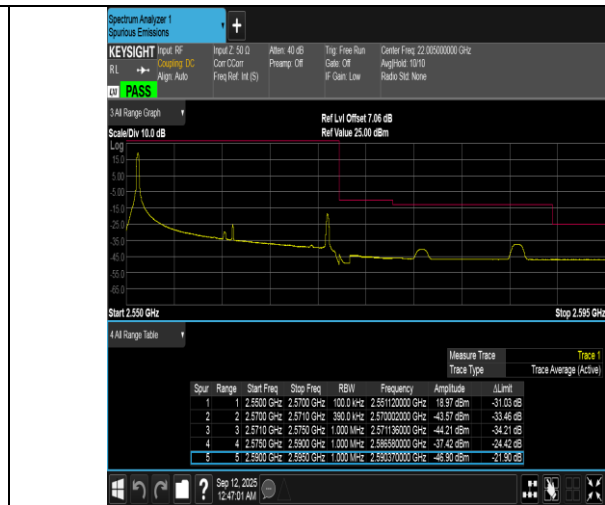
Band7-20MHz-16QAM-21350-1RB#0-PASS
