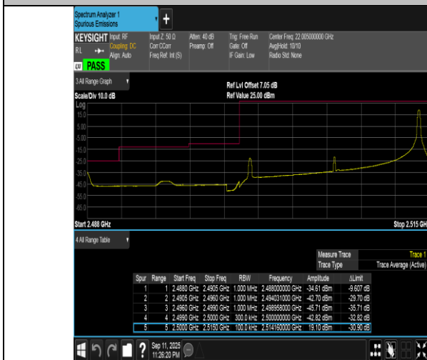
Band7-15MHz-16QAM-20825-1RB#74-PASS
