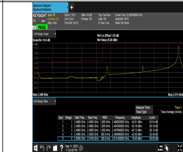
Band7-15MHz-QPSK-20825-1RB#74-PASS
