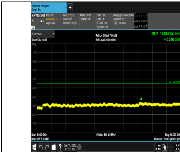
Band7-5MHz-QPSK-20775-1RB#0-3000~18000-PASS
