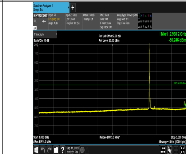
Band7-5MHz-QPSK-20775-1RB#24-1000~3000-PASS
