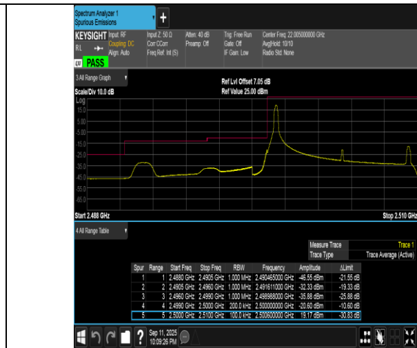
Band7-10MHz-16QAM-20800-1RB#0-PASS
