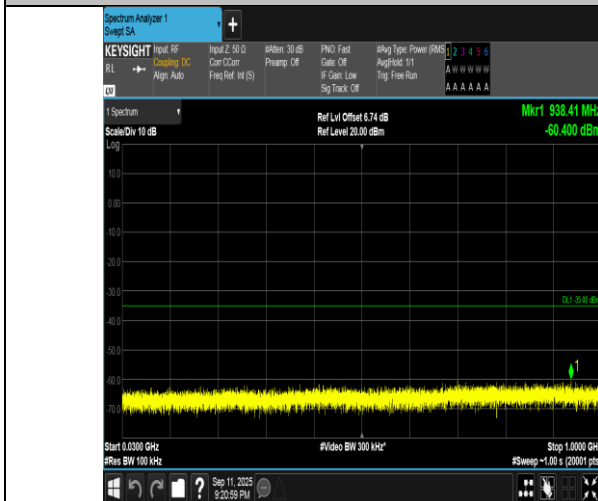
Band7-5MHz-16QAM-20775-1RB#24-30~1000-PASS
