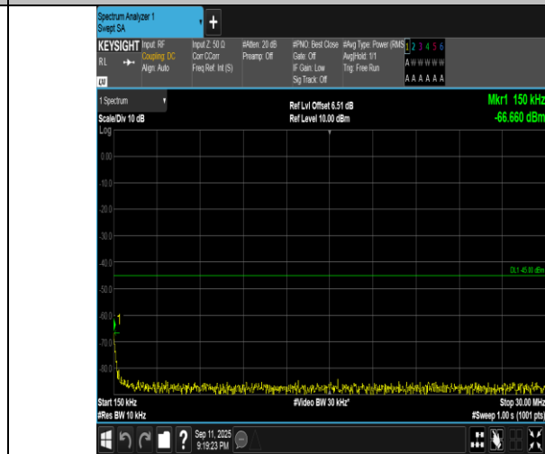
Band7-5MHz-QPSK-20775-1RB#24-0.15~30-PASS
