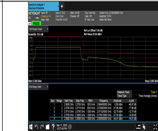
Band7-10MHz-16QAM-21400-50RB#0-PASS
