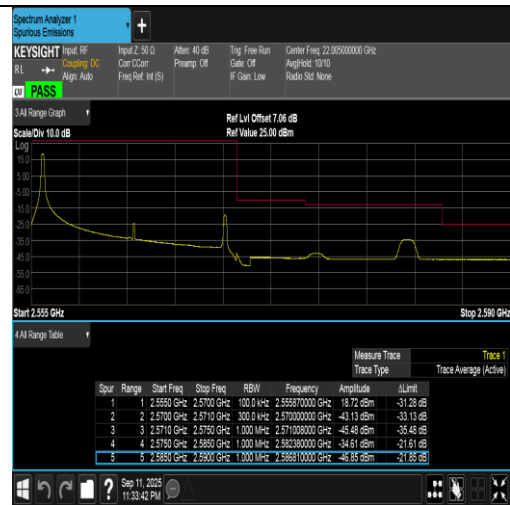
Band7-15MHz-16QAM-21375-1RB#0-PASS
