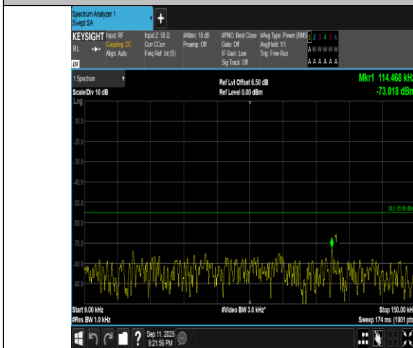
Band7-5MHz-QPSK-20775-25RB#0-0.009~0.15-PASS
