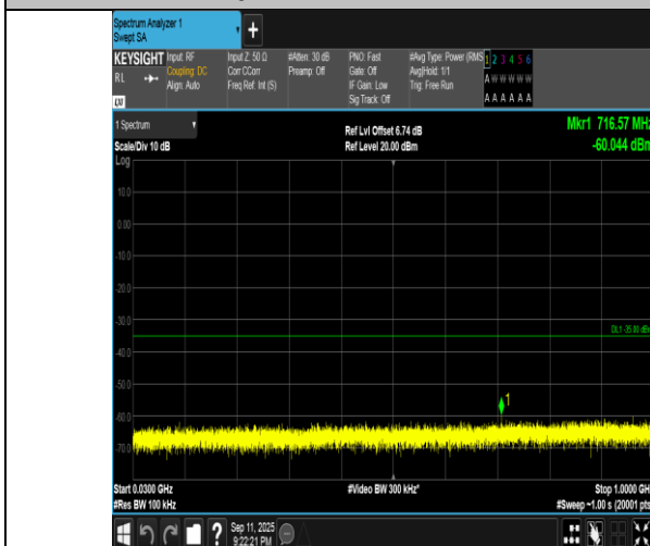
Band7-5MHz-QPSK-20775-25RB#0-30~1000-PASS
