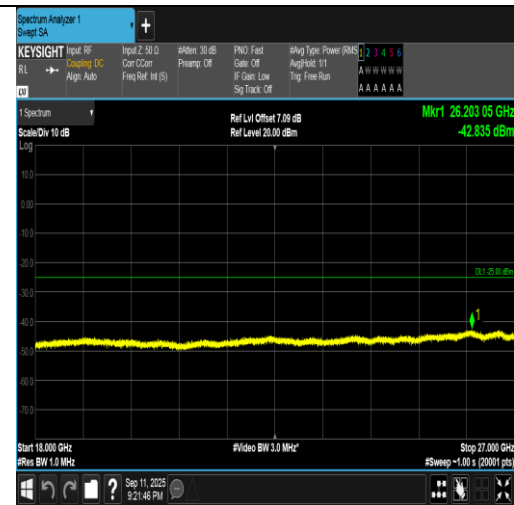
Band7-5MHz-16QAM-20775-1RB#24-18000~27000-PASS
