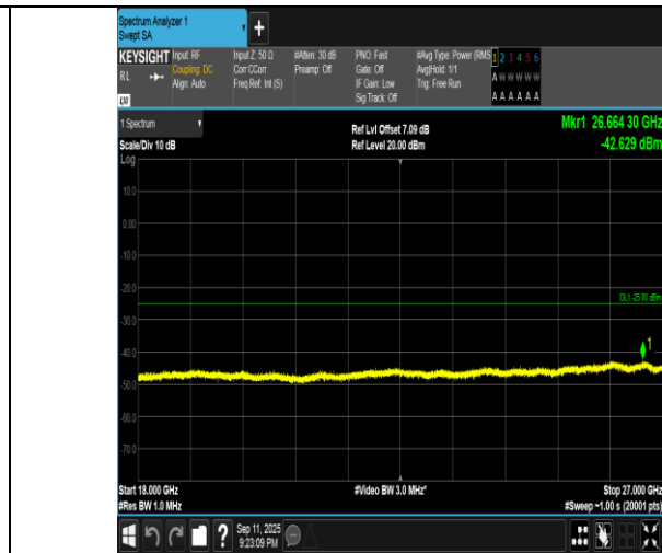
Band7-5MHz-QPSK-20775-25RB#0-18000~27000-PASS
