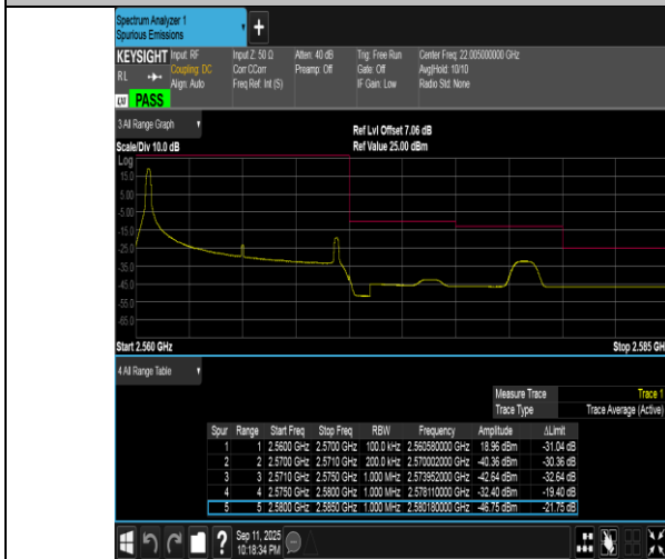
Band7-10MHz-QPSK-21400-1RB#0-PASS
