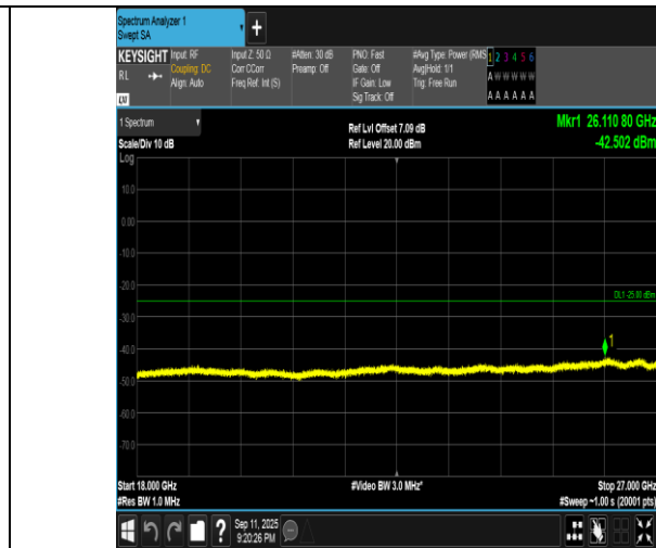
Band7-5MHz-QPSK-20775-1RB#24-18000~27000-PASS
