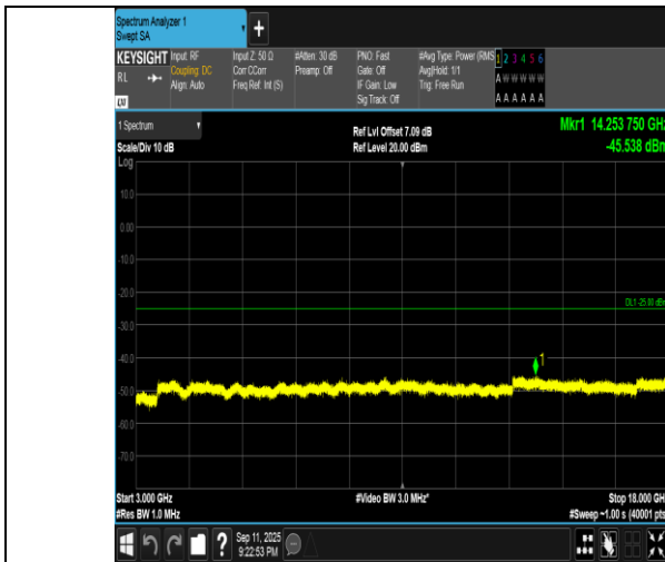
Band7-5MHz-QPSK-20775-25RB#0-3000~18000-PASS
