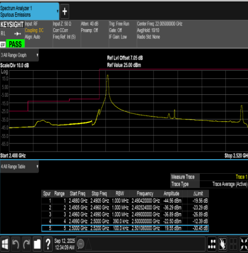
Band7-20MHz-QPSK-20850-1RB#0-PASS
