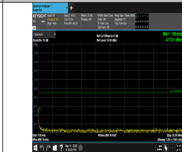
Band7-5MHz-16QAM-20775-1RB#0-0.15~30-PASS
