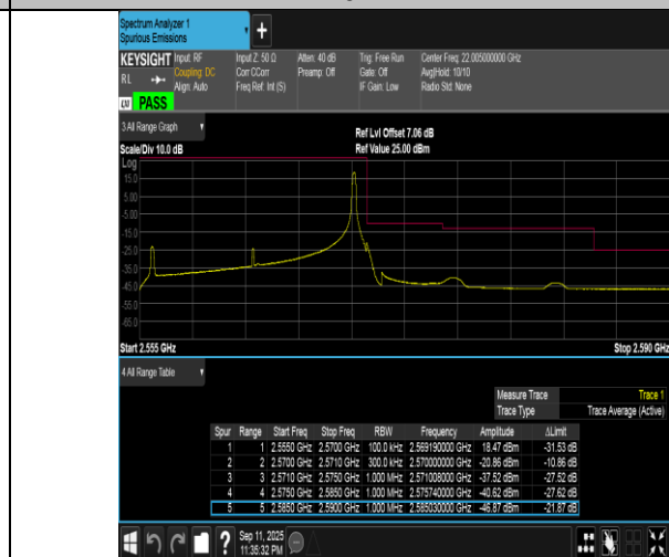
Band7-15MHz-QPSK-21375-1RB#74-PASS
