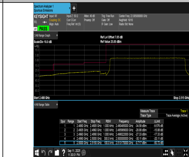
Band7-15MHz-16QAM-20825-75RB#0-PASS
