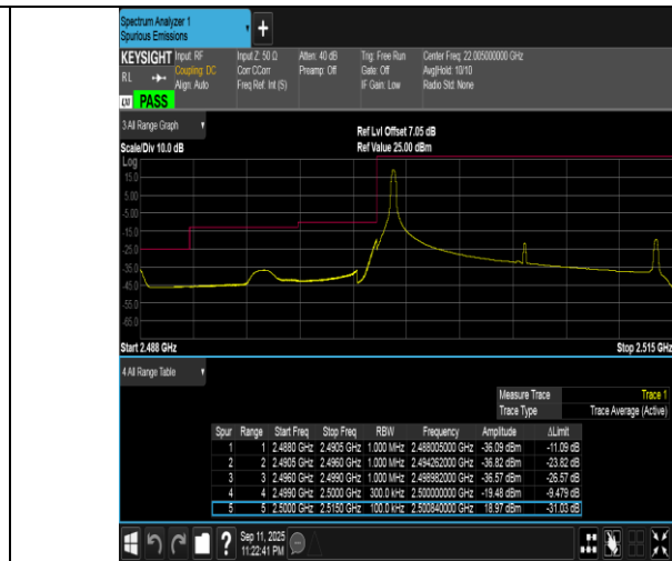
Band7-15MHz-16QAM-20825-1RB#0-PASS
