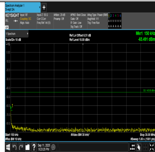
Band7-5MHz-16QAM-20775-25RB#0-0.15~30-PASS
