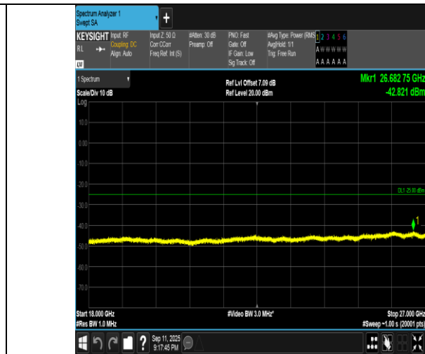
Band7-5MHz-QPSK-20775-1RB#0-18000~27000-PASS
