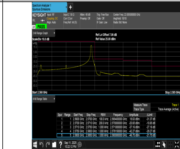
Band7-10MHz-QPSK-21400-1RB#49-PASS
