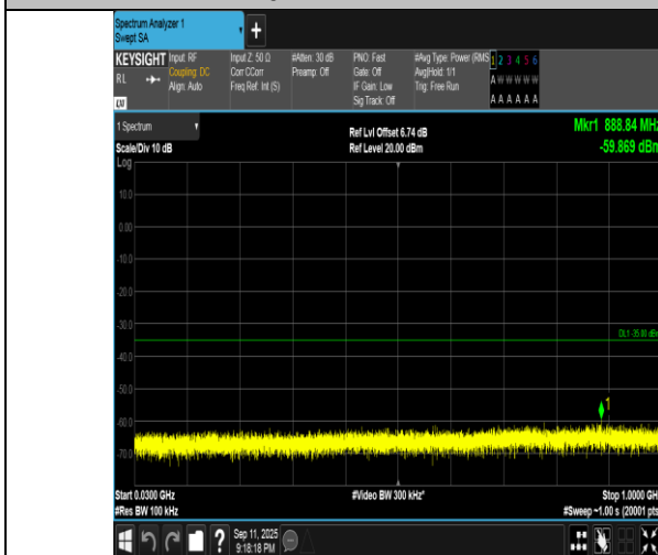
Band7-5MHz-16QAM-20775-1RB#0-30~1000-PASS
