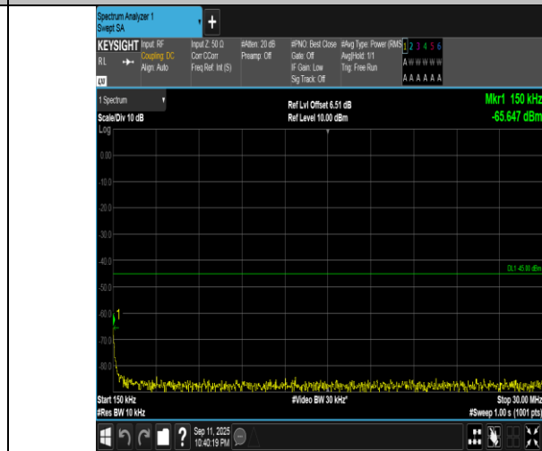
Band7-10MHz-16QAM-21100-1RB#49-0.15~30-PASS
