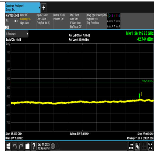
Band7-10MHz-16QAM-21400-1RB#49-18000~27000-PASS
