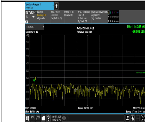
Band7-10MHz-16QAM-21100-1RB#49-0.009~0.15-PASS
