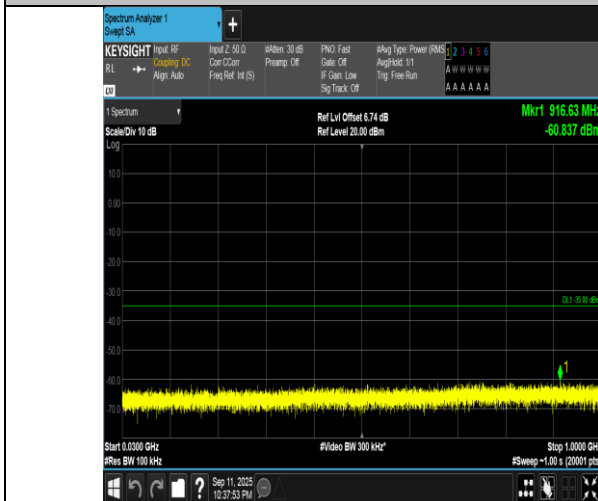
Band7-10MHz-16QAM-21100-1RB#0-30~1000-PASS
