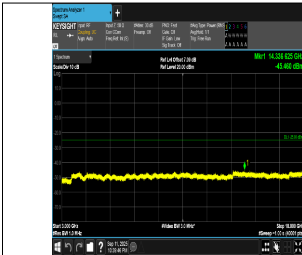
Band7-10MHz-QPSK-21100-1RB#49-3000~18000-PASS
