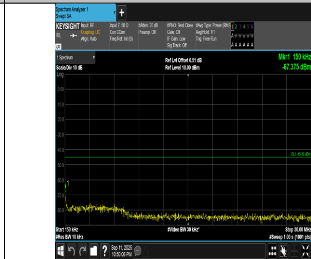
Band7-10MHz-QPSK-21400-50RB#0-0.15~30-PASS
