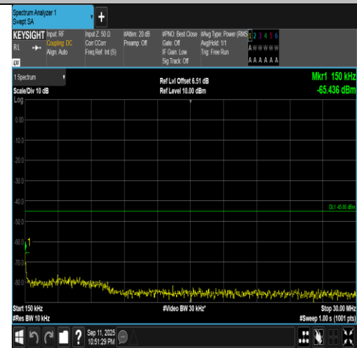
Band7-10MHz-16QAM-21400-50RB#0-0.15~30-PASS
