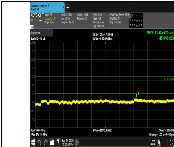
Band7-10MHz-QPSK-21400-50RB#0-3000~18000-PASS
