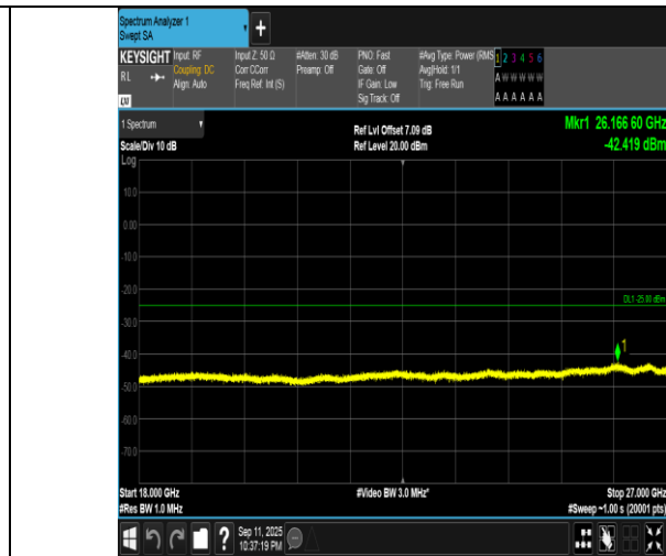
Band7-10MHz-QPSK-21100-1RB#0-18000~27000-PASS
