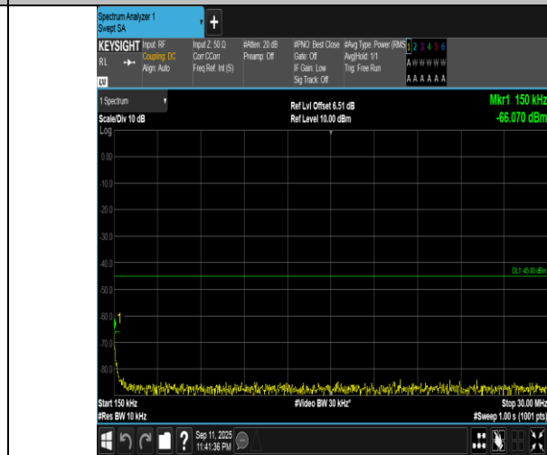
Band7-15MHz-QPSK-20825-1RB#0-0.15~30-PASS
