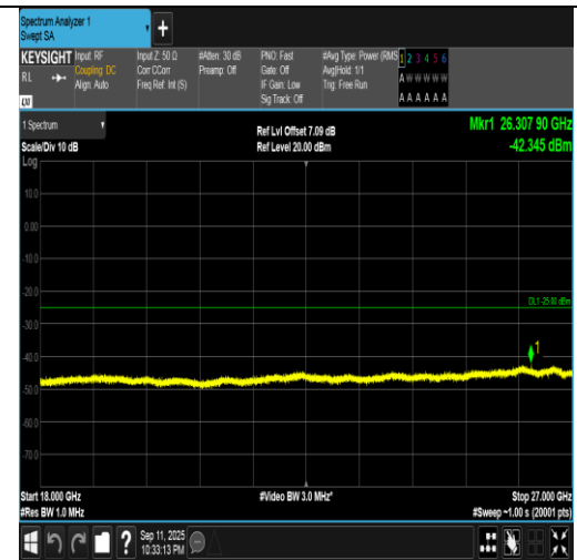
Band7-10MHz-16QAM-20800-1RB#49-18000~27000-PASS
