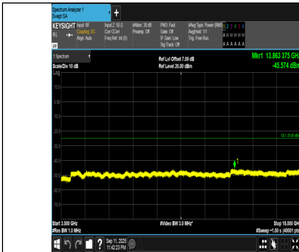
Band7-15MHz-QPSK-20825-1RB#0-3000~18000-PASS
