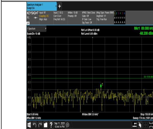
Band7-10MHz-QPSK-21400-1RB#0-0.009~0.15-PASS
