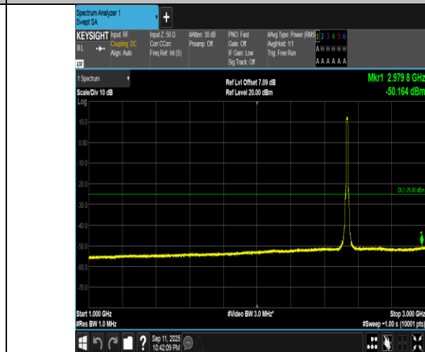
Band7-10MHz-QPSK-21100-50RB#0-1000~3000-PASS
