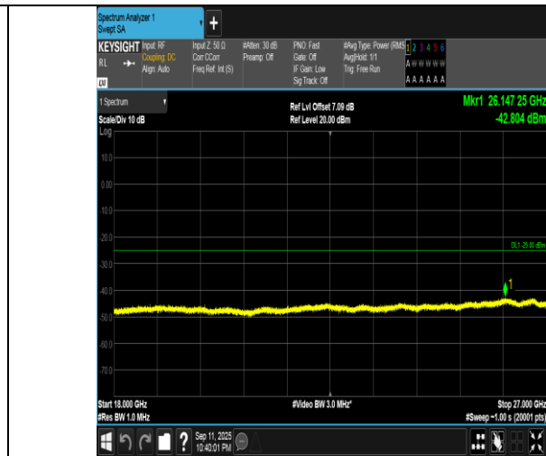
Band7-10MHz-QPSK-21100-1RB#49-18000~27000-PASS
