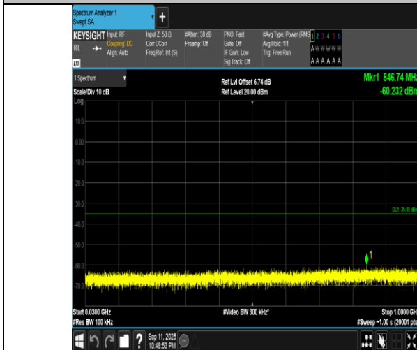
Band7-10MHz-16QAM-21400-1RB#49-30~1000-PASS
