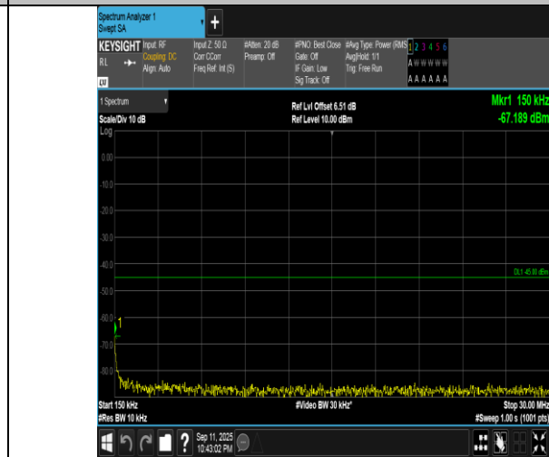
Band7-10MHz-16QAM-21100-50RB#0-0.15~30-PASS
