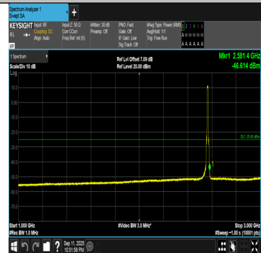
Band7-10MHz-16QAM-21400-50RB#0-1000~3000-PASS
