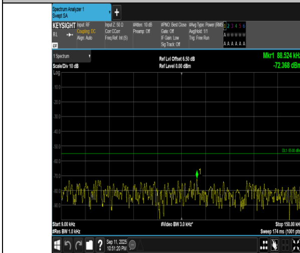
Band7-10MHz-16QAM-21400-50RB#0-0.009~0.15-PASS
