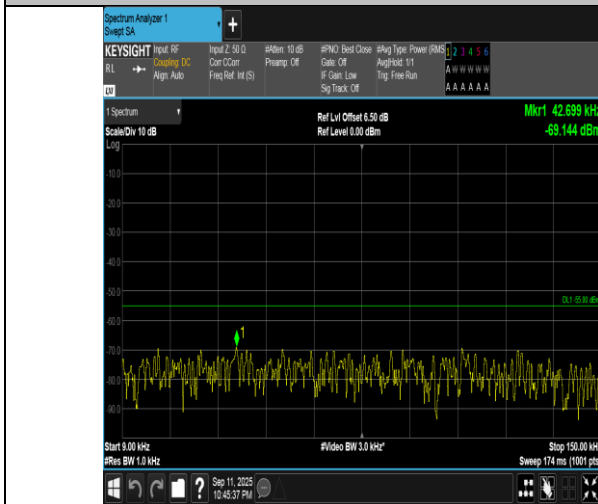
Band7-10MHz-16QAM-21400-1RB#0-0.009~0.15-PASS
