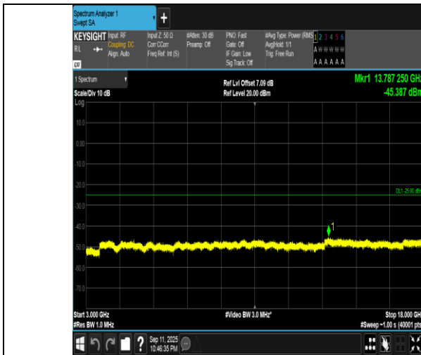
Band7-10MHz-16QAM-21400-1RB#0-3000~18000-PASS
