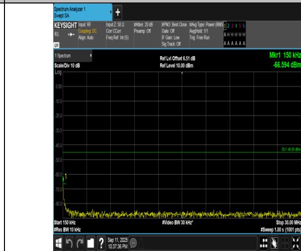
Band7-10MHz-16QAM-21100-1RB#0-0.15~30-PASS
