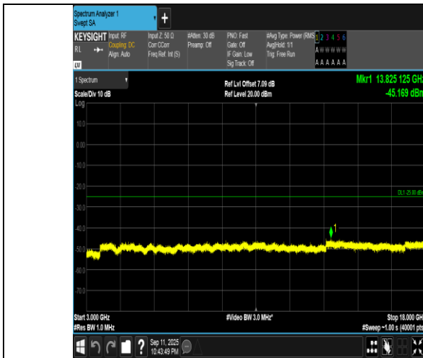
Band7-10MHz-16QAM-21100-50RB#0-3000~18000-PASS
