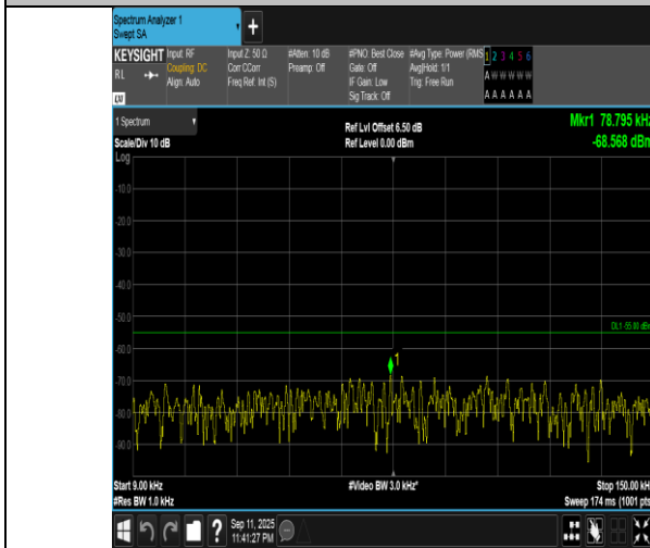
Band7-15MHz-QPSK-20825-1RB#0-0.009~0.15-PASS
