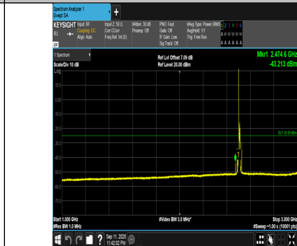
Band7-15MHz-QPSK-20825-1RB#0-1000~3000-PASS
