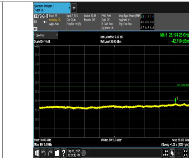
Band7-10MHz-QPSK-21400-50RB#0-18000~27000-PASS
