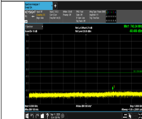
Band7-10MHz-QPSK-21100-50RB#0-30~1000-PASS
