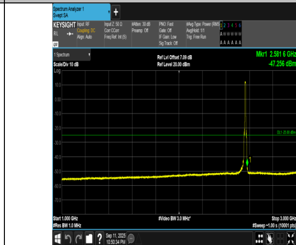
Band7-10MHz-QPSK-21400-50RB#0-1000~3000-PASS
