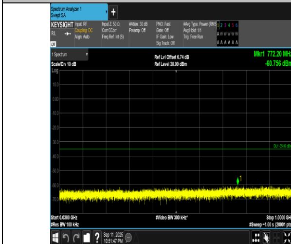
Band7-10MHz-16QAM-21400-50RB#0-30~1000-PASS
