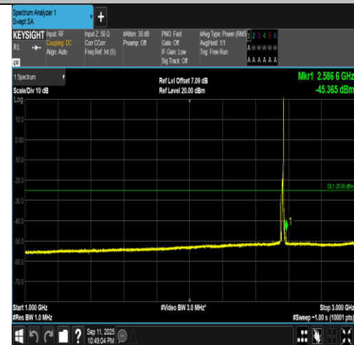
Band7-10MHz-16QAM-21400-1RB#49-1000~3000-PASS
