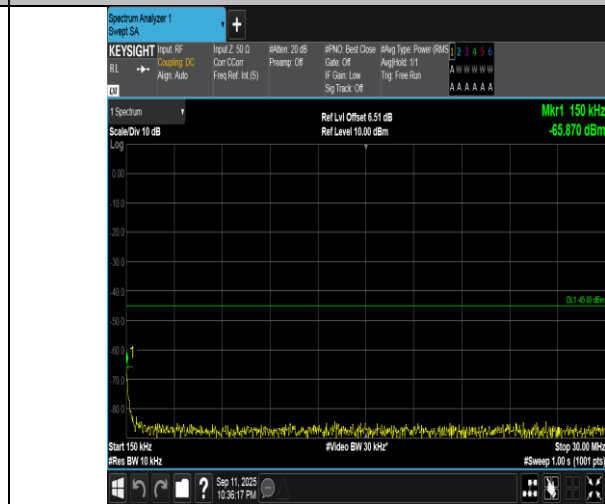
Band7-10MHz-QPSK-21100-1RB#0-0.15~30-PASS
