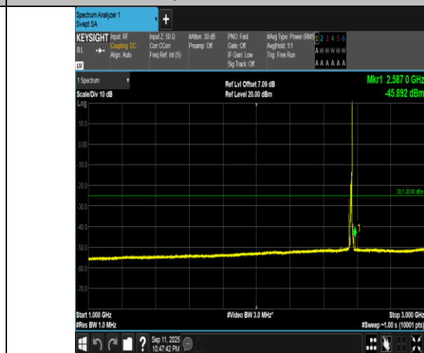
Band7-10MHz-QPSK-21400-1RB#49-1000~3000-PASS
