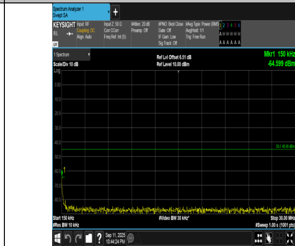
Band7-10MHz-QPSK-21400-1RB#0-0.15~30-PASS
