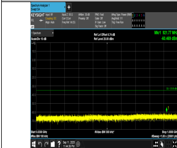
Band7-15MHz-QPSK-20825-1RB#74-30~1000-PASS
