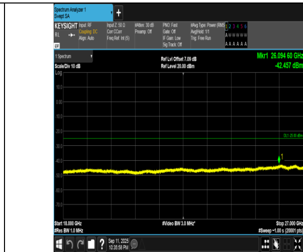
Band7-10MHz-16QAM-20800-50RB#0-18000~27000-PASS
