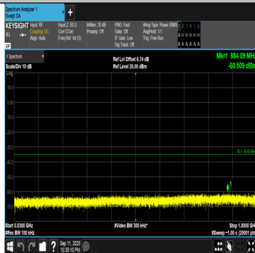
Band7-10MHz-16QAM-20800-50RB#0-30~1000-PASS
