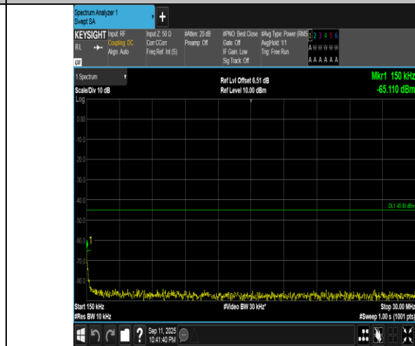
Band7-10MHz-QPSK-21100-50RB#0-0.15~30-PASS
