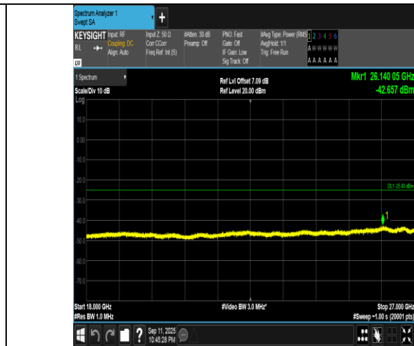
Band7-10MHz-QPSK-21400-1RB#0-18000~27000-PASS
