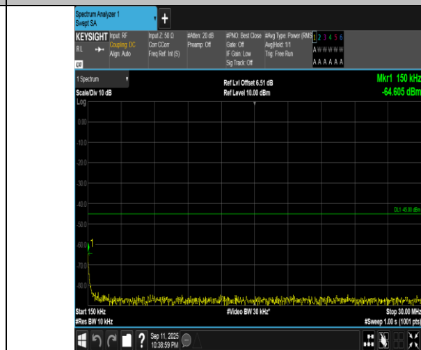
Band7-10MHz-QPSK-21100-1RB#49-0.15~30-PASS
