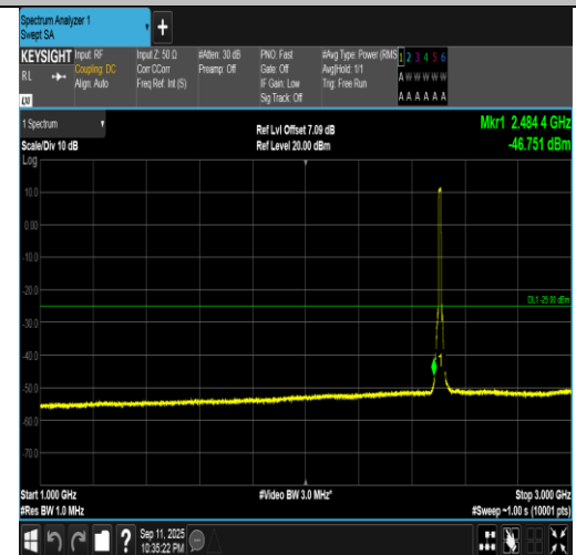
Band7-10MHz-16QAM-20800-50RB#0-1000~3000-PASS
