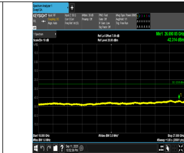
Band7-10MHz-16QAM-21400-50RB#0-18000~27000-PASS
