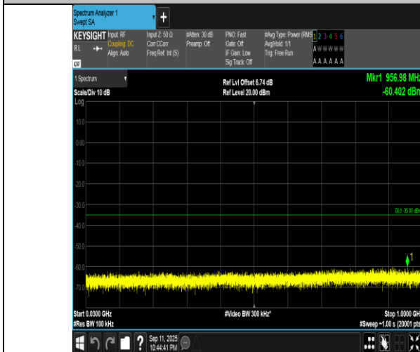
Band7-10MHz-QPSK-21400-1RB#0-30~1000-PASS
