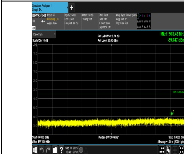
Band7-10MHz-16QAM-21100-50RB#0-30~1000-PASS
