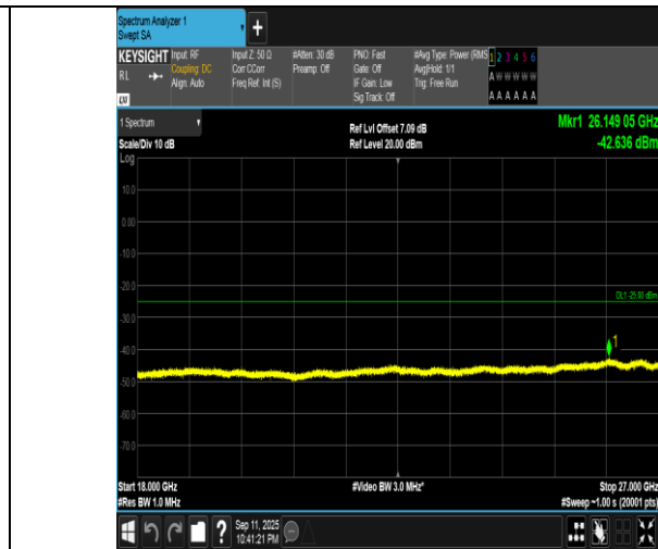
Band7-10MHz-16QAM-21100-1RB#49-18000~27000-PASS
