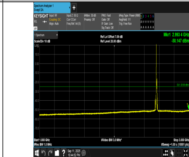
Band7-10MHz-QPSK-21400-1RB#0-1000~3000-PASS
