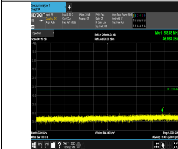
Band7-10MHz-QPSK-21400-50RB#0-30~1000-PASS
