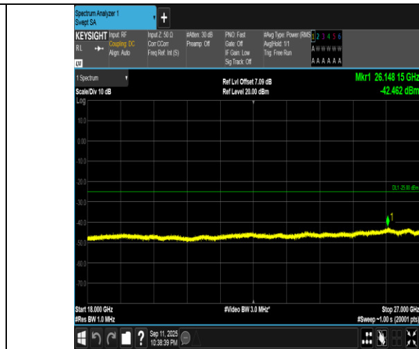
Band7-10MHz-16QAM-21100-1RB#0-18000~27000-PASS
