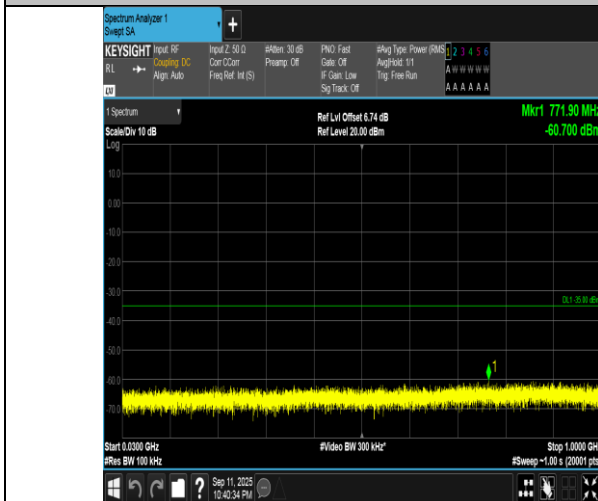
Band7-10MHz-16QAM-21100-1RB#49-30~1000-PASS
