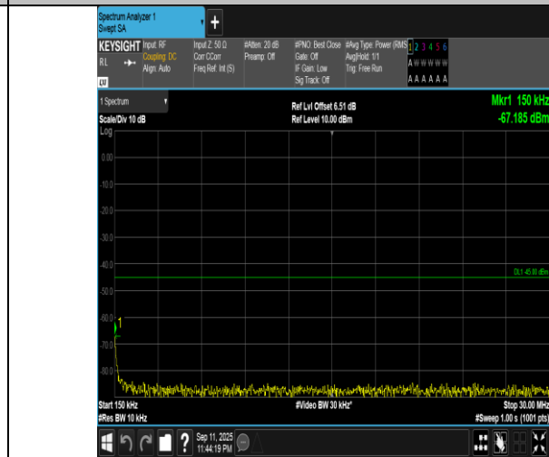
Band7-15MHz-QPSK-20825-1RB#74-0.15~30-PASS
