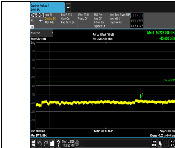
Band7-10MHz-16QAM-21100-1RB#0-3000~18000-PASS
