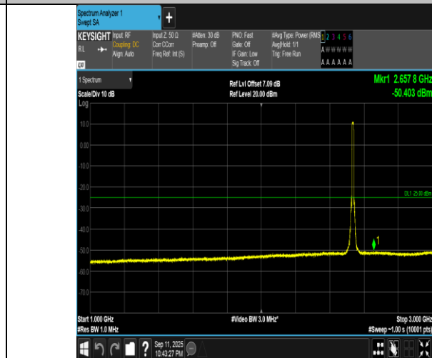
Band7-10MHz-16QAM-21100-50RB#0-1000~3000-PASS
