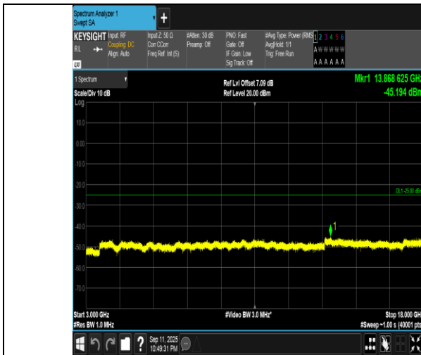
Band7-10MHz-16QAM-21400-1RB#49-3000~18000-PASS
