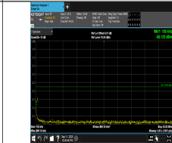
Band7-10MHz-16QAM-21400-1RB#0-0.15~30-PASS
