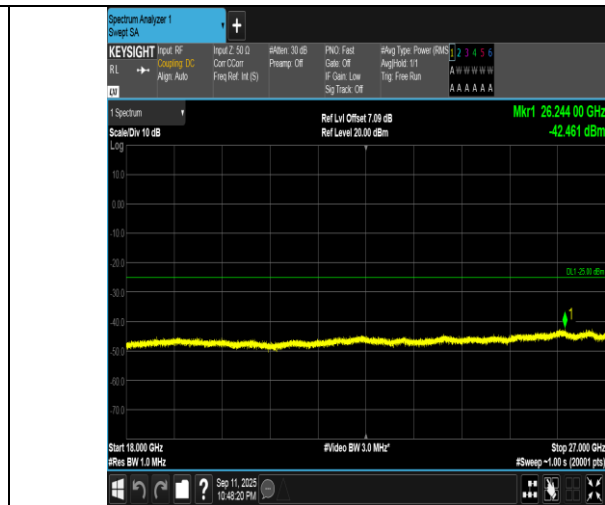
Band7-10MHz-QPSK-21400-1RB#49-18000~27000-PASS
