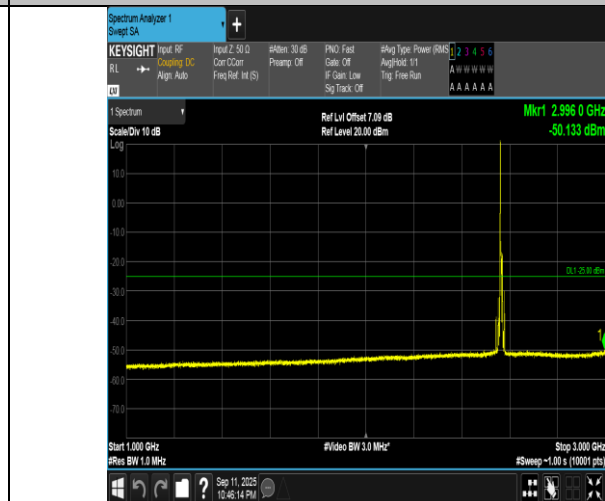
Band7-10MHz-16QAM-21400-1RB#0-1000~3000-PASS
