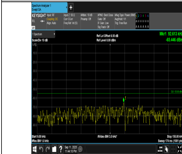
Band7-15MHz-QPSK-20825-1RB#74-0.009~0.15-PASS
