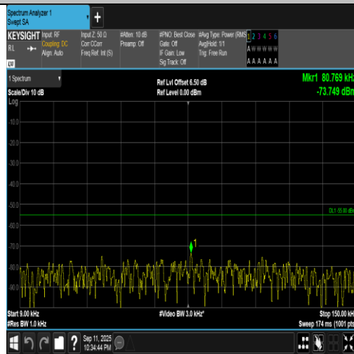
Band7-10MHz-16QAM-20800-50RB#0-0.009~0.15-PASS
