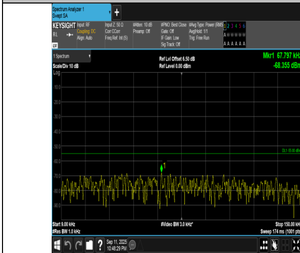
Band7-10MHz-16QAM-21400-1RB#49-0.009~0.15-PASS
