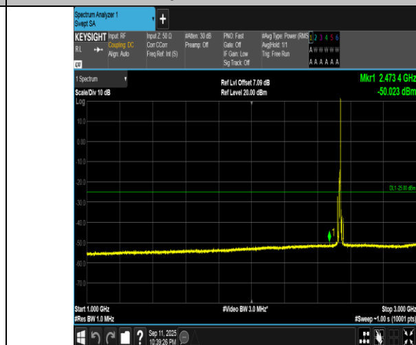
Band7-10MHz-QPSK-21100-1RB#49-1000~3000-PASS
