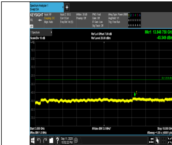
Band7-10MHz-16QAM-21400-50RB#0-3000~18000-PASS
