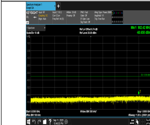
Band7-10MHz-16QAM-21400-1RB#0-30~1000-PASS
