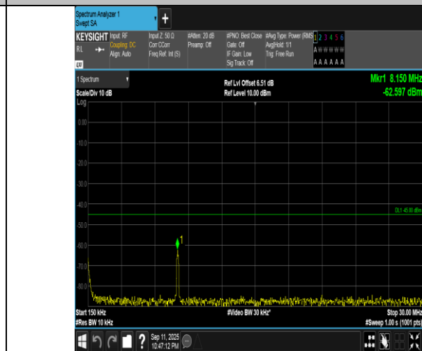
Band7-10MHz-QPSK-21400-1RB#49-0.15~30-PASS
