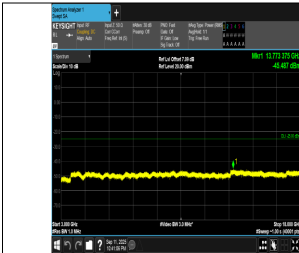
Band7-10MHz-16QAM-21100-1RB#49-3000~18000-PASS
