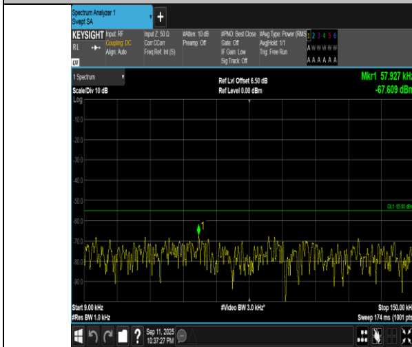
Band7-10MHz-16QAM-21100-1RB#0-0.009~0.15-PASS
