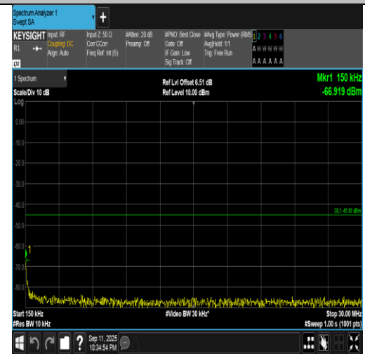
Band7-10MHz-16QAM-20800-50RB#0-0.15~30-PASS
