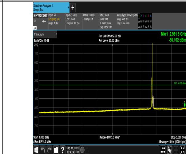
Band7-10MHz-16QAM-21100-1RB#49-1000~3000-PASS
