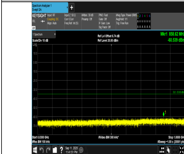
Band7-15MHz-QPSK-20825-1RB#0-30~1000-PASS
