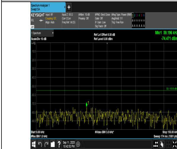
Band7-10MHz-16QAM-21100-50RB#0-0.009~0.15-PASS
