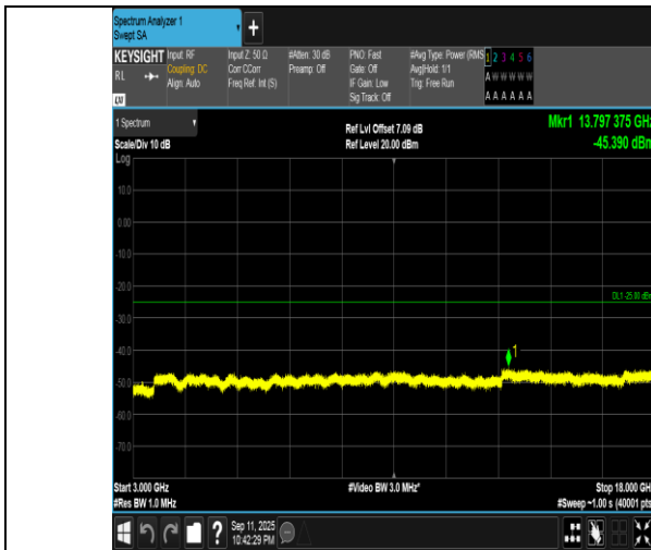
Band7-10MHz-QPSK-21100-50RB#0-3000~18000-PASS
