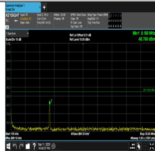
Band7-10MHz-16QAM-21400-1RB#49-0.15~30-PASS
