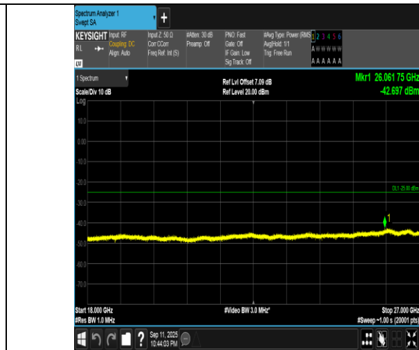
Band7-10MHz-16QAM-21100-50RB#0-18000~27000-PASS
