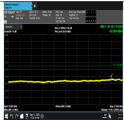
Band7-15MHz-16QAM-21100-1RB#0-18000~27000-PASS
