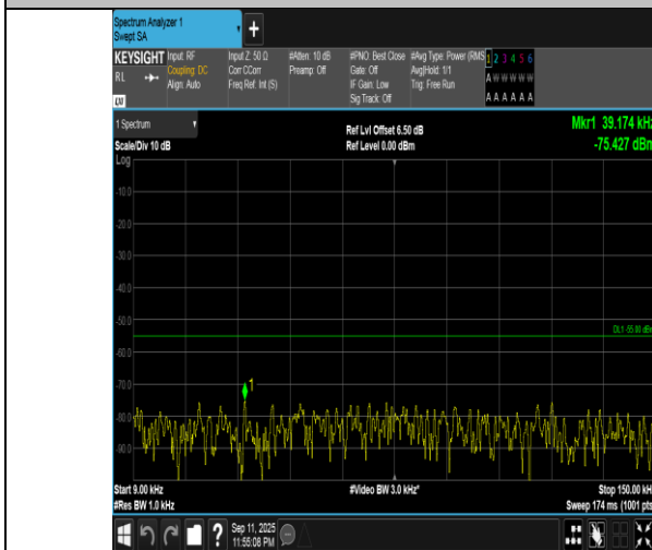
Band7-15MHz-QPSK-21100-75RB#0-0.009~0.15-PASS
