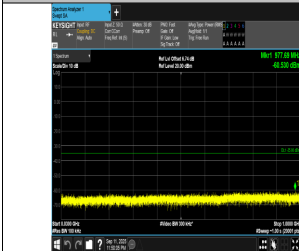
Band7-15MHz-QPSK-21100-1RB#0-30~1000-PASS
