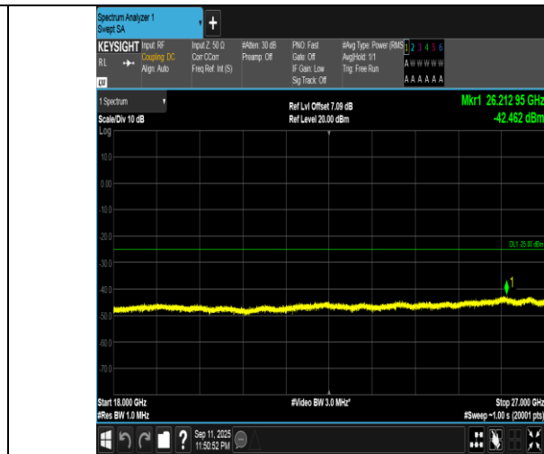
Band7-15MHz-QPSK-21100-1RB#0-18000~27000-PASS
