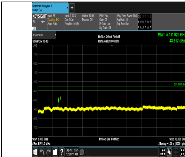
Band7-15MHz-16QAM-21375-1RB#0-3000~18000-PASS
