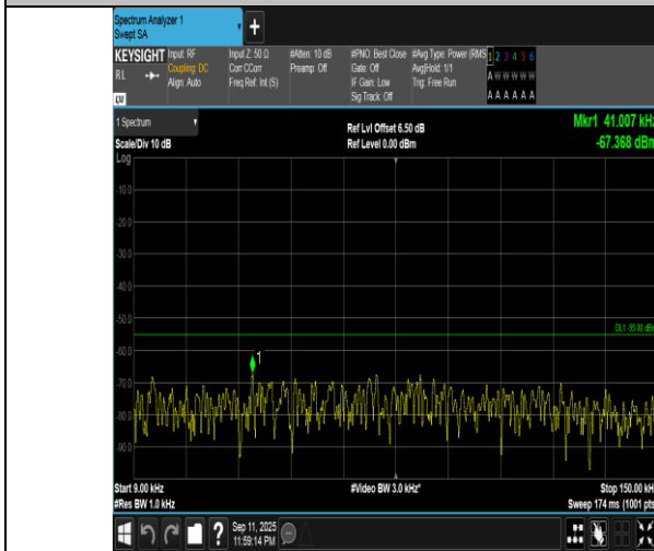
Band7-15MHz-16QAM-21375-1RB#0-0.009~0.15-PASS
