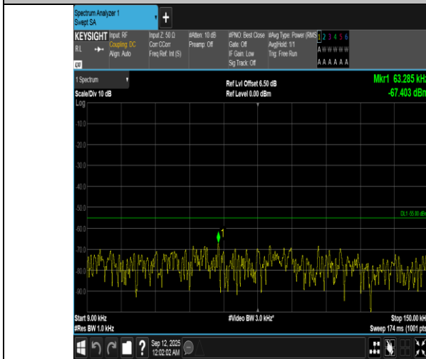
Band7-15MHz-16QAM-21375-1RB#74-0.009~0.15-PASS
