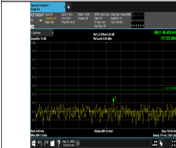
Band7-15MHz-QPSK-21375-75RB#0-0.009~0.15-PASS
