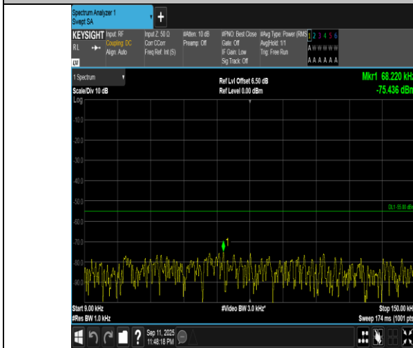
Band7-15MHz-16QAM-20825-75RB#0-0.009~0.15-PASS
