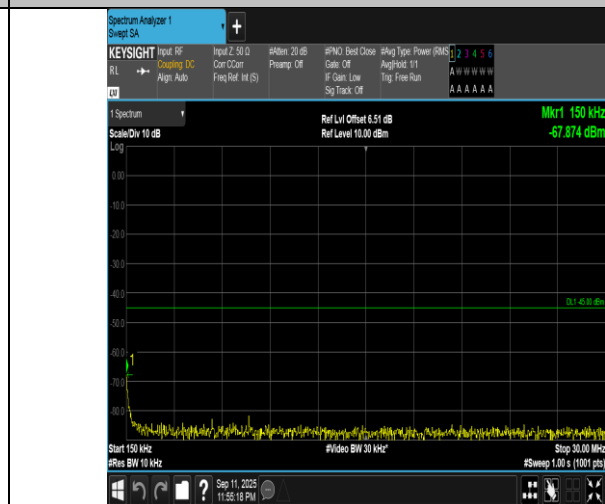
Band7-15MHz-QPSK-21100-75RB#0-0.15~30-PASS
