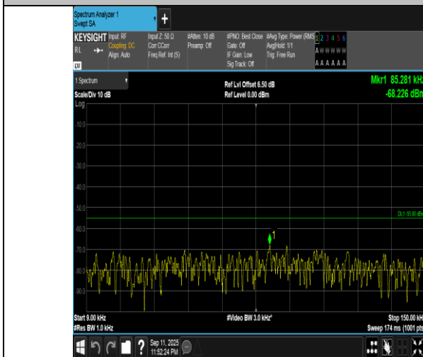
Band7-15MHz-QPSK-21100-1RB#74-0.009~0.15-PASS
