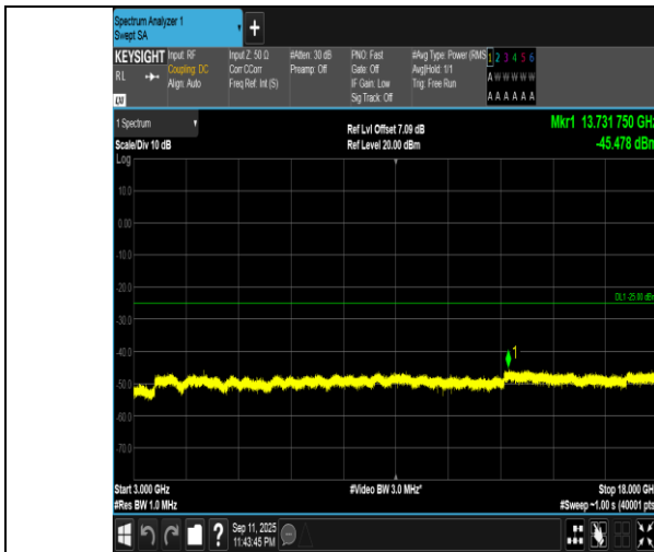
Band7-15MHz-16QAM-20825-1RB#0-3000~18000-PASS
