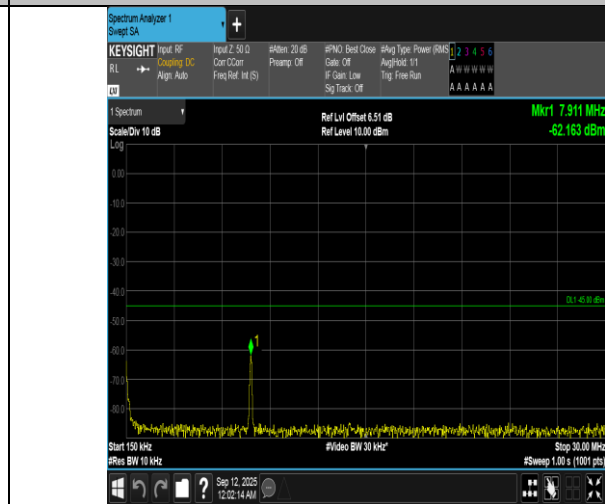
Band7-15MHz-16QAM-21375-1RB#74-0.15~30-PASS
