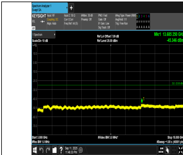
Band7-15MHz-16QAM-20825-1RB#74-3000~18000-PASS
