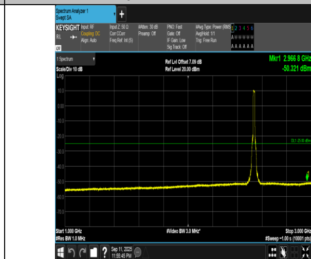
Band7-15MHz-QPSK-21100-75RB#0-1000~3000-PASS
