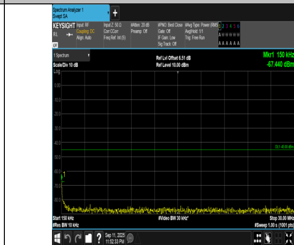
Band7-15MHz-QPSK-21100-1RB#74-0.15~30-PASS
