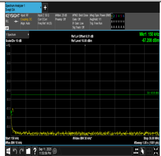
Band7-15MHz-16QAM-21100-1RB#74-0.15~30-PASS
