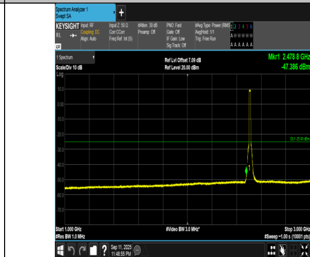
Band7-15MHz-16QAM-20825-75RB#0-1000~3000-PASS
