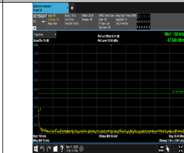
Band7-15MHz-16QAM-21100-1RB#0-0.15~30-PASS
