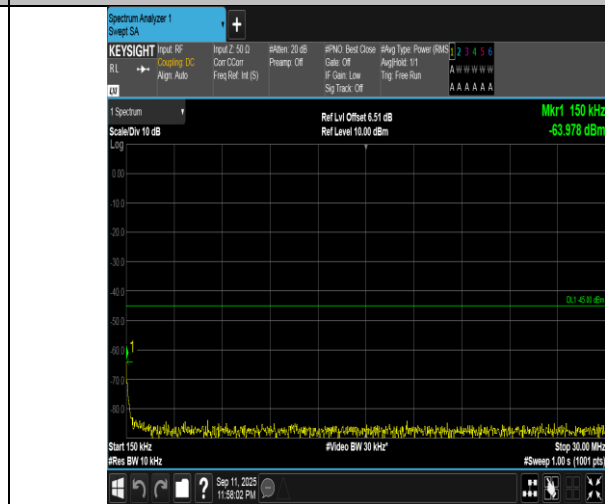
Band7-15MHz-QPSK-21375-1RB#0-0.15~30-PASS
