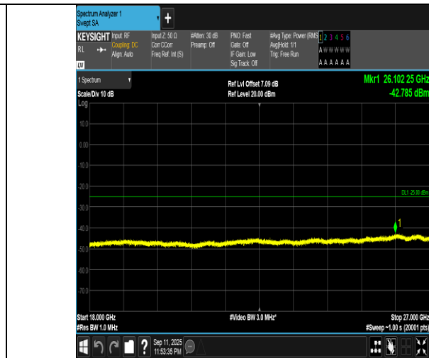
Band7-15MHz-QPSK-21100-1RB#74-18000~27000-PASS
