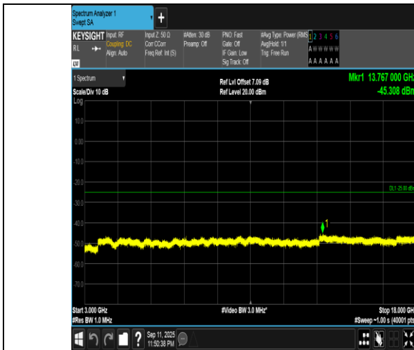
Band7-15MHz-QPSK-21100-1RB#0-3000~18000-PASS
