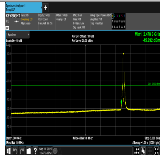
Band7-15MHz-QPSK-20825-75RB#0-1000~3000-PASS
