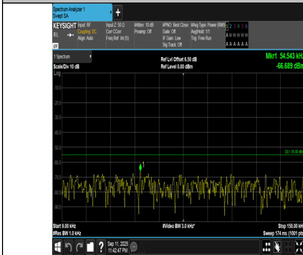
Band7-15MHz-16QAM-20825-1RB#0-0.009~0.15-PASS
