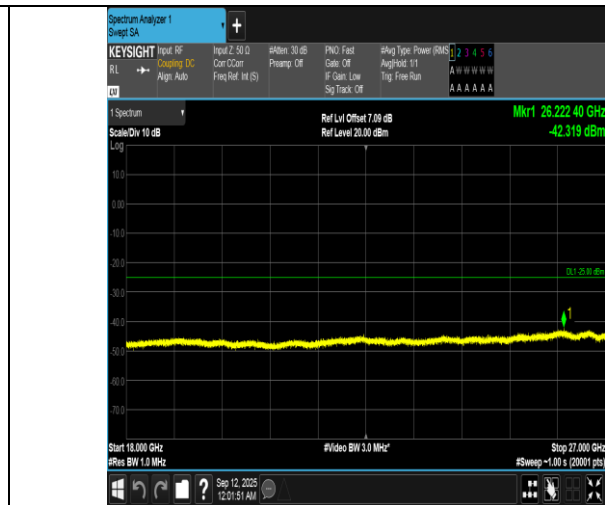
Band7-15MHz-QPSK-21375-1RB#74-18000~27000-PASS
