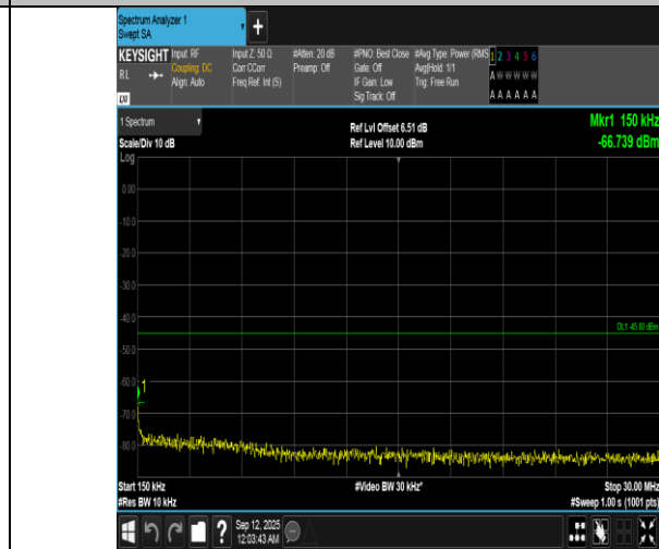
Band7-15MHz-QPSK-21375-75RB#0-0.15~30-PASS
