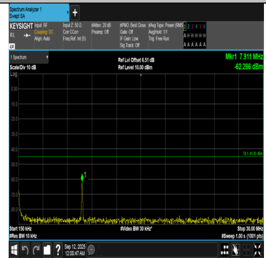
Band7-15MHz-QPSK-21375-1RB#74-0.15~30-PASS
