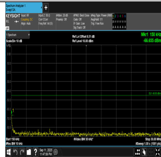
Band7-15MHz-QPSK-20825-75RB#0-0.15~30-PASS
