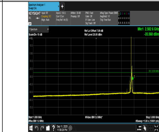
Band7-15MHz-QPSK-21375-1RB#0-1000~3000-PASS
