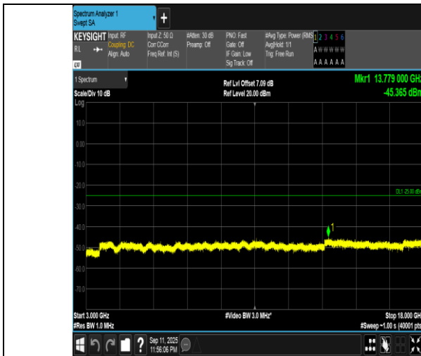
Band7-15MHz-QPSK-21100-75RB#0-3000~18000-PASS
