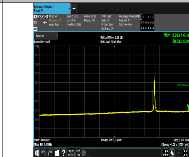
Band7-15MHz-QPSK-21100-1RB#74-1000~3000-PASS
