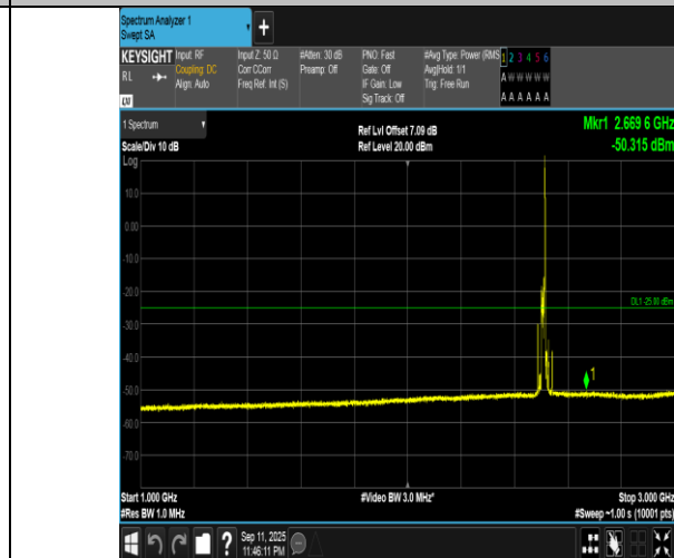
Band7-15MHz-16QAM-20825-1RB#74-1000~3000-PASS
