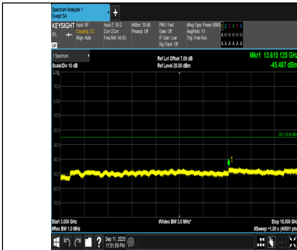
Band7-15MHz-16QAM-21100-1RB#0-3000~18000-PASS
