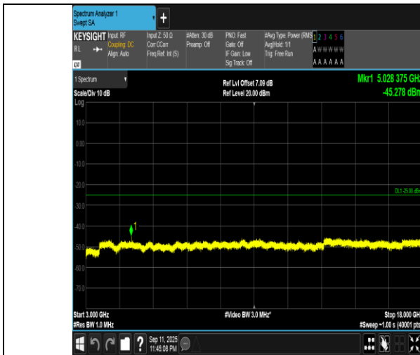
Band7-15MHz-QPSK-20825-1RB#74-3000~18000-PASS
