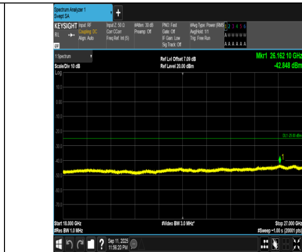
Band7-15MHz-QPSK-21100-75RB#0-18000~27000-PASS
