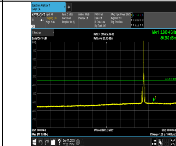
Band7-15MHz-QPSK-21100-1RB#0-1000~3000-PASS
