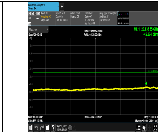
Band7-15MHz-16QAM-21375-1RB#0-18000~27000-PASS
