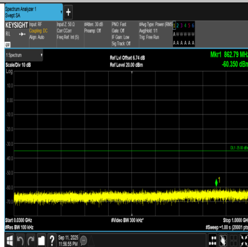
Band7-15MHz-16QAM-21100-75RB#0-30~1000-PASS
