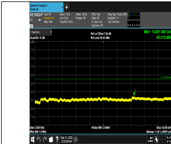
Band7-15MHz-16QAM-21375-1RB#74-3000~18000-PASS
