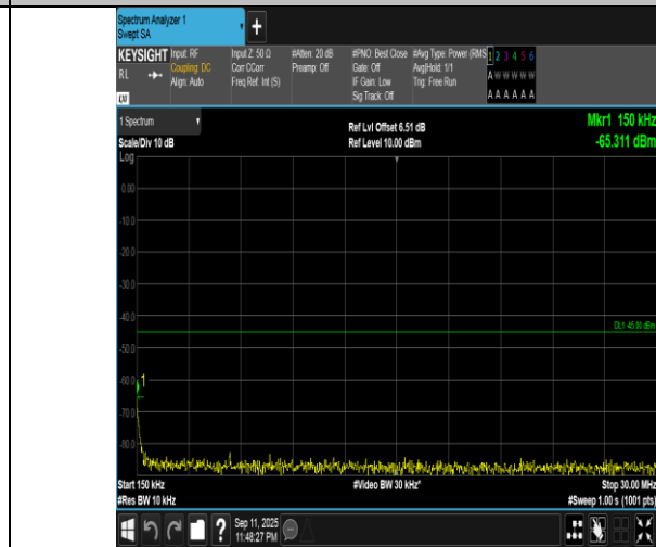
Band7-15MHz-16QAM-20825-75RB#0-0.15~30-PASS
