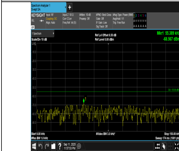
Band7-15MHz-QPSK-21375-1RB#0-0.009~0.15-PASS
