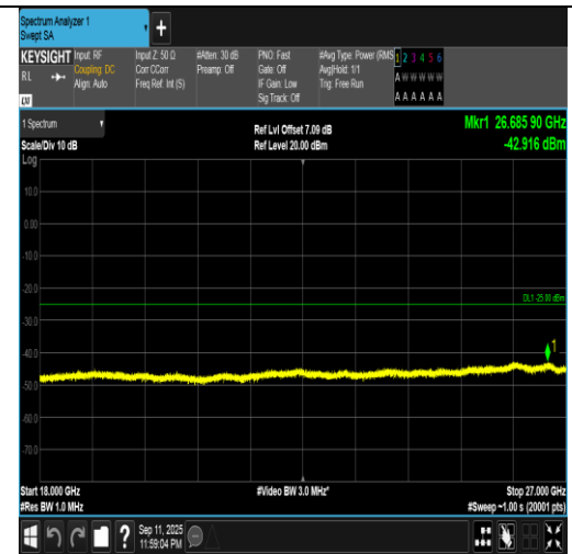
Band7-15MHz-QPSK-21375-1RB#0-18000~27000-PASS
