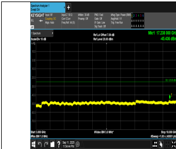
Band7-15MHz-16QAM-21100-1RB#74-3000~18000-PASS
