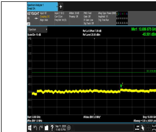
Band7-15MHz-16QAM-20825-75RB#0-3000~18000-PASS
