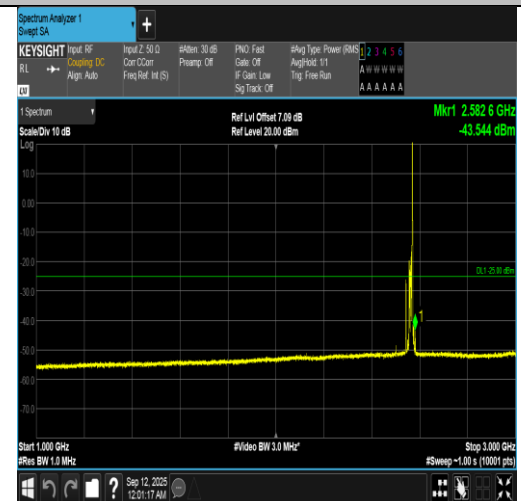
Band7-15MHz-QPSK-21375-1RB#74-1000~3000-PASS
