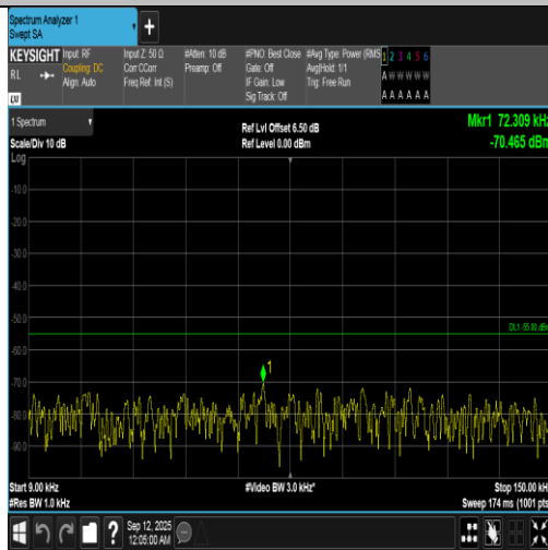
Band7-15MHz-16QAM-21375-75RB#0-0.009~0.15-PASS
