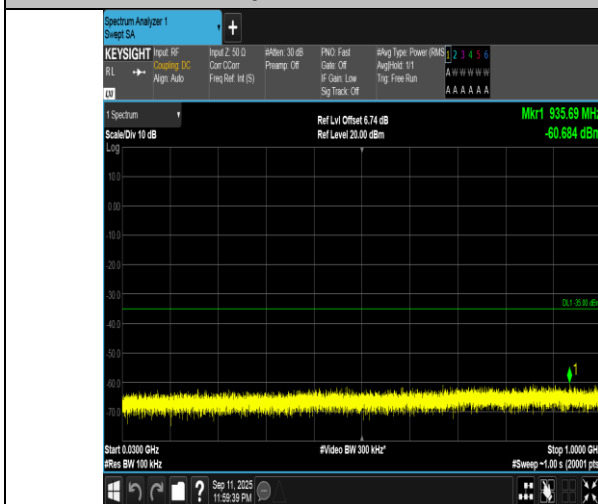
Band7-15MHz-16QAM-21375-1RB#0-30~1000-PASS
