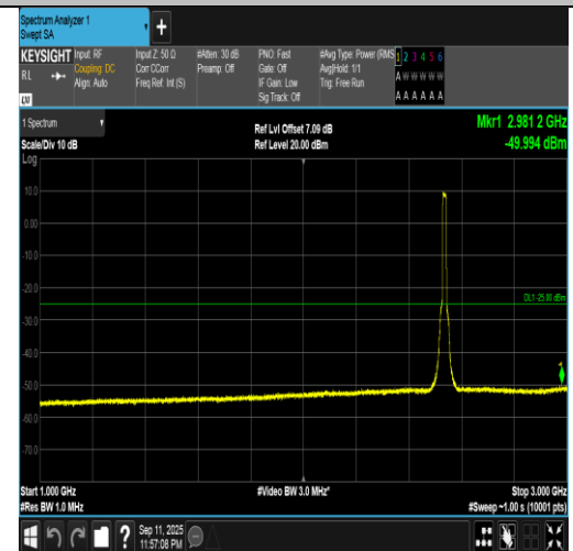
Band7-15MHz-16QAM-21100-75RB#0-1000~3000-PASS
