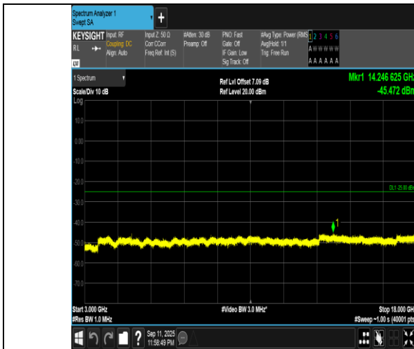
Band7-15MHz-QPSK-21375-1RB#0-3000~18000-PASS
