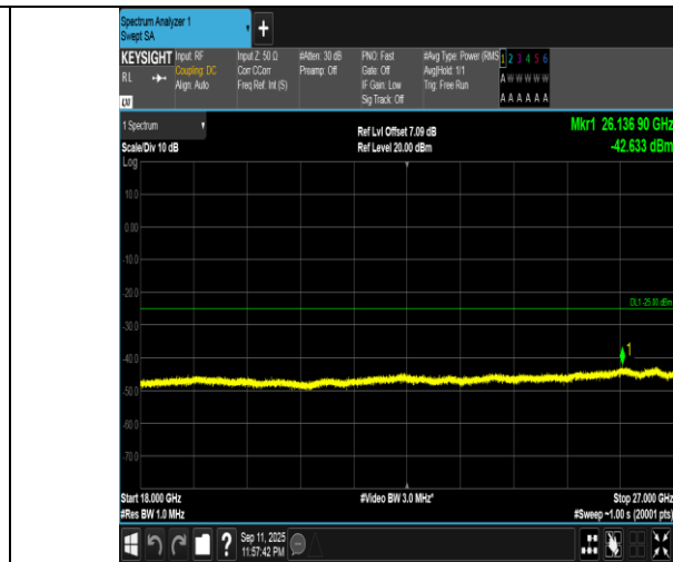
Band7-15MHz-16QAM-21100-75RB#0-18000~27000-PASS
