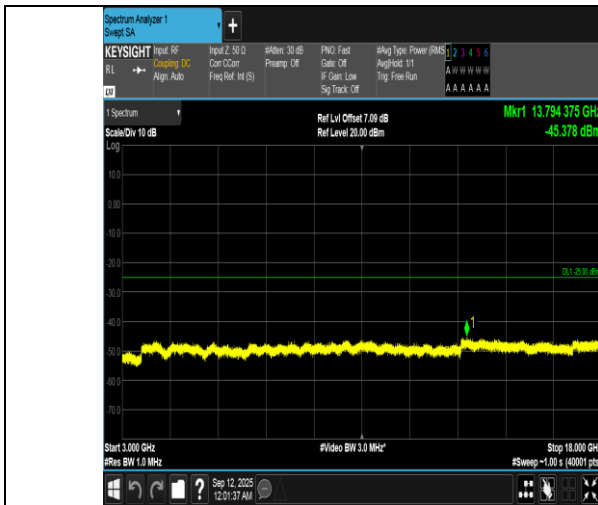
Band7-15MHz-QPSK-21375-1RB#74-3000~18000-PASS
