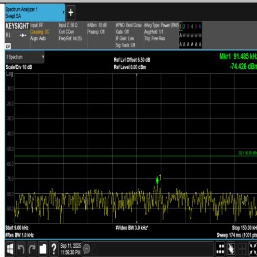
Band7-15MHz-16QAM-21100-75RB#0-0.009~0.15-PASS
