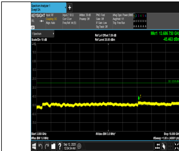
Band7-15MHz-QPSK-21375-75RB#0-3000~18000-PASS
