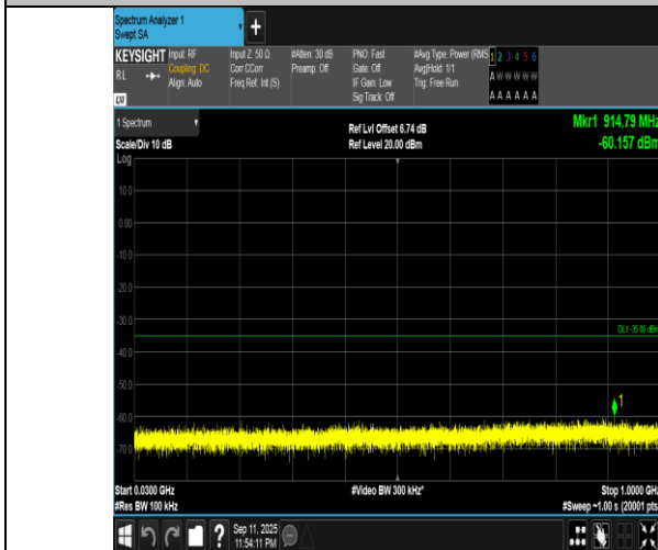
Band7-15MHz-16QAM-21100-1RB#74-30~1000-PASS
