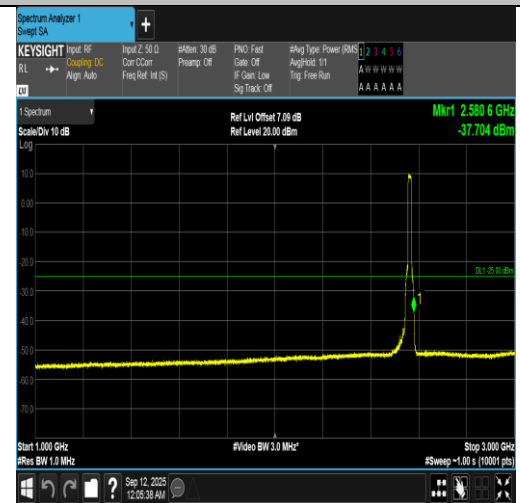
Band7-15MHz-16QAM-21375-75RB#0-1000~3000-PASS
