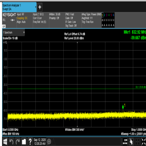
Band7-15MHz-16QAM-21375-75RB#0-30~1000-PASS
