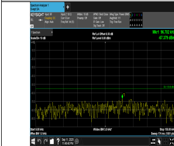
Band7-15MHz-QPSK-21100-1RB#0-0.009~0.15-PASS
