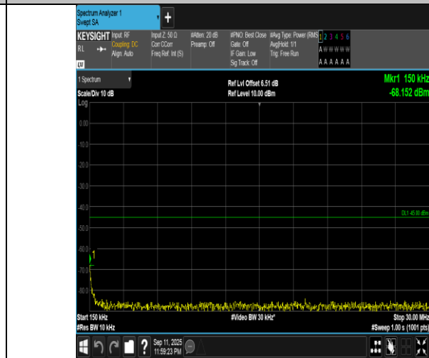
Band7-15MHz-16QAM-21375-1RB#0-0.15~30-PASS
