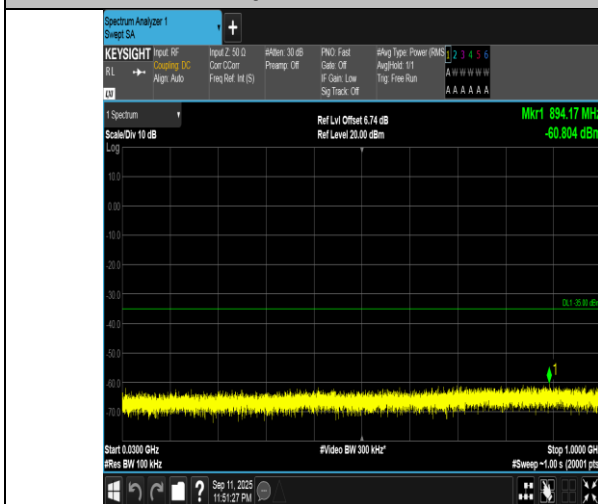
Band7-15MHz-16QAM-21100-1RB#0-30~1000-PASS
