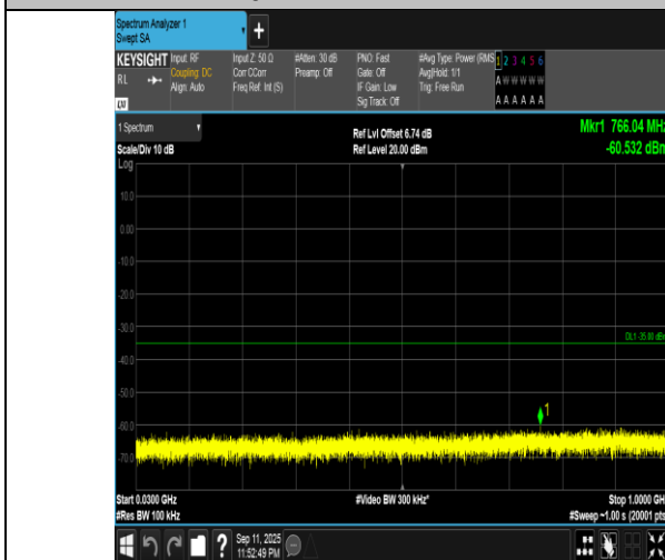
Band7-15MHz-QPSK-21100-1RB#74-30~1000-PASS
