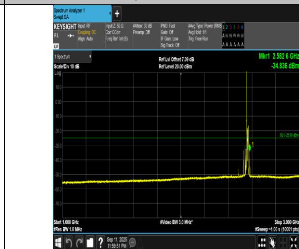
Band7-15MHz-16QAM-21375-1RB#0-1000~3000-PASS
