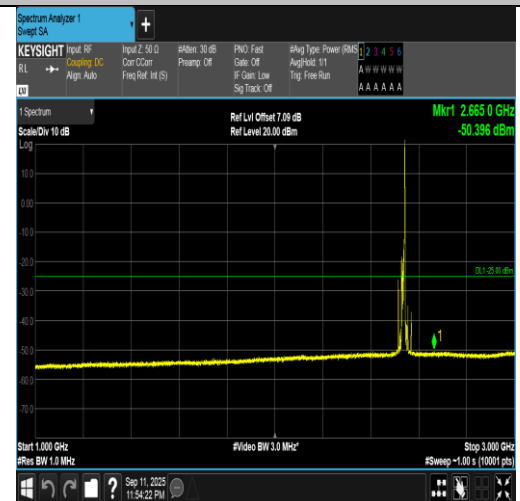
Band7-15MHz-16QAM-21100-1RB#74-1000~3000-PASS
