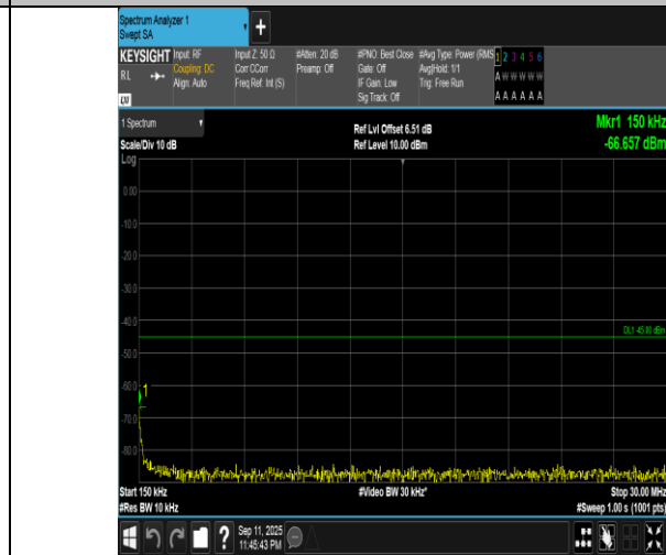
Band7-15MHz-16QAM-20825-1RB#74-0.15~30-PASS
