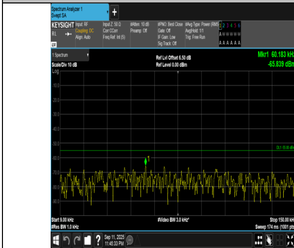
Band7-15MHz-16QAM-20825-1RB#74-0.009~0.15-PASS
