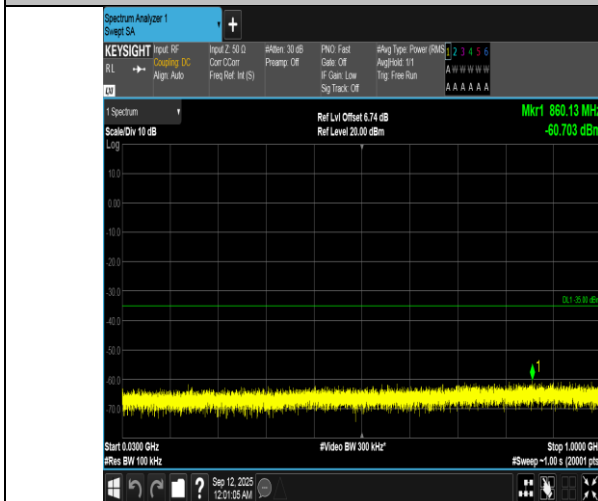
Band7-15MHz-QPSK-21375-1RB#74-30~1000-PASS
