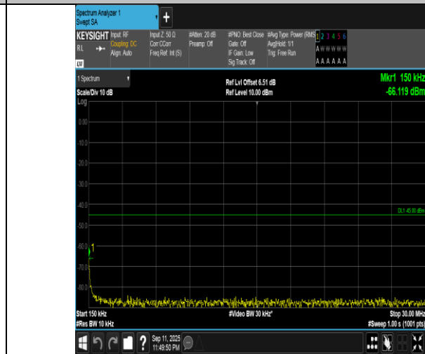
Band7-15MHz-QPSK-21100-1RB#0-0.15~30-PASS
