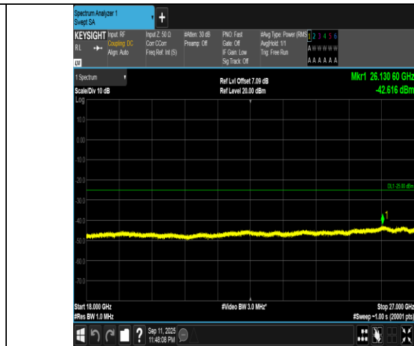
Band7-15MHz-QPSK-20825-75RB#0-18000~27000-PASS
