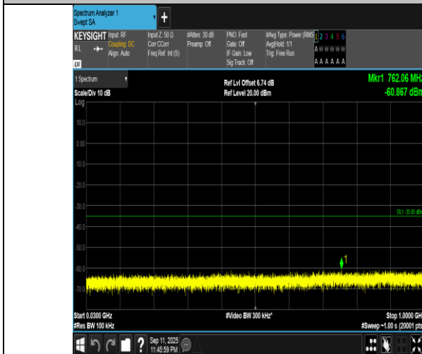
Band7-15MHz-16QAM-20825-1RB#74-30~1000-PASS
