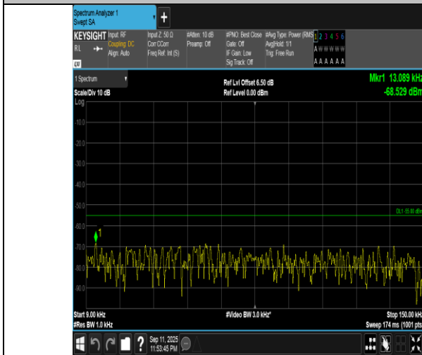
Band7-15MHz-16QAM-21100-1RB#74-0.009~0.15-PASS
