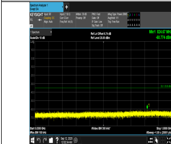
Band7-15MHz-16QAM-21375-1RB#74-30~1000-PASS
