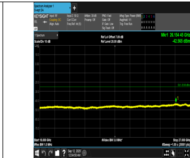
Band7-15MHz-QPSK-21375-75RB#0-18000~27000-PASS
