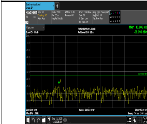
Band7-15MHz-QPSK-21375-1RB#74-0.009~0.15-PASS
