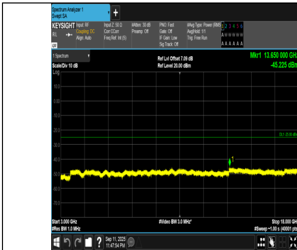
Band7-15MHz-QPSK-20825-75RB#0-3000~18000-PASS
