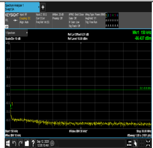
Band7-15MHz-16QAM-21375-75RB#0-0.15~30-PASS
