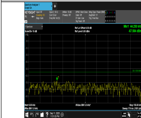
Band7-15MHz-16QAM-21100-1RB#0-0.009~0.15-PASS
