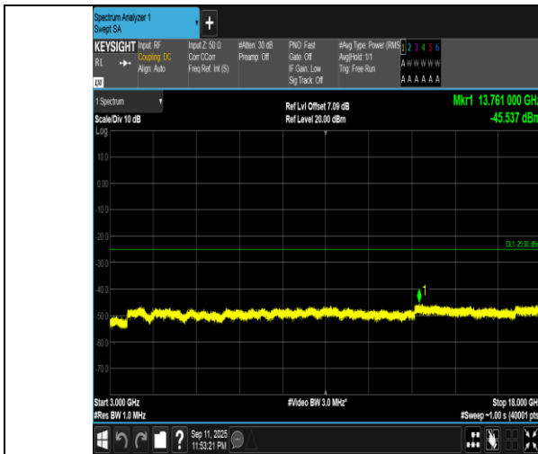
Band7-15MHz-QPSK-21100-1RB#74-3000~18000-PASS
