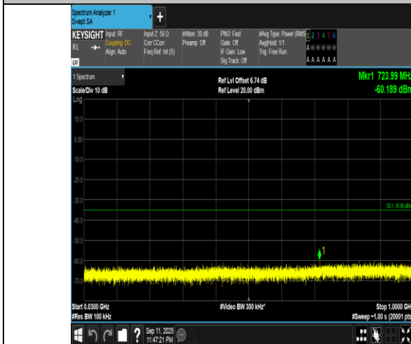
Band7-15MHz-QPSK-20825-75RB#0-30~1000-PASS
