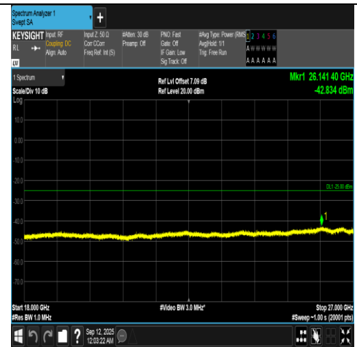
Band7-15MHz-16QAM-21375-1RB#74-18000~27000-PASS
