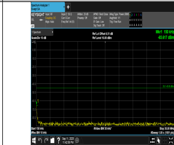
Band7-15MHz-16QAM-20825-1RB#0-0.15~30-PASS
