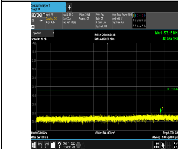
Band7-15MHz-16QAM-20825-75RB#0-30~1000-PASS
