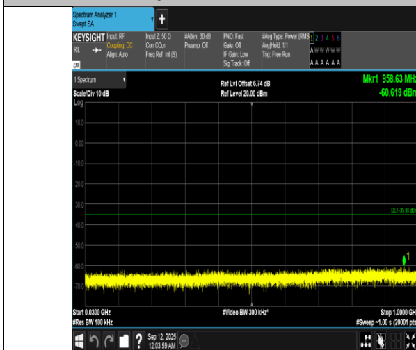
Band7-15MHz-QPSK-21375-75RB#0-30~1000-PASS
