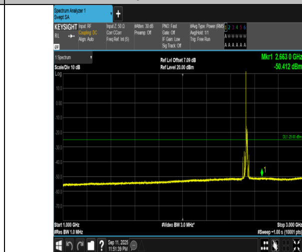
Band7-15MHz-16QAM-21100-1RB#0-1000~3000-PASS
