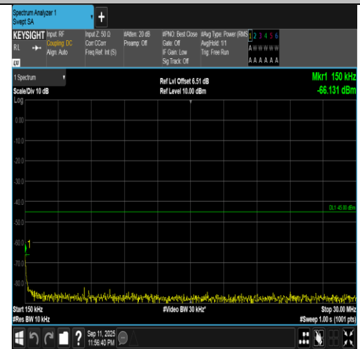
Band7-15MHz-16QAM-21100-75RB#0-0.15~30-PASS
