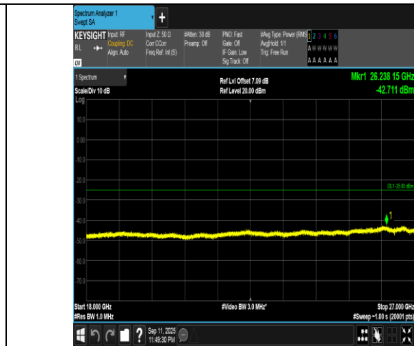
Band7-15MHz-16QAM-20825-75RB#0-18000~27000-PASS
