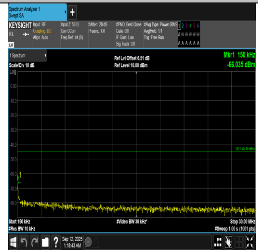
Band7-20MHz-16QAM-21350-100RB#0-0.15~30-PASS
