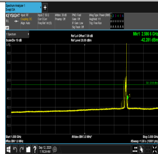
Band7-20MHz-16QAM-21350-1RB#99-1000~3000-PASS
