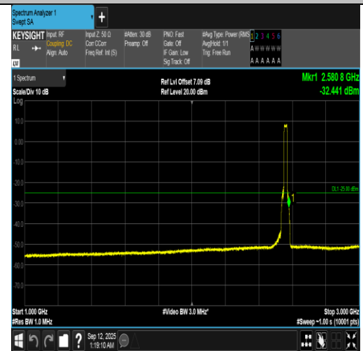
Band7-20MHz-16QAM-21350-100RB#0-1000~3000-PASS
