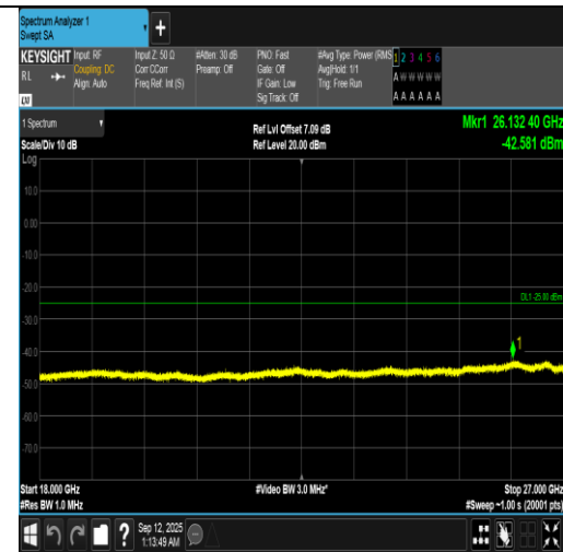
Band7-20MHz-16QAM-21350-1RB#0-18000~27000-PASS
