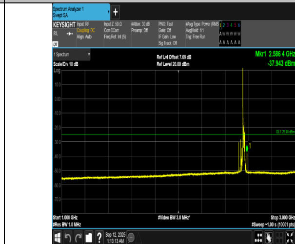
Band7-20MHz-16QAM-21350-1RB#0-1000~3000-PASS
