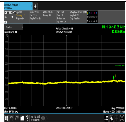
Band7-20MHz-16QAM-21350-1RB#99-18000~27000-PASS
