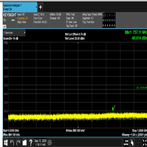
Band7-20MHz-16QAM-21350-1RB#99-30~1000-PASS
