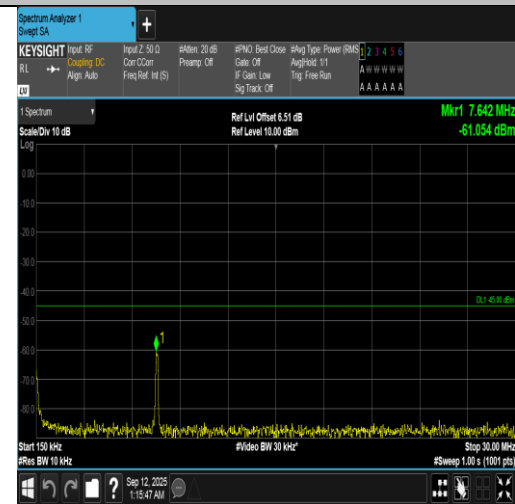
Band7-20MHz-16QAM-21350-1RB#99-0.15~30-PASS
