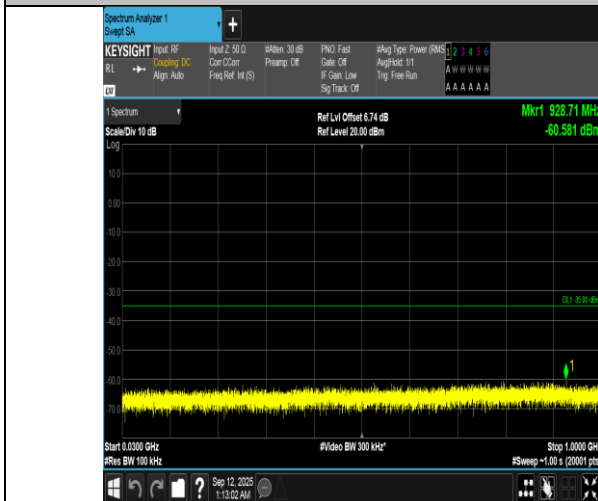
Band7-20MHz-16QAM-21350-1RB#0-30~1000-PASS
