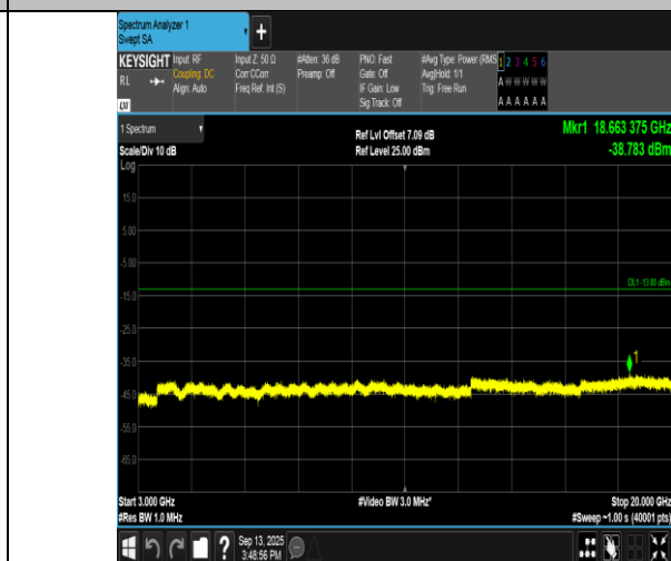
Band2-9400-3000~20000MHz-PASS
