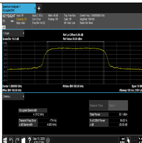
Band2-9400-5-PASS
