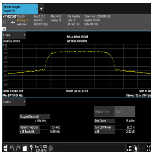
Band2-9262-4-PASS
