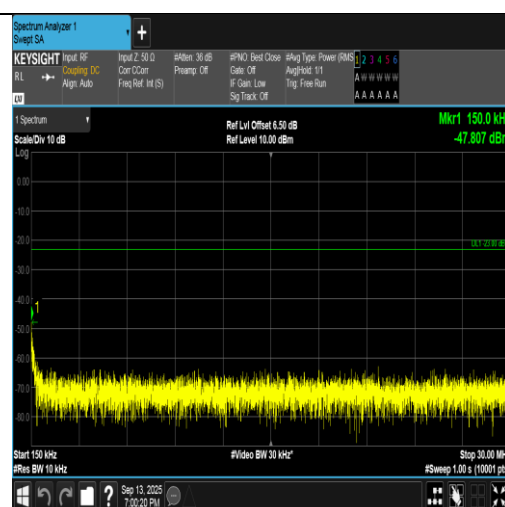
Band5-4132-0.15~30MHz-PASS
