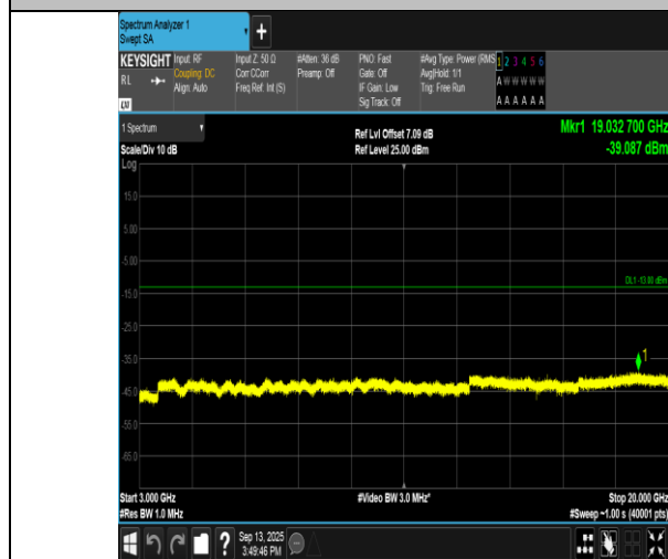
Band2-9538-3000~20000MHz-PASS
