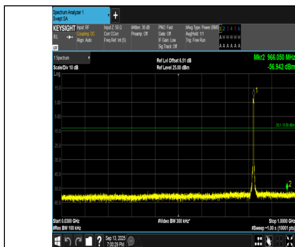
Band5-4132-30~1000MHz-PASS
