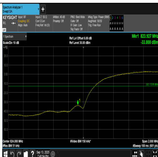
Band5-4132-2-PASS
