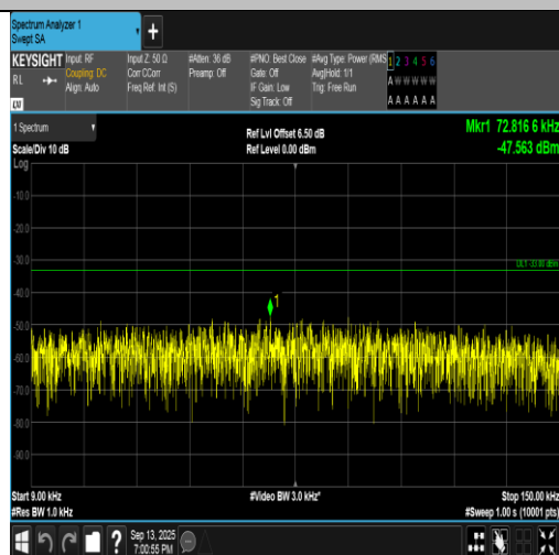
Band5-4182-0.009~0.15MHz-PASS
