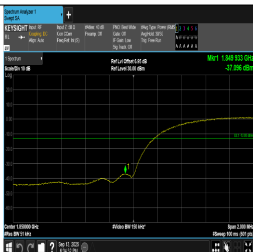
Band2-9262-3-PASS
