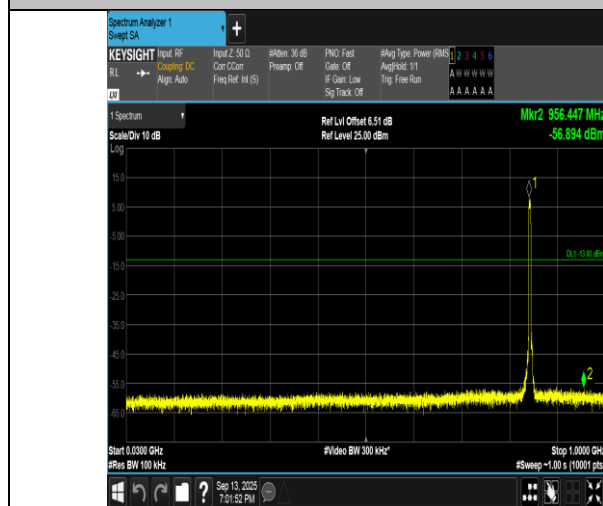
Band5-4233-30~1000MHz-PASS
