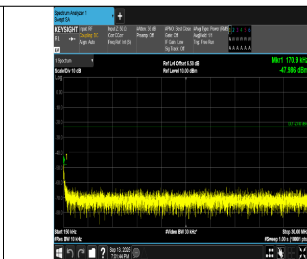
Band5-4233-0.15~30MHz-PASS
