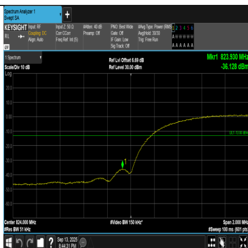
Band5-4132-1-PASS
