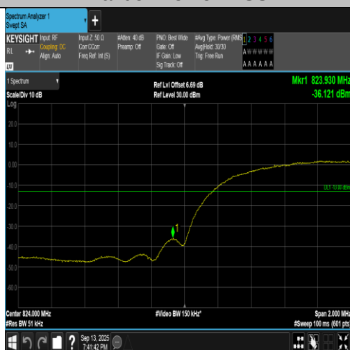
Band5-4132-4-PASS
