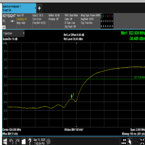
Band5-4132-3-PASS
