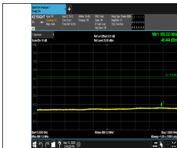
Band2-9538-30~1000MHz-PASS
