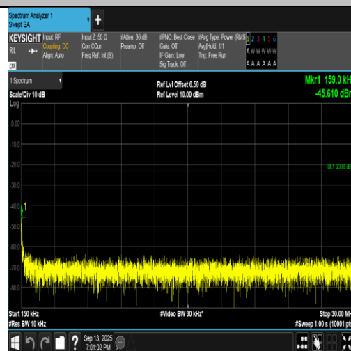
Band5-4182-0.15~30MHz-PASS
