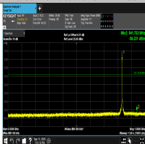
Band5-4182-30~1000MHz-PASS
