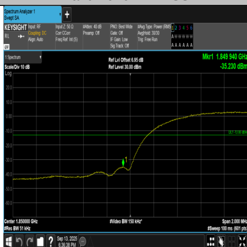
Band2-9262-5-PASS
