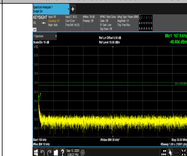
Band2-9538-0.15~30MHz-PASS
