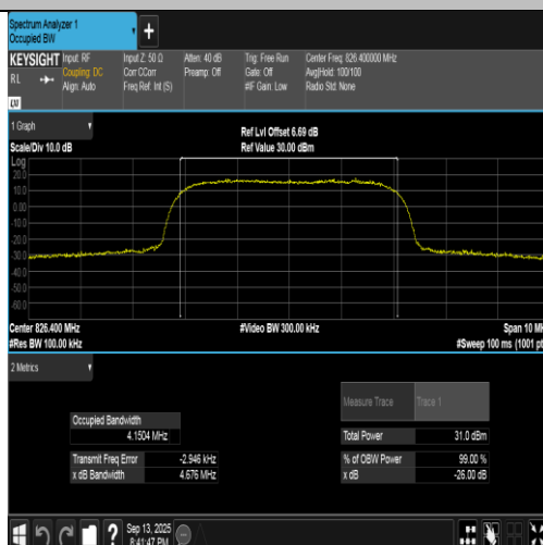
Band5-4132-5-PASS
