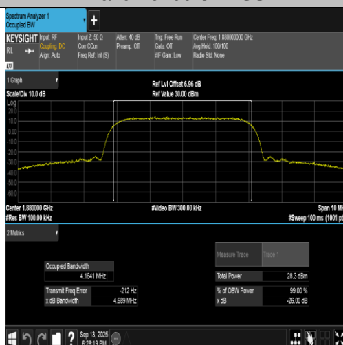
Band2-9400-4-PASS
