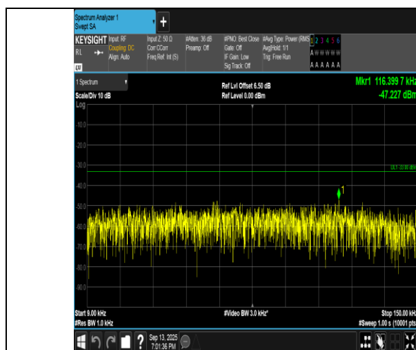
Band5-4233-0.009~0.15MHz-PASS
