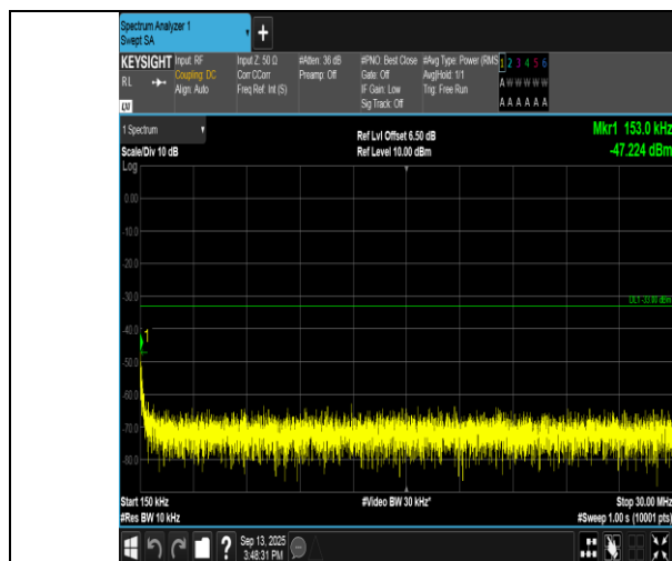
Band2-9400-0.15~30MHz-PASS
