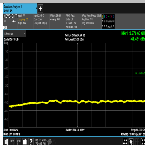
Band5-4182-1000~10000MHz-PASS
