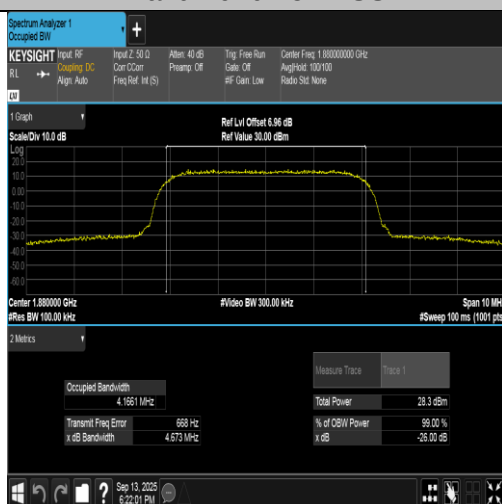
Band2-9400-1-PASS
