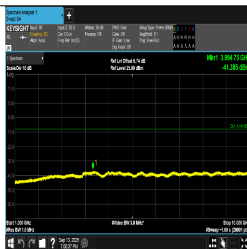
Band5-4132-1000~10000MHz-PASS
