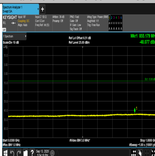
Band2-9262-4-30~1000MHz-PASS
