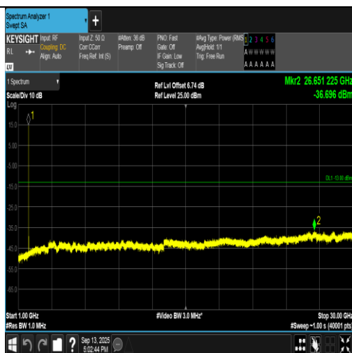
Band2-9400-3-1000~30000MHz-PASS
