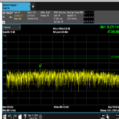
Band5-4132-3-0.009~0.15MHz-PASS
