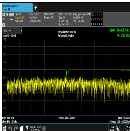
Band2-9400-3-0.009~0.15MHz-PASS
