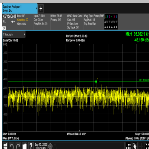
Band2-9538-4-0.009~0.15MHz-PASS
