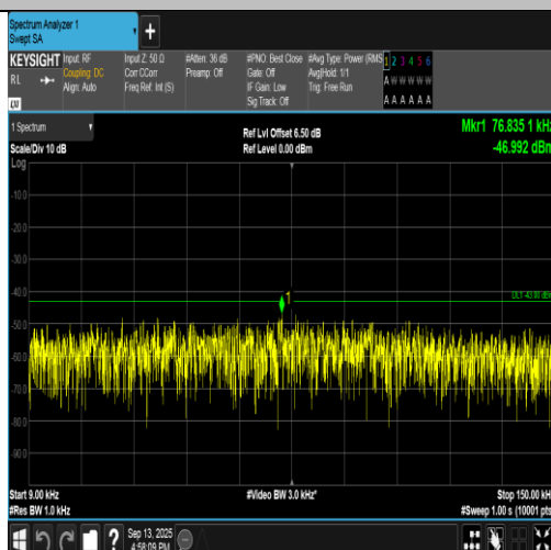
Band2-9538-1-0.009~0.15MHz-PASS
