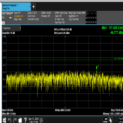
Band5-4182-2-0.009~0.15MHz-PASS
