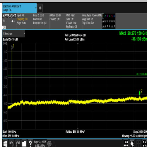
Band2-9262-2-1000~30000MHz-PASS
