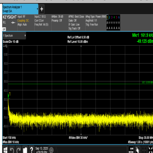
Band2-9400-2-0.15~30MHz-PASS
