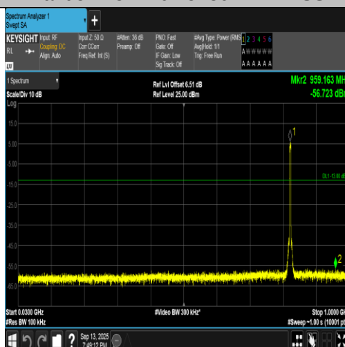
Band5-4132-4-30~1000MHz-PASS
