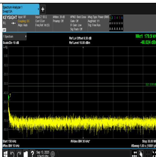
Band2-9400-4-0.15~30MHz-PASS
