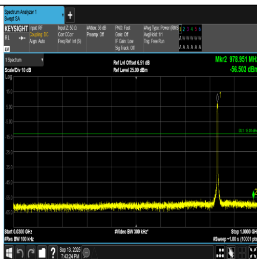
Band5-4182-1-30~1000MHz-PASS
