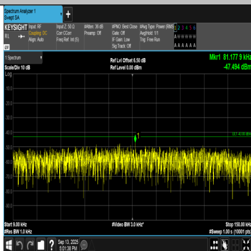
Band2-9262-3-0.009~0.15MHz-PASS
