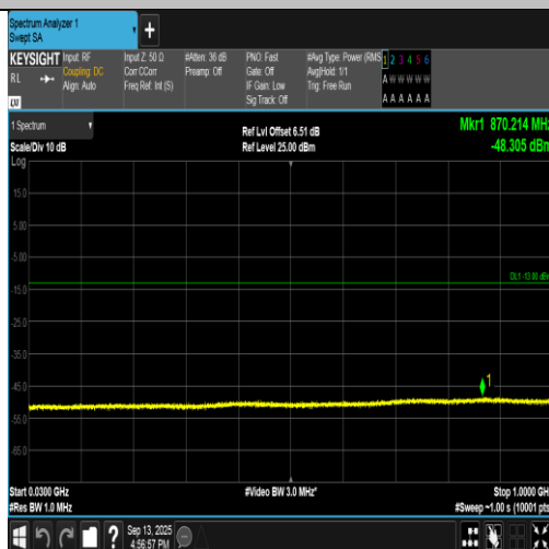
Band2-9262-1-30~1000MHz-PASS
