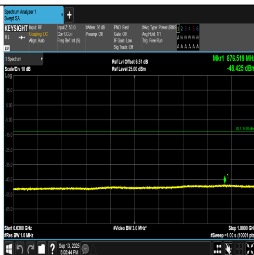
Band2-9538-4-30~1000MHz-PASS
