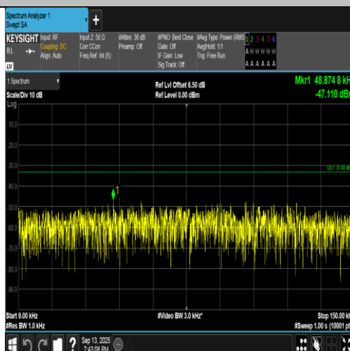
Band5-4182-1-0.009~0.15MHz-PASS
