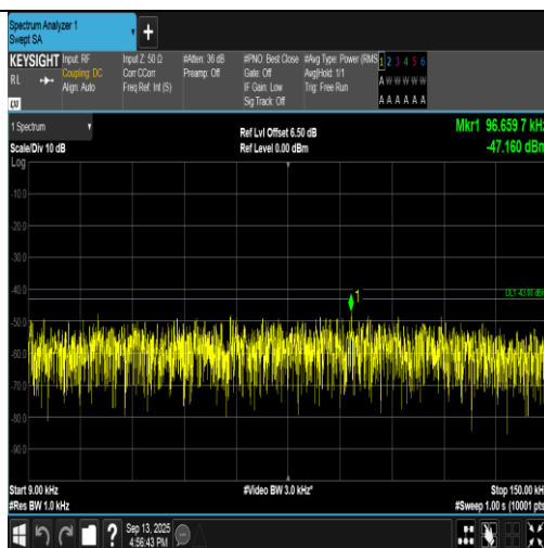
Band2-9262-1-0.009~0.15MHz-PASS
