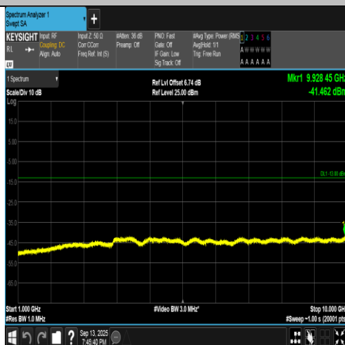
Band5-4182-2-1000~10000MHz-PASS
