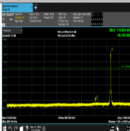
Band5-4182-3-30~1000MHz-PASS
