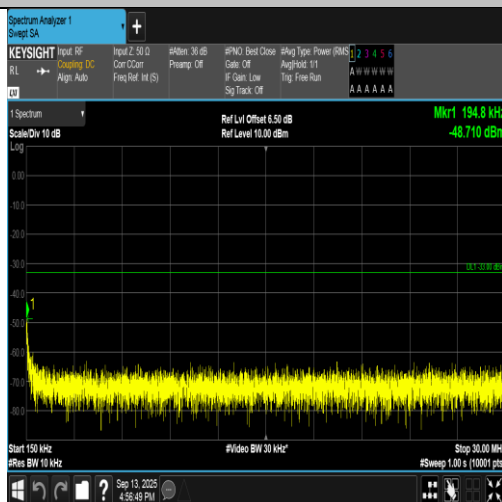
Band2-9262-1-0.15~30MHz-PASS
