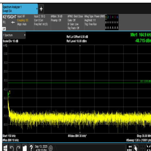
Band2-9262-2-0.15~30MHz-PASS
