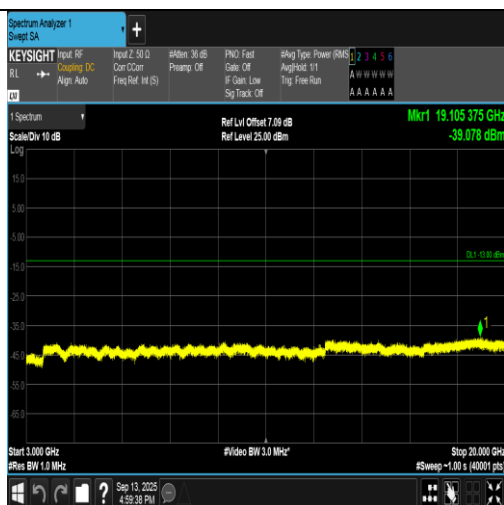
Band2-9262-2-3000~20000MHz-PASS
