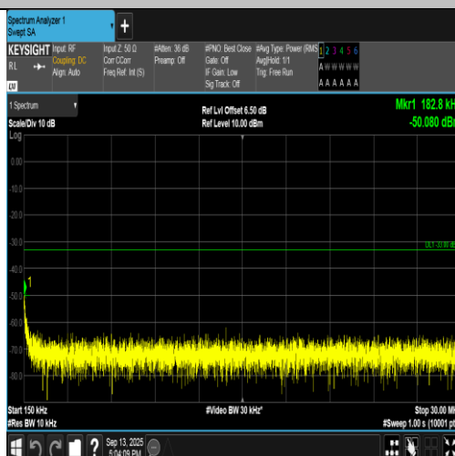
Band2-9262-4-0.15~30MHz-PASS
