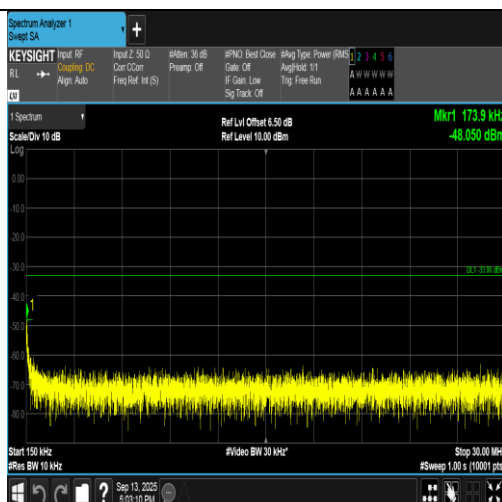
Band2-9538-3-0.15~30MHz-PASS
