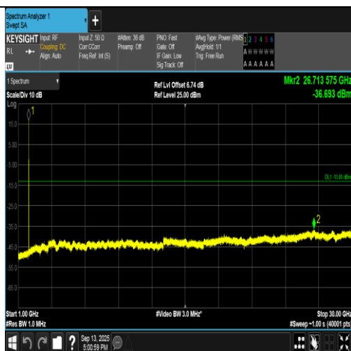
Band2-9538-2-1000~30000MHz-PASS
