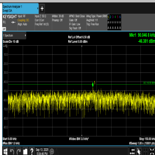
Band2-9400-4-0.009~0.15MHz-PASS
