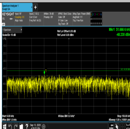
Band2-9400-2-0.009~0.15MHz-PASS
