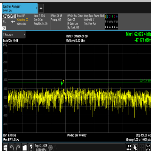
Band2-9262-2-0.009~0.15MHz-PASS
