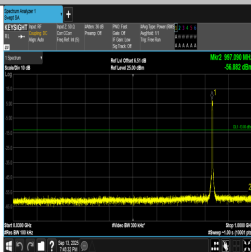
Band5-4182-2-30~1000MHz-PASS
