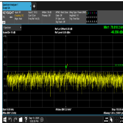
Band2-9538-2-0.009~0.15MHz-PASS
