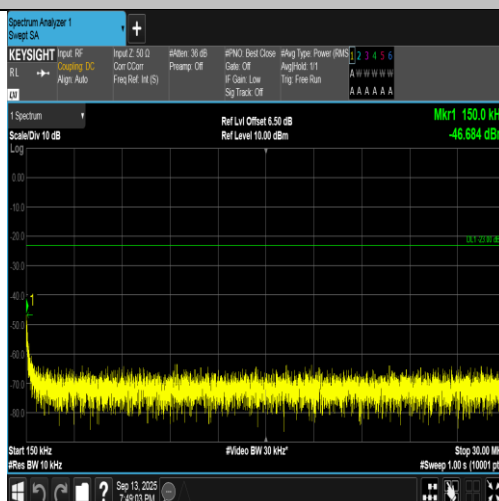
Band5-4132-4-0.15~30MHz-PASS
