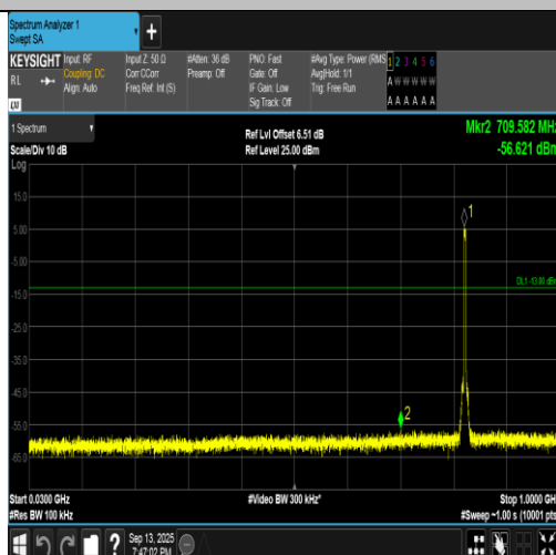
Band5-4132-3-30~1000MHz-PASS
