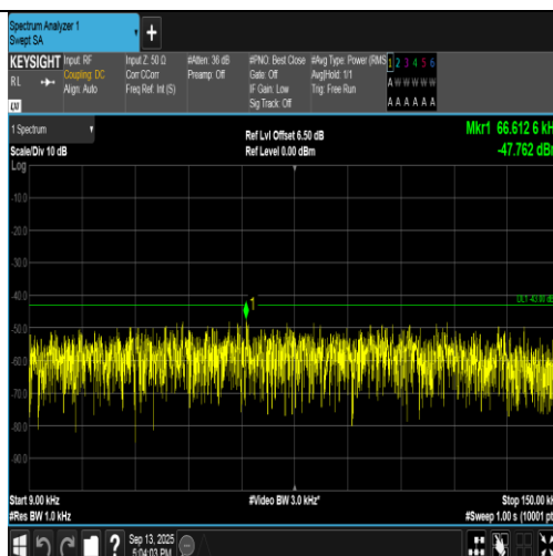
Band2-9262-4-0.009~0.15MHz-PASS
