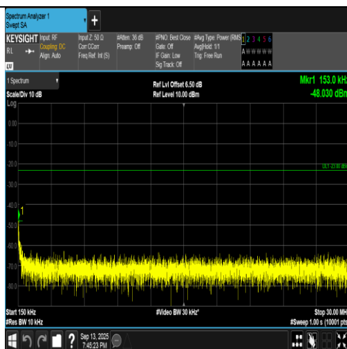
Band5-4182-2-0.15~30MHz-PASS
