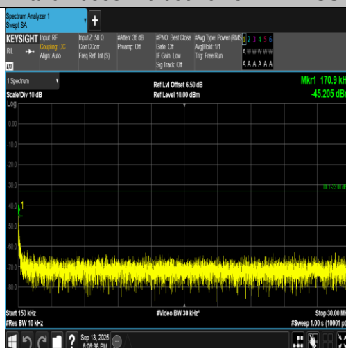
Band2-9538-4-0.15~30MHz-PASS
