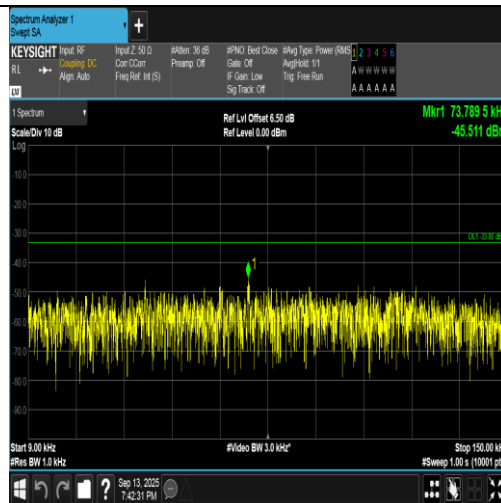
Band5-4132-1-0.009~0.15MHz-PASS
