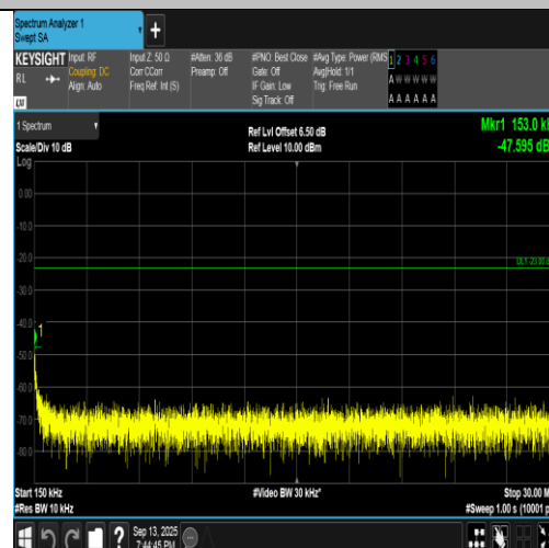
Band5-4132-2-0.15~30MHz-PASS
