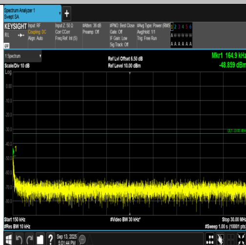
Band2-9262-3-0.15~30MHz-PASS
