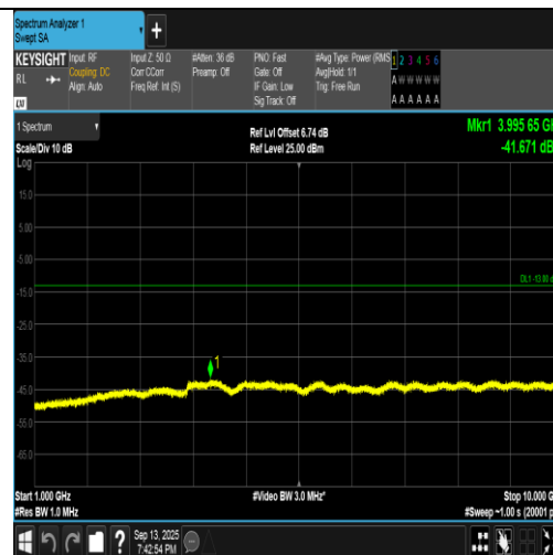
Band5-4132-1-1000~10000MHz-PASS
