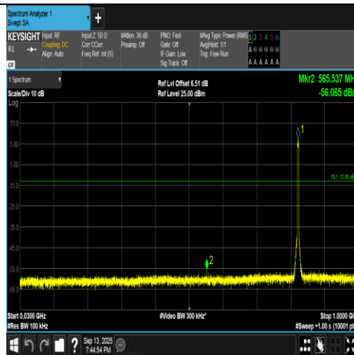
Band5-4132-2-30~1000MHz-PASS
