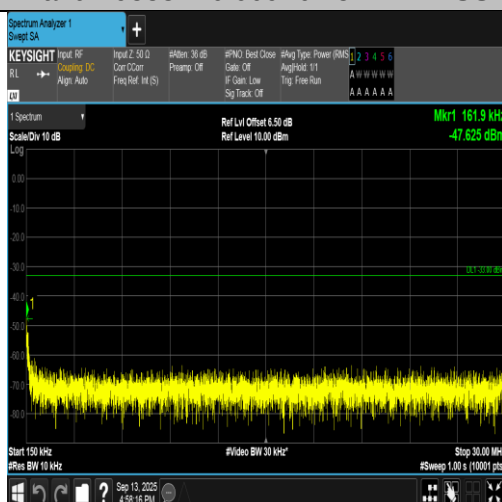
Band2-9538-1-0.15~30MHz-PASS
