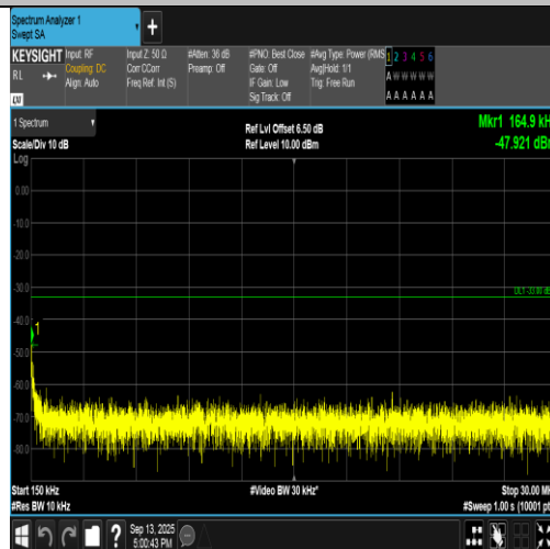
Band2-9538-2-0.15~30MHz-PASS
