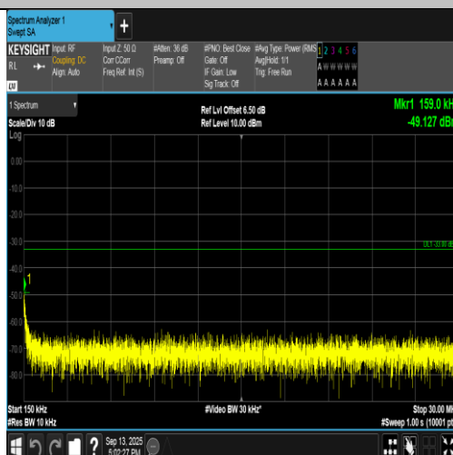
Band2-9400-3-0.15~30MHz-PASS
