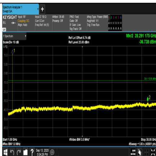
Band2-9262-4-1000~30000MHz-PASS
