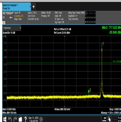
Band5-4132-1-30~1000MHz-PASS
