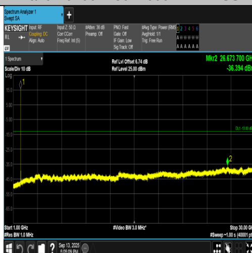
Band2-9400-4-1000~30000MHz-PASS
