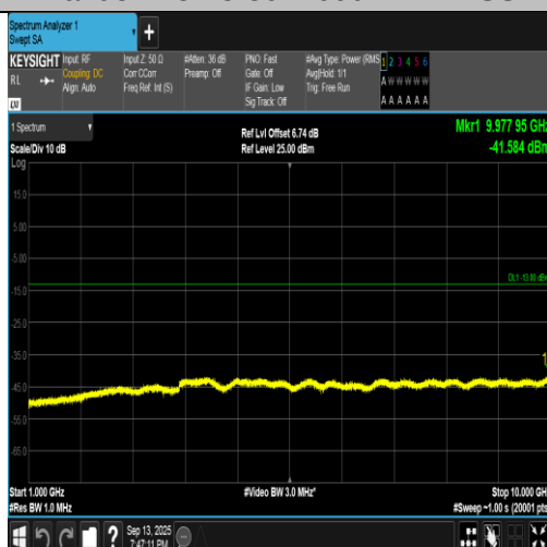
Band5-4132-3-1000~10000MHz-PASS
