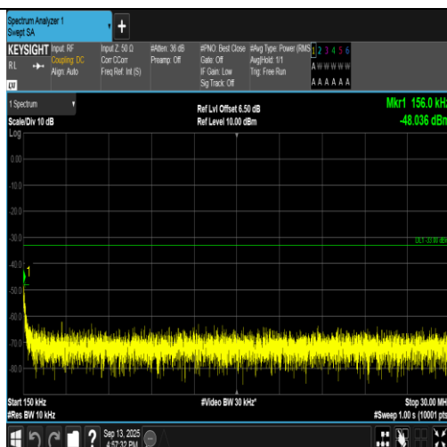
Band2-9400-1-0.15~30MHz-PASS
