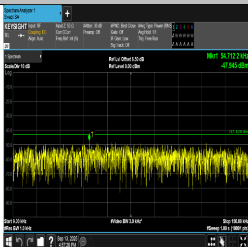
Band2-9400-1-0.009~0.15MHz-PASS
