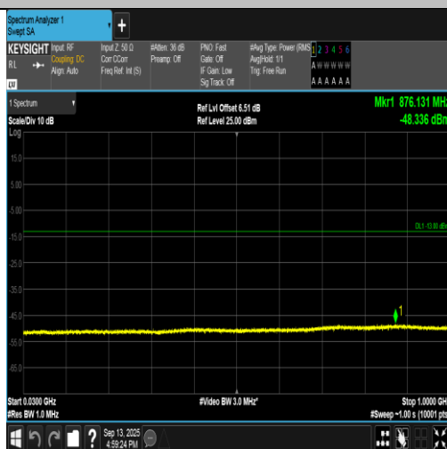
Band2-9262-2-30~1000MHz-PASS
