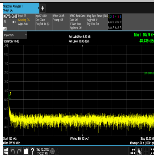
Band5-4132-1-0.15~30MHz-PASS
