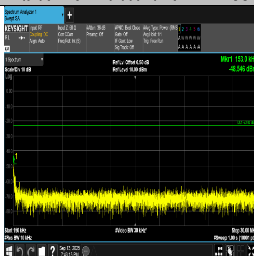
Band5-4182-1-0.15~30MHz-PASS
