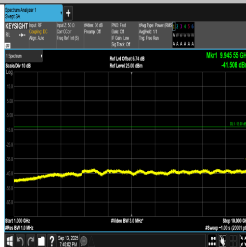
Band5-4132-2-1000~10000MHz-PASS
