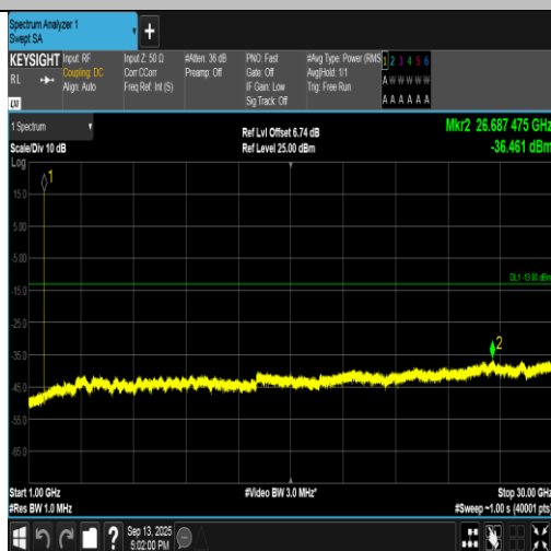
Band2-9262-3-1000~30000MHz-PASS
