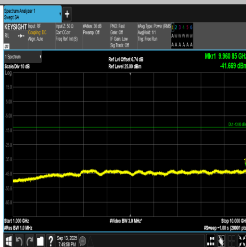
Band5-4182-4-1000~10000MHz-PASS
