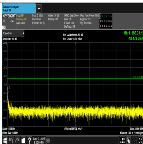
Band2-9262-5-0.15~30MHz-PASS
