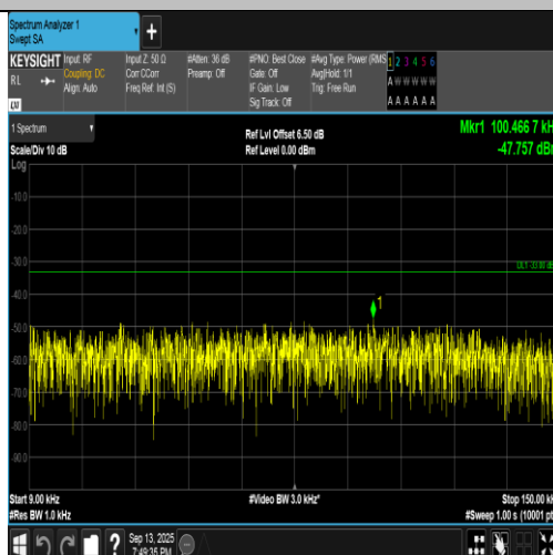
Band5-4182-4-0.009~0.15MHz-PASS
