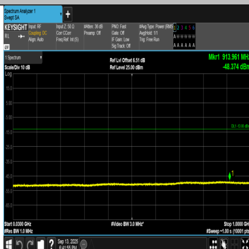
Band2-9262-2-30~1000MHz-PASS
