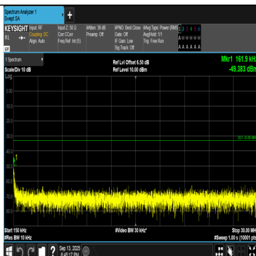
Band2-9400-3-0.15~30MHz-PASS
