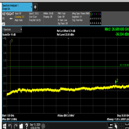
Band2-9262-5-1000~30000MHz-PASS
