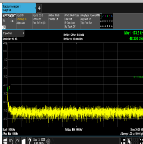
Band2-9538-3-0.15~30MHz-PASS
