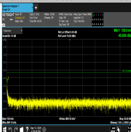
Band2-9400-1-0.15~30MHz-PASS
