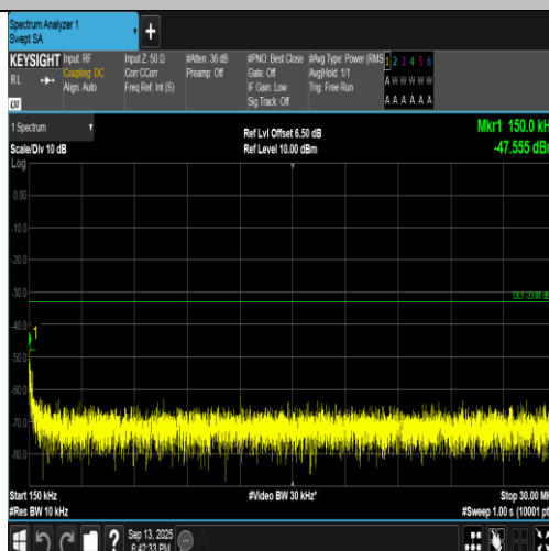
Band2-9400-2-0.15~30MHz-PASS
