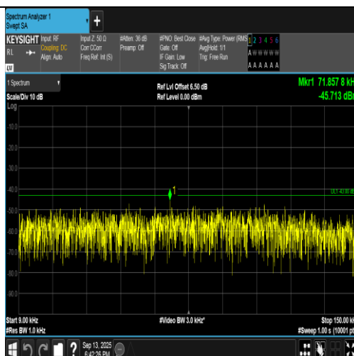
Band2-9400-2-0.009~0.15MHz-PASS
