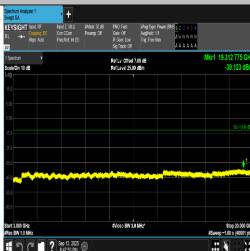
Band2-9262-4-3000~20000MHz-PASS
