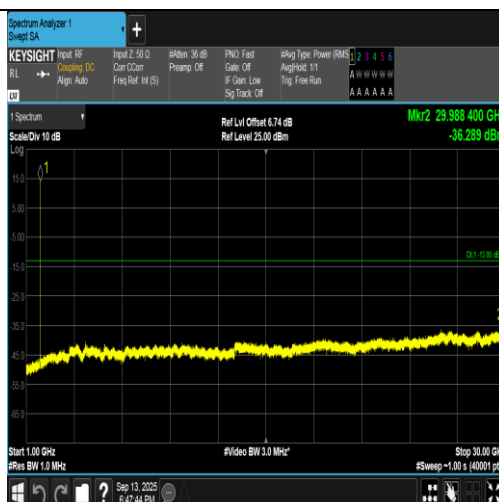
Band2-9262-4-1000~30000MHz-PASS
