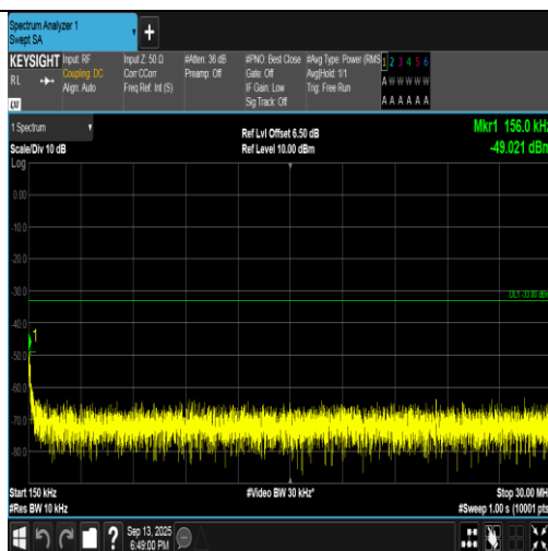
Band2-9538-4-0.15~30MHz-PASS
