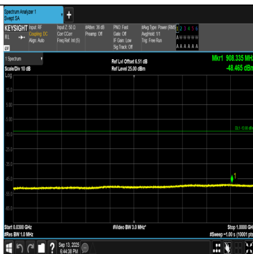
Band2-9262-3-30~1000MHz-PASS
