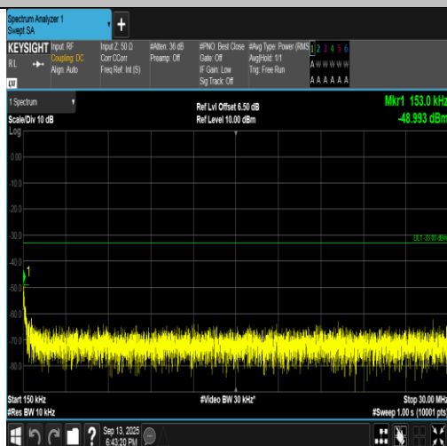
Band2-9538-2-0.15~30MHz-PASS
