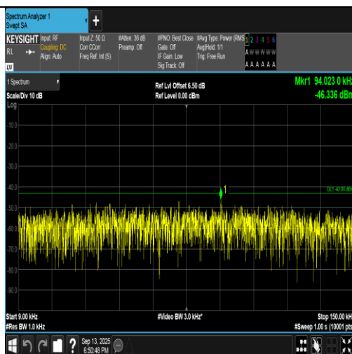
Band2-9400-5-0.009~0.15MHz-PASS
