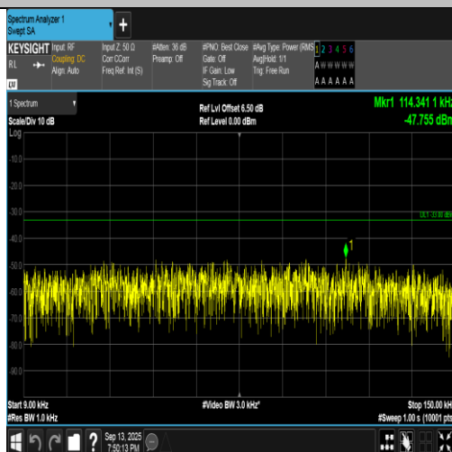
Band5-4233-4-0.009~0.15MHz-PASS
