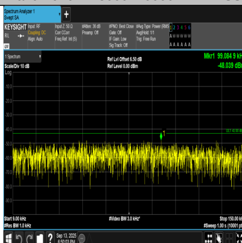
Band2-9262-5-0.009~0.15MHz-PASS
