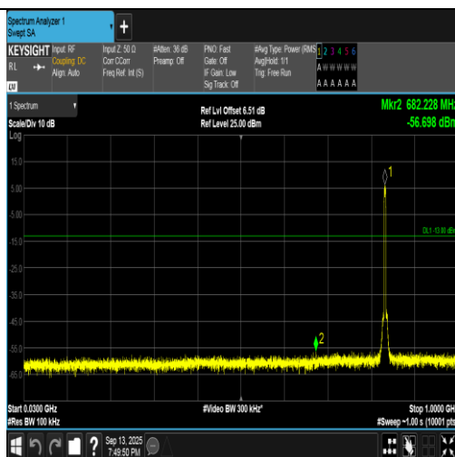
Band5-4182-4-30~1000MHz-PASS
