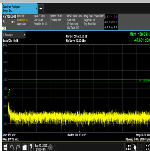
Band2-9400-5-0.15~30MHz-PASS
