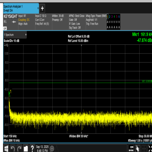
Band2-9400-4-0.15~30MHz-PASS
