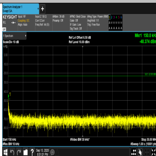
Band5-4132-1-0.15~30MHz-PASS
