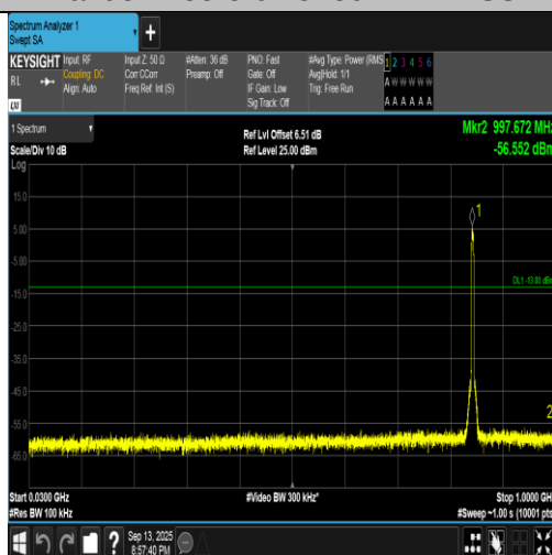
Band5-4233-3-30~1000MHz-PASS
