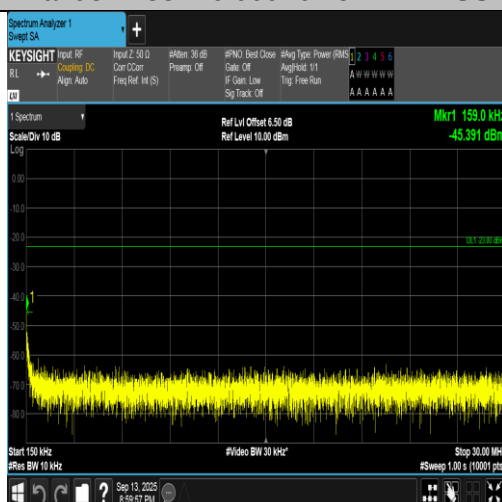
Band5-4233-4-0.15~30MHz-PASS
