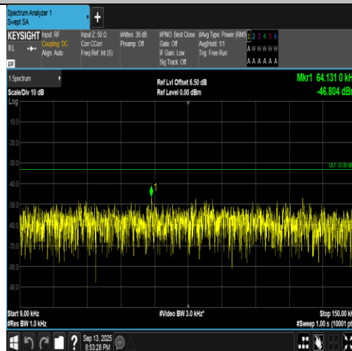
Band5-4132-2-0.009~0.15MHz-PASS
