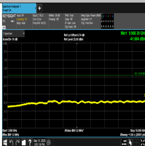
Band5-4132-5-1000~10000MHz-PASS
