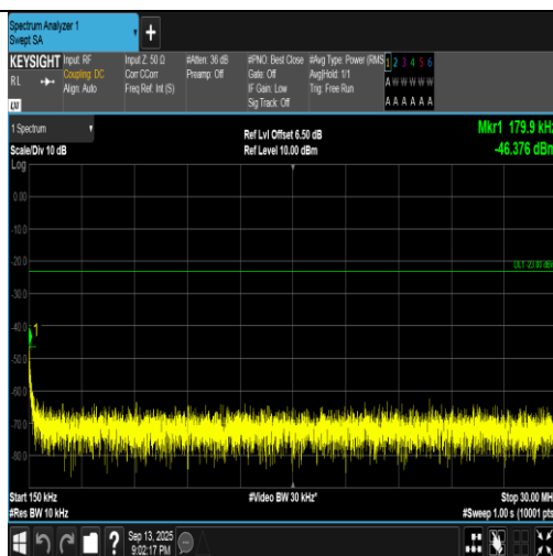
Band5-4233-5-0.15~30MHz-PASS
