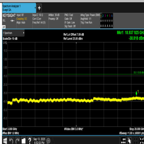
Band2-9538-5-3000~20000MHz-PASS
