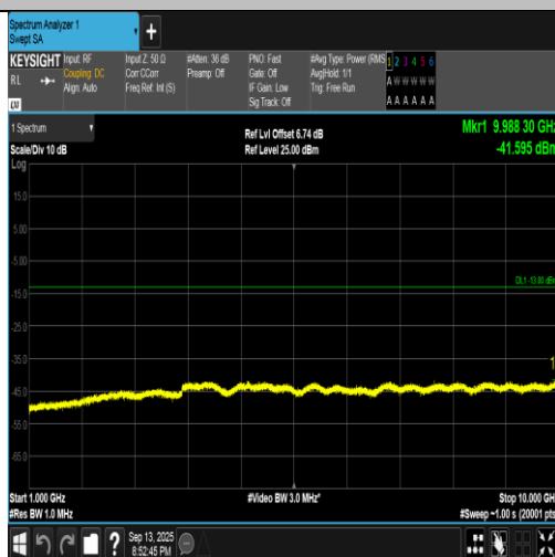
Band5-4233-1-1000~10000MHz-PASS
