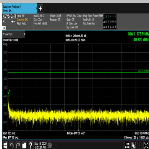
Band5-4182-5-0.15~30MHz-PASS
