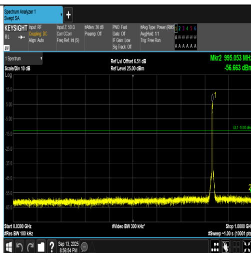
Band5-4182-3-30~1000MHz-PASS
