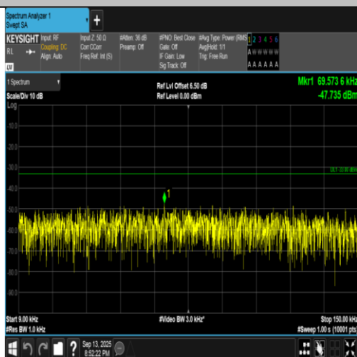
Band5-4233-1-0.009~0.15MHz-PASS
