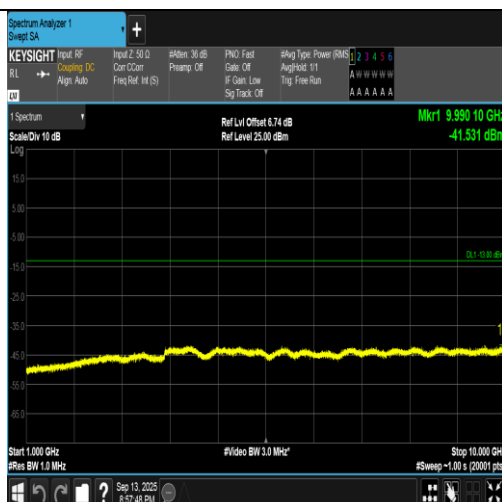
Band5-4233-3-1000~10000MHz-PASS
