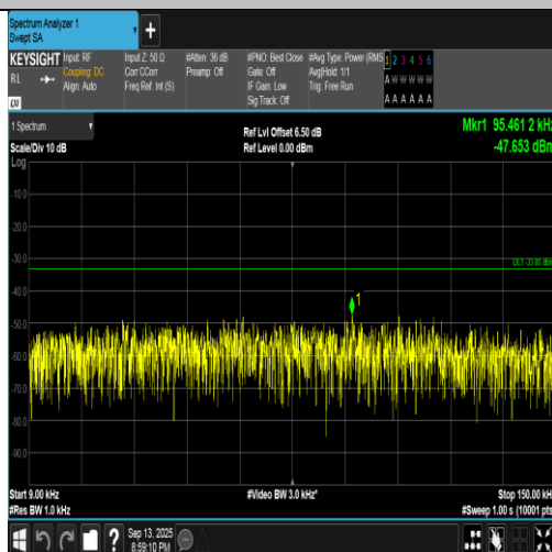
Band5-4182-4-0.009~0.15MHz-PASS
