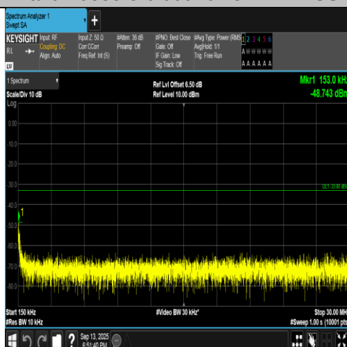
Band2-9538-5-0.15~30MHz-PASS
