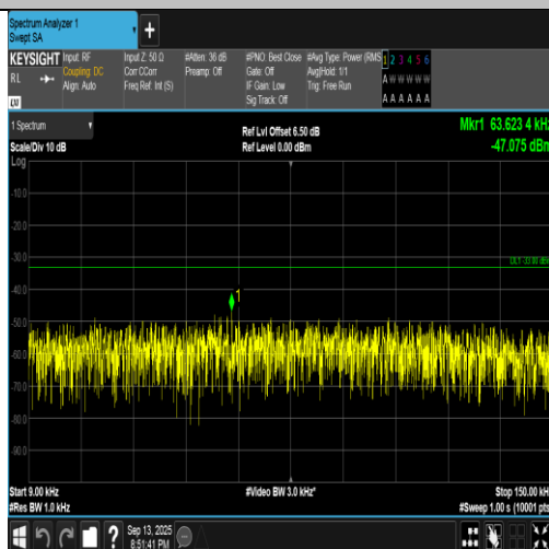
Band5-4182-1-0.009~0.15MHz-PASS
