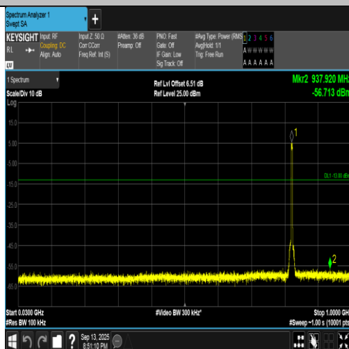
Band5-4132-1-30~1000MHz-PASS
