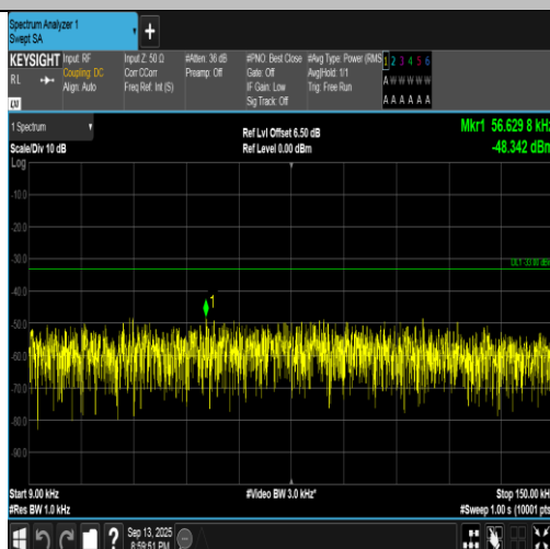
Band5-4233-4-0.009~0.15MHz-PASS
