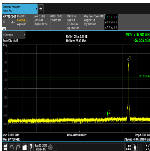
Band5-4233-4-30~1000MHz-PASS
