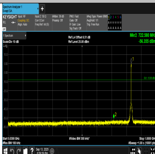
Band5-4182-4-30~1000MHz-PASS
