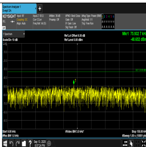
Band5-4233-3-0.009~0.15MHz-PASS
