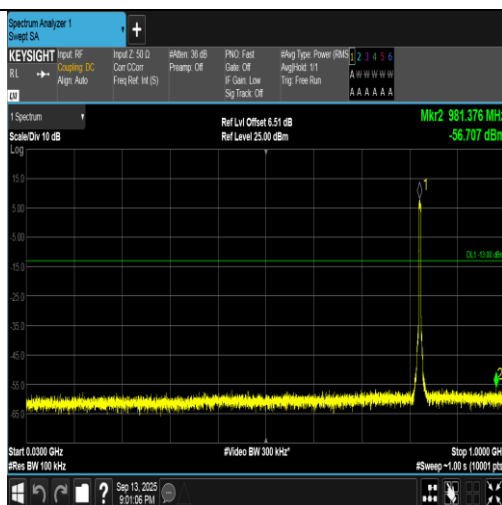
Band5-4132-5-30~1000MHz-PASS
