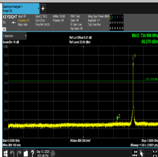
Band5-4182-5-30~1000MHz-PASS
