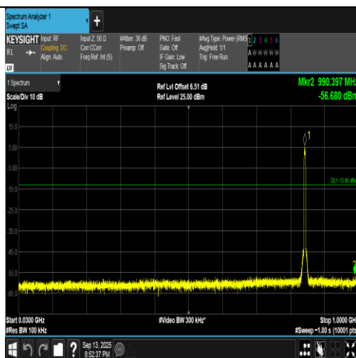
Band5-4233-1-30~1000MHz-PASS
