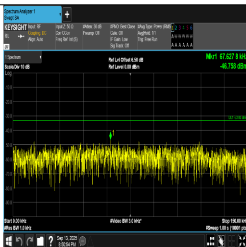
Band5-4132-1-0.009~0.15MHz-PASS
