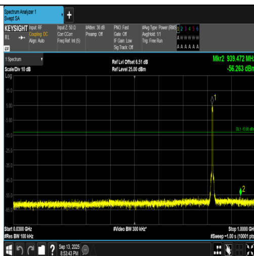
Band5-4132-2-30~1000MHz-PASS
