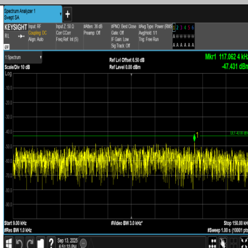
Band2-9538-5-0.009~0.15MHz-PASS
