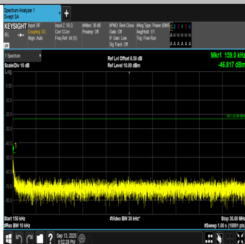
Band5-4233-1-0.15~30MHz-PASS
