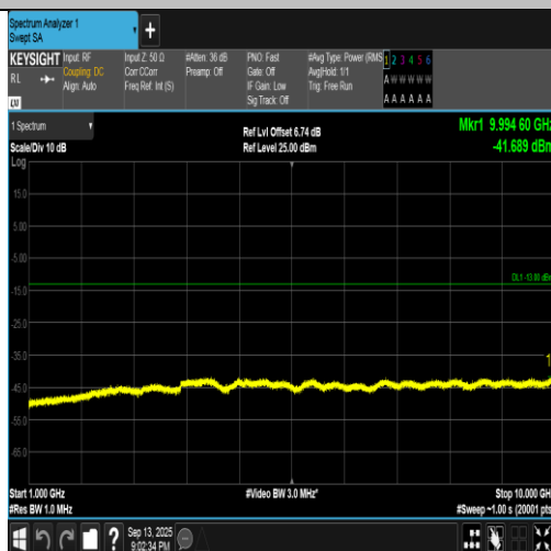
Band5-4233-5-1000~10000MHz-PASS
