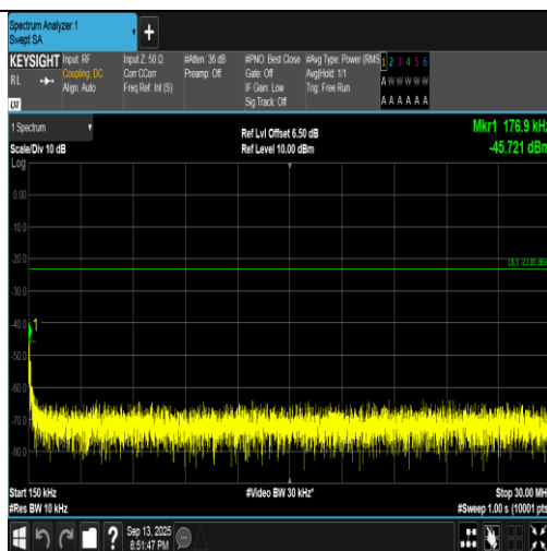
Band5-4182-1-0.15~30MHz-PASS
