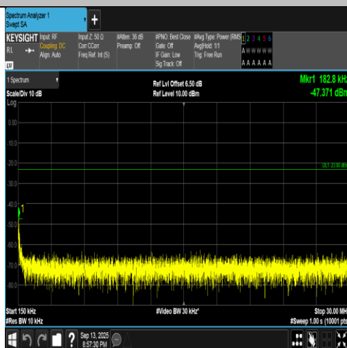
Band5-4233-3-0.15~30MHz-PASS
