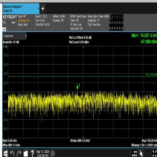
Band5-4132-3-0.009~0.15MHz-PASS
