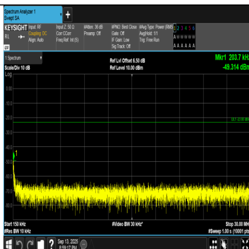
Band5-4182-4-0.15~30MHz-PASS
