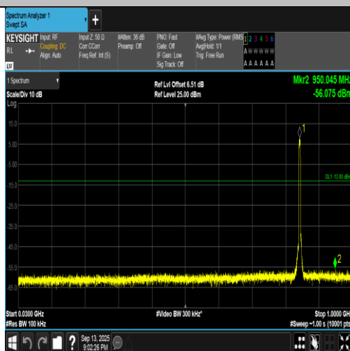
Band5-4233-5-30~1000MHz-PASS
