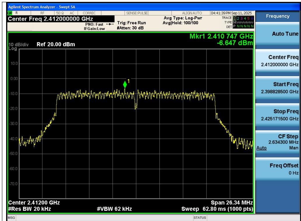
Test_Graph_802.11n20_ANT1_2412_MCS0_PSD
