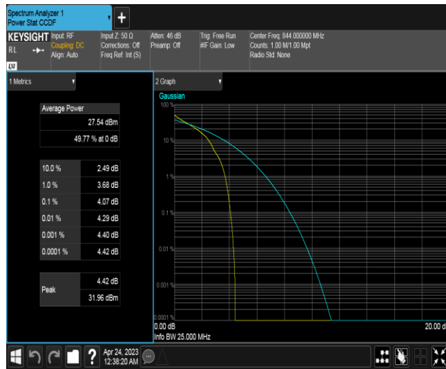
Band26-10MHz-QPSK-26990-50RB#0
