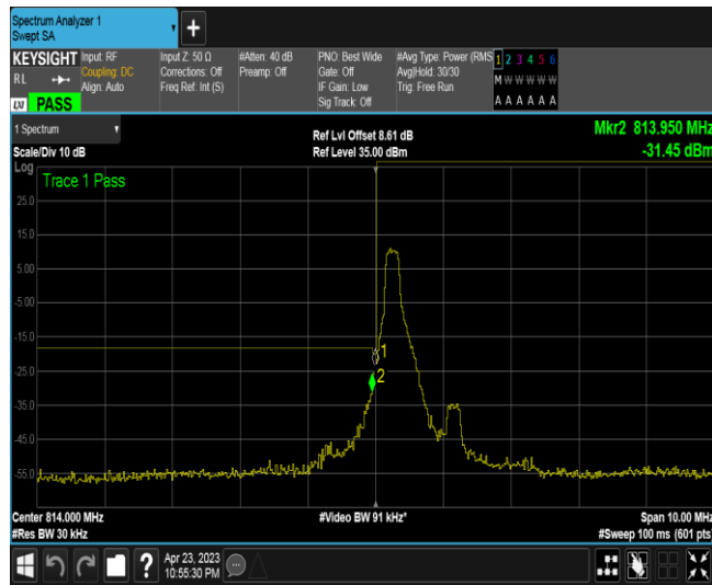
Band26-1.4MHz-16QAM-26697-1RB#5
