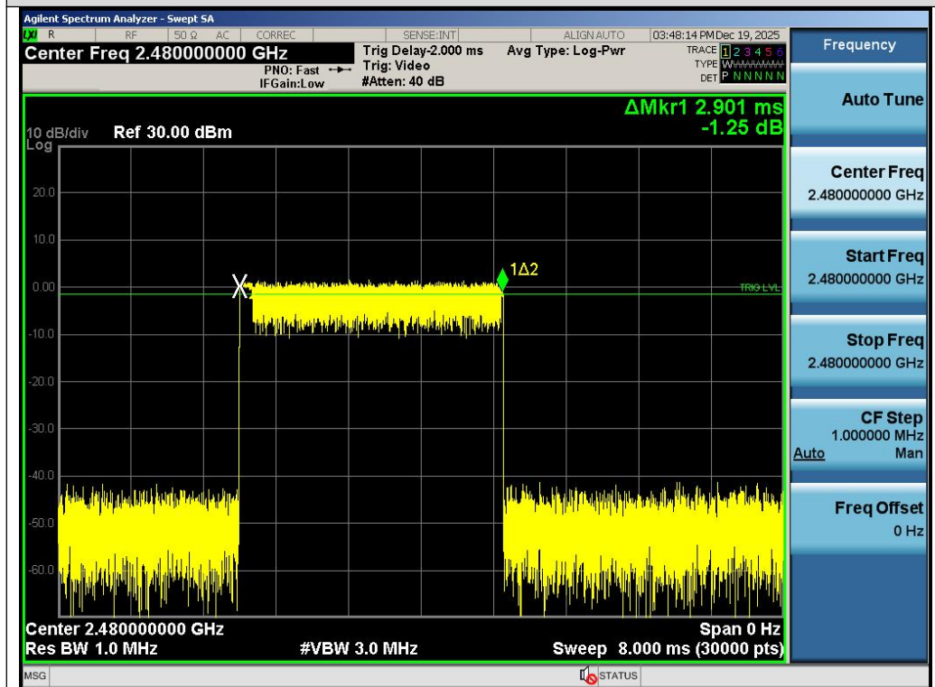
Test_Graph_EDR_HOP_ANT1_NA_2Mbps_2480_Number of Busrt
