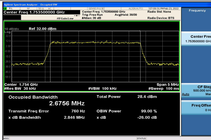
Band4-3MHz-QPSK-20385-15RB#0-2.6756
