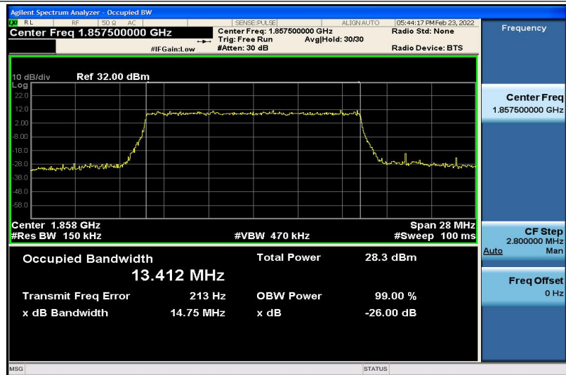
Band2-15MHz-16QAM-18675-75RB#0-13.412
