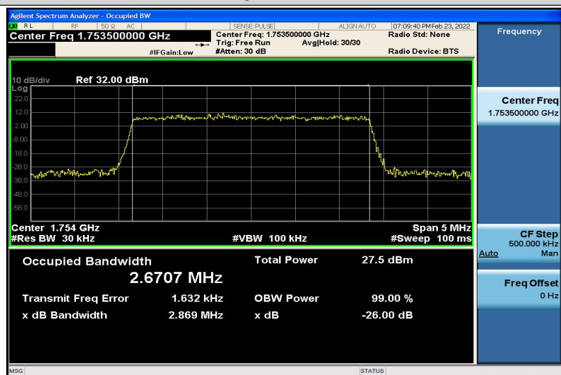
Band4-3MHz-16QAM-20385-15RB#0-2.6707
