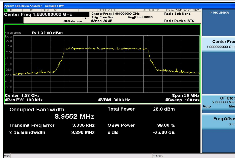
Band2-10MHz-16QAM-18900-50RB#0-8.9552
