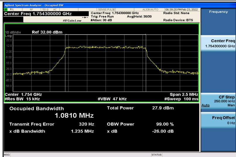
Band4-1.4MHz-QPSK-20393-6RB#0-1.0810
