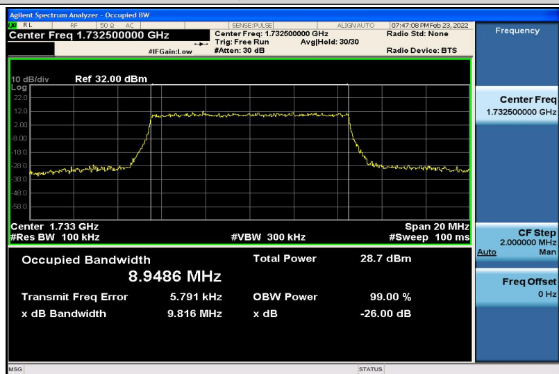
Band4-10MHz-QPSK-20175-50RB#0-8.9486
