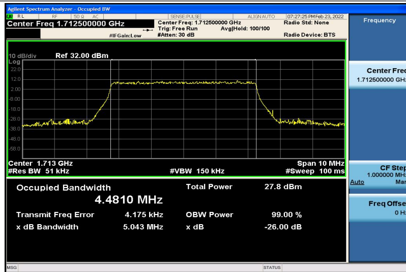
Band4-5MHz-16QAM-19975-25RB#0-4.4810
