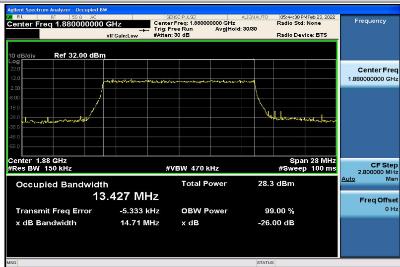
Band2-15MHz-16QAM-18900-75RB#0-13.427
