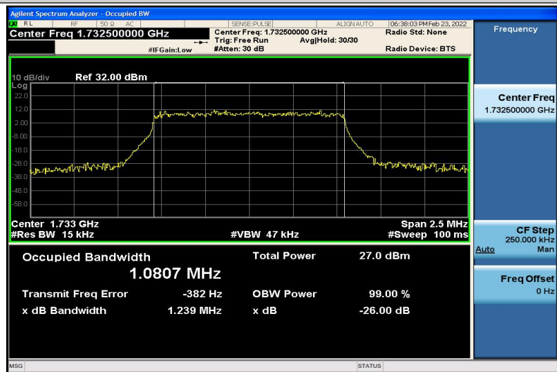
Band4-1.4MHz-16QAM-20175-6RB#0-1.0807
