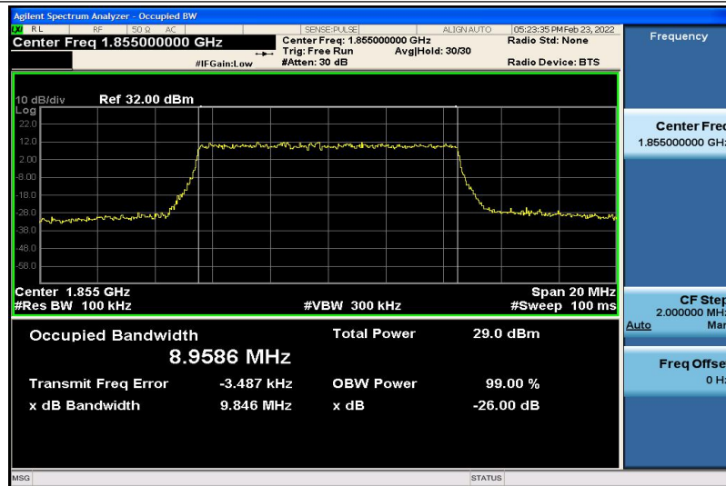
Band2-10MHz-QPSK-18650-50RB#0-8.9586
