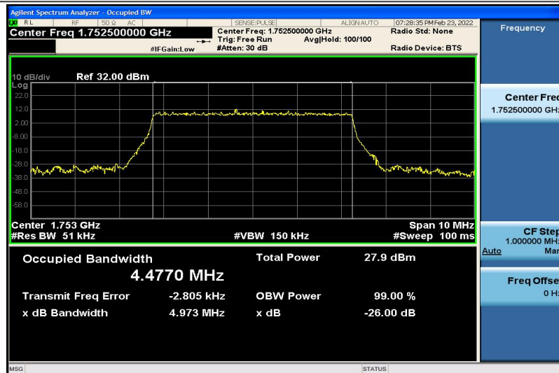
Band4-5MHz-16QAM-20375-25RB#0-4.4770
