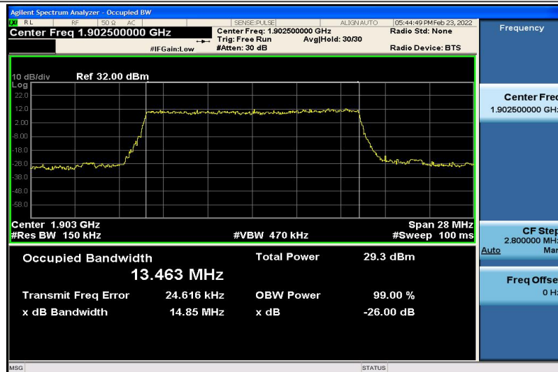
Band2-15MHz-QPSK-19125-75RB#0-13.463
