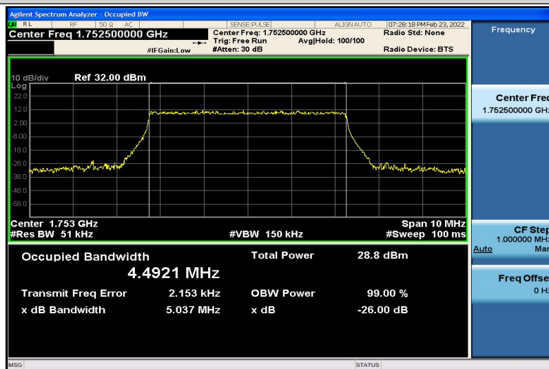
Band4-5MHz-QPSK-20375-25RB#0-4.4921
