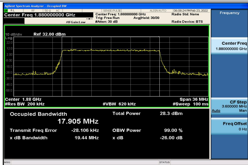
Band2-20MHz-16QAM-18900-100RB#0-17.905
