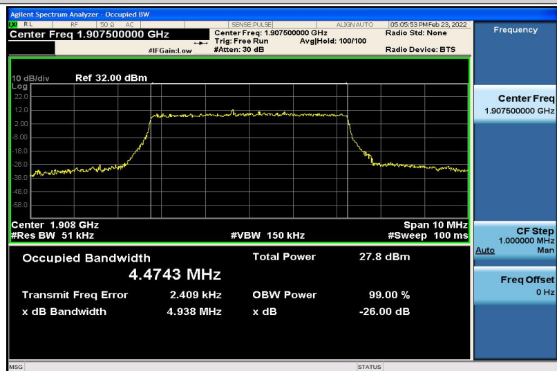
Band2-5MHz-16QAM-19175-25RB#0-4.4743
