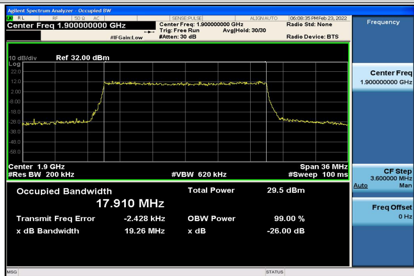
Band2-20MHz-QPSK-19100-100RB#0-17.910
