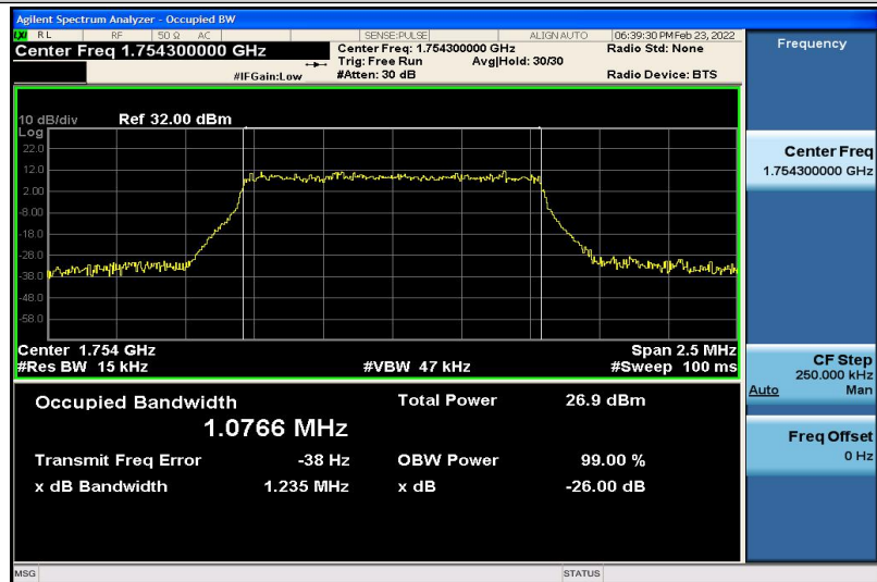
Band4-1.4MHz-16QAM-20393-6RB#0-1.0766
