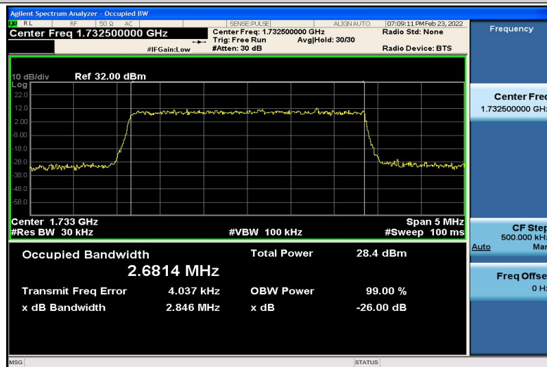
Band4-3MHz-QPSK-20175-15RB#0-2.6814
