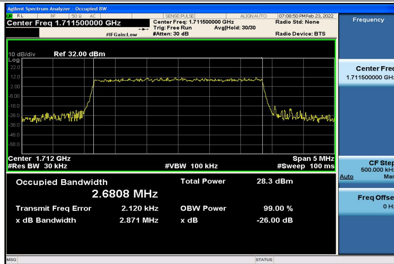
Band4-3MHz-QPSK-19965-15RB#0-2.6808
