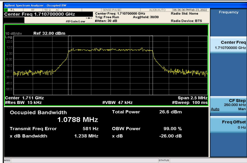
Band4-1.4MHz-16QAM-19957-6RB#0-1.0788
