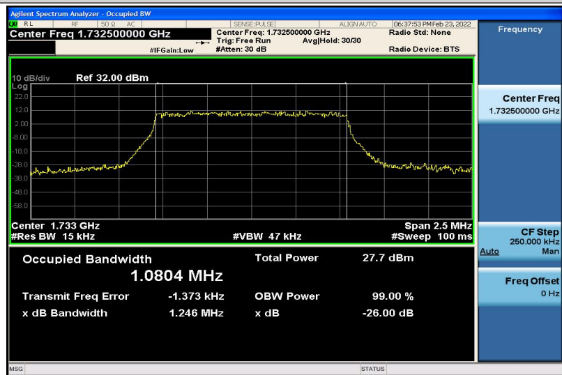
Band4-1.4MHz-QPSK-20175-6RB#0-1.0804
