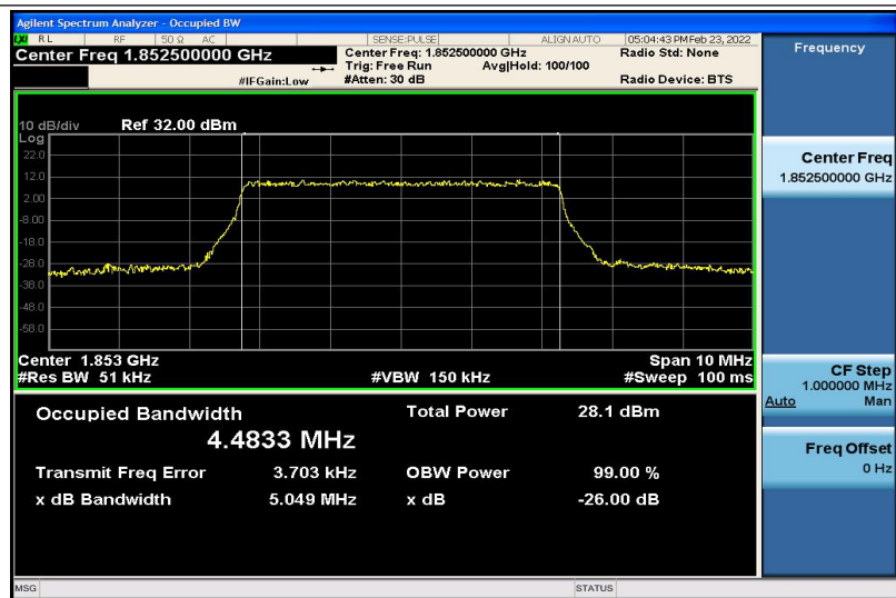
Band2-5MHz-16QAM-18625-25RB#0-4.4833
