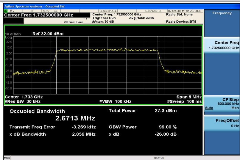
Band4-3MHz-16QAM-20175-15RB#0-2.6713
