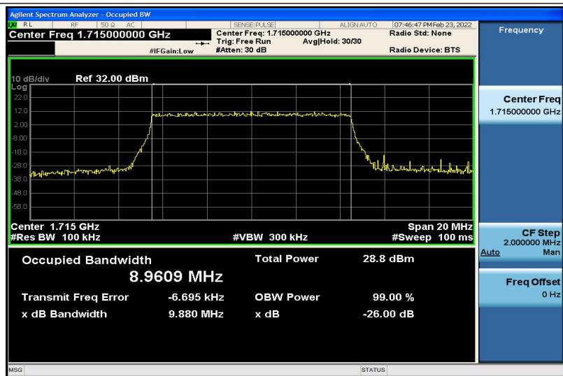
Band4-10MHz-QPSK-20000-50RB#0-8.9609
