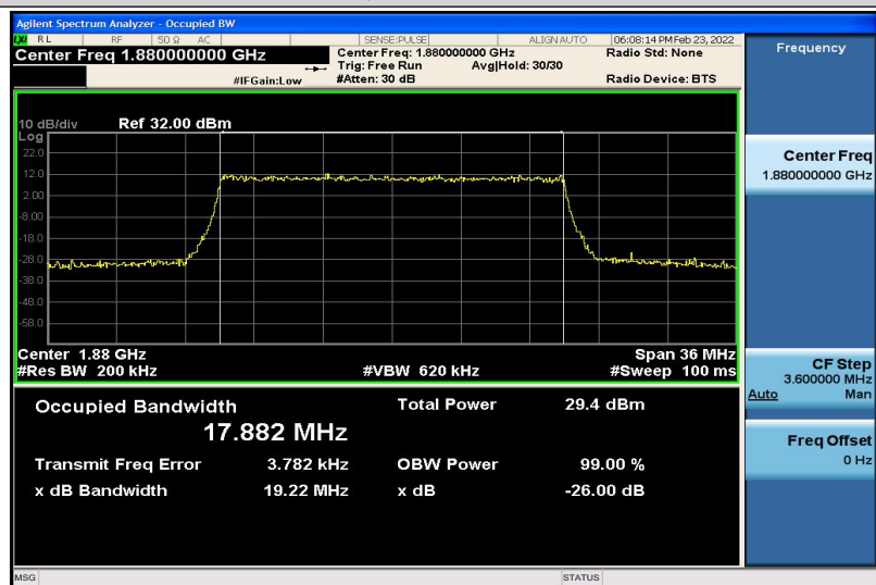
Band2-20MHz-QPSK-18900-100RB#0-17.882
