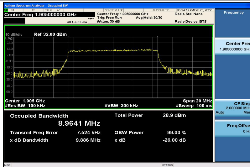
Band2-10MHz-QPSK-19150-50RB#0-8.9641
