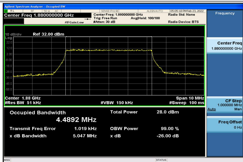
Band2-5MHz-16QAM-18900-25RB#0-4.4892
