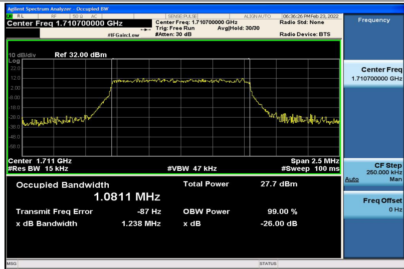
Band4-1.4MHz-QPSK-19957-6RB#0-1.0811
