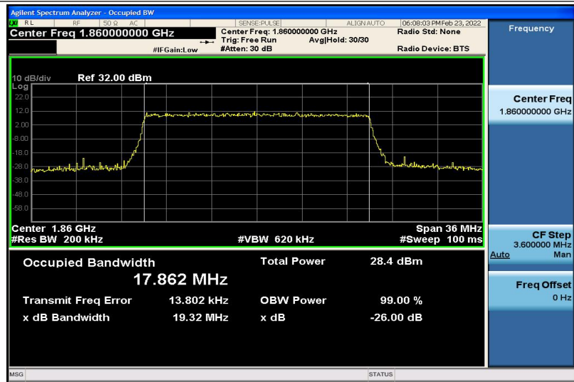
Band2-20MHz-16QAM-18700-100RB#0-17.862
