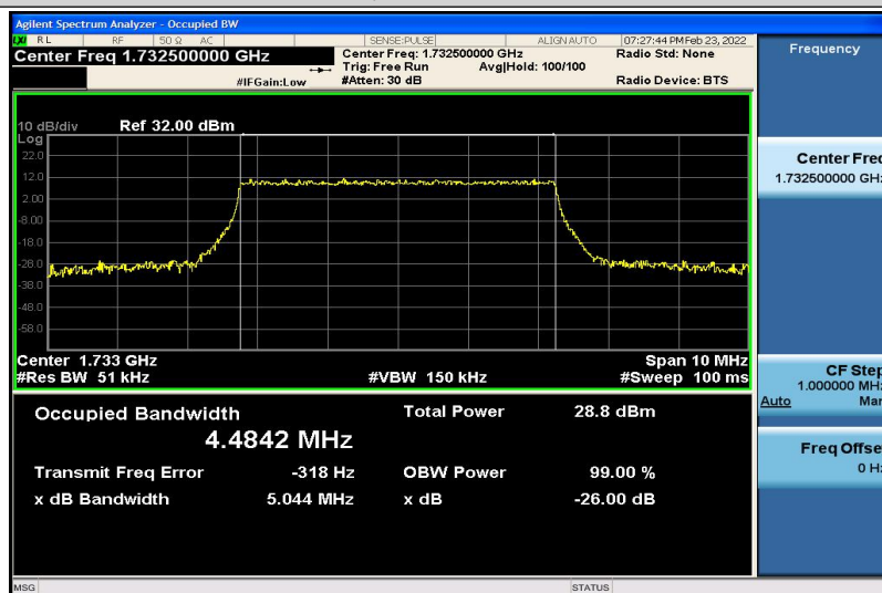
Band4-5MHz-QPSK-20175-25RB#0-4.4842
