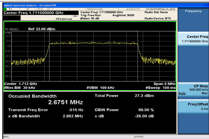
Band4-3MHz-16QAM-19965-15RB#0-2.6751
