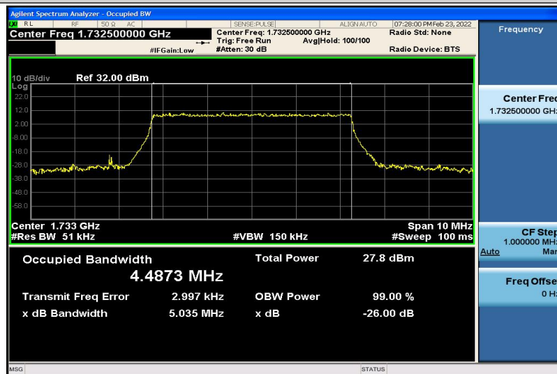
Band4-5MHz-16QAM-20175-25RB#0-4.4873
