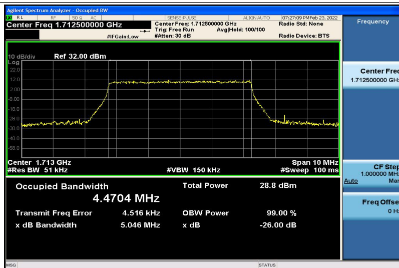
Band4-5MHz-QPSK-19975-25RB#0-4.4704
