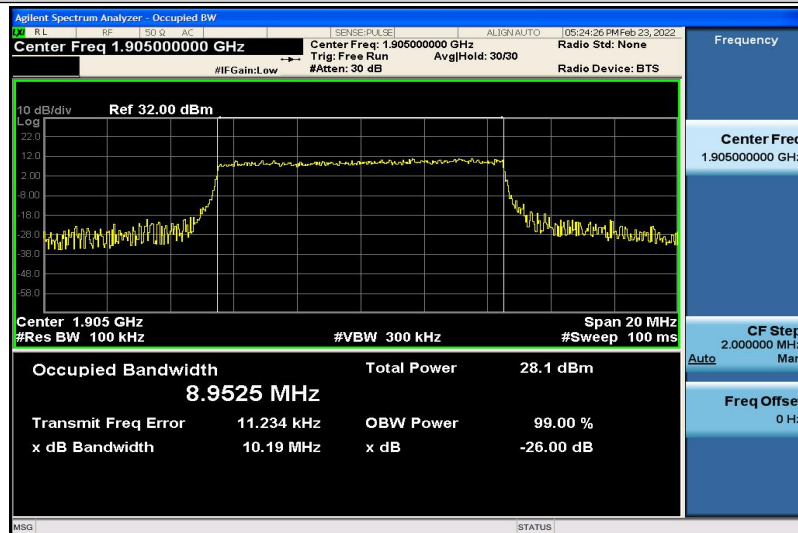
Band2-10MHz-16QAM-19150-50RB#0-8.9525
