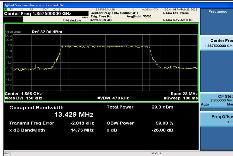
Band2-15MHz-QPSK-18675-75RB#0-13.429
