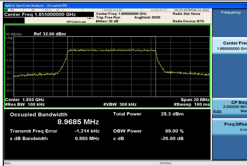
Band2-10MHz-16QAM-18650-50RB#0-8.9685
