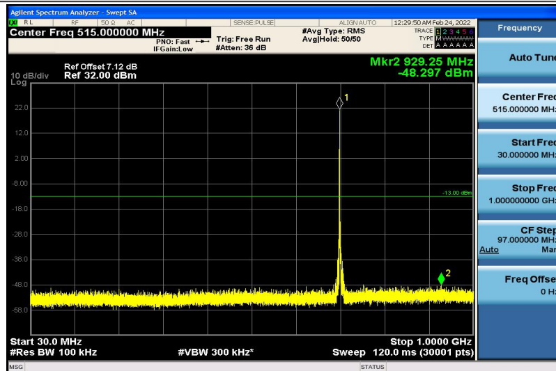
Band12-3MHz-16QAM-23095-1RB#0-30~1000MHz
