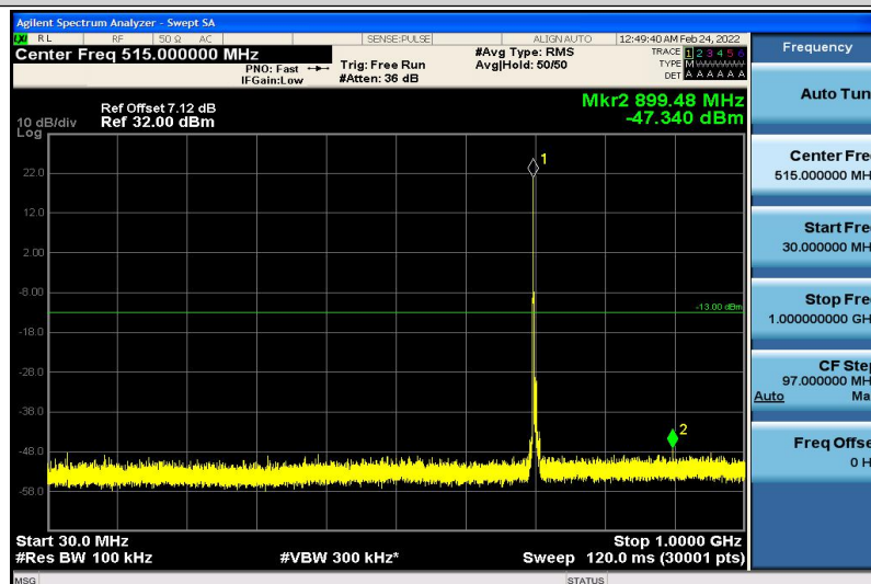
Band12-5MHz-16QAM-23095-1RB#0-30~1000MHz
