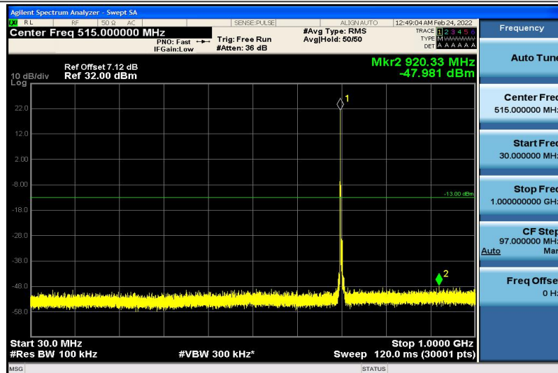
Band12-5MHz-QPSK-23095-1RB#0-30~1000MHz
