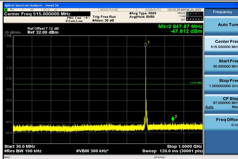
Band17-5MHz-QPSK-23790-1RB#0-30~1000MHz
