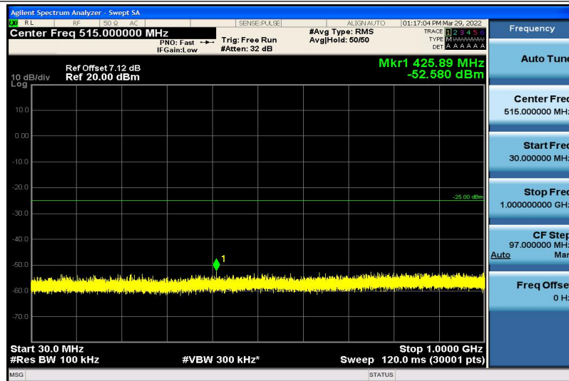
Band41-10MHz-16QAM-40640-1RB#0-30~1000MHz
