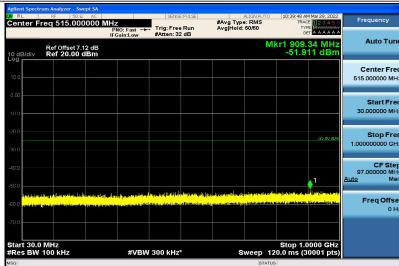
Band41-10MHz-16QAM-41190-1RB#0-30~1000MHz
