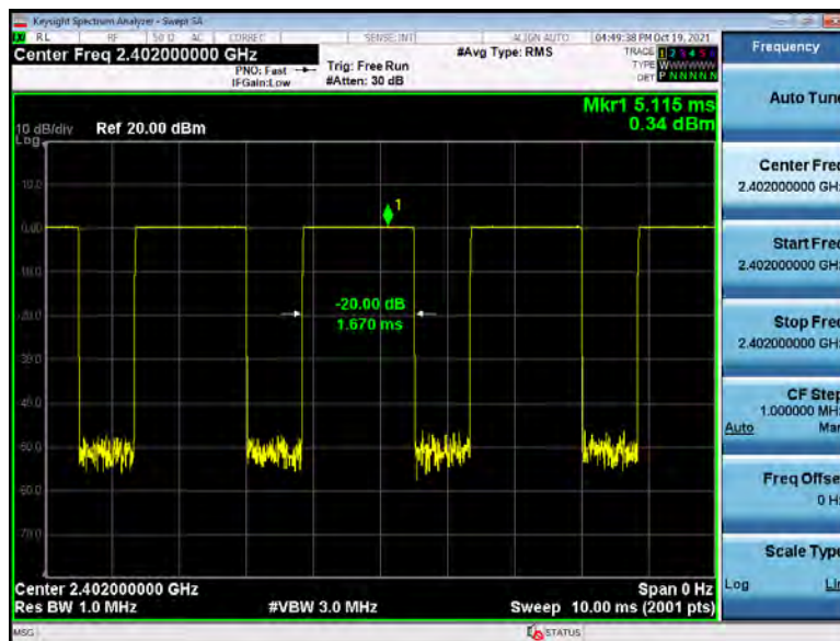
GFSK DH3 2402MHZ
