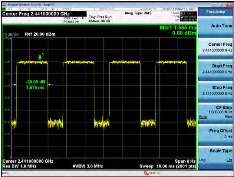
8-DPSK 3DH3 2441MHZ
