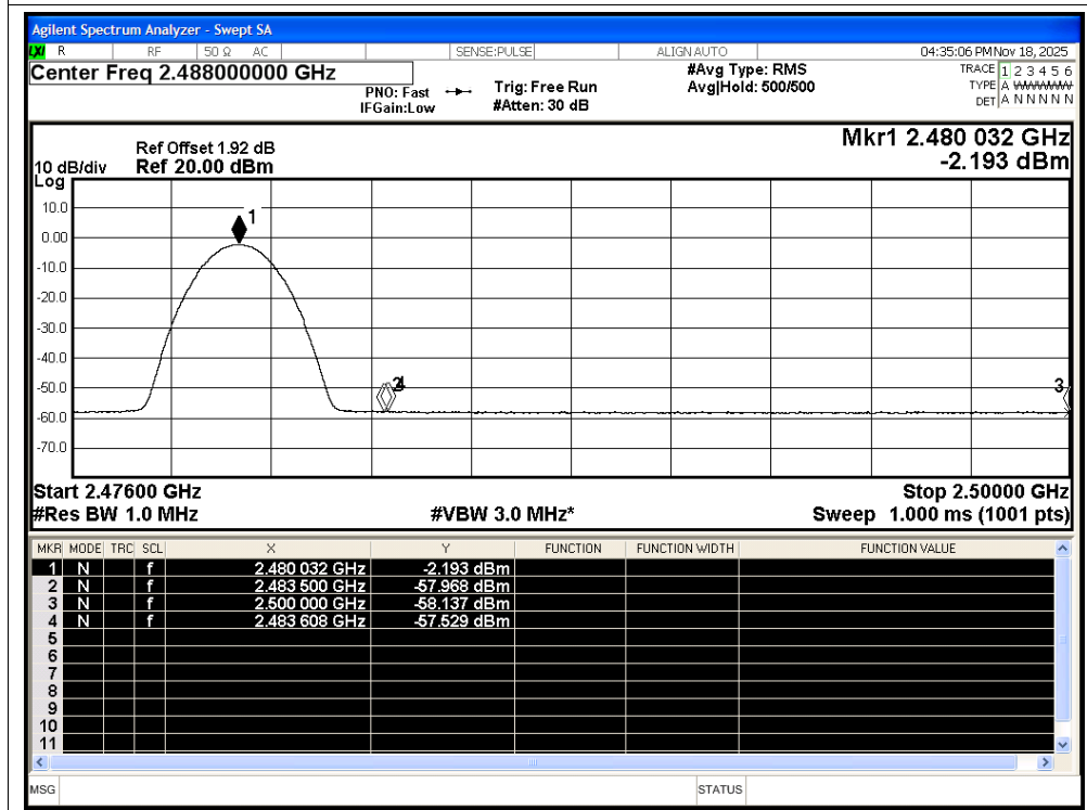
Restrict Band NVNT BLE 1M 2480MHz Ant1 Average
