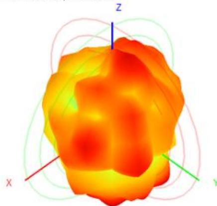
5850.0MHz H+V, Eff: 34.6%
