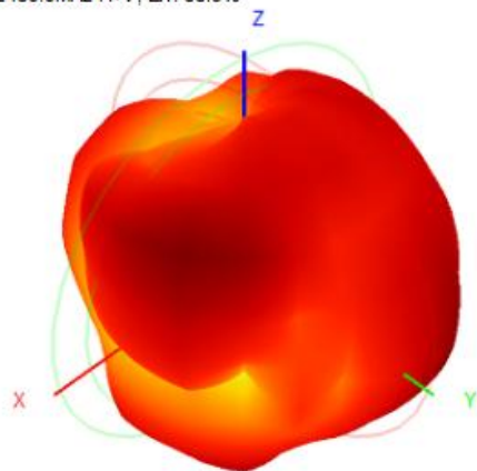
2450.0MHz H+V, Eff: 33.9%
