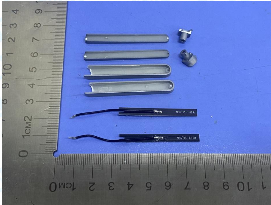
Photo 13 Appearance of Antenna
