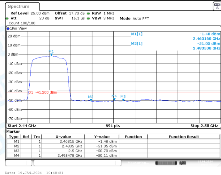
11N20-MIMO_Ant2_High_2462_Peak
