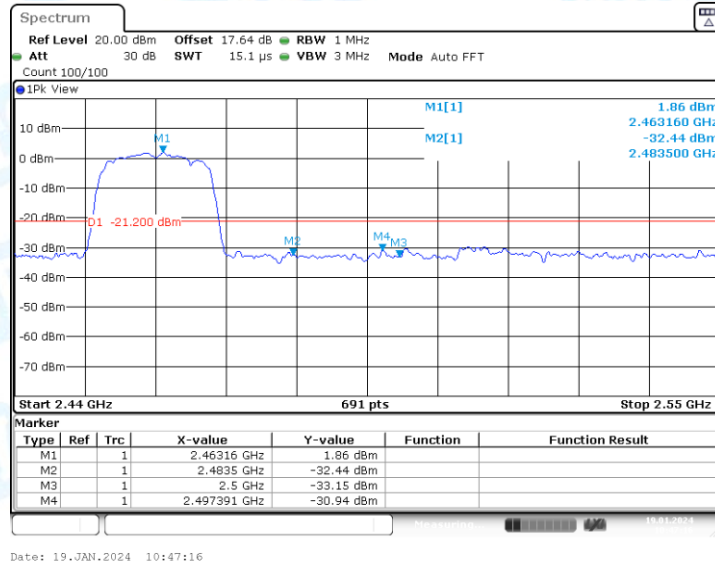
11N20-MIMO_Ant2_High_2462_AV
