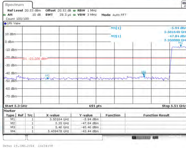
11AC20-MIMO_Ant2_Low_5500_AV
