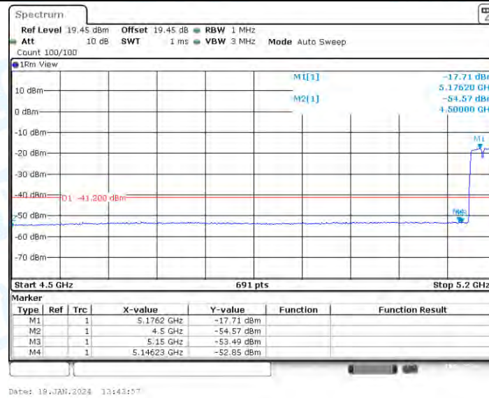
11N20-MIMO_Ant1_Low_5180_Peak
