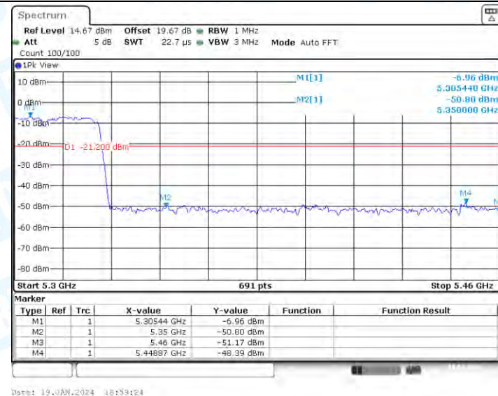
11AC40-MIMO_Ant2_High_5310_AV
