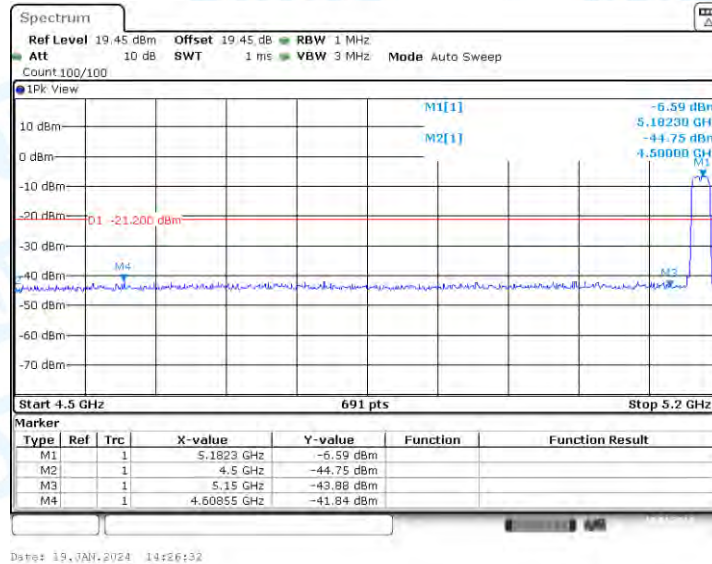
11AC20-MIMO_Ant2_Low_5180_AV
