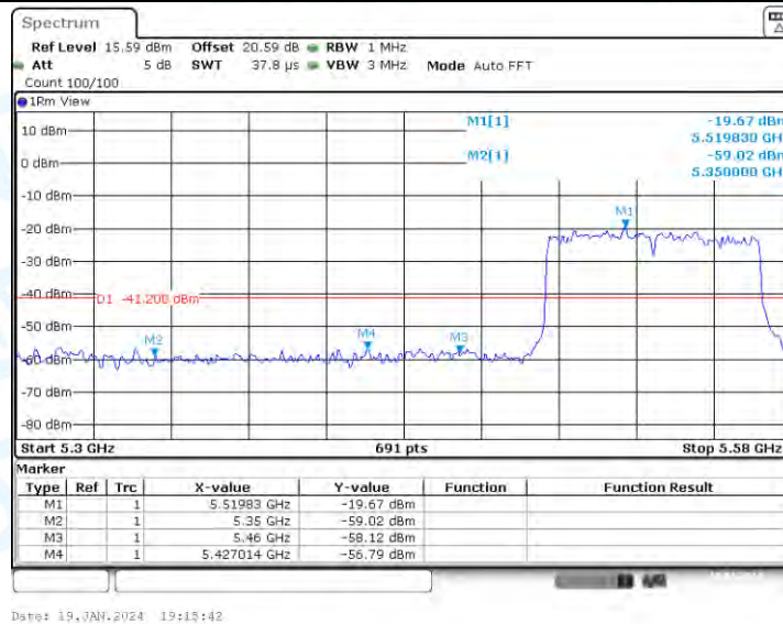
11AC80-MIMO_Ant2_Low_5530_Peak
