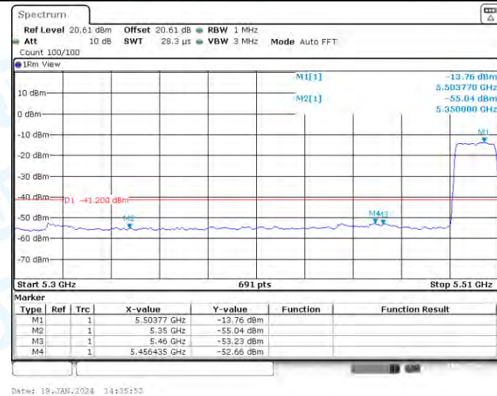
11AC20-MIMO_Ant2_Low_5500_Peak
