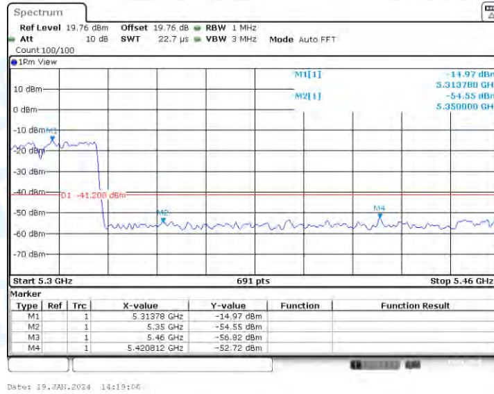
11N40-MIMO_Ant2_High_5310_Peak
