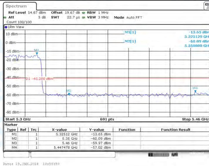
11AC40-MIMO_Ant1_High_5310_Peak
