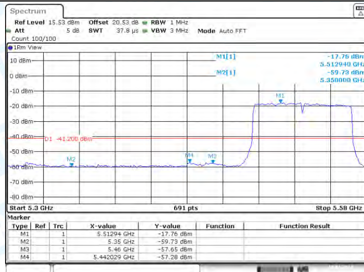
11AC80-MIMO_Ant1_Low_5530_AV
