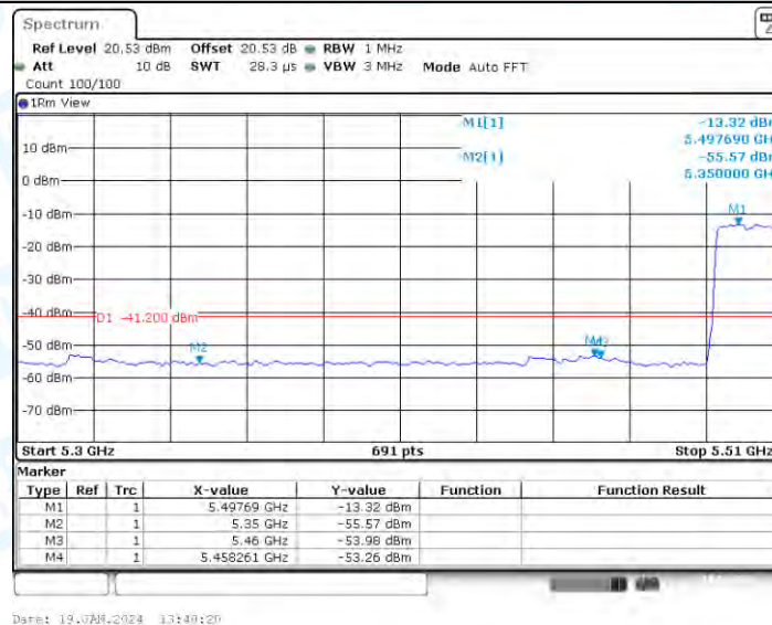
11A-CCD_Ant1_Low_5500_Peak
