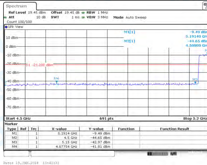
11N20-MIMO_Ant2_Low_5180_AV
