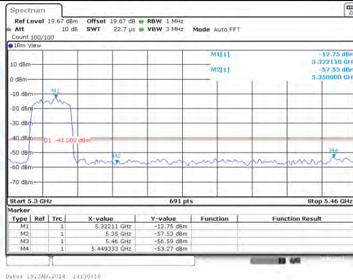
11AC20-MIMO_Ant1_High_5320_Peak
