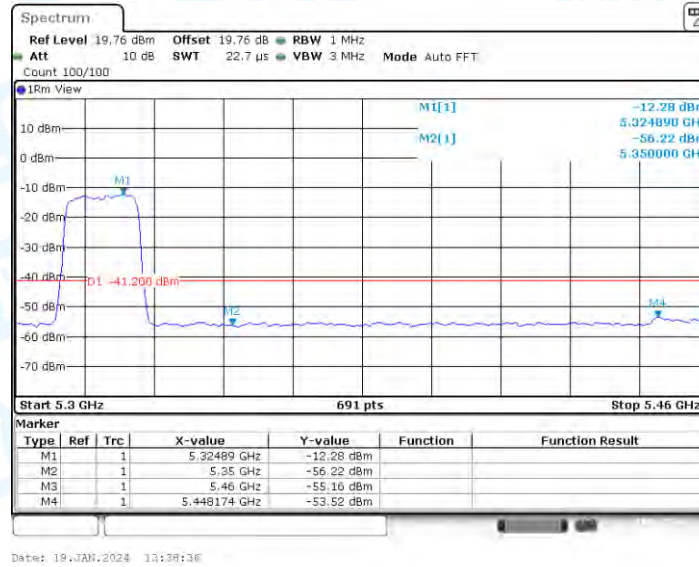
11A-CCD_Ant2_High_5320_Peak
