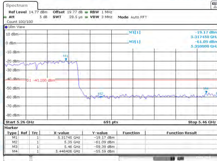
11AC80-MIMO_Ant2_High_5290_Peak
