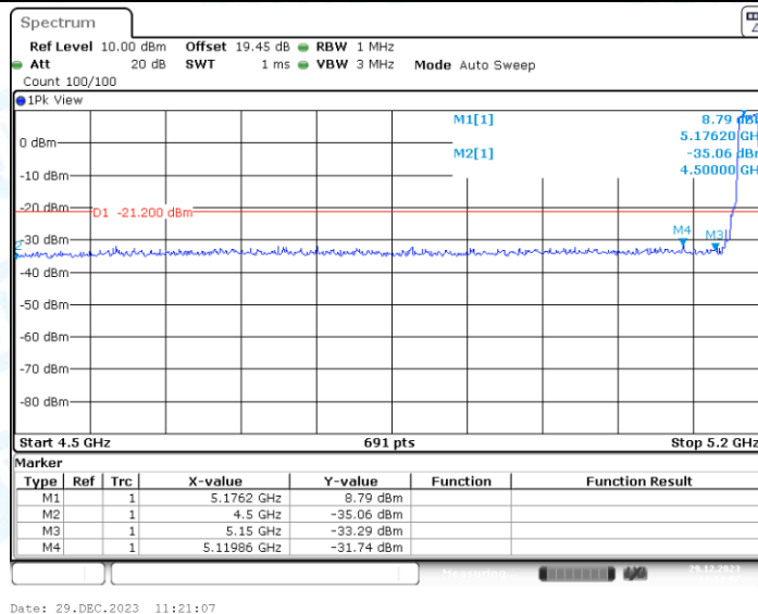
11AC20SISO_Ant1_High_5240_AV
