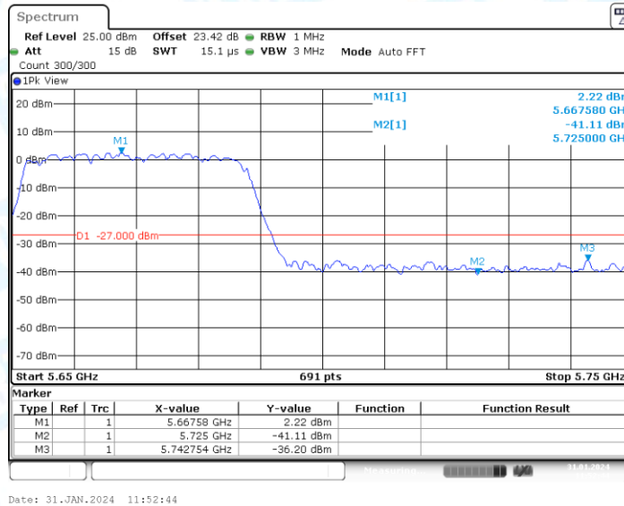
11N40MIMO_Ant2_High_5670
