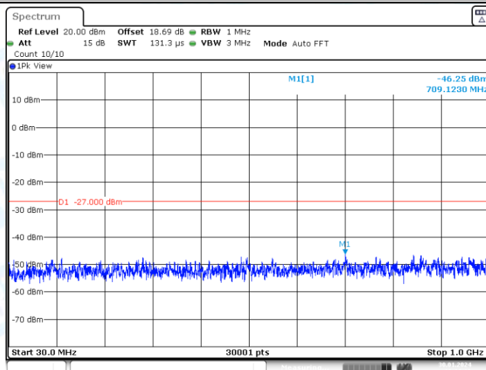
11A-CDD_Ant1_5785_30~1000
