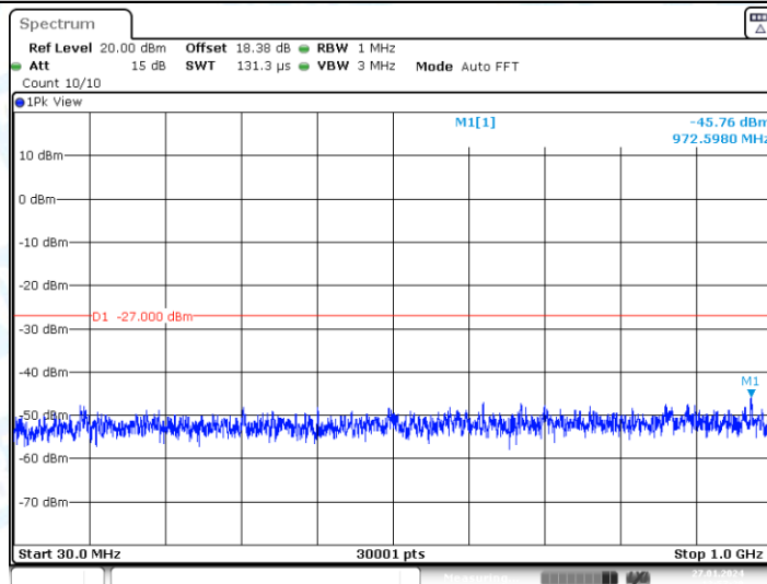
11A-CDD_Ant1_5200_30~1000
