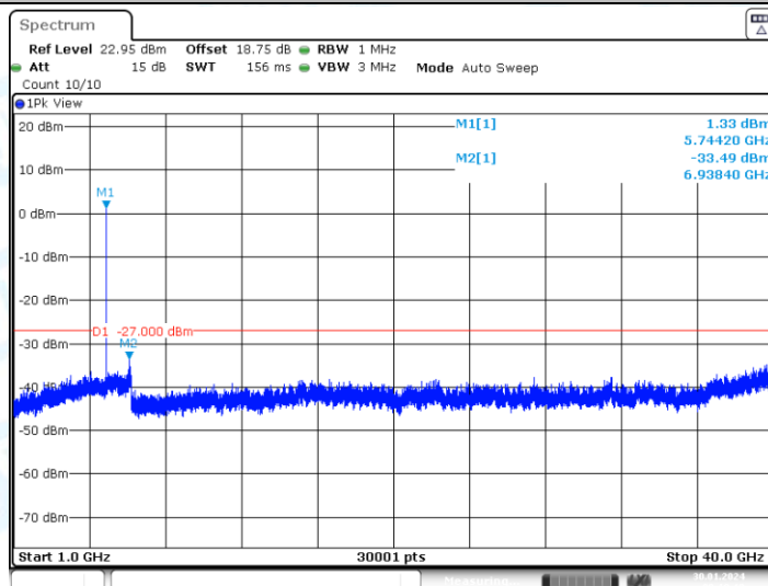
11A-CDD_Ant2_5745_1000~40000
