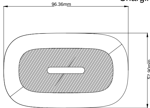
Charging box
