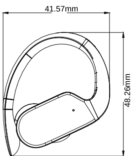
Headset
