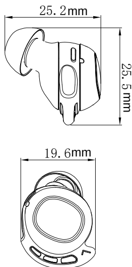
Headset
